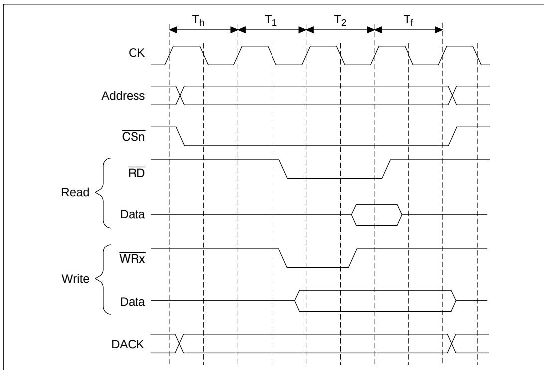
Figure 10.6 \overline{\text{CS}} Assert Period Extension Function
