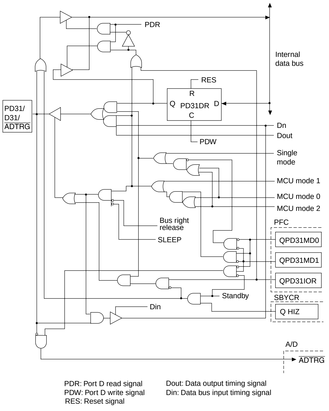
Figure B.31 PD31/D31/ADTRG Block Diagram
