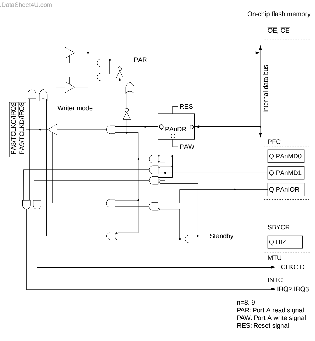
Figure B.6 PAn/TCLKm/IRQx Block Diagram (F-ZTAT Version)
