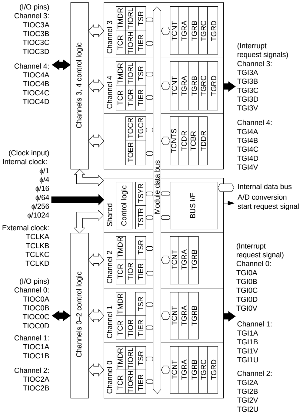
Figure 12.1 MTU Block Diagram
