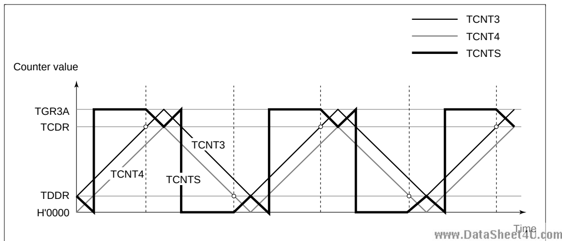
Figure 12.39 Complementary PWM Mode Counter Operation
