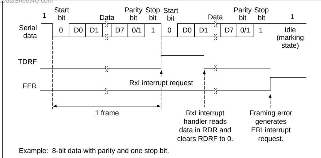
Figure 14.9 SCI Receive Operation
