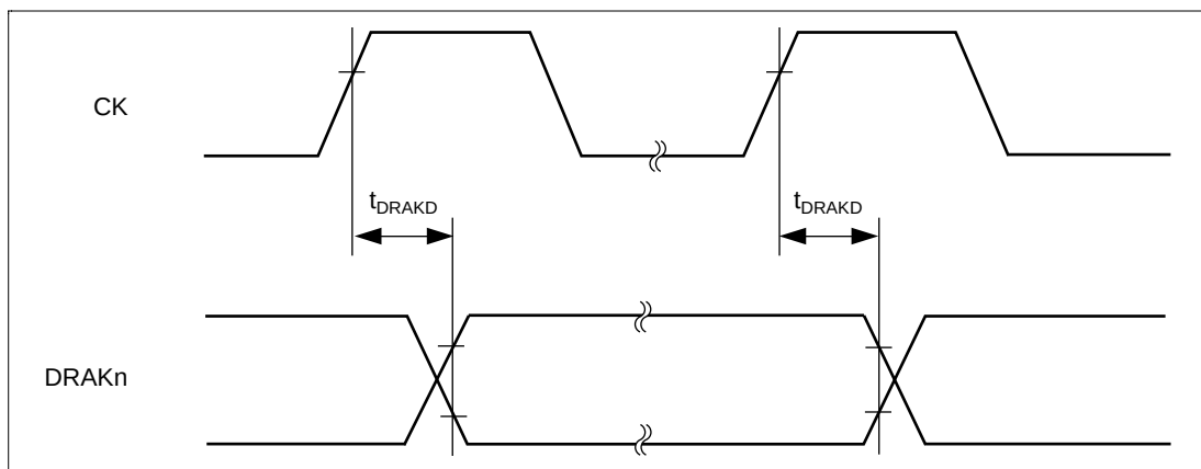
Figure 26.22 \text{DRAKn} Output Delay Time
