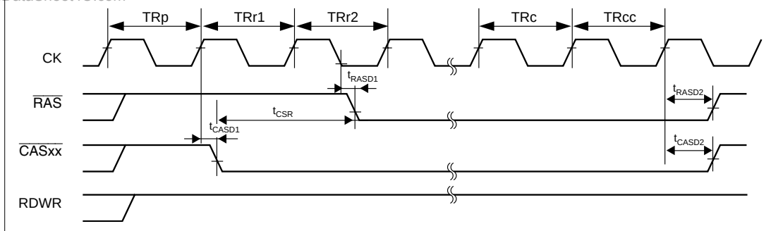
Figure 25.18 Self Refresh
