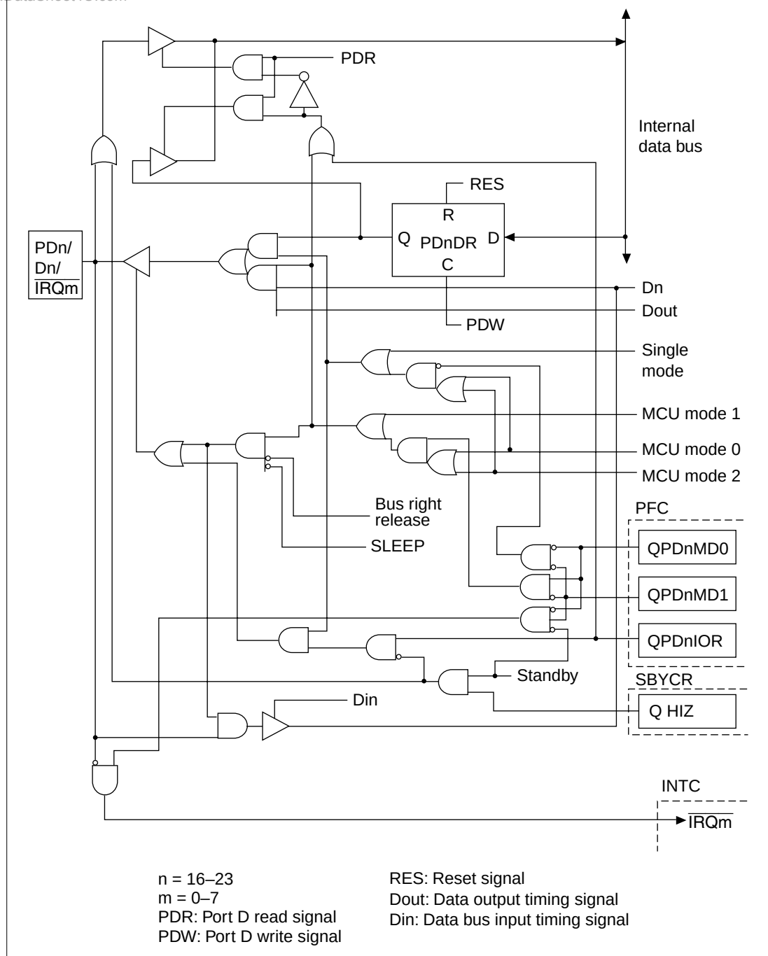
Figure B.26 PDn/Dn/IRQm Block Diagram ( n = 16-23 )
