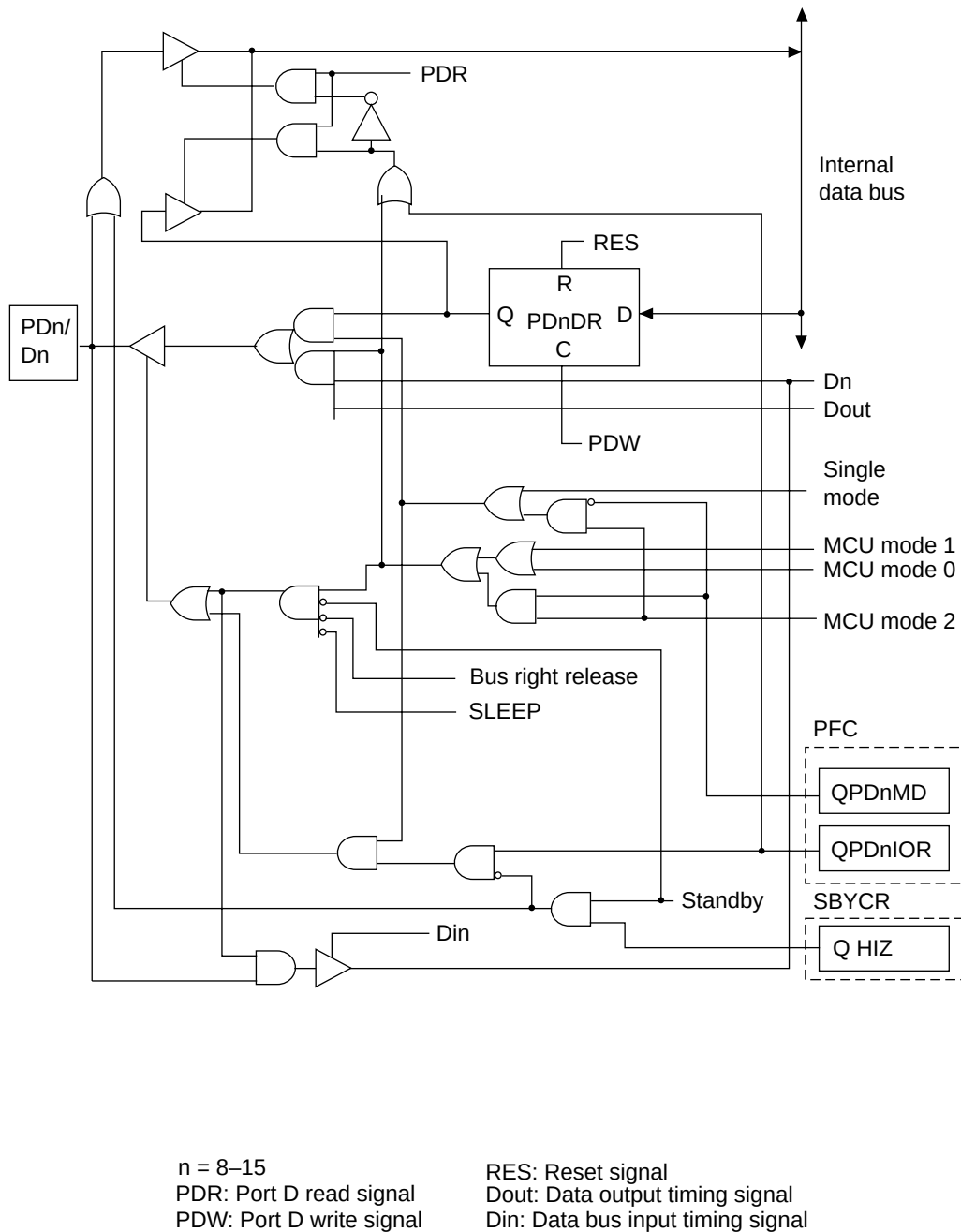
Figure B.32 PDn/Dn Block Diagram
