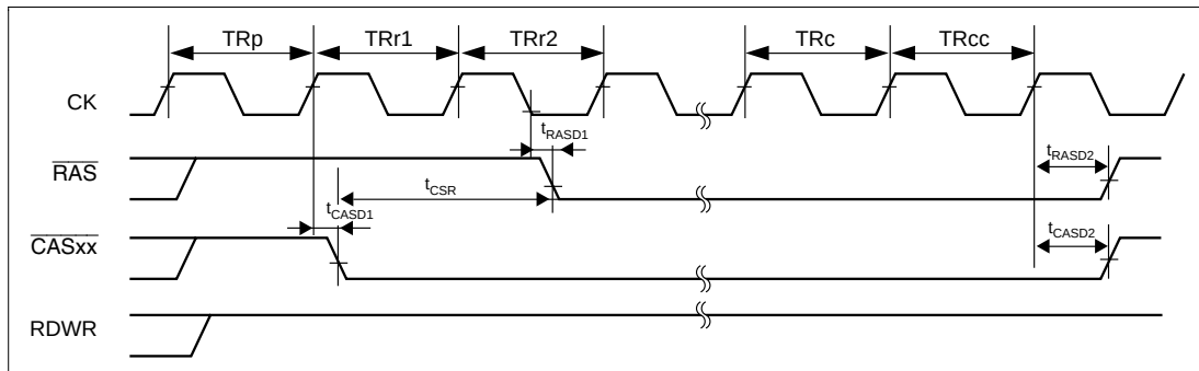
Figure 26.18 Self Refresh
