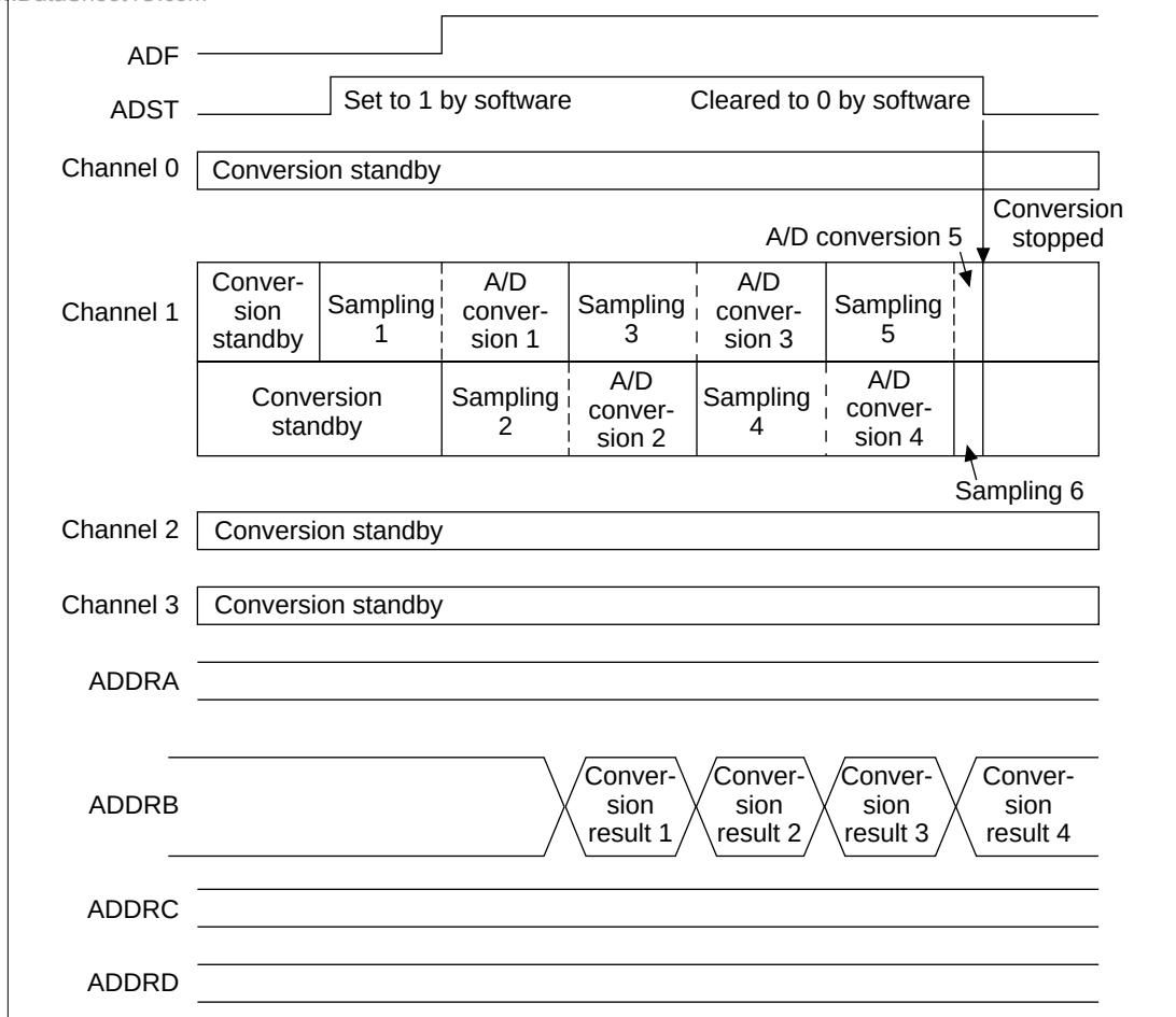
Figure 15.5 A/D Converter Operation Example (Select-Scan Mode)
