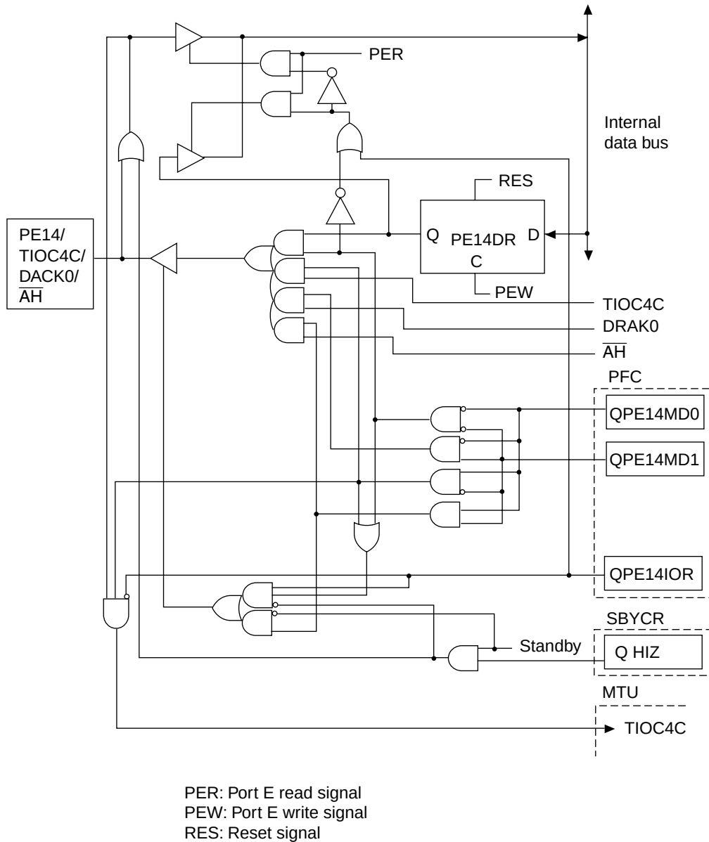
Figure B.34 PE14/TIOC4C/DACK0/AH Block Diagram
