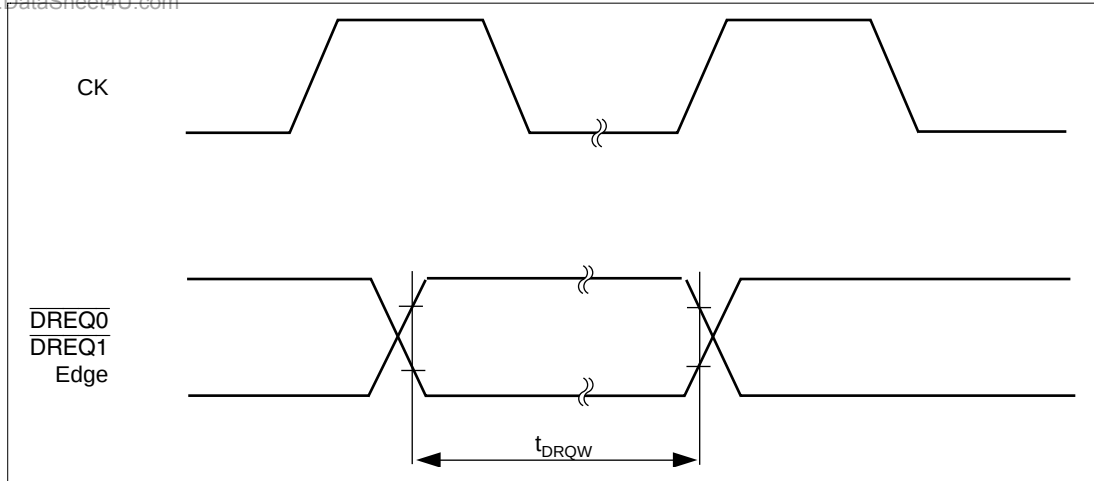
Figure 25.21 DREQ0 and DREQ1 Input Timing (2)
