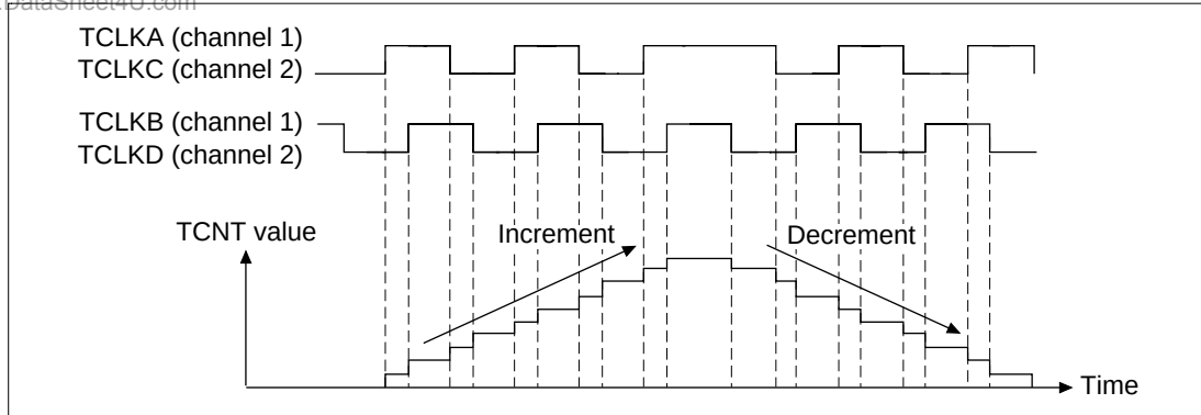
Figure 12.30 Phase Counting Mode 1 Operation
