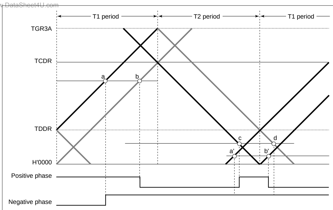
Figure 12.47 Example of Complementary PWM Mode Waveform Output (3)
