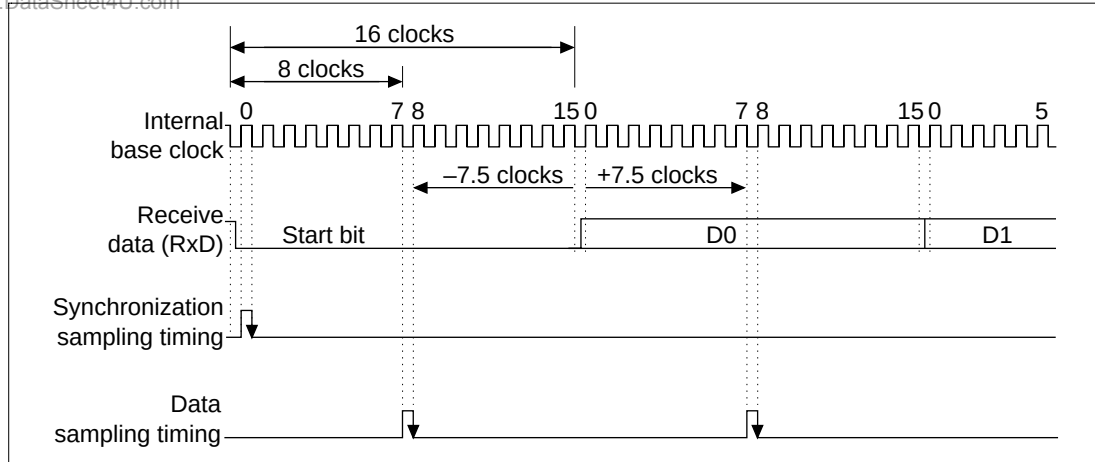
Figure 14.24 Receive Data Sampling Timing in Asynchronous Mode
