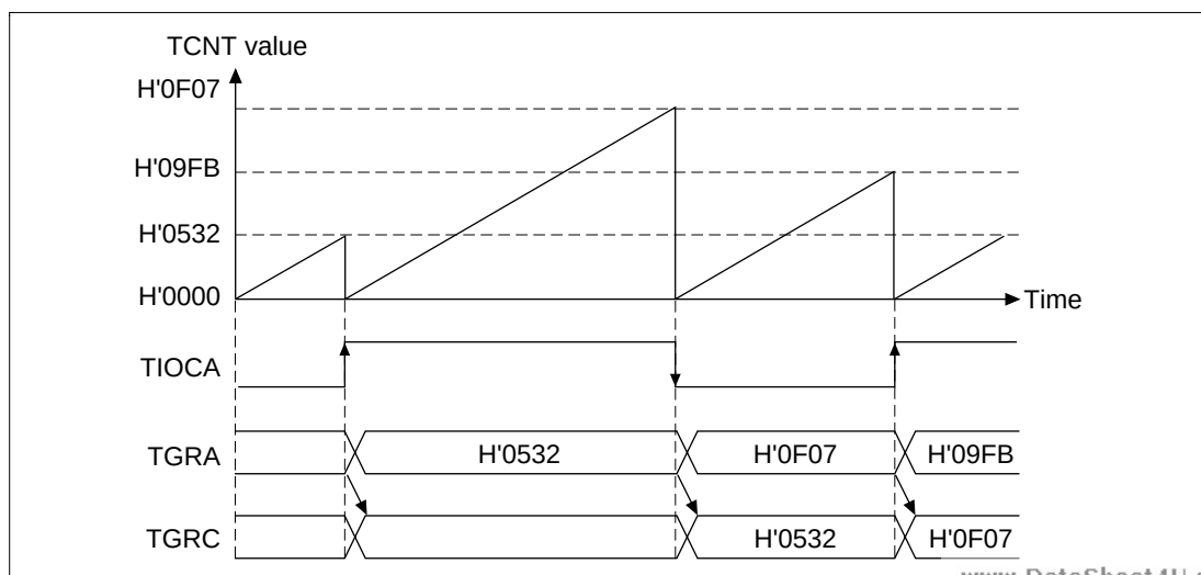
Figure 12.21 Buffer Operation Example (Input Capture Register)
