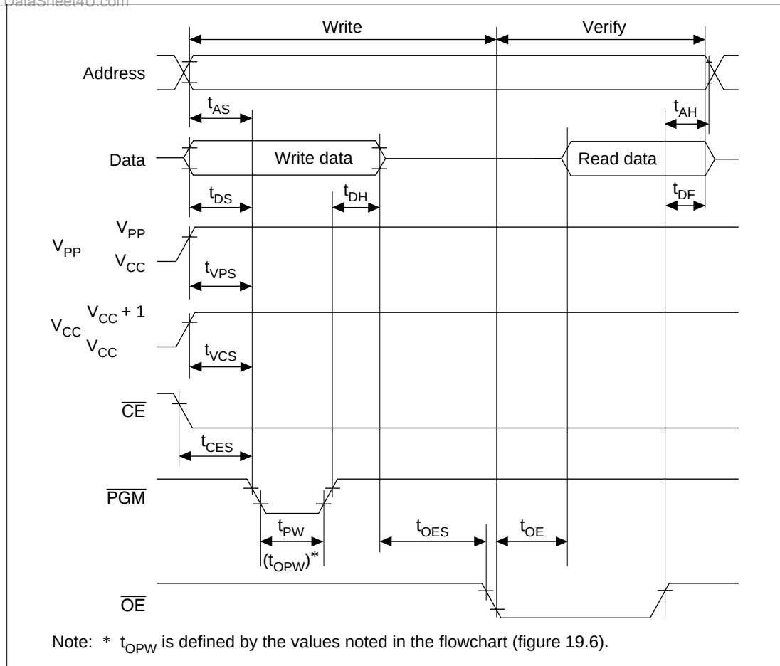
Figure 21.7 Write/Verify Timing
