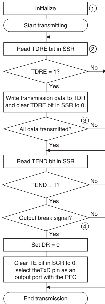
Figure 12.5 Sample Flowchart for Transmitting Serial Data
