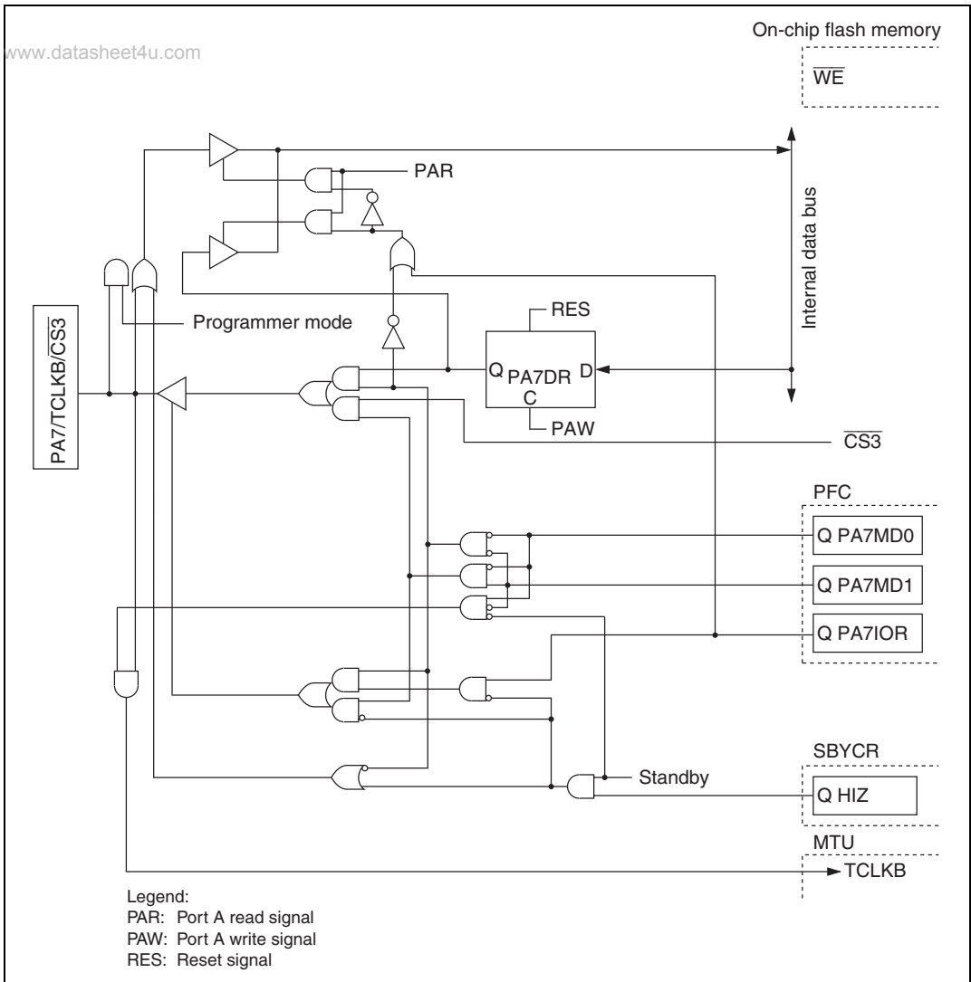
Figure B.4 PA7/TCLKB/ \overline{\text{CS3}} Block Diagram (F-ZTAT Version)
