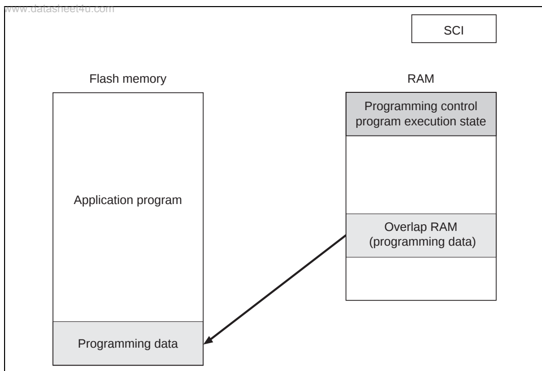
Figure 18.6 Programming to the Flash Memory
