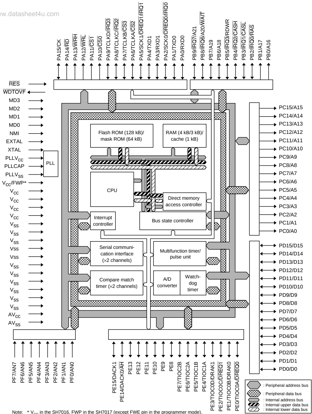
Figure 1.2 Block Diagram of the SH7016, SH7017
