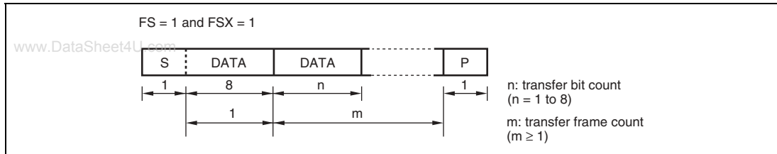
Figure 15.10 I²C Bus Data Format (Serial Format)
