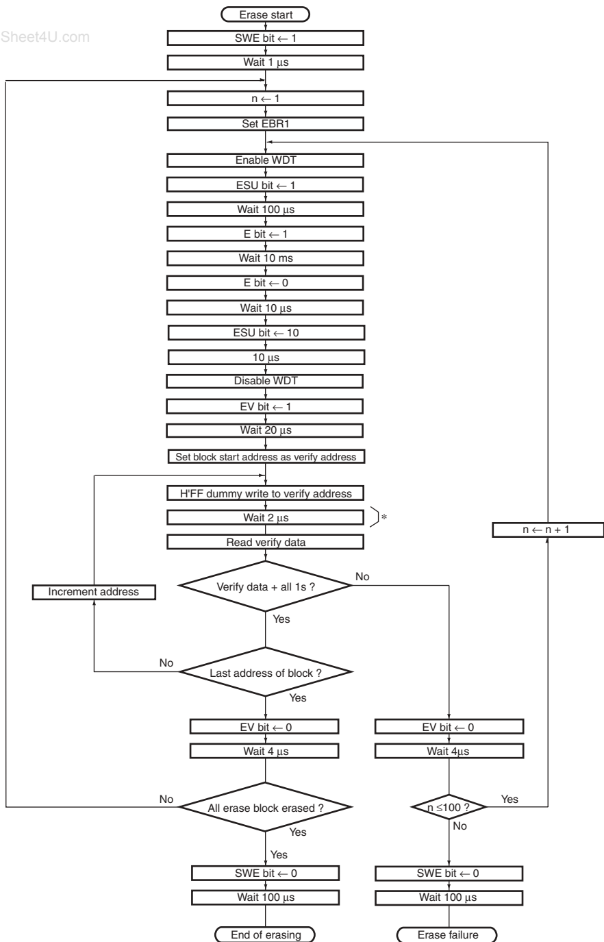
Figure 7.4 Erase/Eraser-Verify Flowchart www.DataSheet4U.com
