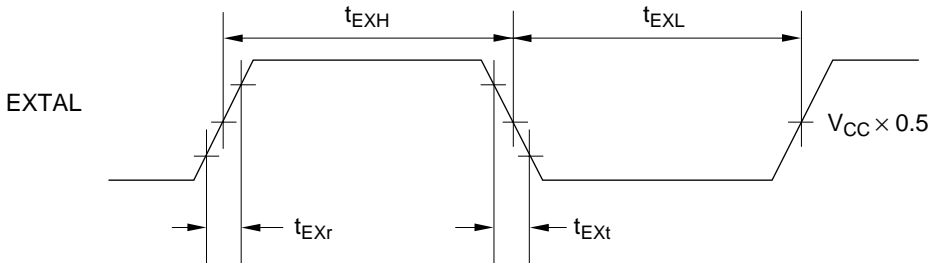
Figure 6.6 External Clock Input Timing
