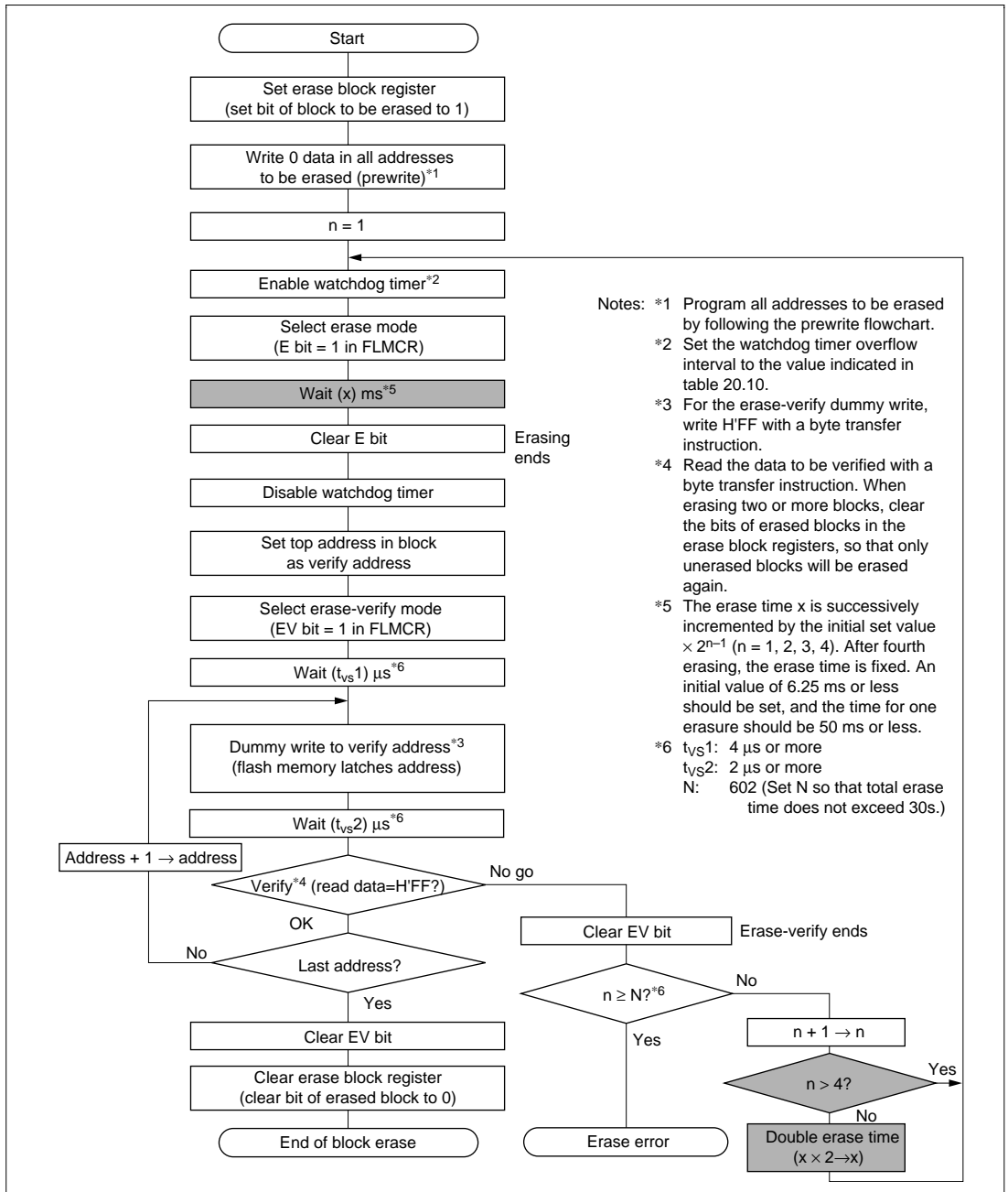
Figure 20.9 Erasing Flowchart
