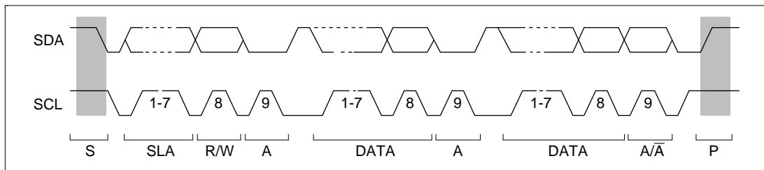
Figure 13.5 I²C Bus Timing
