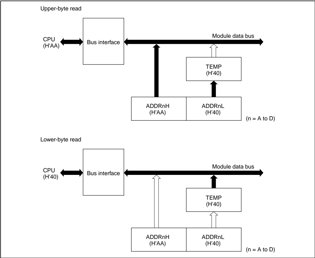
Figure 15.2 A/D Data Register Access Operation (Reading H'AA)
