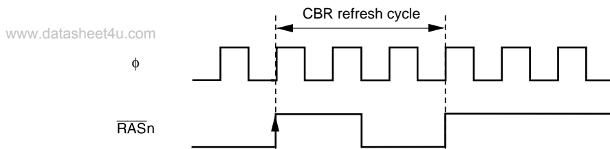
(b) CAS-before-RAS refresh cycle
