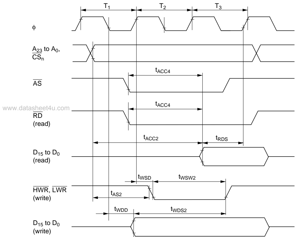
Figure 21.14 Basic Bus Cycle: three State Access
