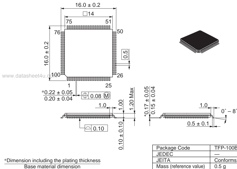
Figure G.2 Package Dimensions (TFP-100B)
