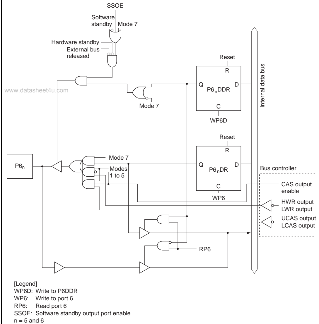
Figure C.6 (f) Port 6 Block Diagram (Pins P6 5 and P6 6 )
