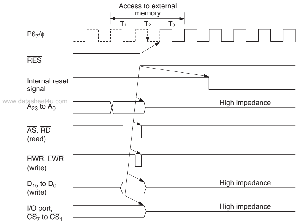
Figure D.3 Reset during Memory Access (Mode 5)
