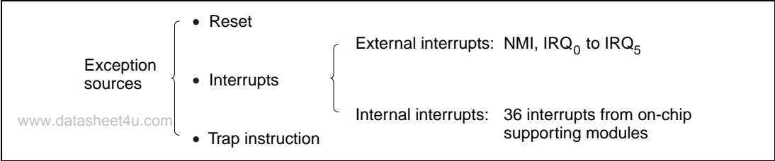
Figure 4.1 Exception Sources
