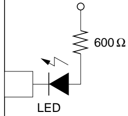
Figure 21.8 Sample LED Circuit
