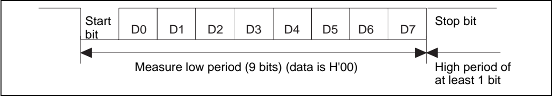
Figure 18.7 Automatic Adjustment Operation of SCI Bit Rate
