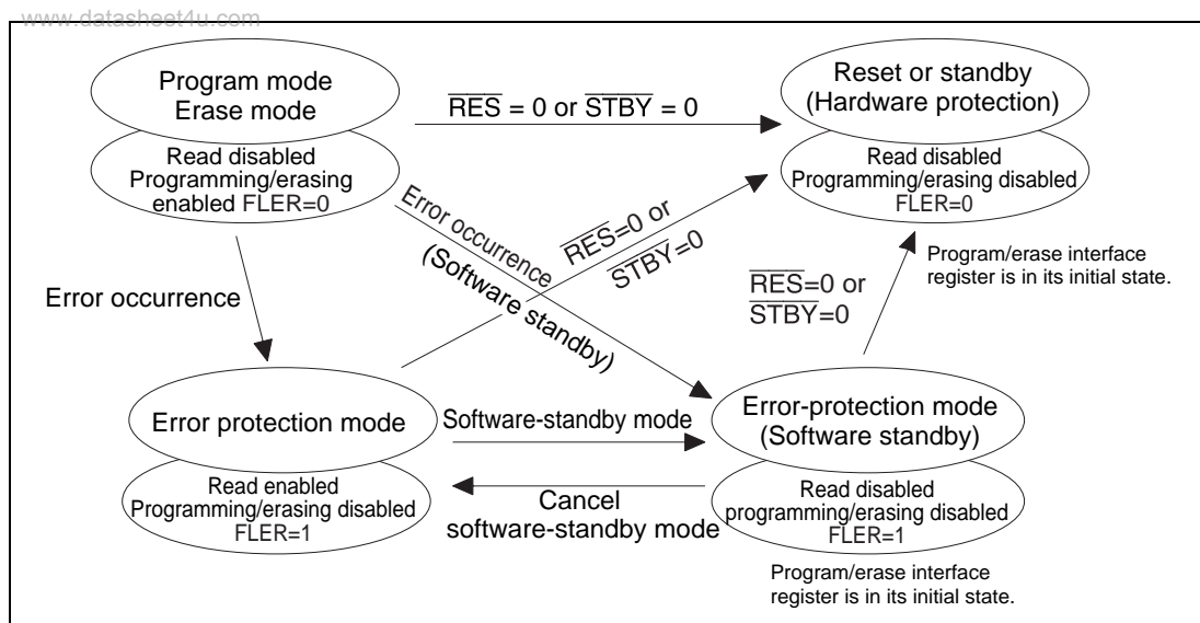
Figure 18.16 Transitions to and from the Error-Protection State
