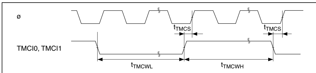
Figure 21.18 8-Bit Timer Clock Input Timing
