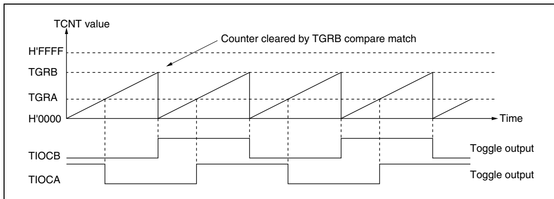
Figure 9.7 Example of Toggle Output Operation
