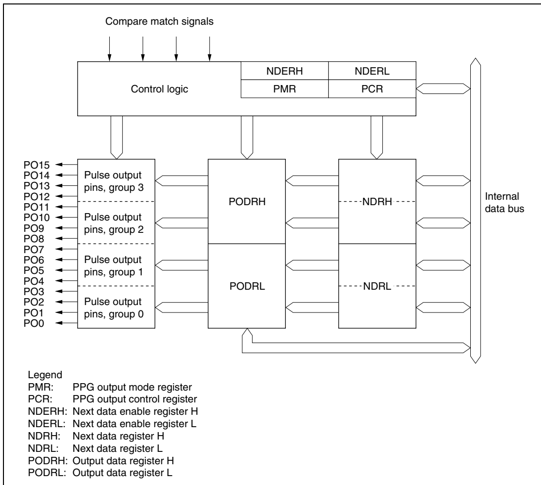
Figure 10.1 Block Diagram of PPG
