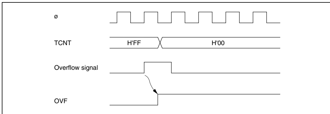
Figure 11.9 Timing of OVF Setting
