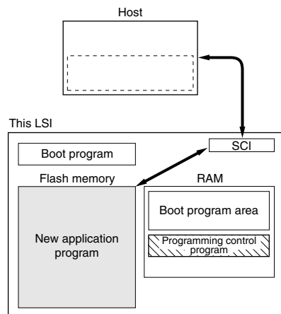
Figure 17.3 Boot Mode
