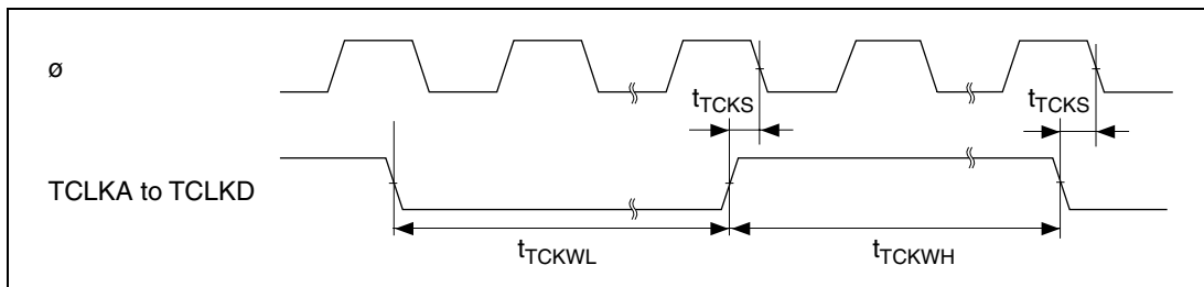
Figure 21.16 TPU Clock Input Timing
