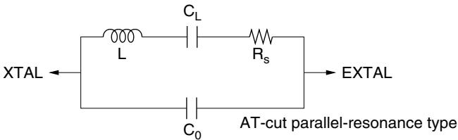
Figure 18.3 Crystal Resonator Equivalent Circuit
