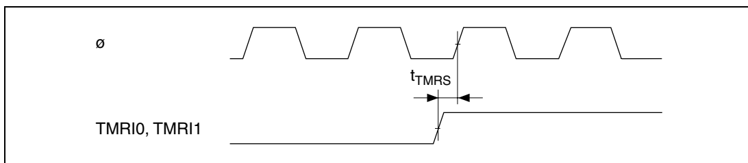
Figure 21.19 8-Bit Timer Reset Input Timing
