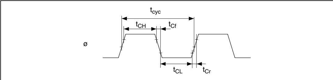
Figure 21.2 System Clock Timing
