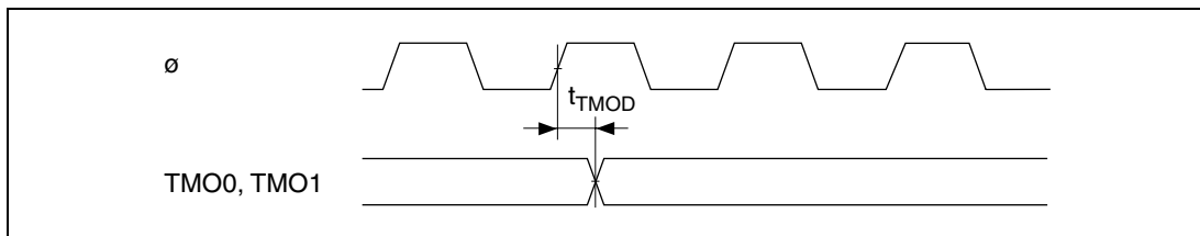
Figure 21.17 8-Bit Timer Output Timing
