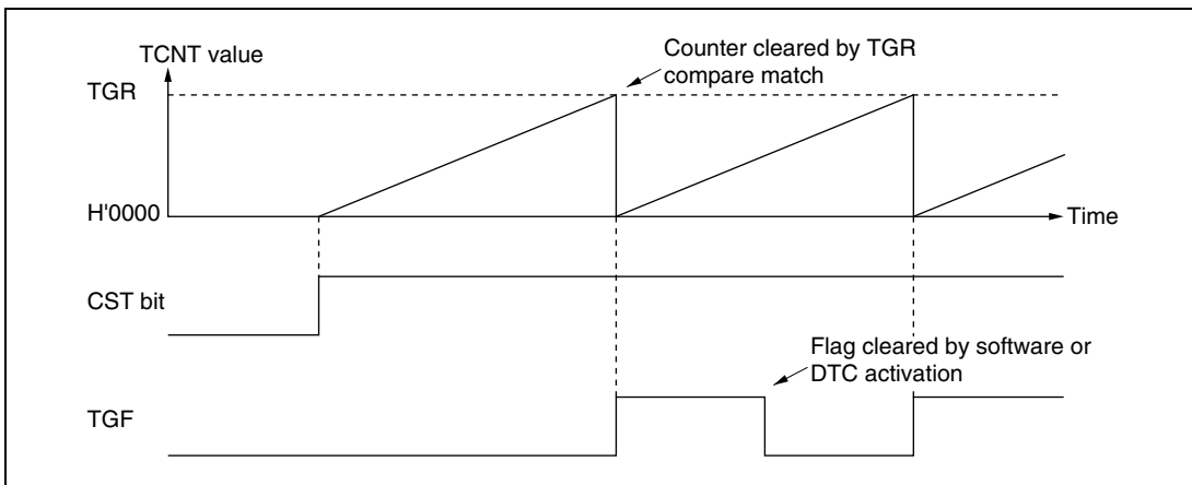
Figure 9.4 Periodic Counter Operation
