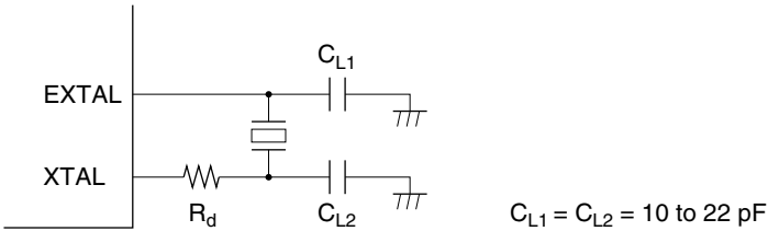
Figure 18.2 Connection of Crystal Resonator (Example)
