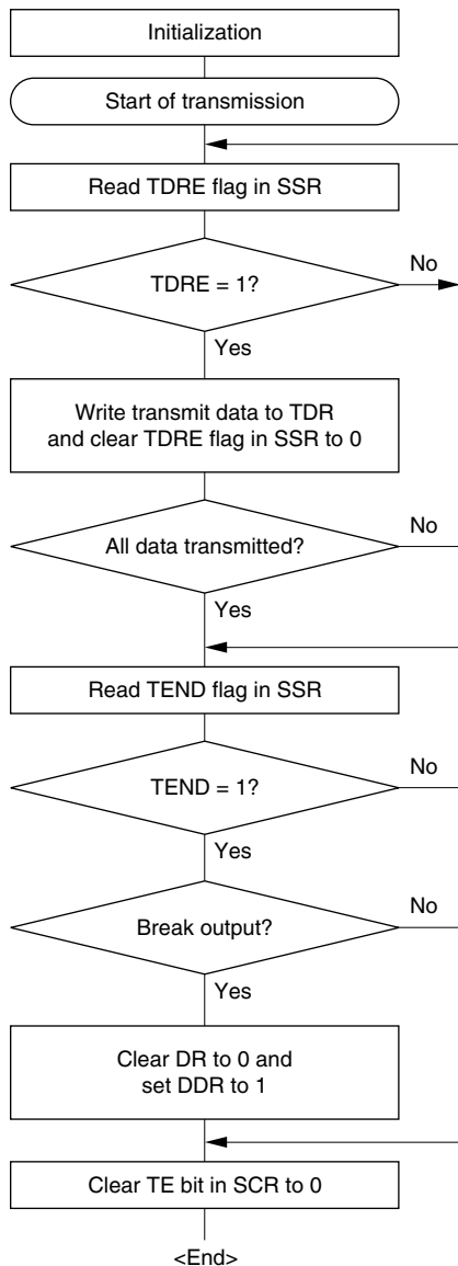
Figure 13.7 Sample Serial Transmission Flowchart
