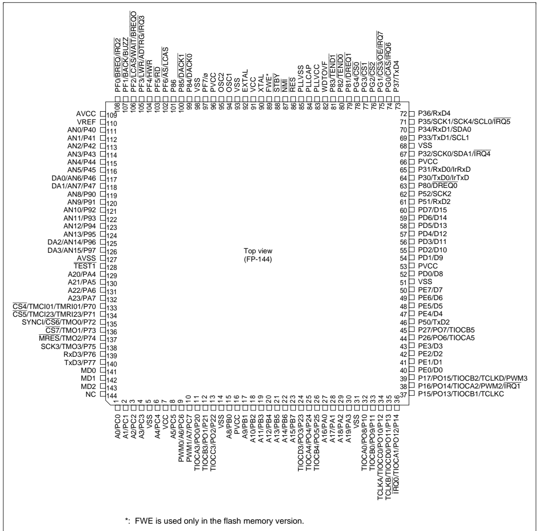
Figure 1-2 Pin Arrangement (FP-144: Top View)
