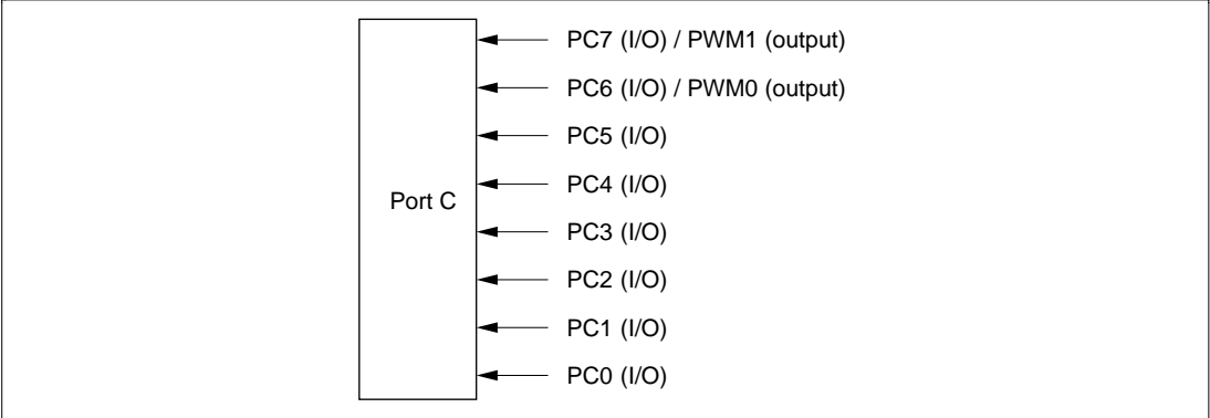
Figure 10-18 Port C Pin Functions (Mode 7)
