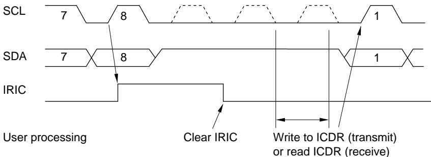
Figure 18-12 IRIC Setting Timing and SCL Control
