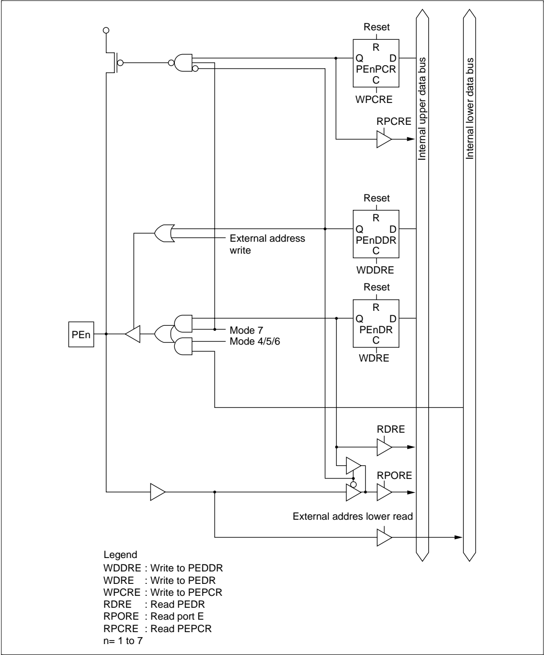
Figure C-13 Port E Block Diagram (Pin PEn)
