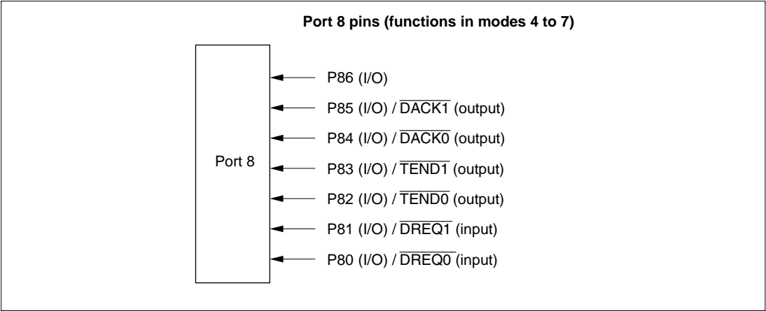
Figure 10-7 Port 8 Pin Functions
