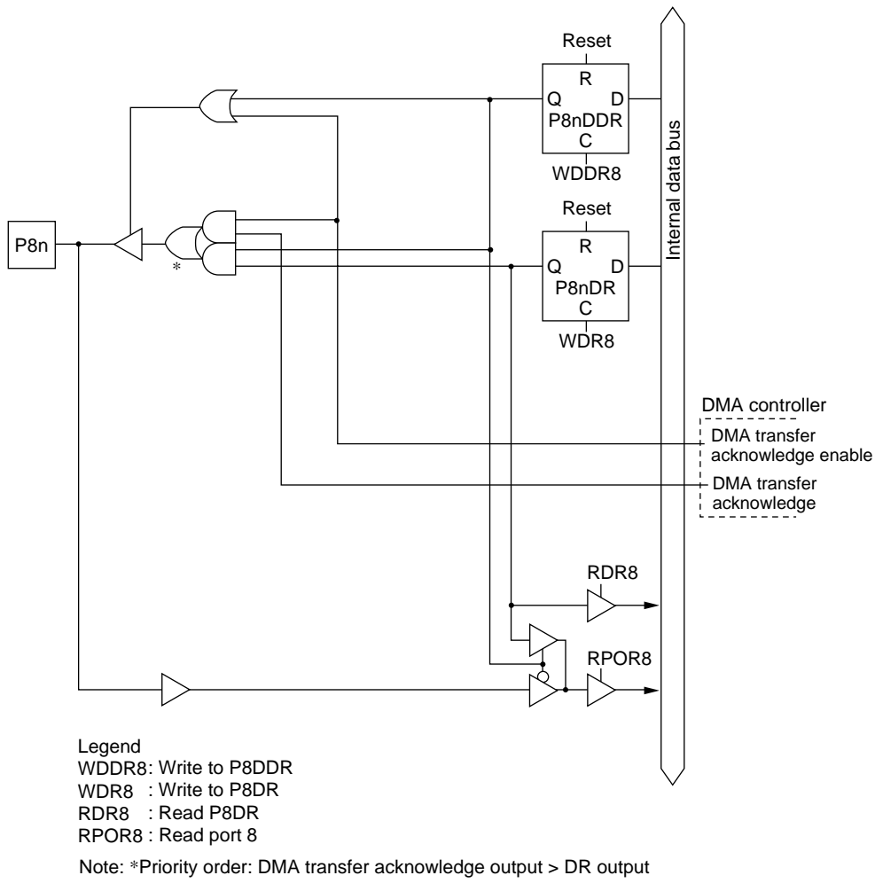
Figure C-7 (c) Port 8 Block Diagram (Pins P84 and P85)
