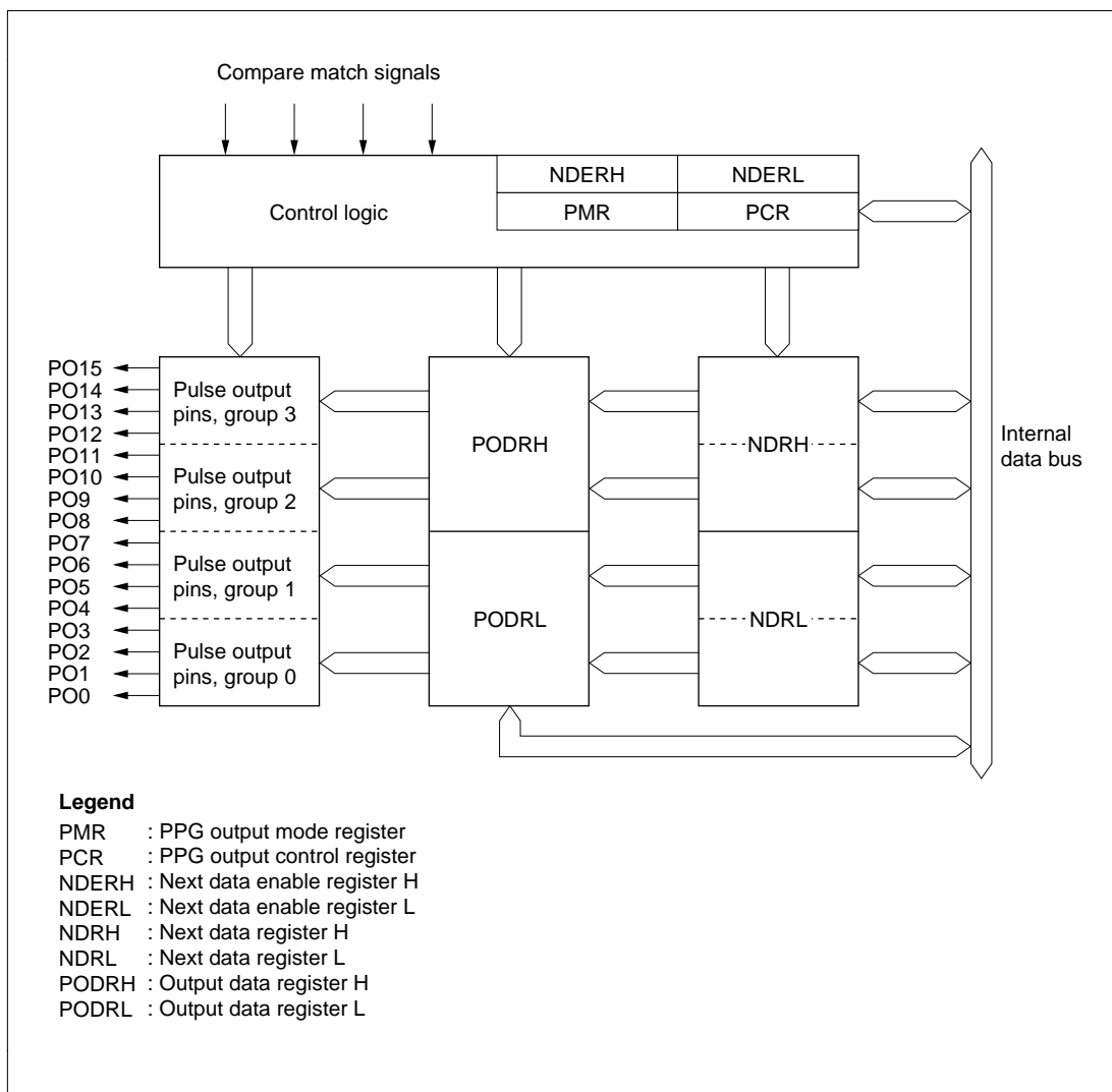
Figure 12-1 Block Diagram of PPG
