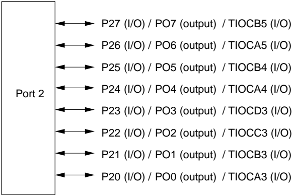
Figure 10-2 Port 2 Pin Functions
