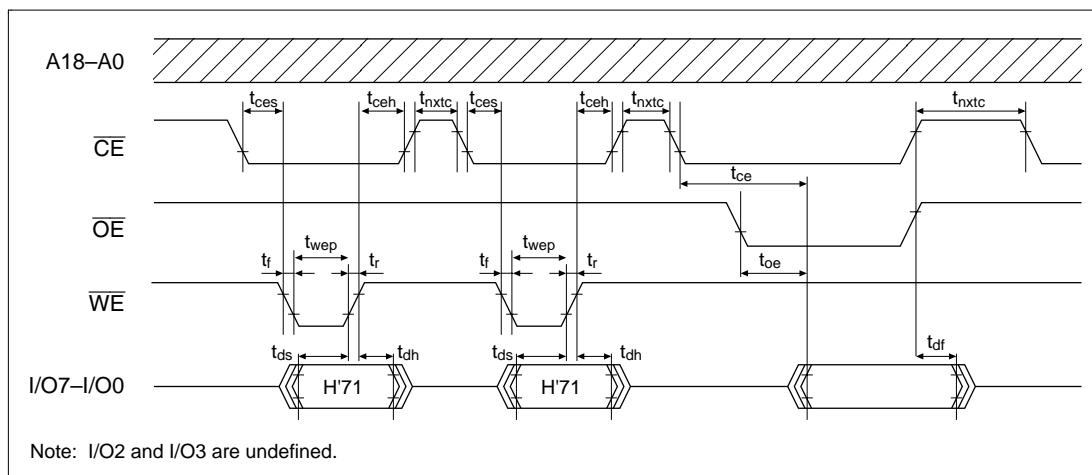
Figure 22-26 Status Read Mode Timing Waveforms
