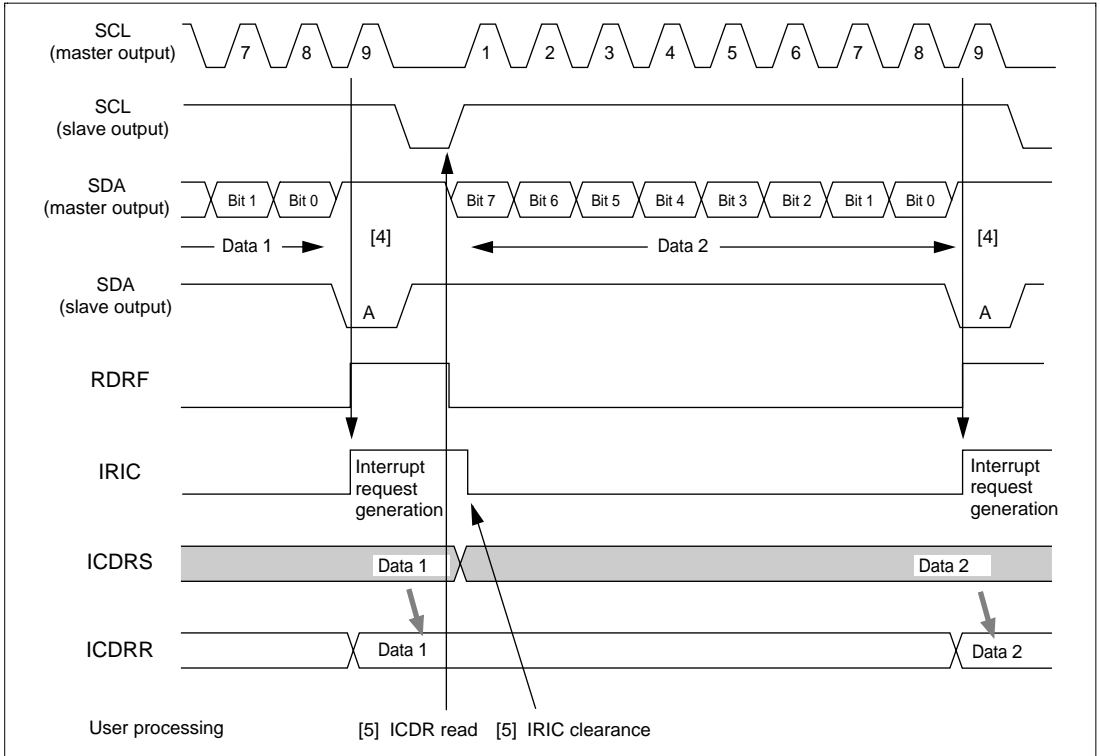
Figure 18-10 Example of Slave Receive Mode Operation Timing (2) (MLS = ACKB = 0)
