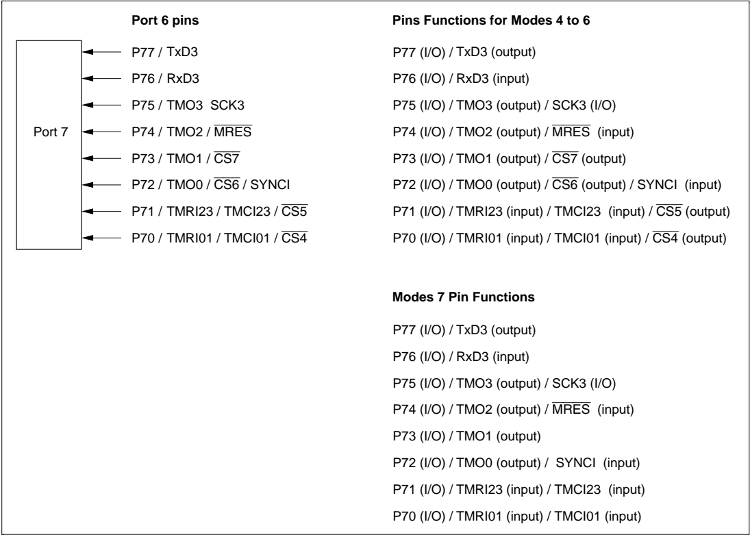
Figure 10-6 Port 6 Pin Functions
