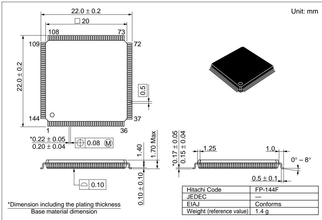
Figure G-1 FP-144F Package Dimensions
