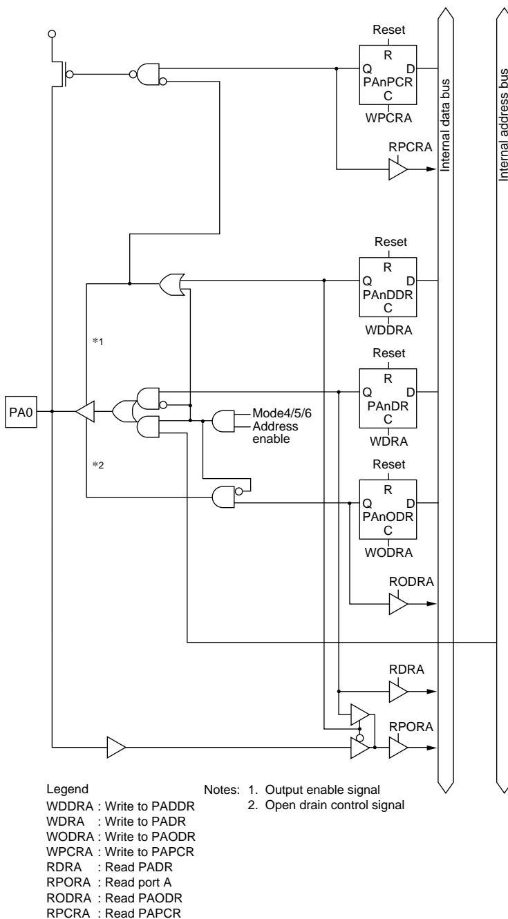
Figure C-9 (a) Port A Block Diagram (Pin PA0)
