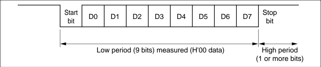
Figure 22-9 Automatic SCI Bit Rate Adjustment
