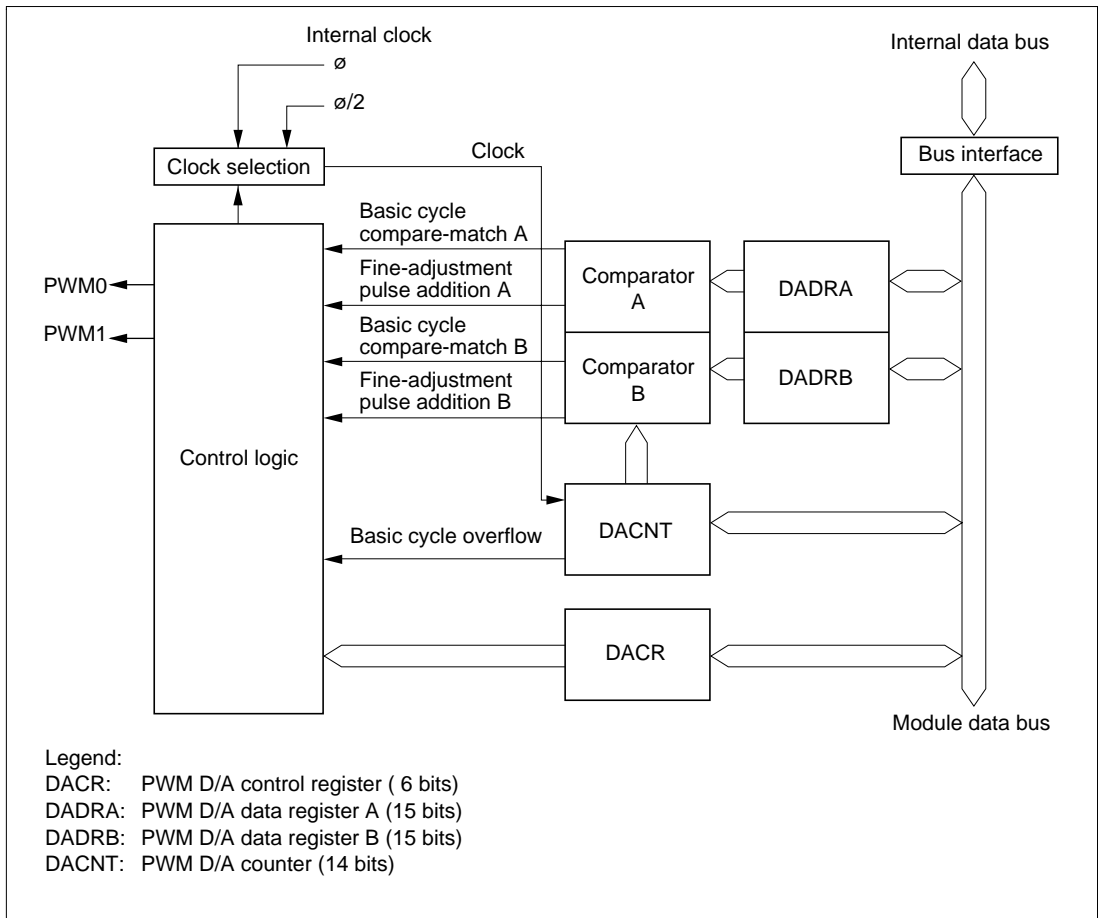
Figure 14-1 PWM D/A Block Diagram
