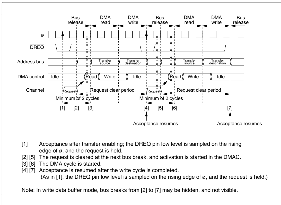
Figure 8-25 Example of DREQ Level Activated Normal Mode Transfer
