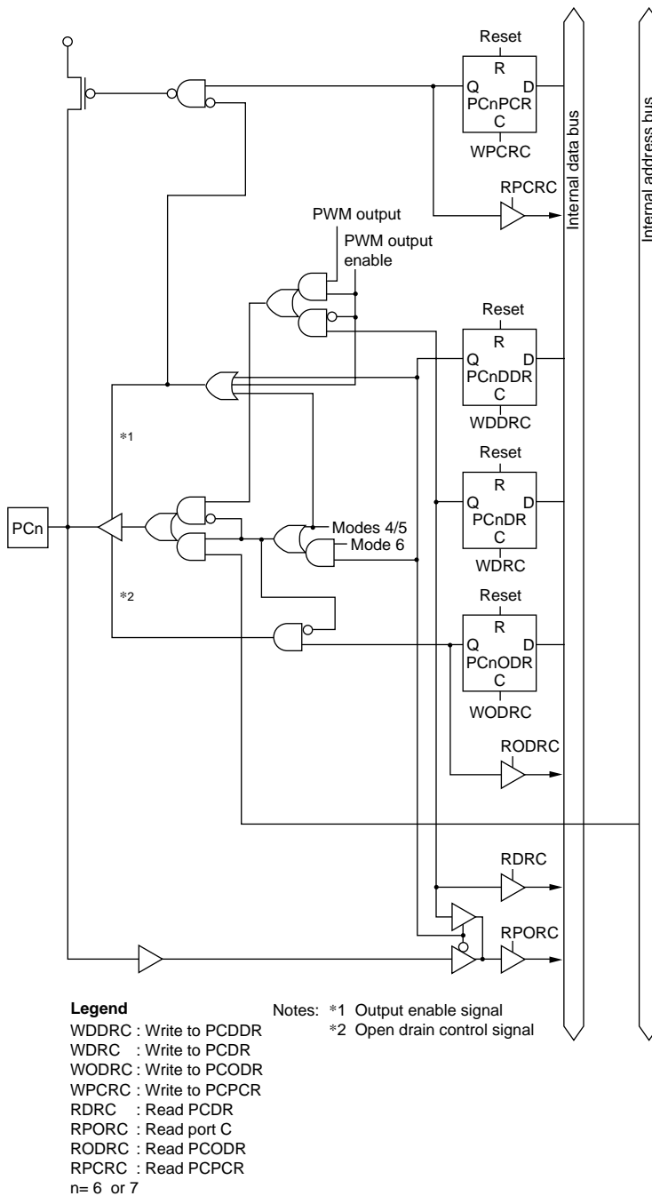
Figure C-8 (b) Port C Block Diagram (Pins PC6 and PC7)
