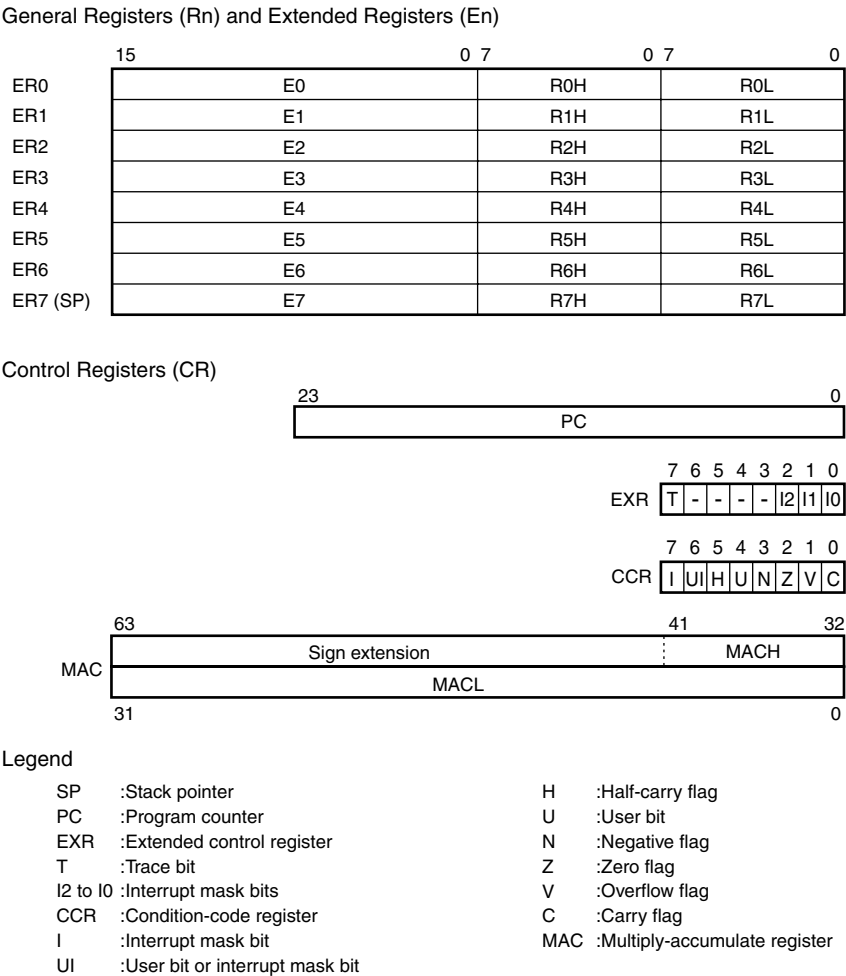
Figure 2-6 CPU Registers
