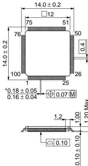
Figure G.2 TFP-100G Package Dimensions (Under development)
