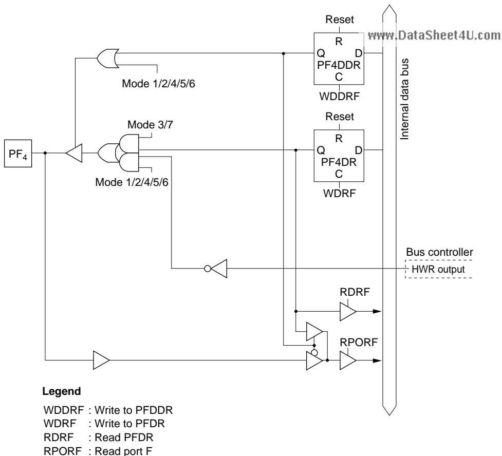
Figure C.10 (e) Port F Block Diagram (Pin PF 4 )
