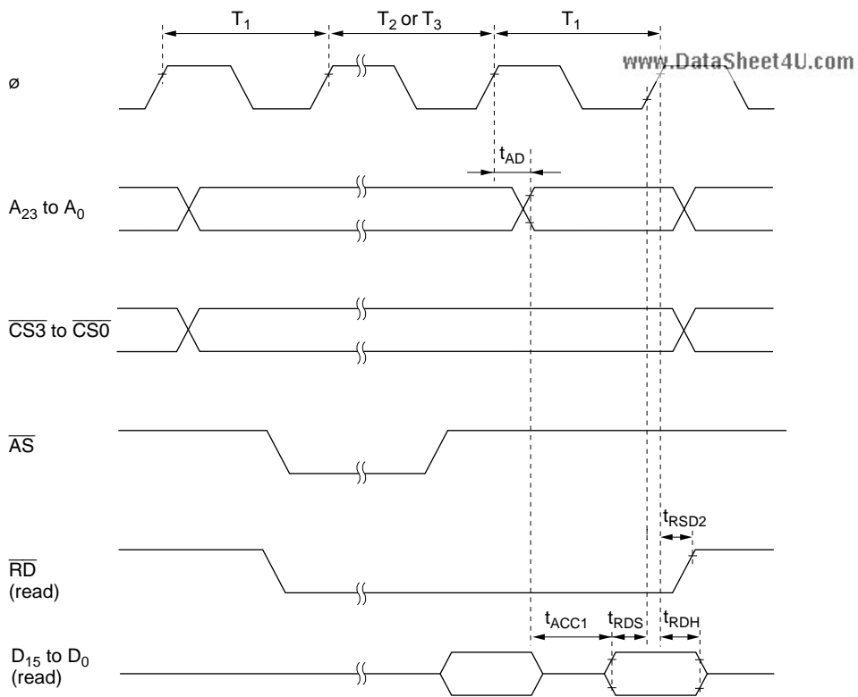
Figure 20.15 Burst ROM Access Timing (One-State Access)
