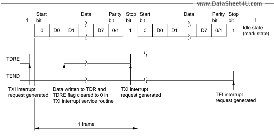
Figure 12.6 Example of Operation in Transmission in Asynchronous Mode (Example with 8-Bit Data, Parity, One Stop Bit)
