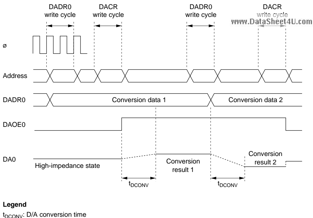
Figure 15.2 Example of D/A Converter Operation
