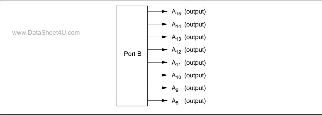
Figure 8.10 Port B Pin Functions (Modes 1, 4, and 5)*
