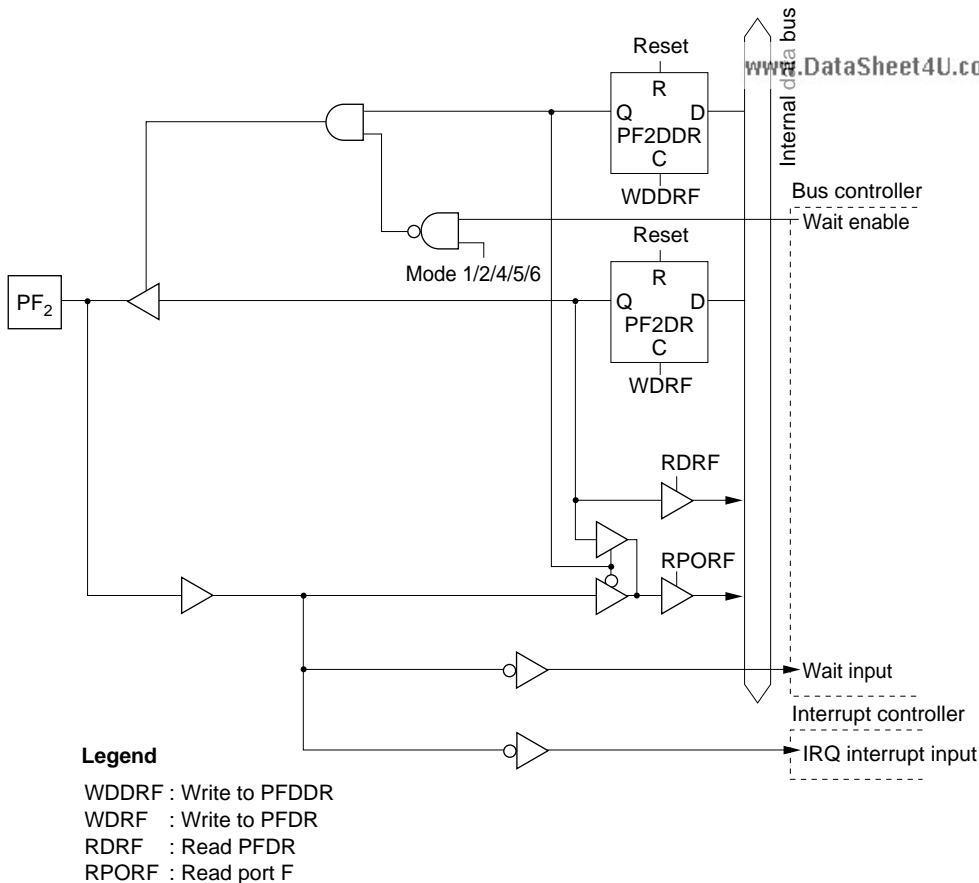
Figure C.10 (c) Port F Block Diagram (Pin PF 2 )
