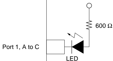
Figure 20.2 LED Drive Circuit (Example)
