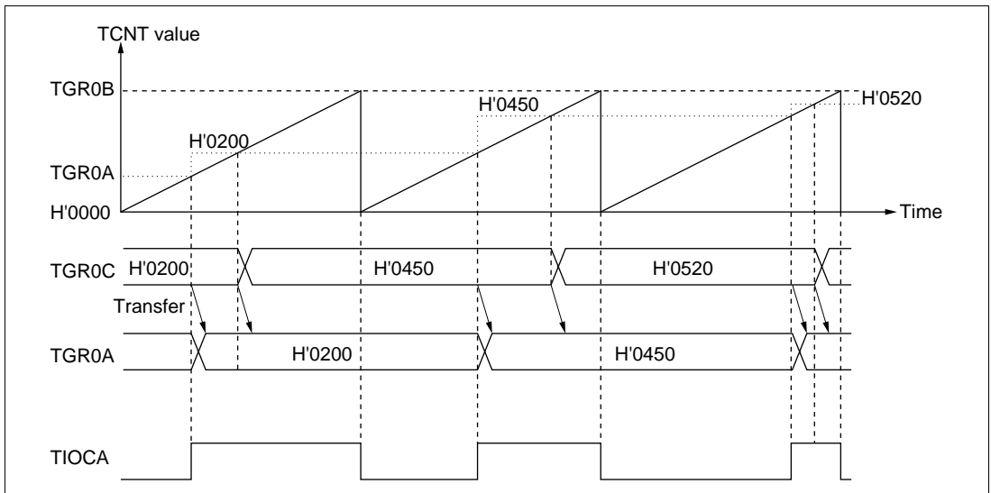
www.DataSheet4U.com Figure 9.19 Example of Buffer Operation (1)
