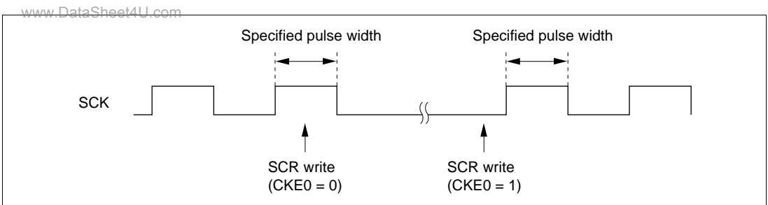
Figure 13.8 Timing for Fixing Clock Output Level
