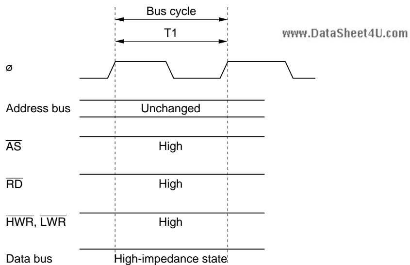
Figure 2.18 Pin States during On-Chip Memory Access
