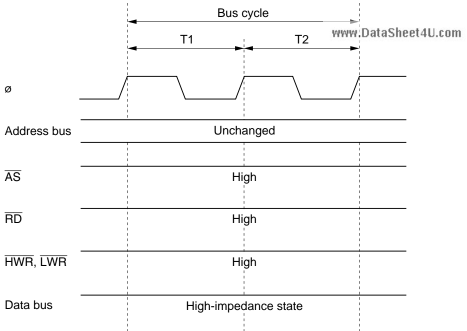
Figure 2.20 Pin States during On-Chip Supporting Module Access
