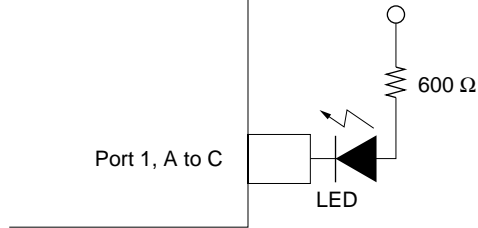
Figure 20.5 LED Drive Circuit (Example)
