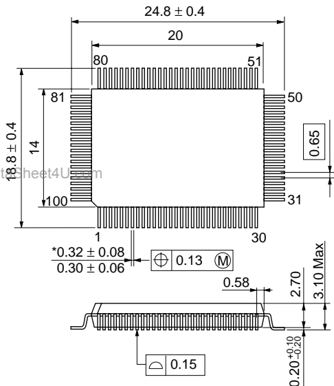
Figure G.2 TFP-100G Package Dimensions (Under development)
