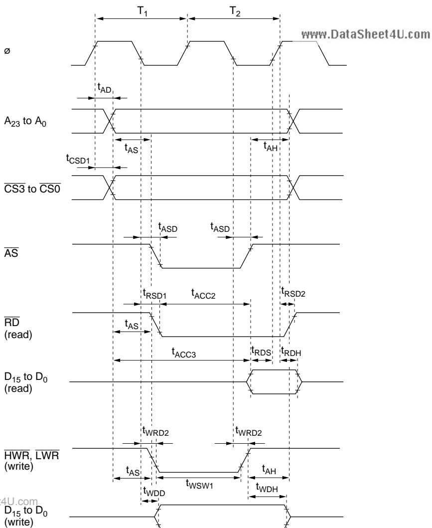
Figure 20.11 Basic Bus Timing (Two-State Access)
