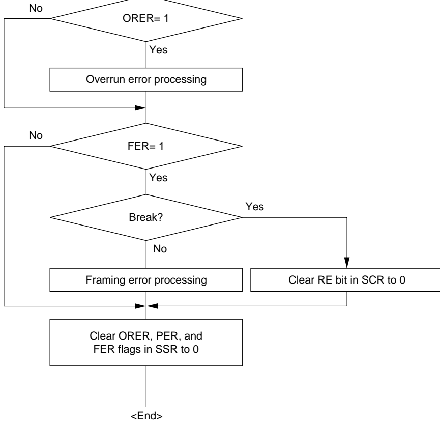
Figure 12.12 Sample Multiprocessor Serial Reception Flowchart (cont)
