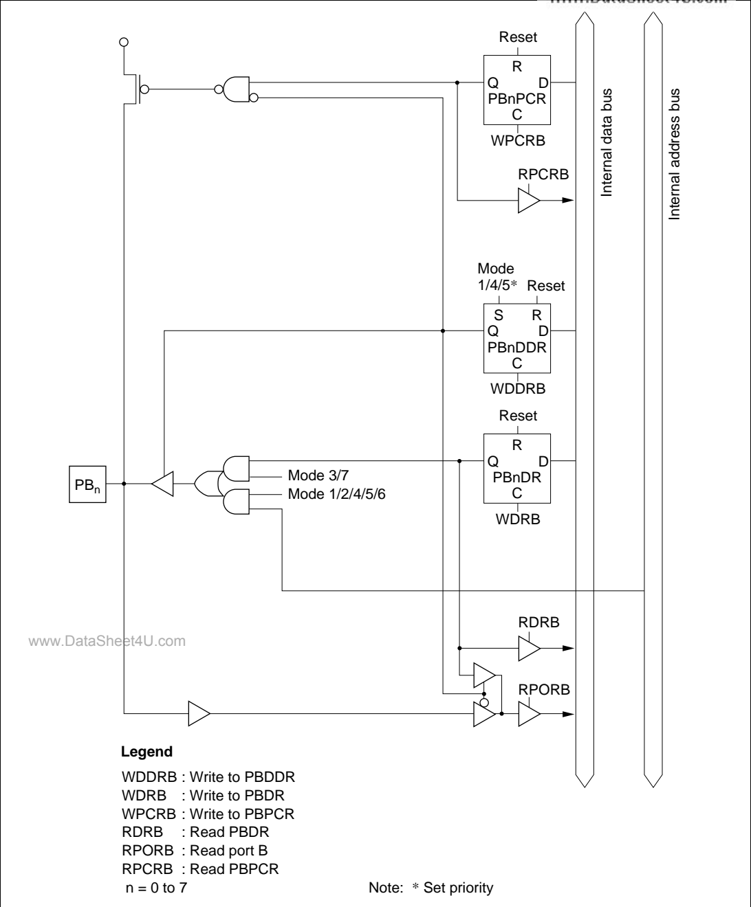
Figure C.6 Port B Block Diagram (Pin PB_n )
