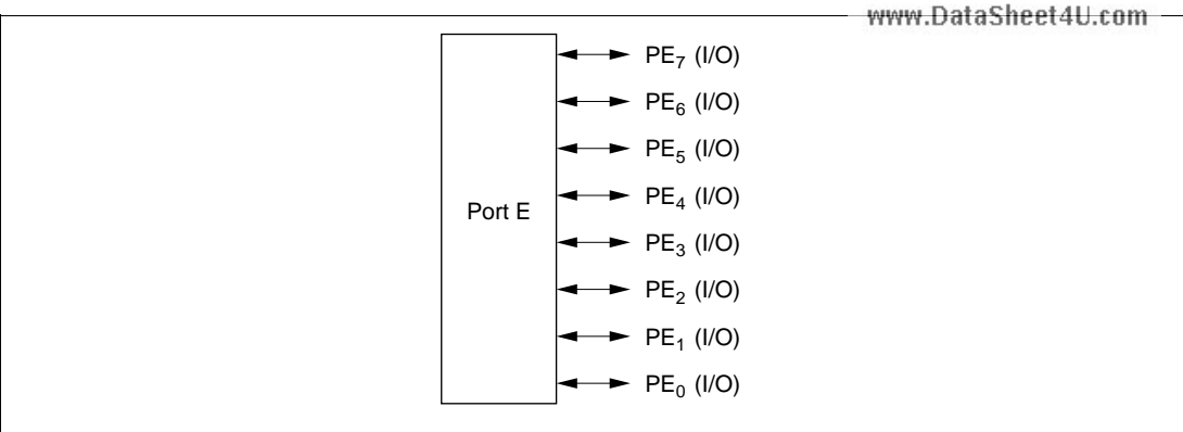
Figure 8.22 Port E Pin Functions (Modes 3 and 7)*
