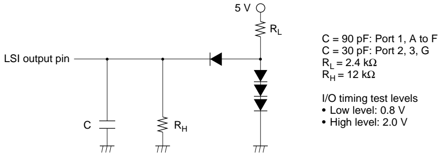
Figure 20.6 Output Load Circuit
