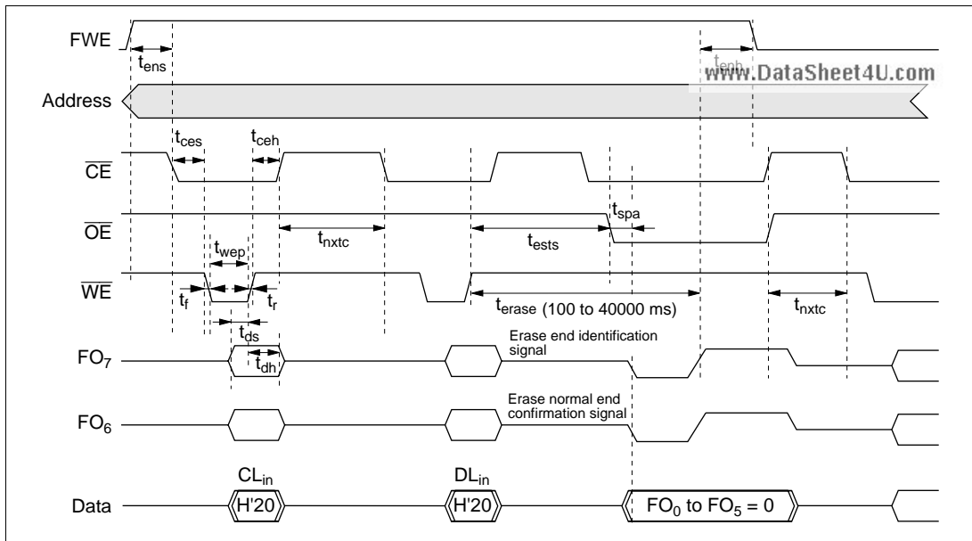
Figure 17.32 Auto-Erase Mode Timing Waveforms
