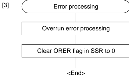
Figure 12.18 Sample Serial Reception Flowchart
