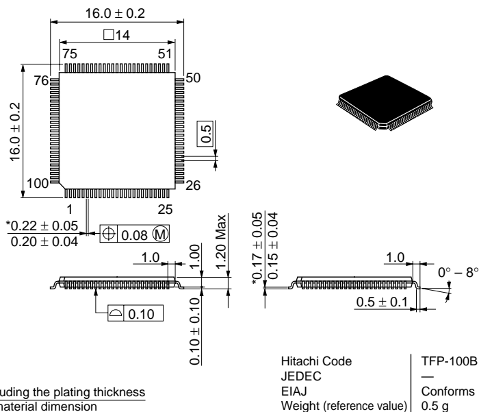
Figure G.1 TFP-100B Package Dimensions
