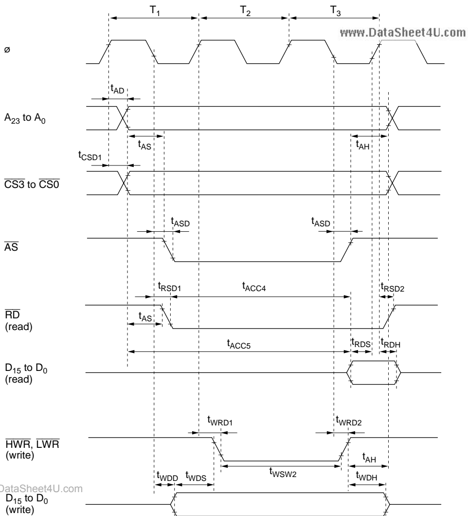
Figure 20.12 Basic Bus Timing (Three-State Access)
