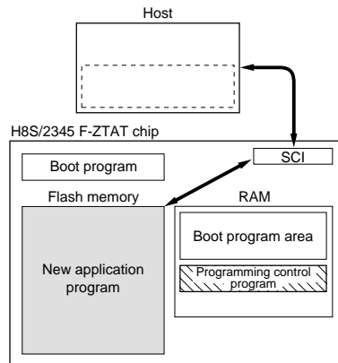
Figure 17.9 Boot Mode
