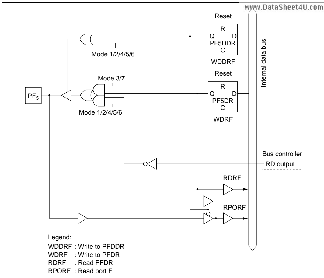
www.DataSheet4U.com Figure C.10 (f) Port F Block Diagram (Pin PF 5 )
