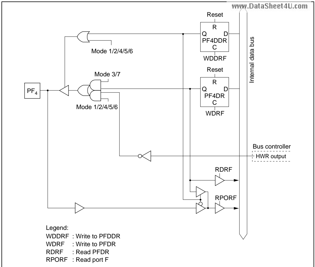
www.DataSheet4U.com Figure C.10 (e) Port F Block Diagram (Pin PF 4 )
