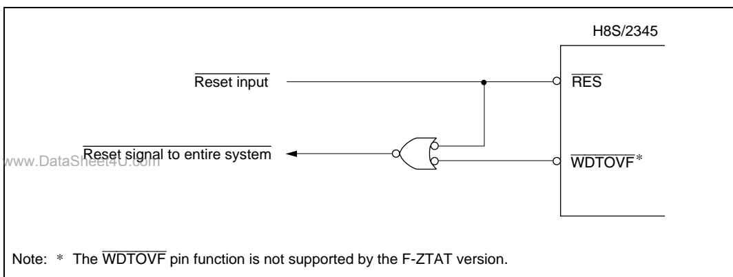
Figure 11.9 Circuit for System Reset by \overline{\text{WDTOVF}} Signal (Example)
