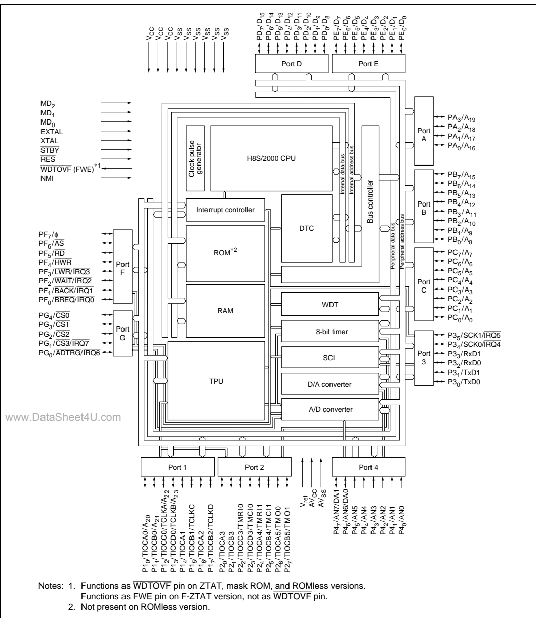
Figure 1.1 Block Diagram
