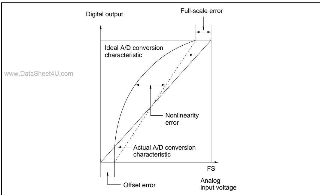
Figure 14.10 A/D Conversion Precision Definitions (2)
