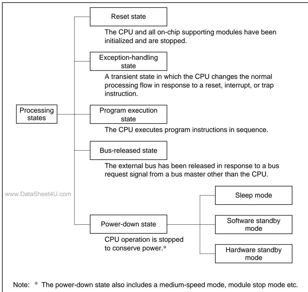
Figure 2.14 Processing States
