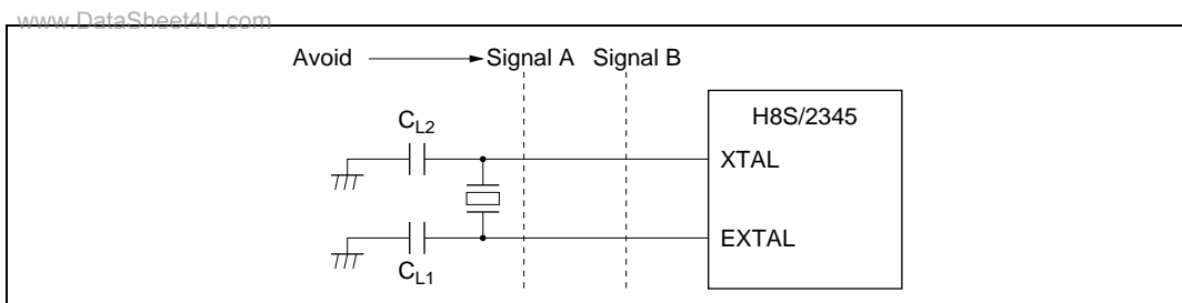
Figure 18.4 Example of Incorrect Board Design
