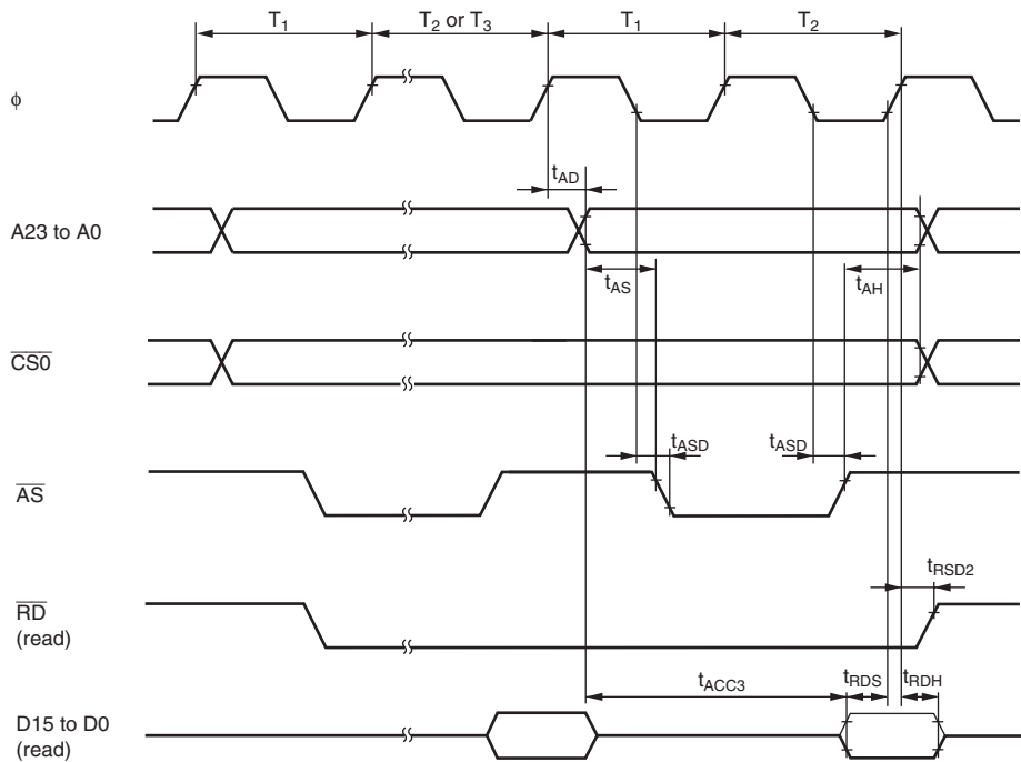
Figure 24.12 Burst ROM Access Timing: Two-State Access
