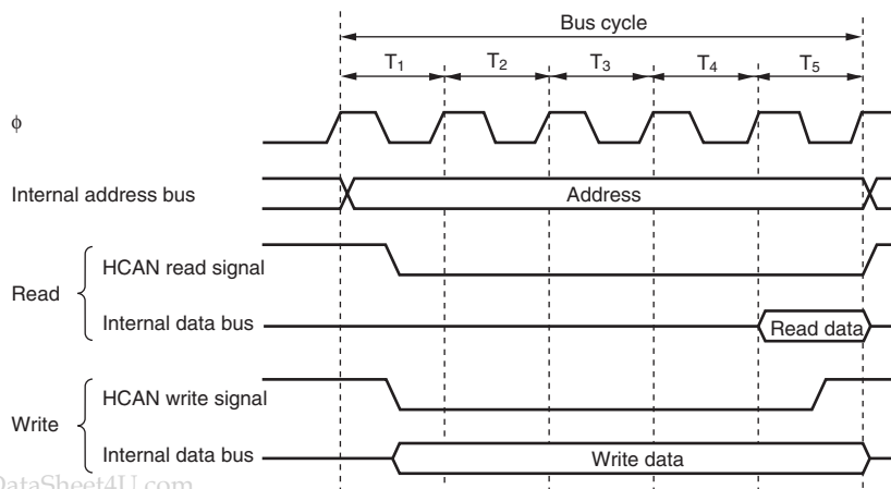
Figure 7.12 On-Chip HCAN Module Access
