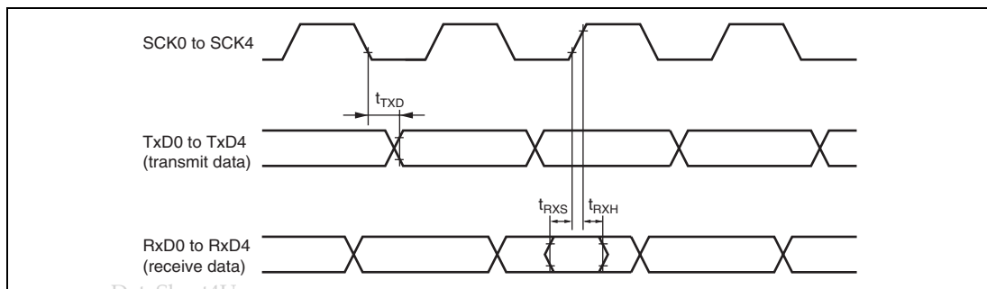
Figure 24.22 SCI Input/Output Timing/Synchronization
