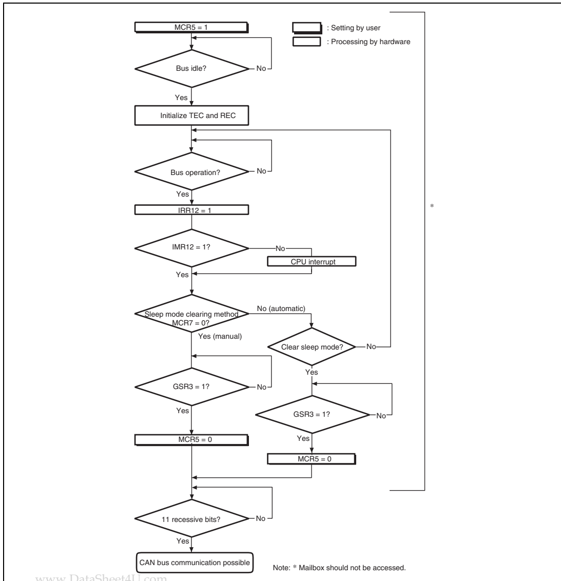
Figure 18.13 HCAN Sleep Mode Flowchart www.DataSheet4U.com
