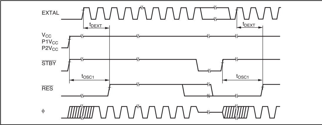
Figure 24.6 Oscillator Settling Timing
