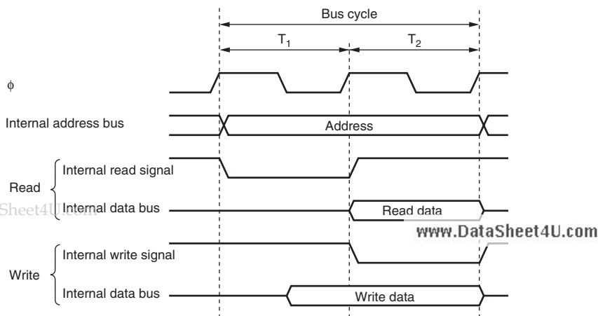
Figure 7.6 On-Chip Peripheral Module Access Cycle
