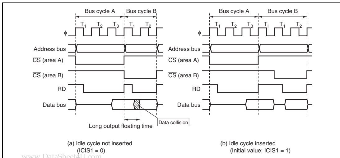
Figure 7.27 Example of Idle Cycle Operation
