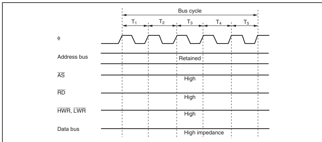
Figure 7.13 Pin States during On-Chip HCAN Module Access
