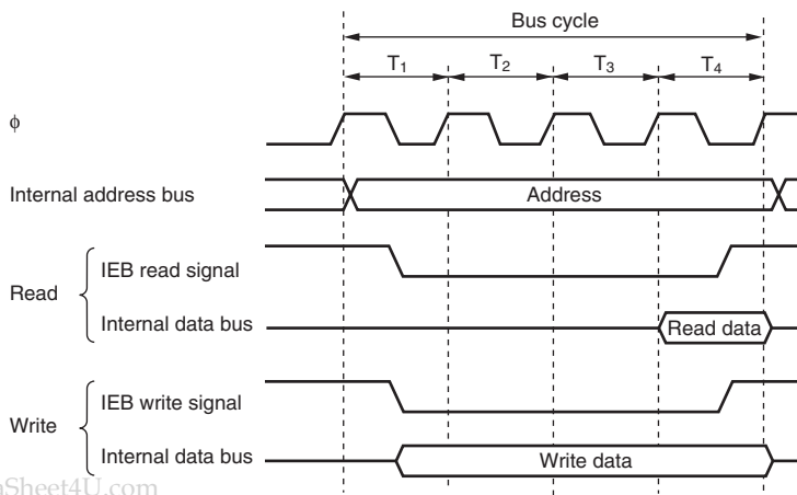
Figure 7.10 On-Chip IEB Module Access Timing
