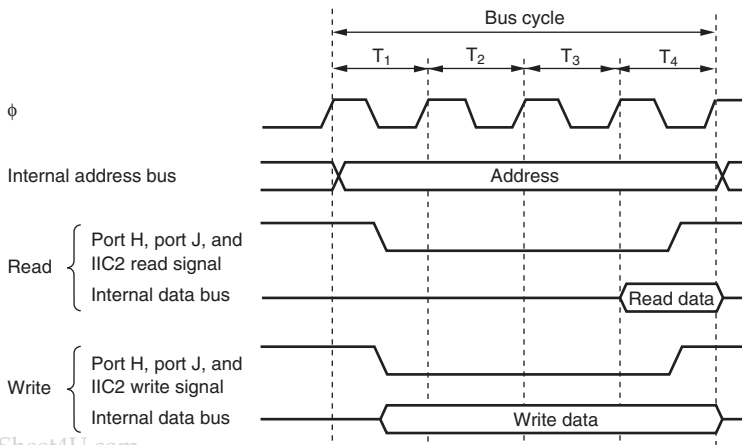
Figure 7.8 On-Chip Port H, Port J, and IIC2 Module Access Timing
