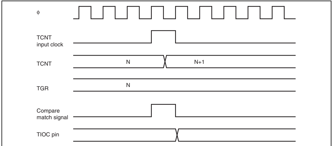
Figure 10.32 Output Compare Output Timing
