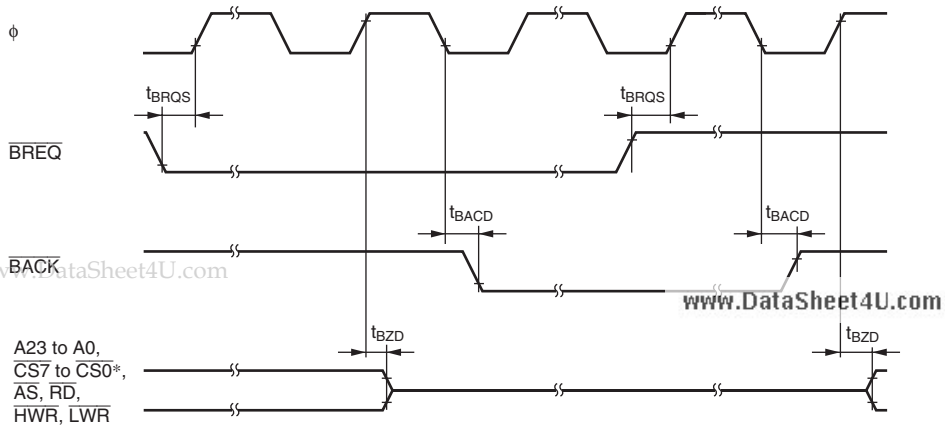
Figure 24.13 External Bus-Released Timing
