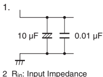
Figure 15.10 Example of Analog Input Protection Circuit
