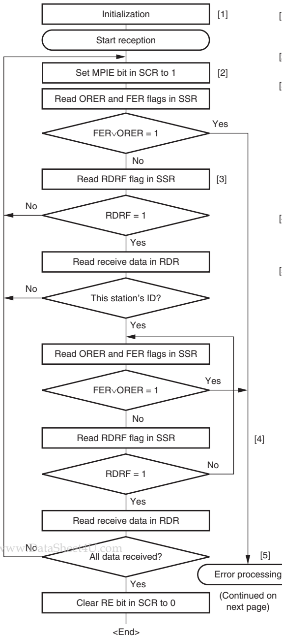
Figure 13.13 Sample Multiprocessor Serial Reception Flowchart (1)
