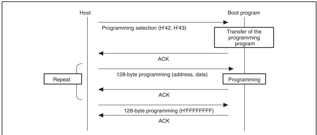
Figure 20.27 Programming Sequence
