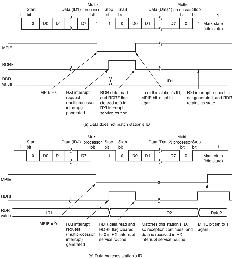
Figure 13.12 Example of SCI Operation in www.DataSheet4U.com (Example with 8-Bit Data, Multiprocessor Bit, One Stop Bit)
