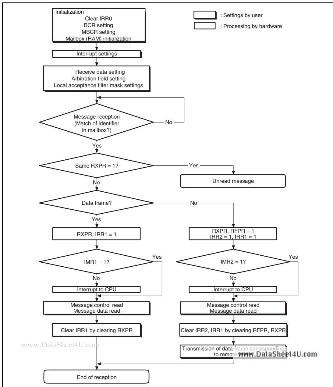
Figure 18.11 Reception Flowchart
