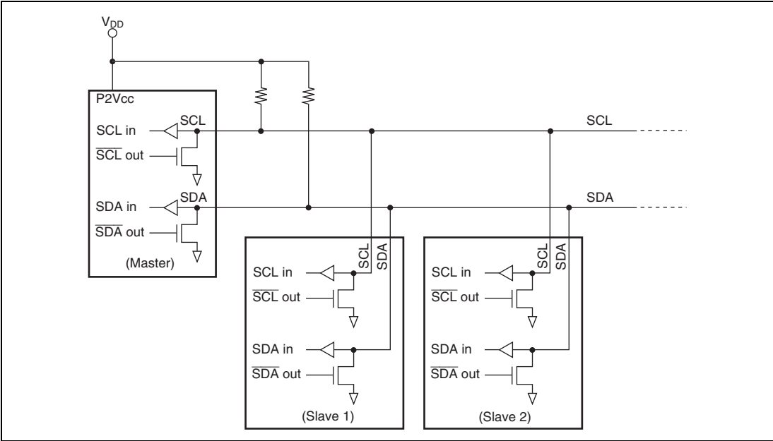
Figure 14.2 External Circuit Connections of I/O Pins
