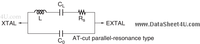
Figure 21.3 Crystal Resonator Equivalent Circuit
