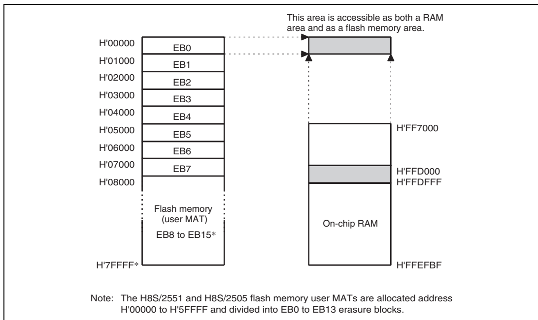
Figure 20.18 Example of a RAM-Overlap Operation
