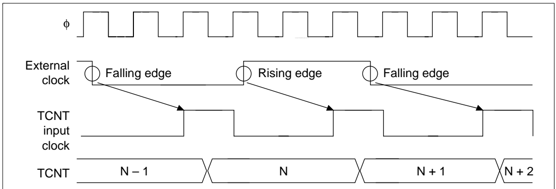
Figure 12.60 TCNT Count Timing during External Clock Operation (Normal Mode)
