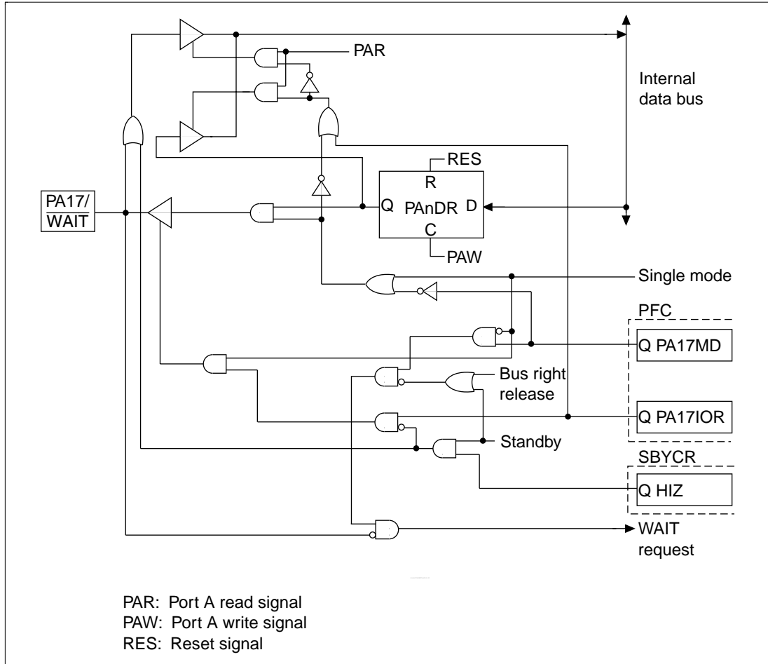
Figure B.13 PA17/WAIT Block Diagram
