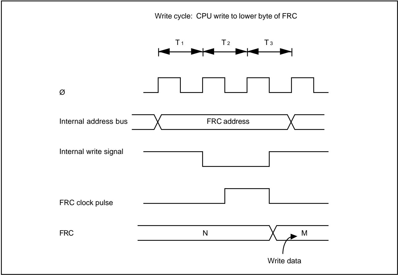
Figure 6-19. FRC Write-Increment Contention
