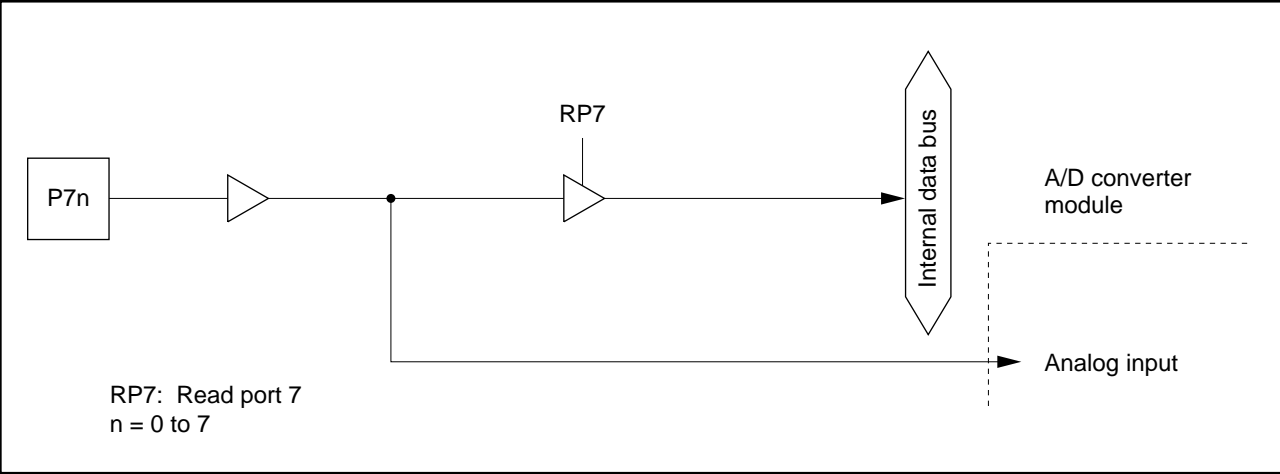
Figure 5-19. Port 7 Schematic Diagram
