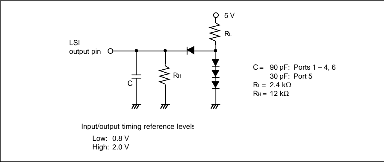
Figure 14-3. Output Load Circuit
