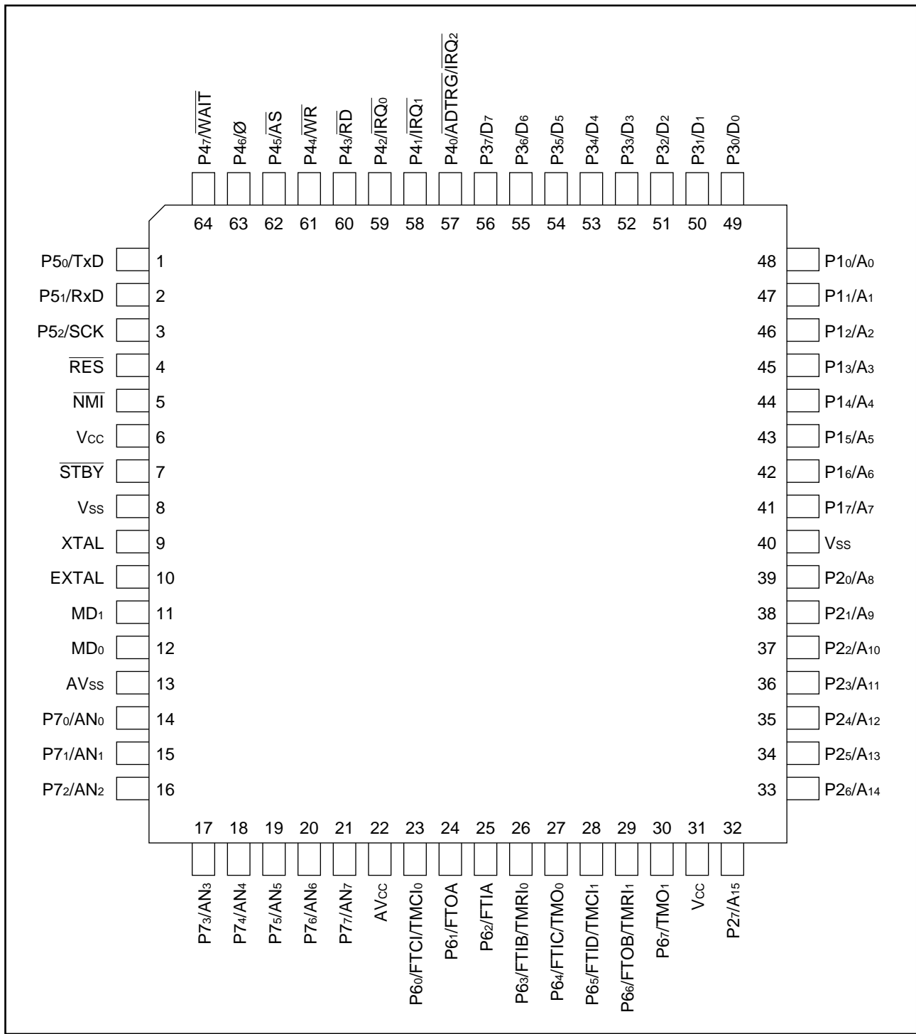
Figure 1-3. Pin Arrangement (FP-64A, Top View)
