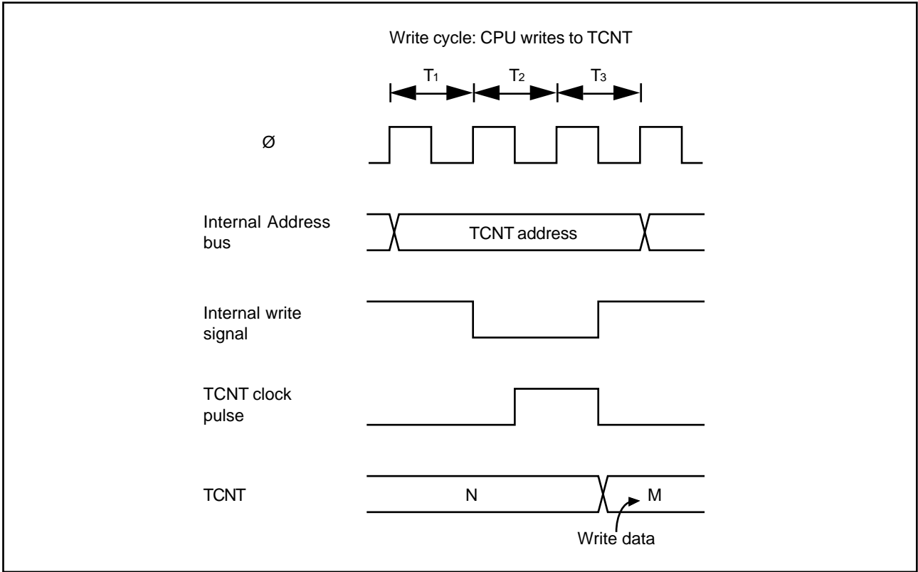
Figure 7-7. Timing of Compare-Match Clear
