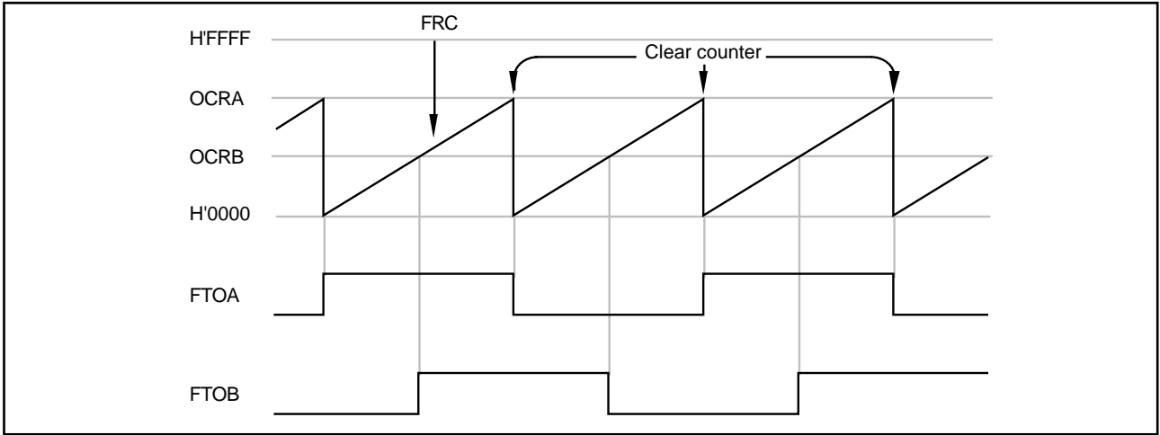
Figure 6-17. Square-Wave Output (Example)
