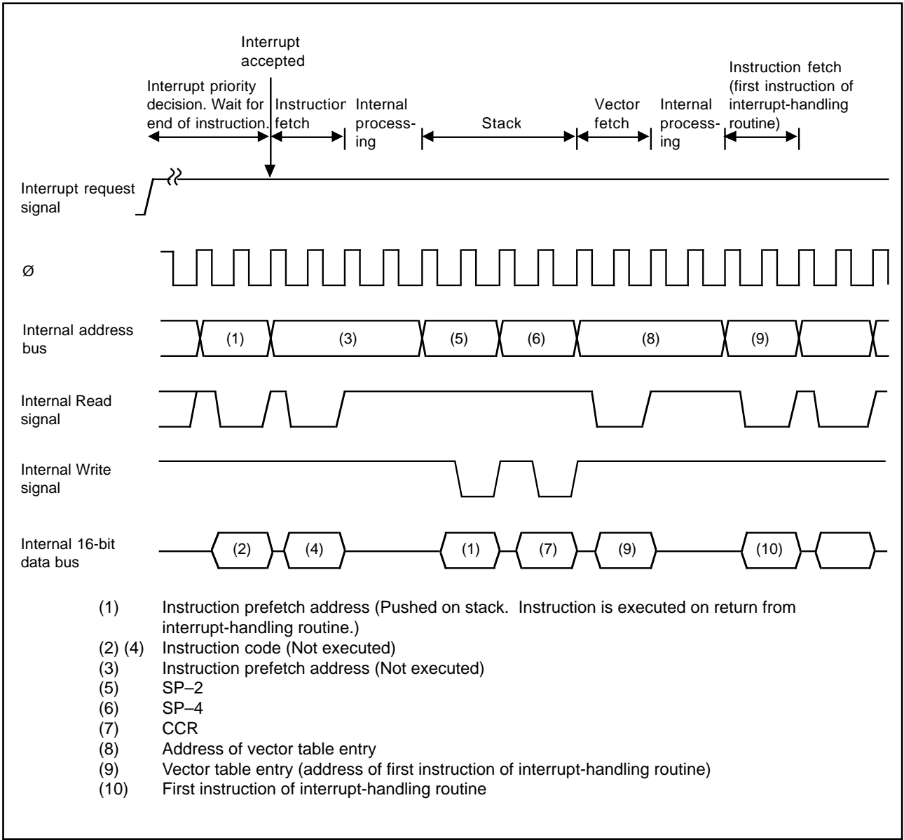
Figure 4-6. Timing of Interrupt Sequence
