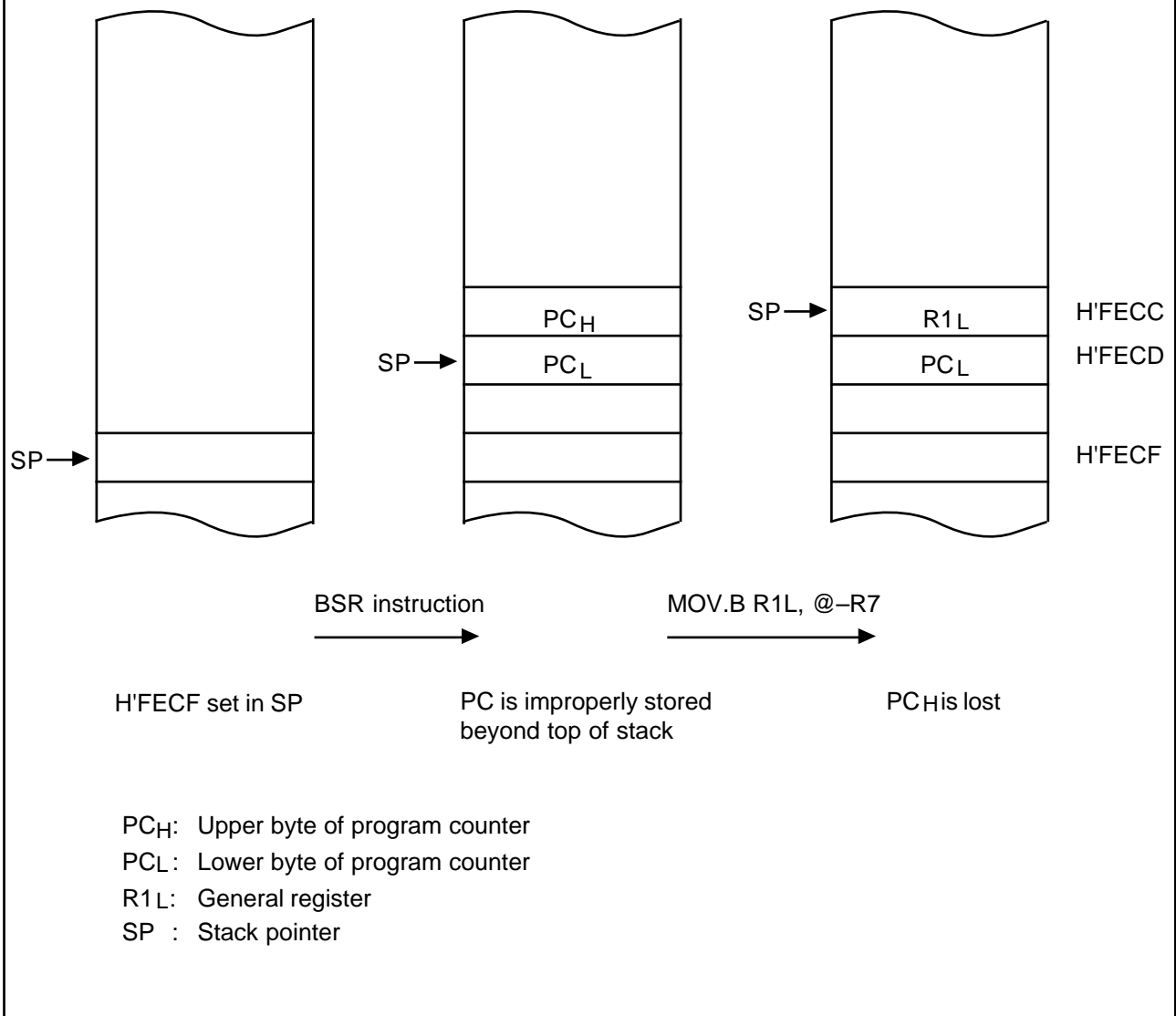
Figure 4-8. Example of Damage Caused by Setting an Odd Address in R7
