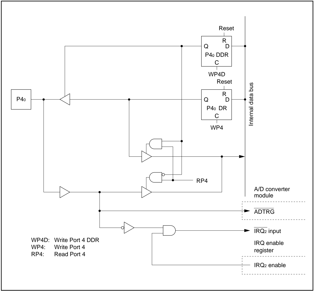
Figure 5-4. Port 4 Schematic Diagram (Pin P40)
