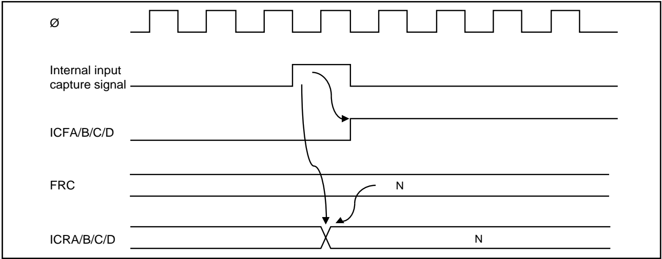
Figure 6-15. Setting of Input Capture Flag
