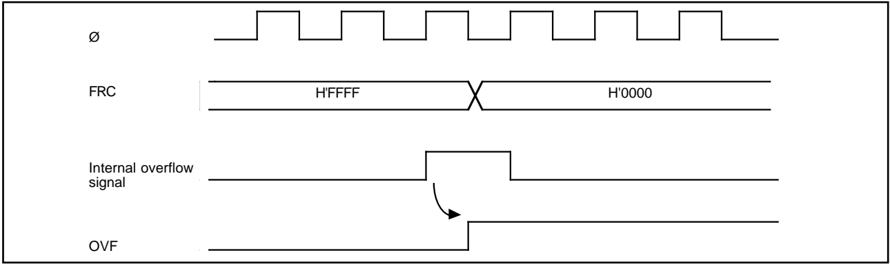
Figure 6-16. Setting of Overflow Flag (OVF)
