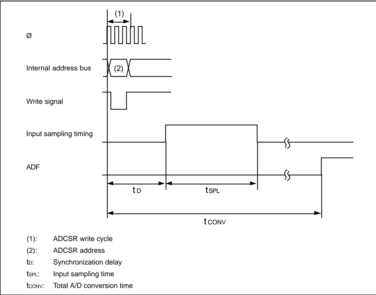
Figure 9-4. A/D Conversion Timing
