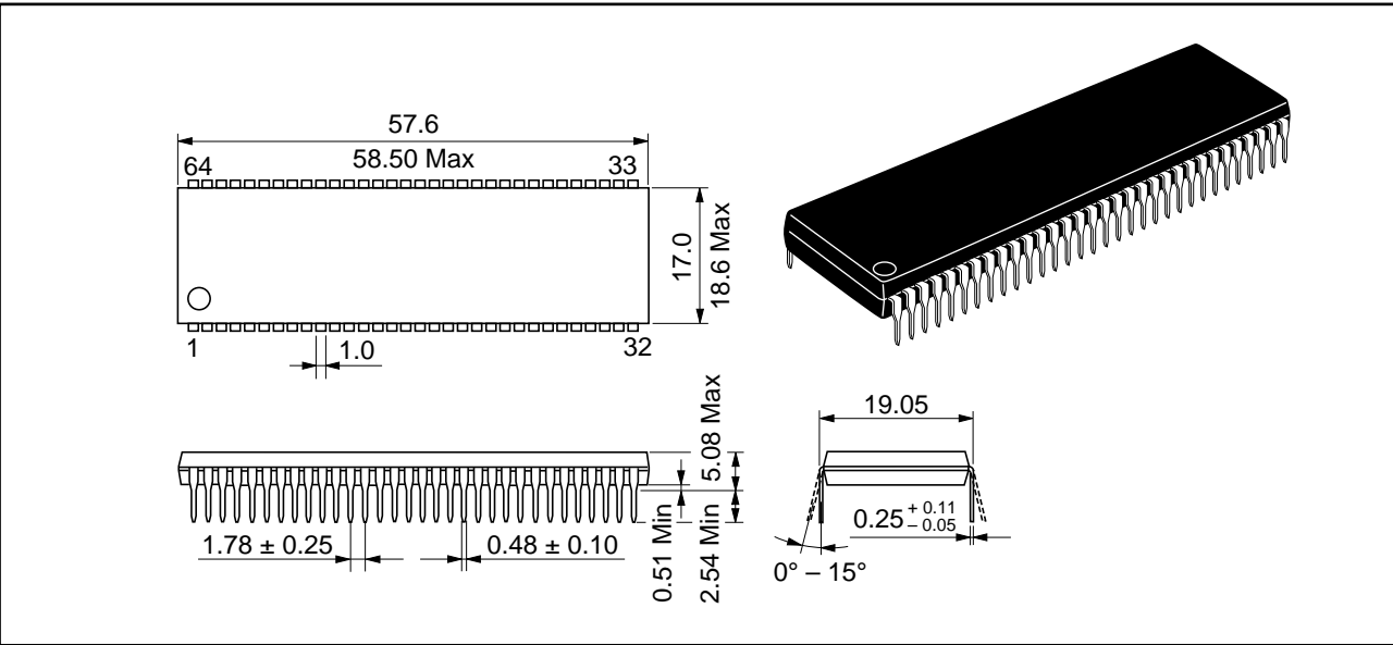
Figure E-2. Package Dimensions (DP-64S)
