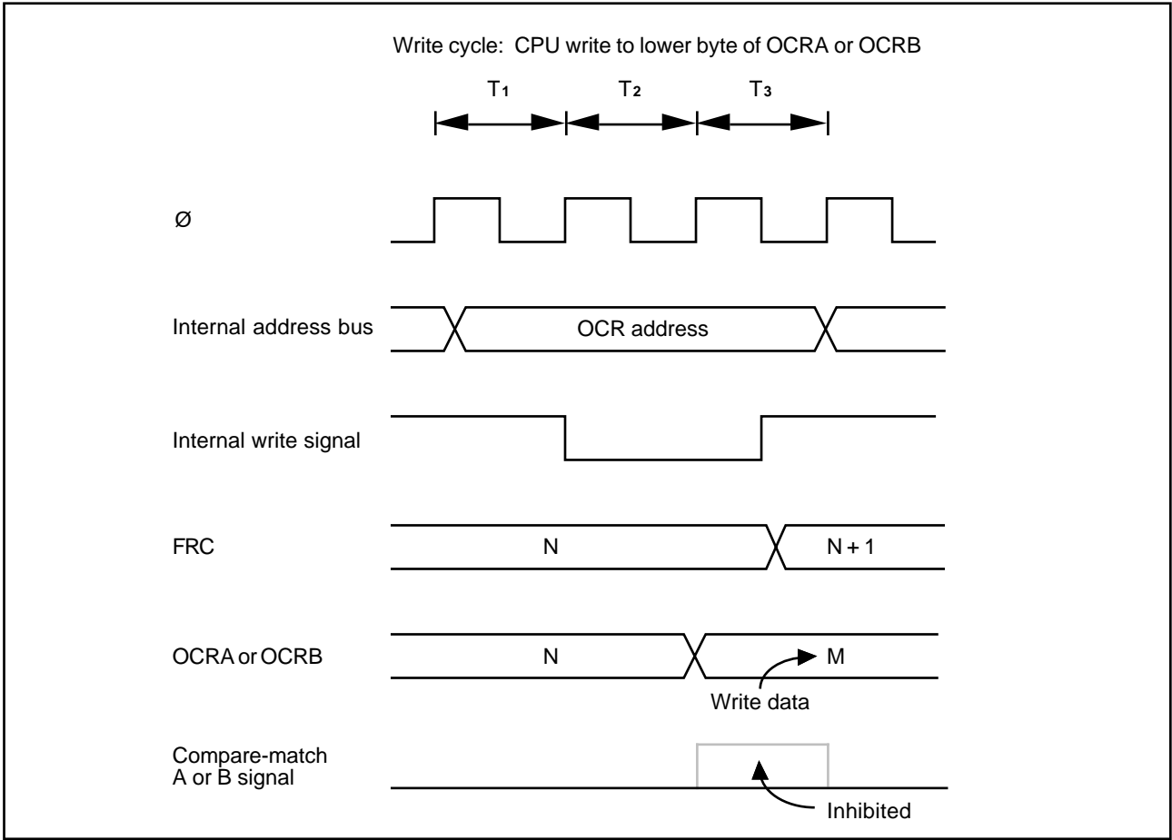
Figure 6-20. Contention between OCR Write and Compare-Match
