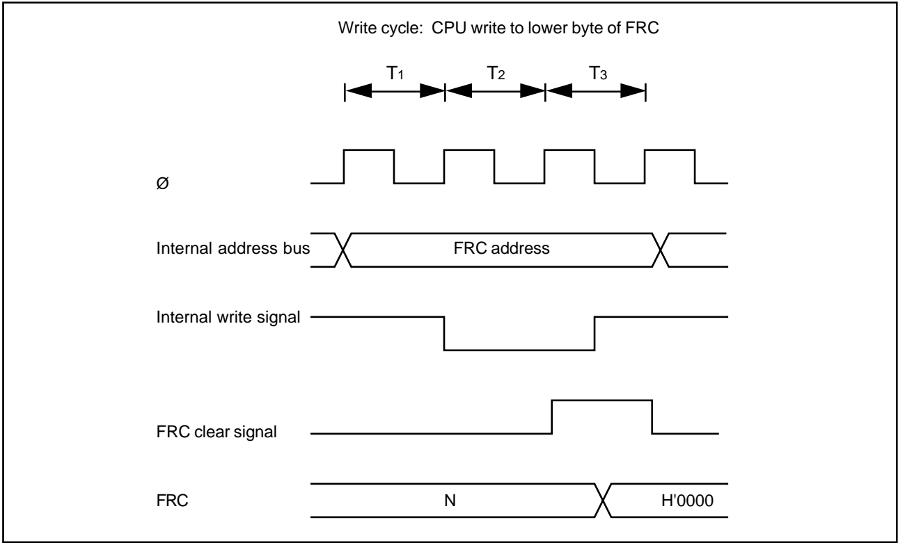
Figure 6-18. FRC Write-Clear Contention
