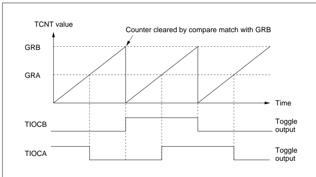
Figure 8-21 Toggle Output (Example)
