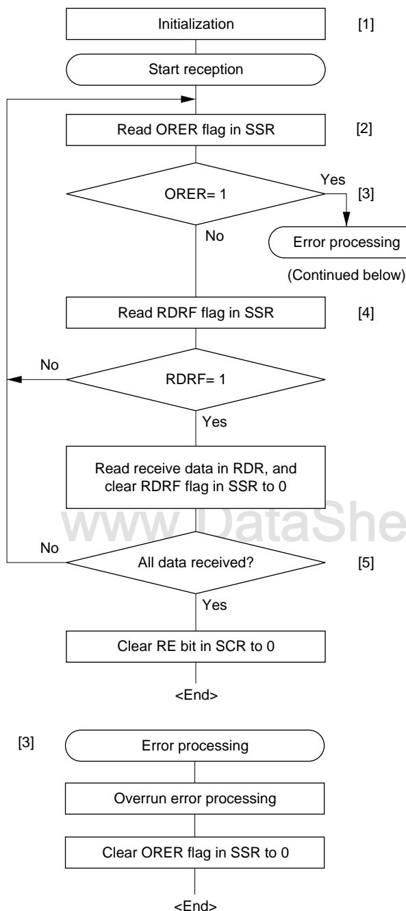
Figure 12.18 Sample Serial Reception Flowchart
