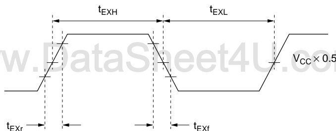
Figure 18.6 External Clock Input Timing
