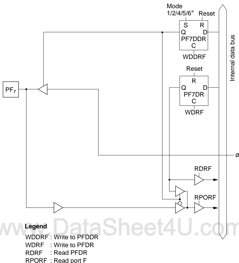
Figure C.10 (h) Port F Block Diagram (Pin PF 7 )
