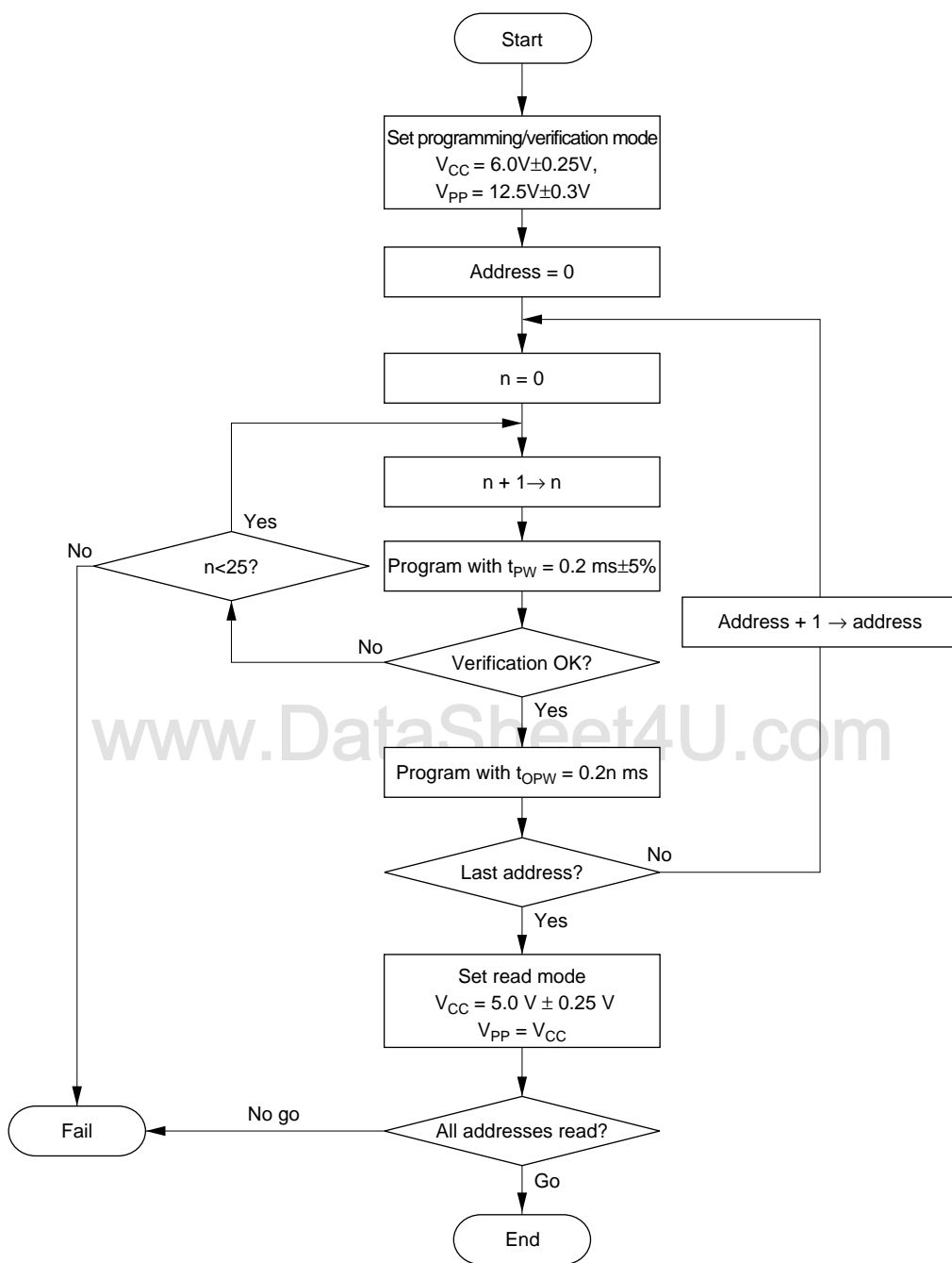
Figure 17.4 High-Speed Programming Flowchart
