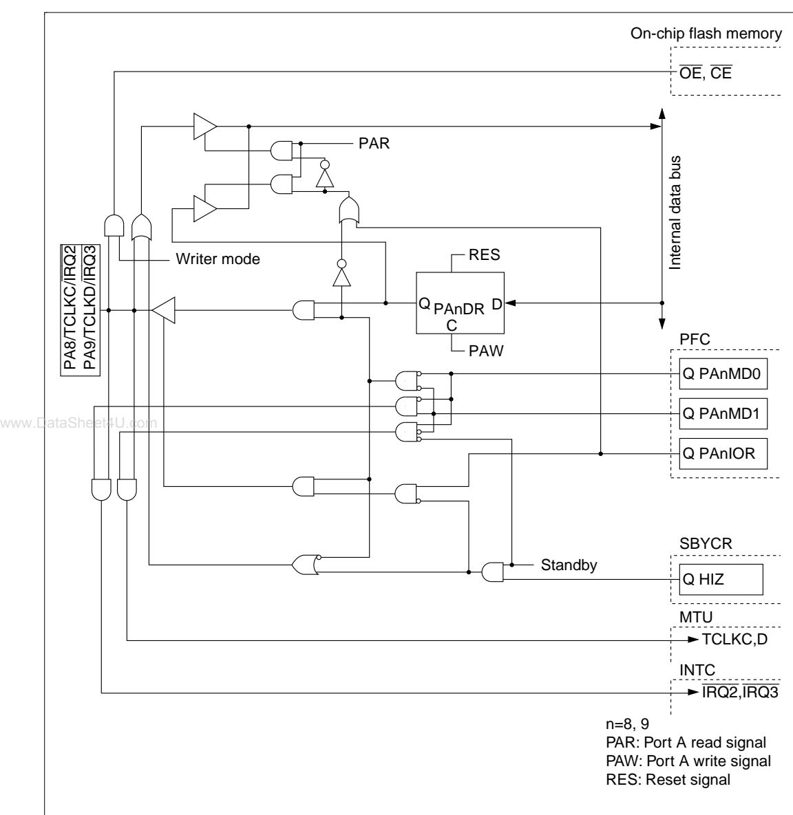
Figure B.6 PAn/TCLKm/IRQx Block Diagram (F-ZTAT Version)
