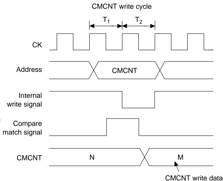
Figure 17.7 CMCNT Word Write and Increment Contention
