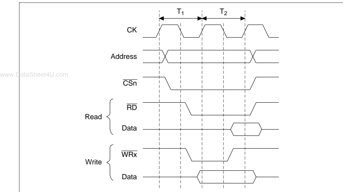
Figure 10.3 Basic Timing of Ordinary Space Access
