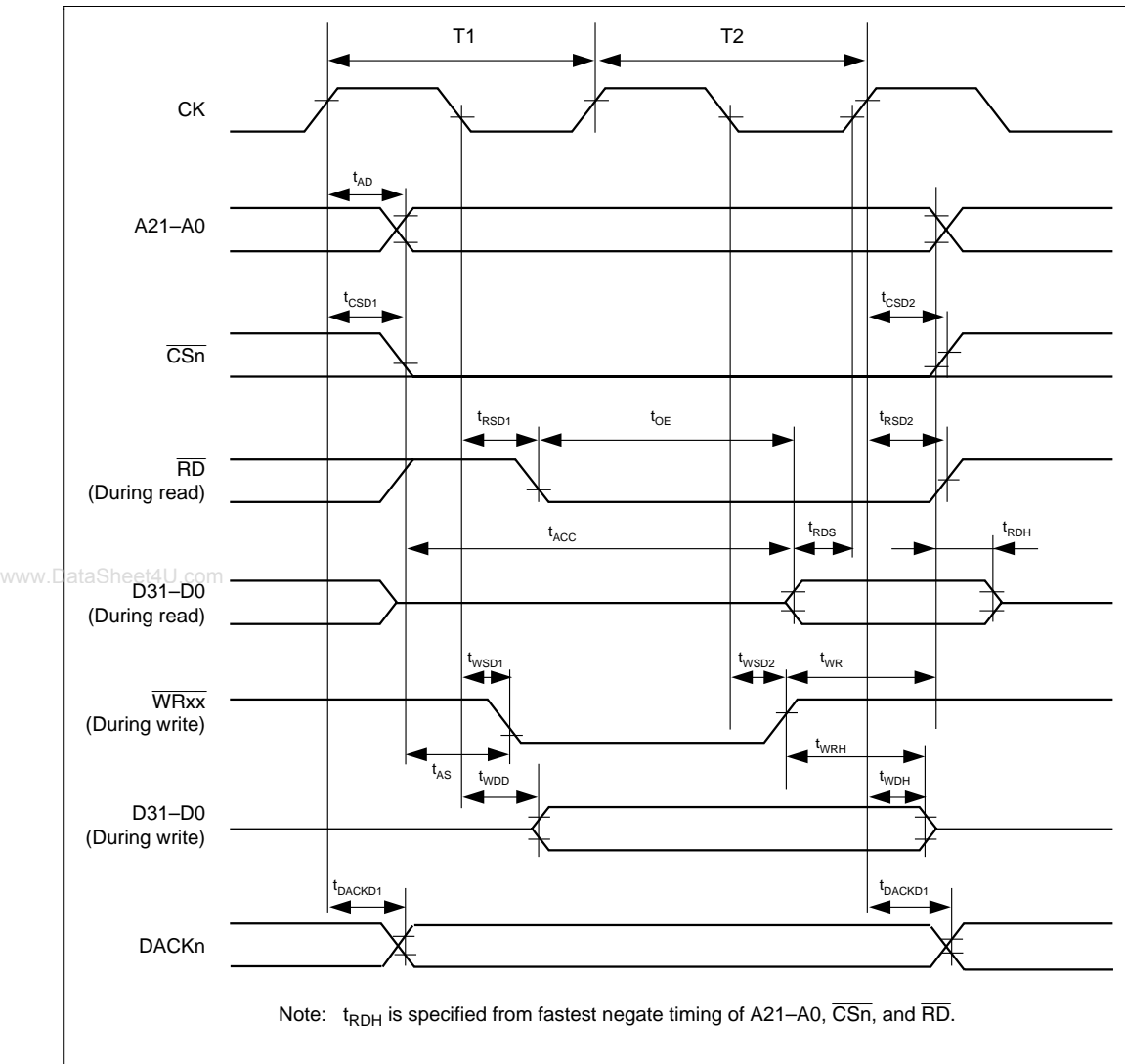
Figure 26.8 Basic Cycle (No Waits)
