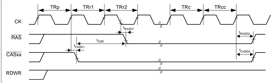
Figure 25.18 Self Refresh
