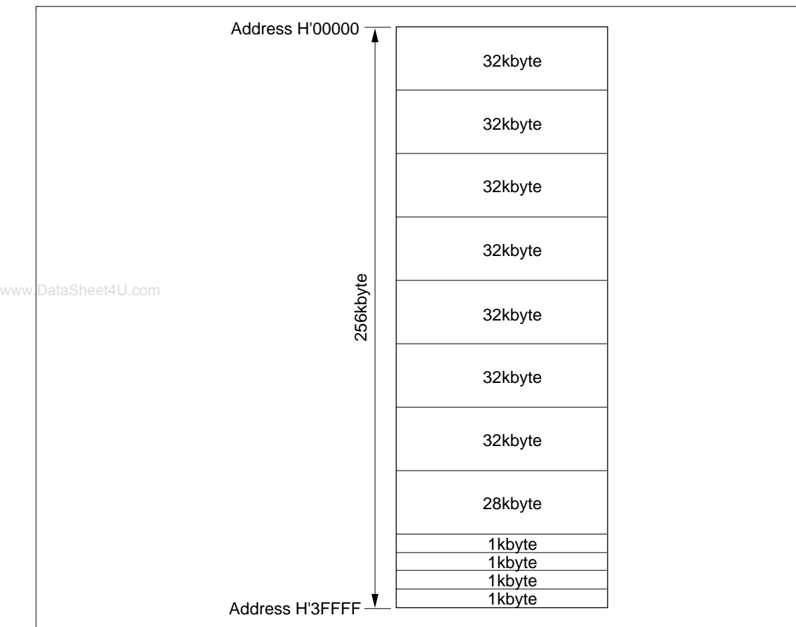
Figure 22.7 Block Configuration
