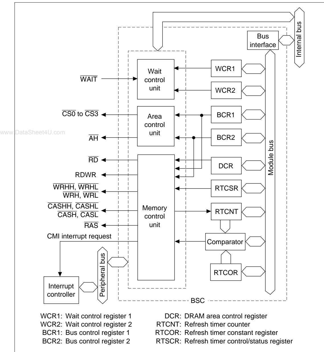
Figure 10.1 BSC Block Diagram
