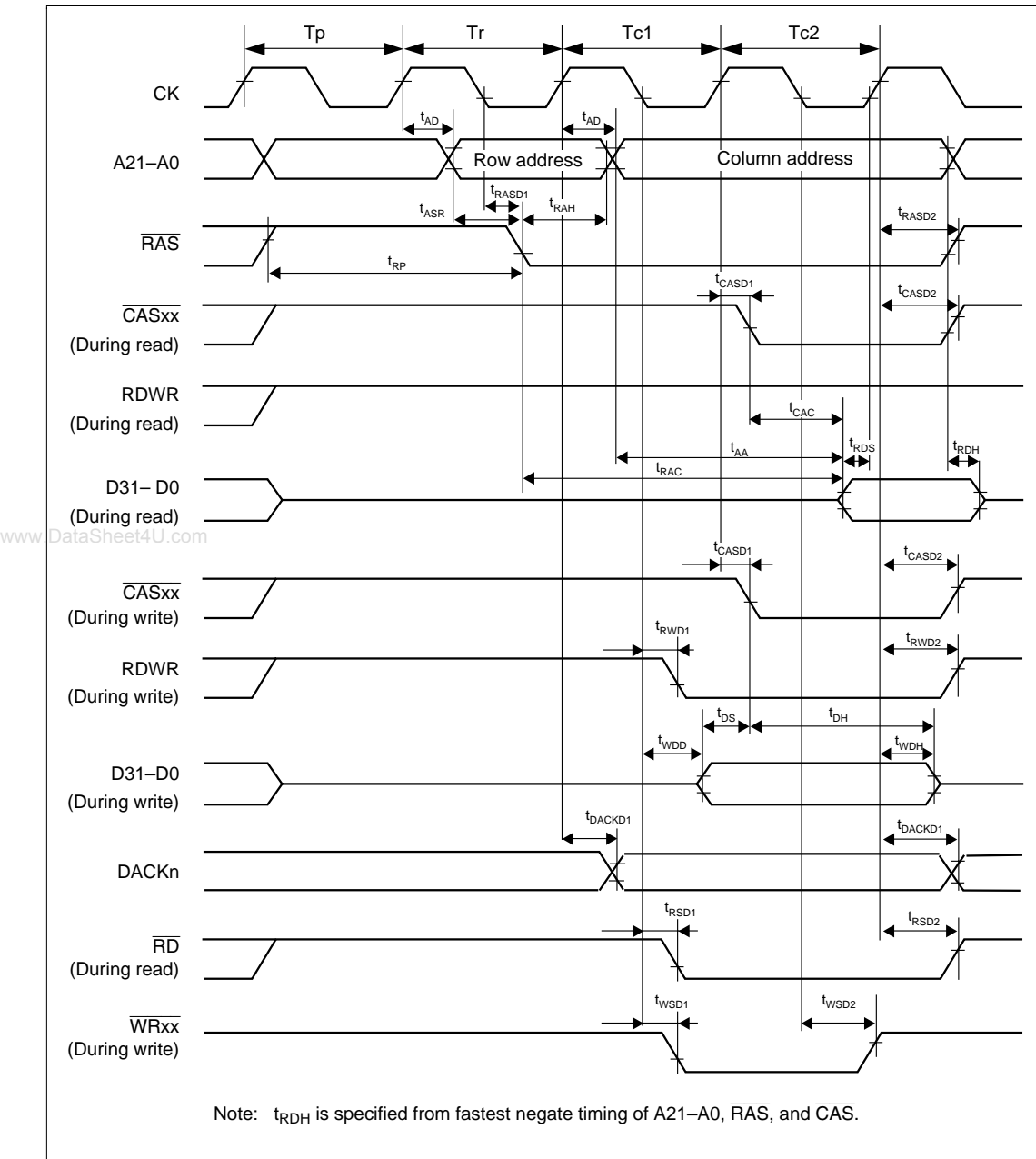
Figure 26.11 DRAM Cycle (Normal Mode, No Wait, TPC = 0, RCD = 0)
