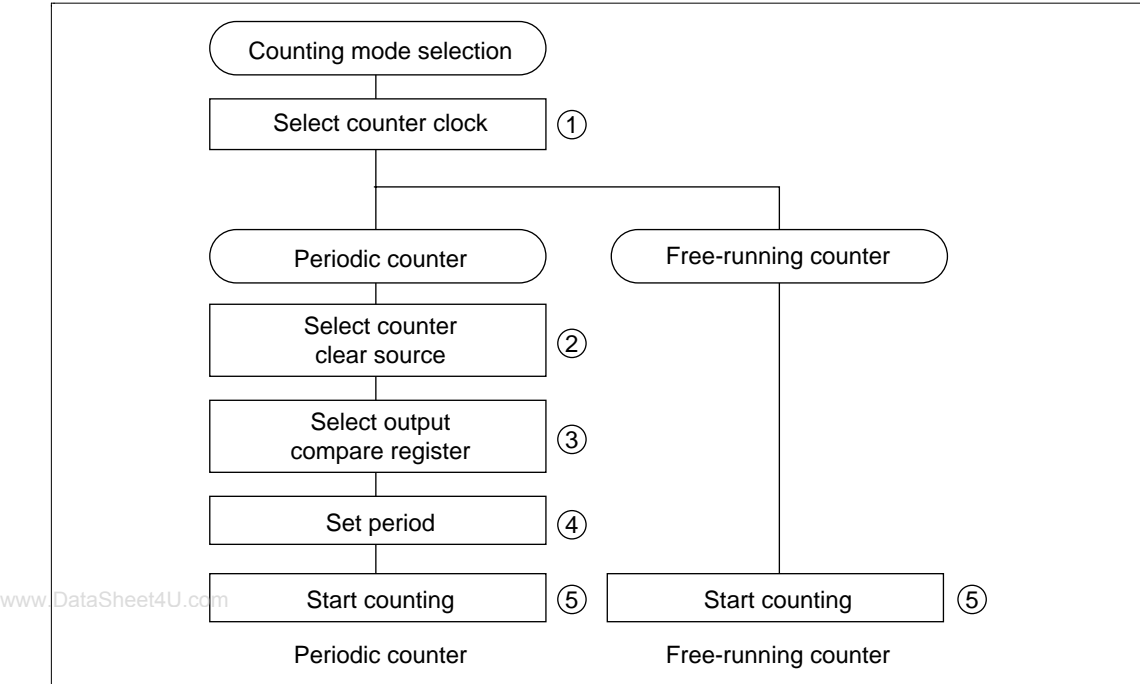
Figure 12.7 Procedure for Selecting the Counting Operation
