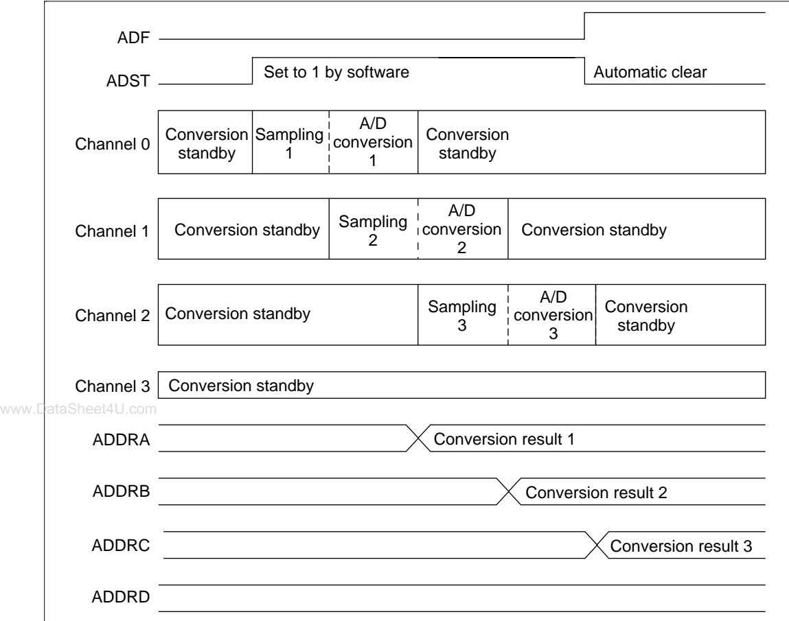
Figure 15.6 A/D Converter Operation Example (Group-Single Mode)
