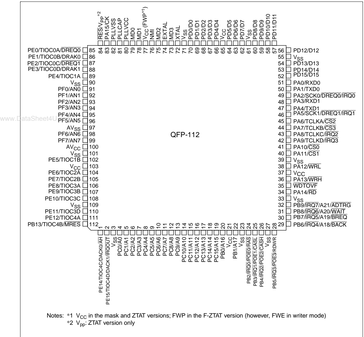
Figure 1.3 SH7040, SH7042, SH7044 Pin Arrangement (QFP-112 Top View)
