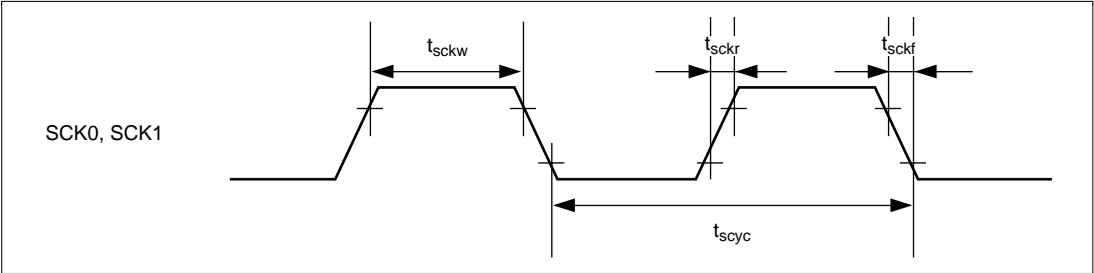
Figure 26.27 Input Clock Timing
