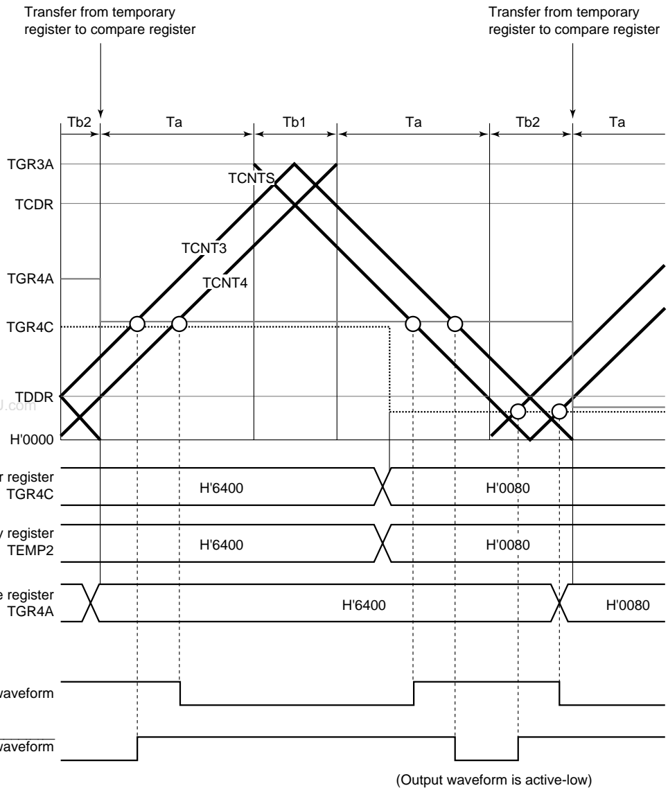
Figure 12.40 Example of Complementary PWM Mode Operation
