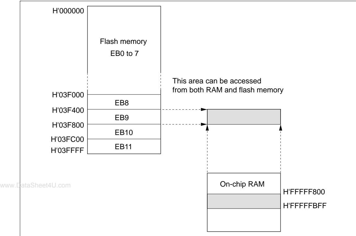
Figure 22.17 Example of RAM Overlap Operation
