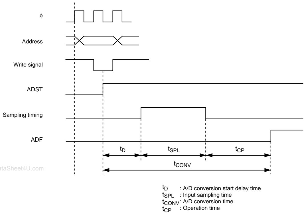
Figure 25.30 Analog Conversion Timing
