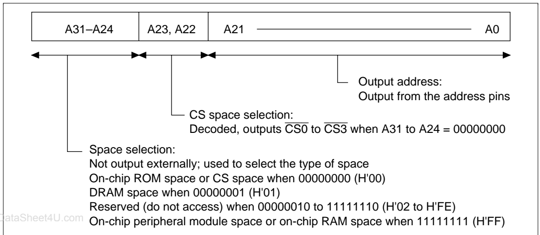
Figure 10.2 Address Format
