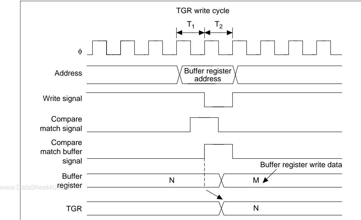
Figure 12.80 TGR Write and Compare-Match Contention (Channels 3 and 4)
