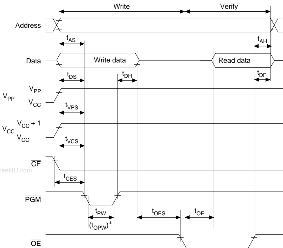
Figure 21.7 Write/Verify Timing
