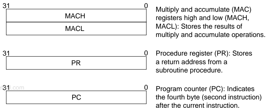
Figure 2.3 System Registers
