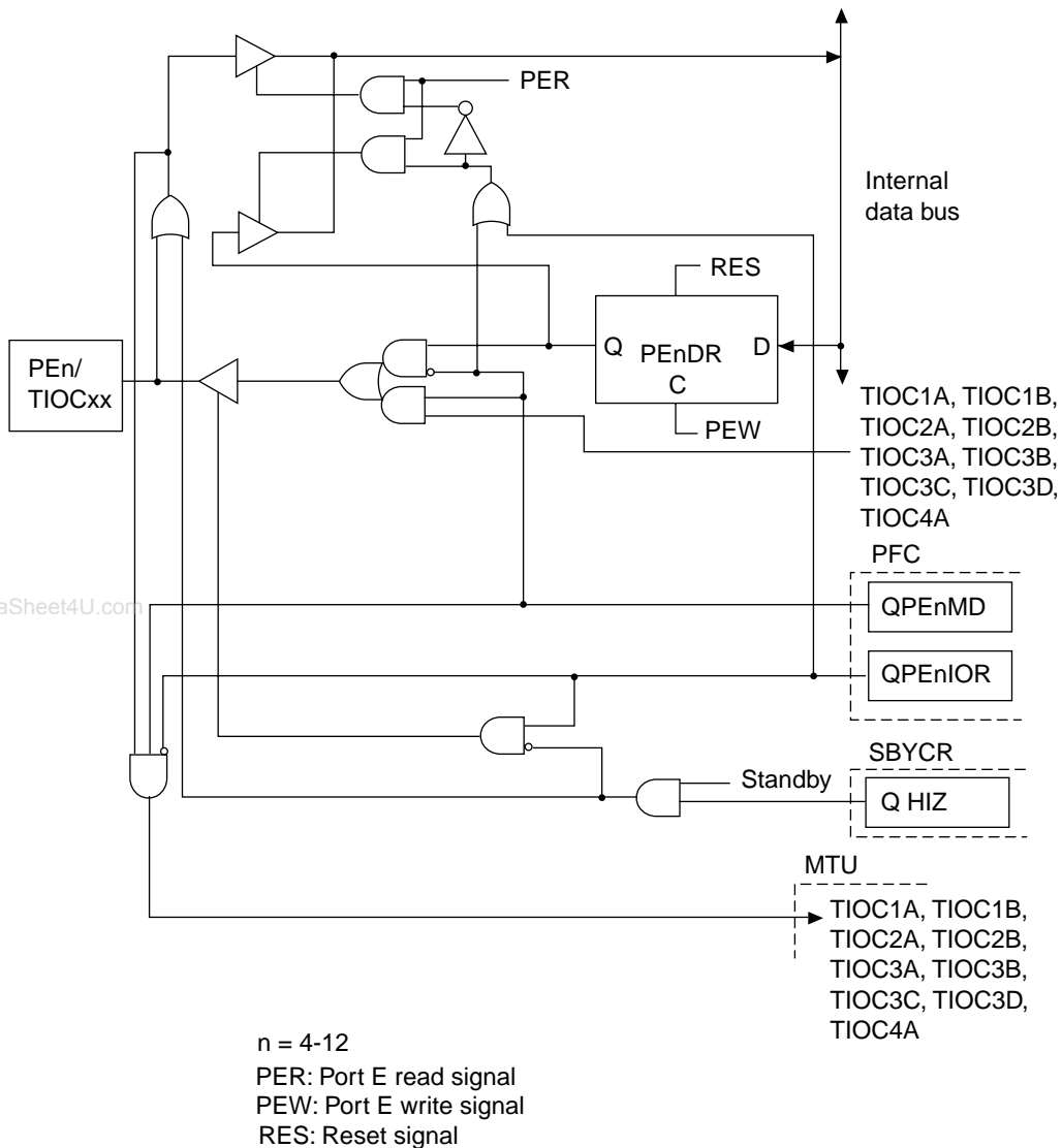
Figure B.36 PEn/TIOCXX Block Diagram
