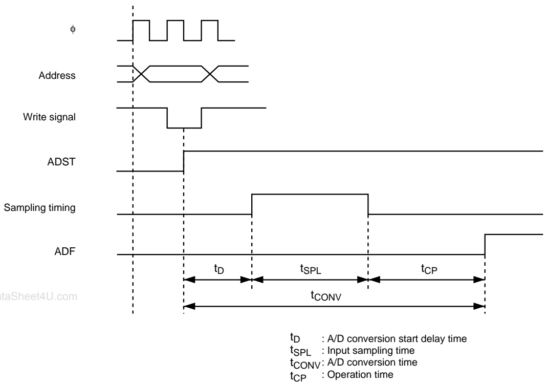
Figure 26.30 Analog Conversion Timing
