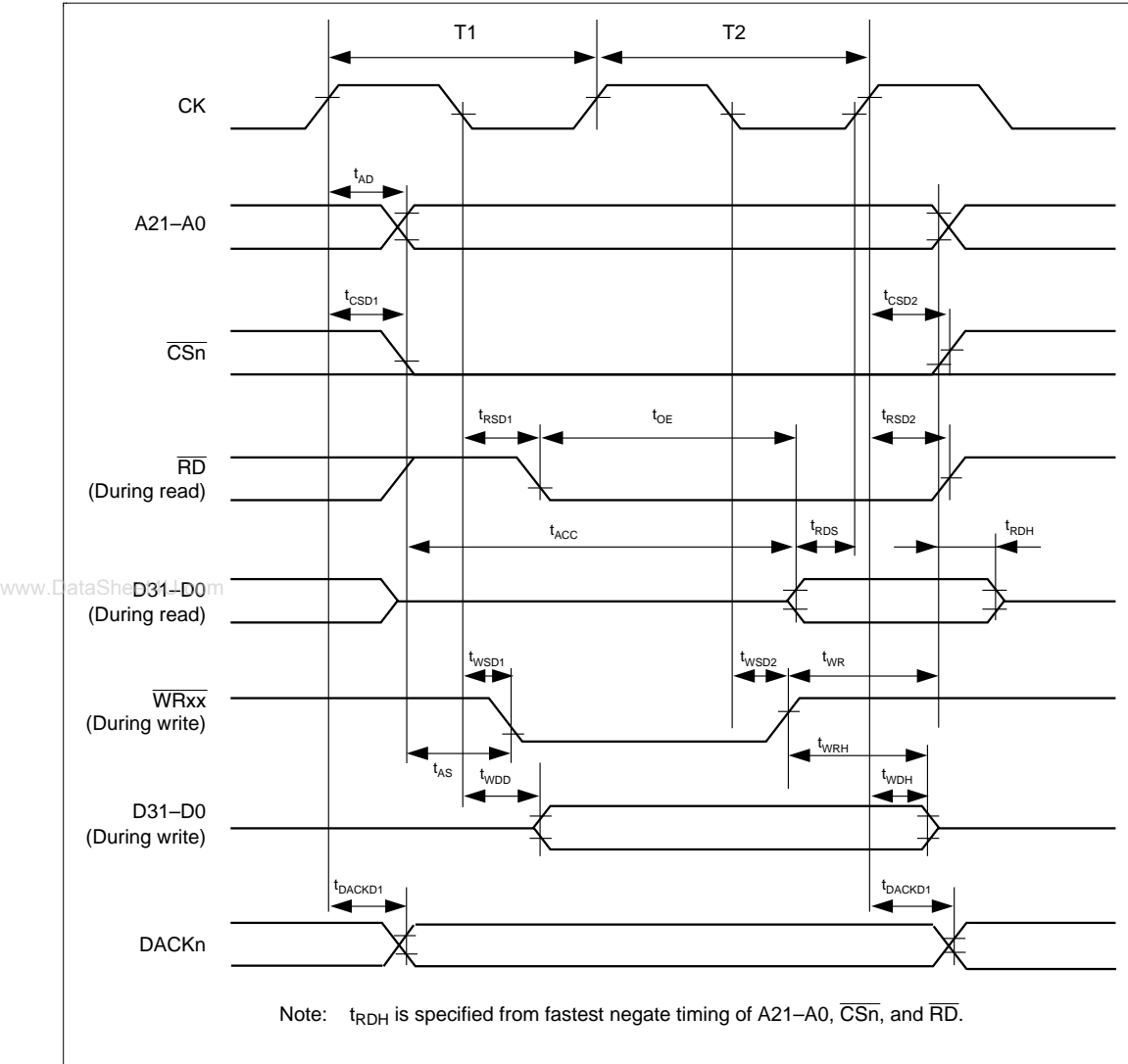
Figure 25.8 Basic Cycle (No Waits)
