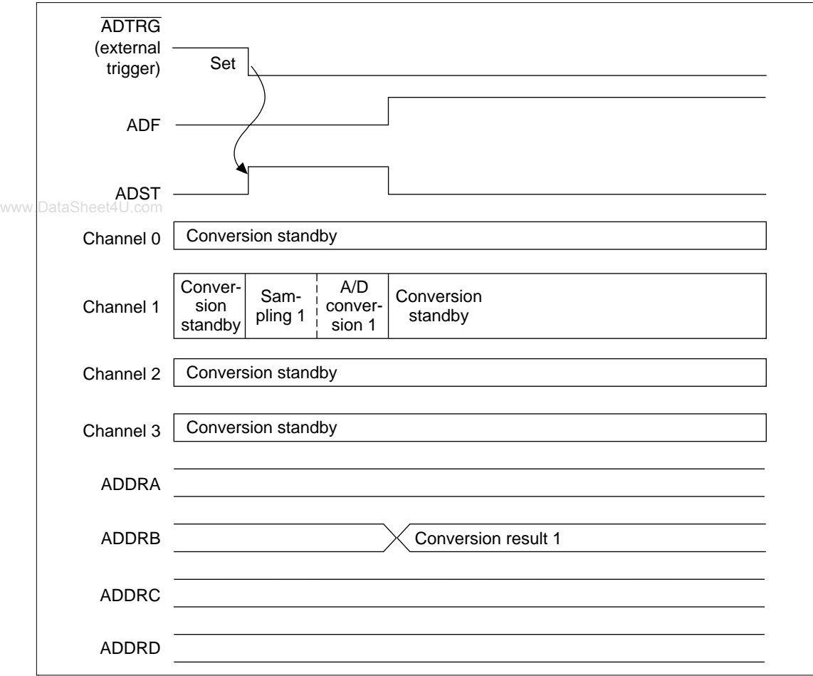
Figure 15.12 Conversion Start by ADTRG Conversion Start Trigger
