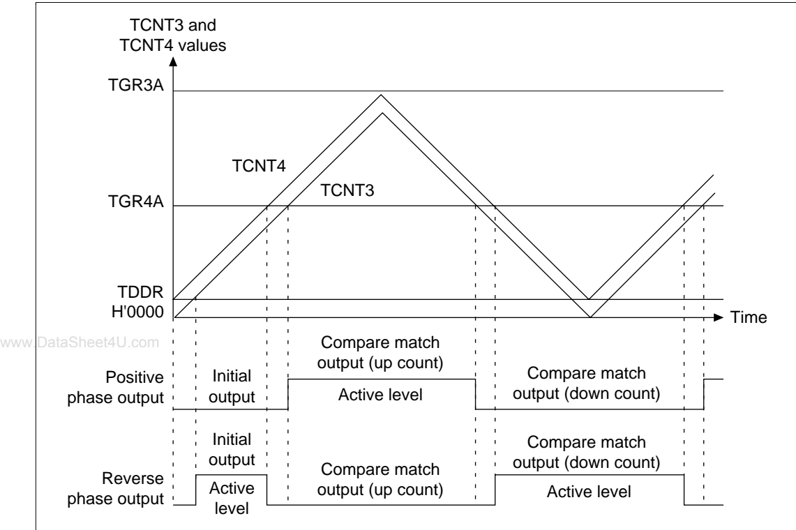
Figure 12.2 Complementary PWM Mode Output Level Example
