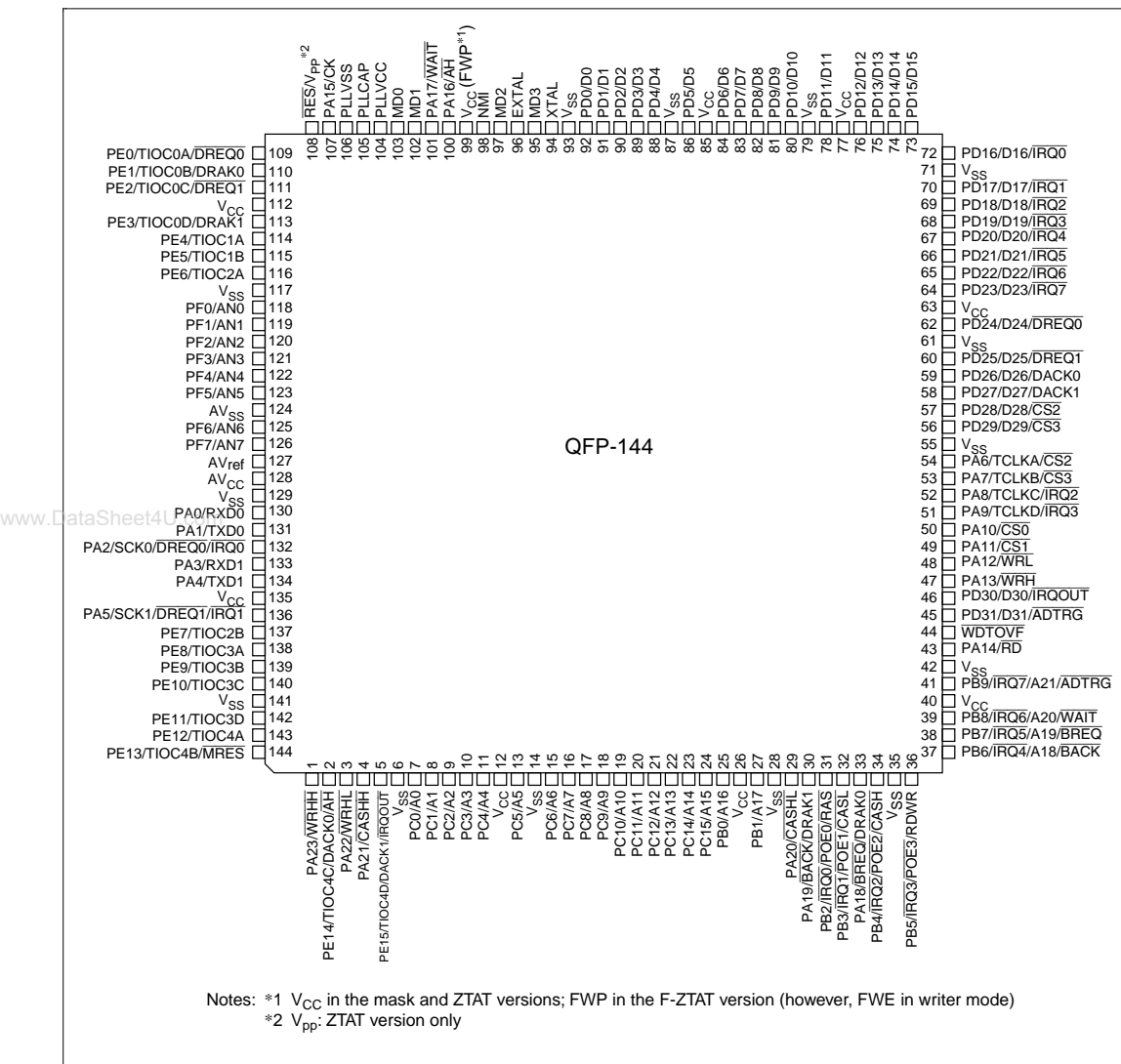
Figure 1.5 SH7041, SH7043, SH7045 Pin Arrangement (QFP-144 Top View)
