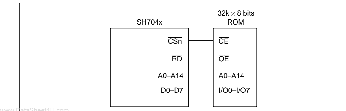
Figure 10.23 8-Bit Data Bus Width ROM Connection
