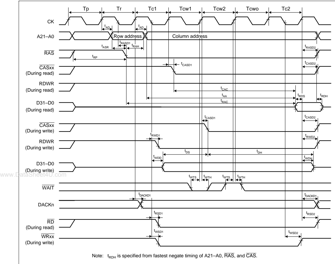
Figure 25.15 DRAM Cycle (Normal Mode, 2 Waits + Wait due to WAIT Signal)
