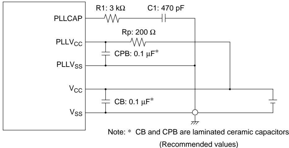
Figure 4.6 Cautions for Use of PLL Oscillator Circuit
