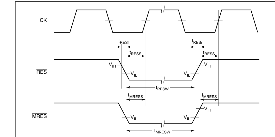
Figure 26.4 Reset Input Timing
