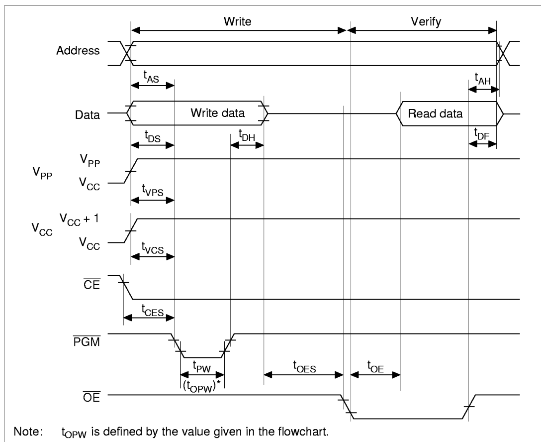
Figure 17.5 Write/Verify Timing
