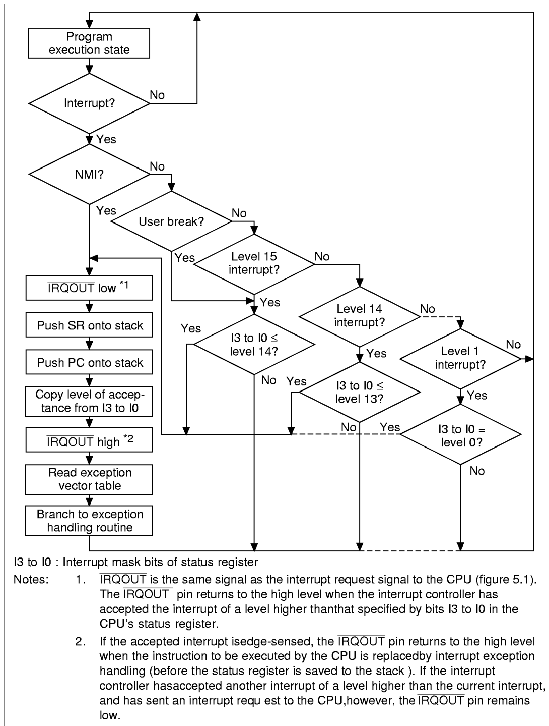
Figure 5.2 Flowchart of Interrupt Operation
