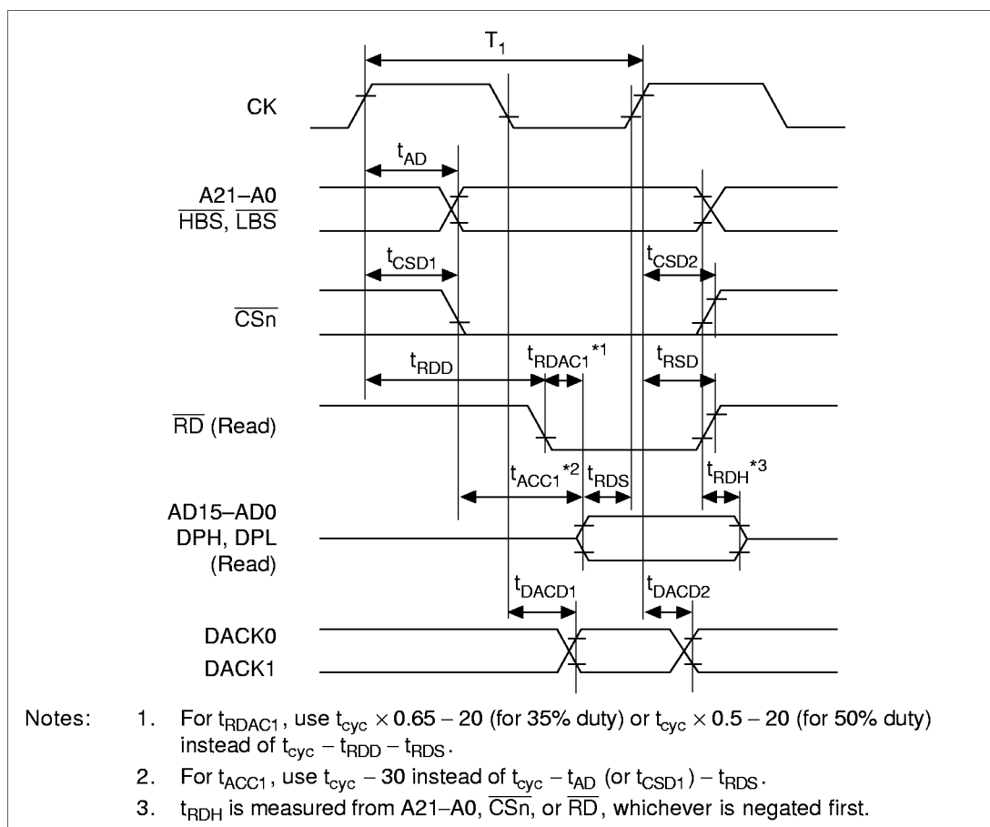
Figure 20.8 Basic Bus Cycle: One-State Access
