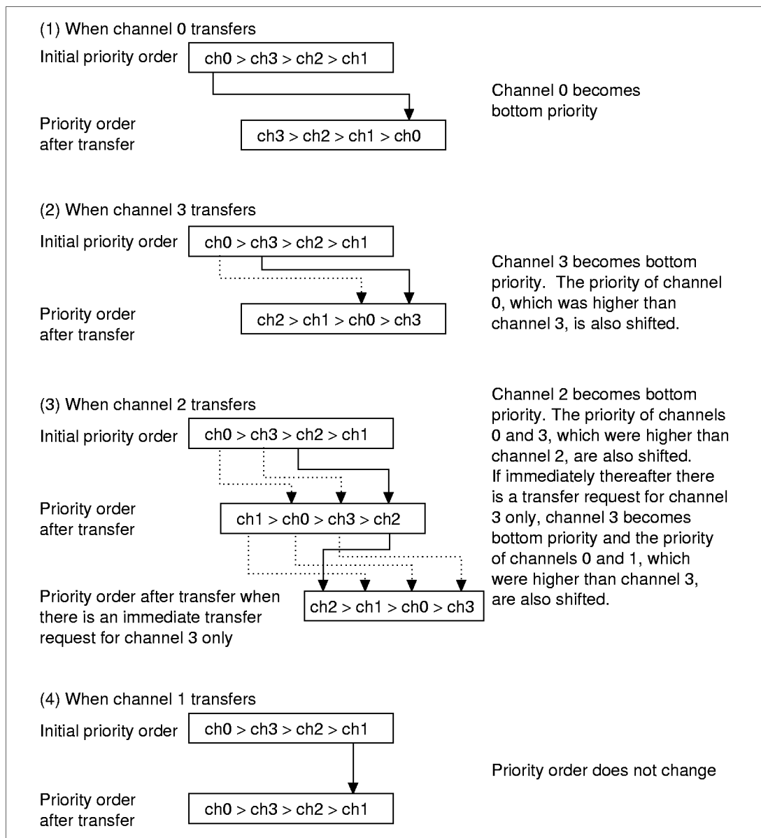
Figure 9.3 Round-Robin Mode
