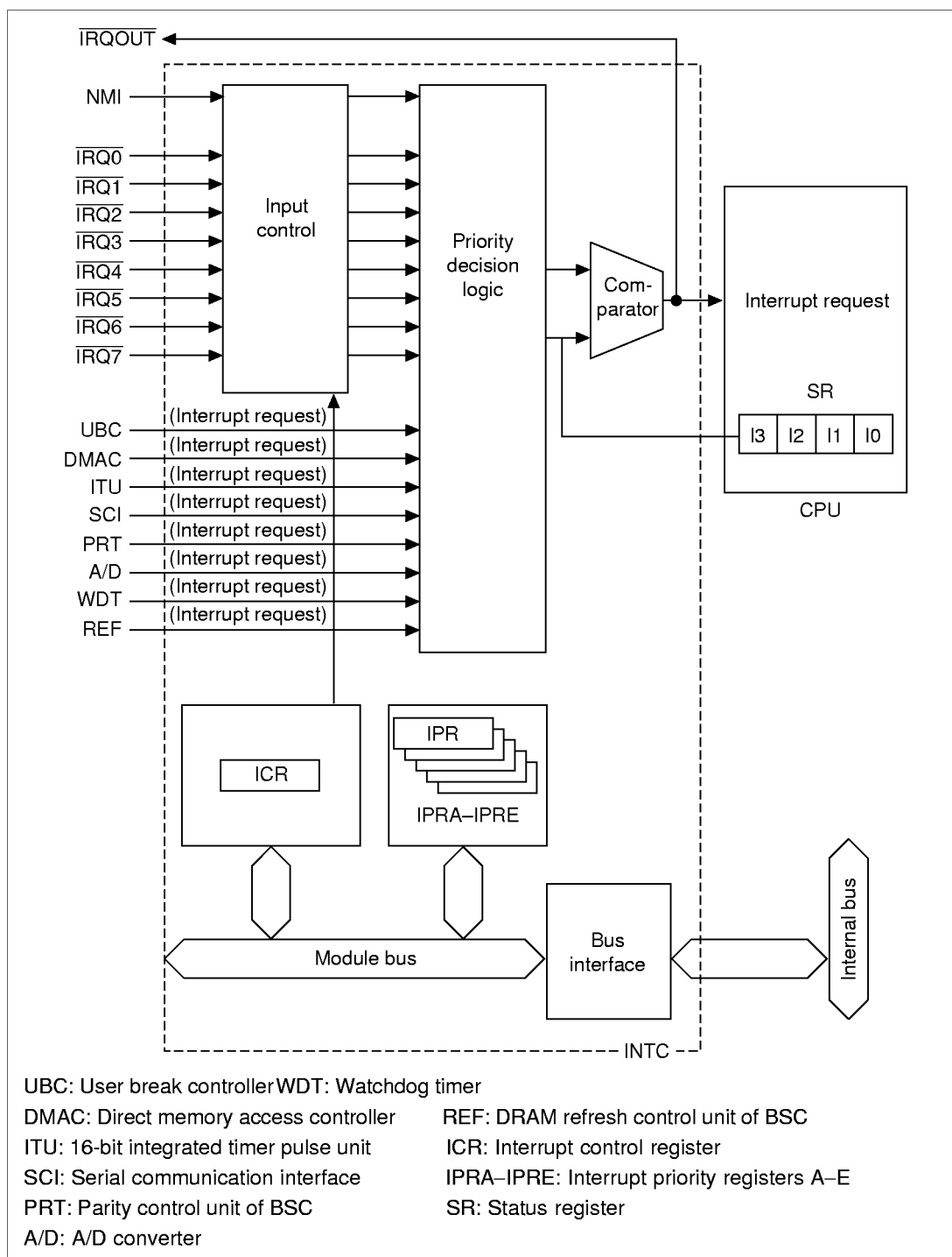
Figure 5.1 Block Diagram of Interrupt Controller
