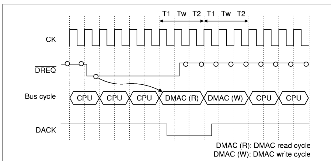
Figure 9.18 \overline{DREQ} Sampling Timing in Cycle-Steal Mode (Output with \overline{DREQ} Level Detection and DACK Active-Low) (Dual Address Mode, Bus Cycle = 2 States + 1 Wait State)
