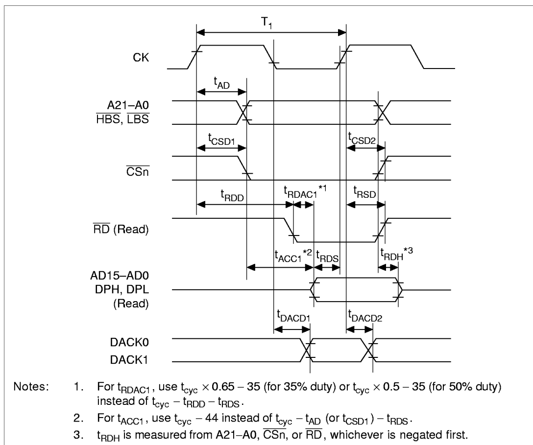
Figure 20.21 Basic Bus Cycle: One-State Access
