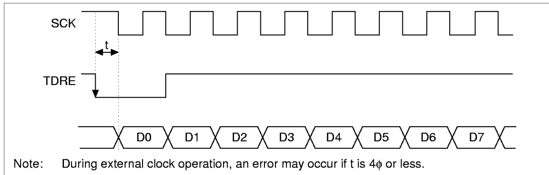
Figure 13.22 Example of Synchronous Transmitting with DMAC
