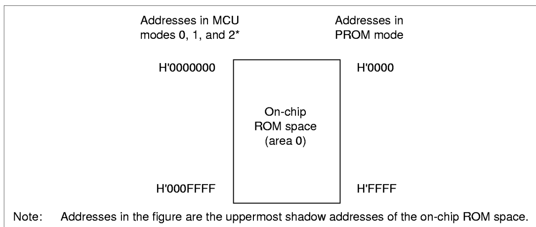
Figure 17.3 Memory Map of On-chip ROM
