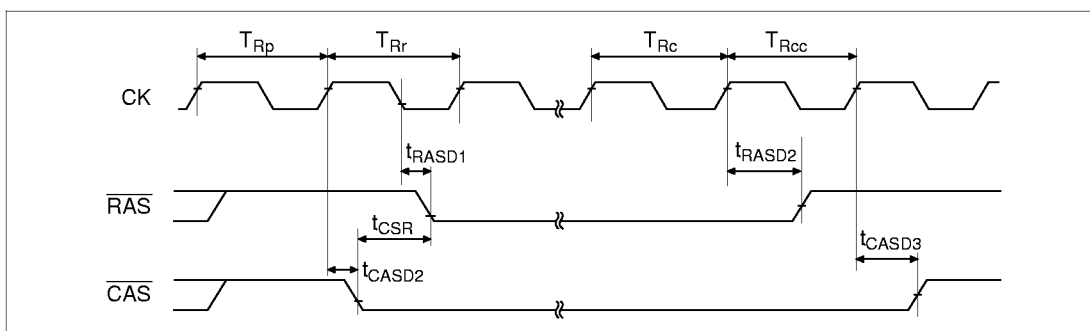
Figure 20.31 Self-Refresh
