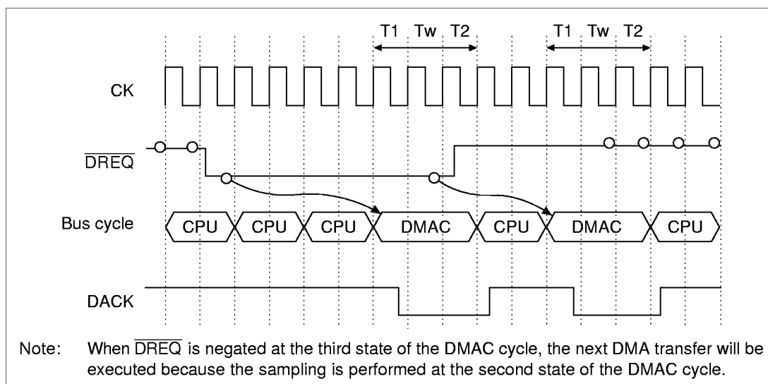
Figure 9.17 \overline{DREQ} Sampling Timing in Cycle-Steal Mode (Output with \overline{DREQ} Level Detection and DACK Active-Low) (Single Address Mode, Bus Cycle = 2 States + 1 Wait State)
