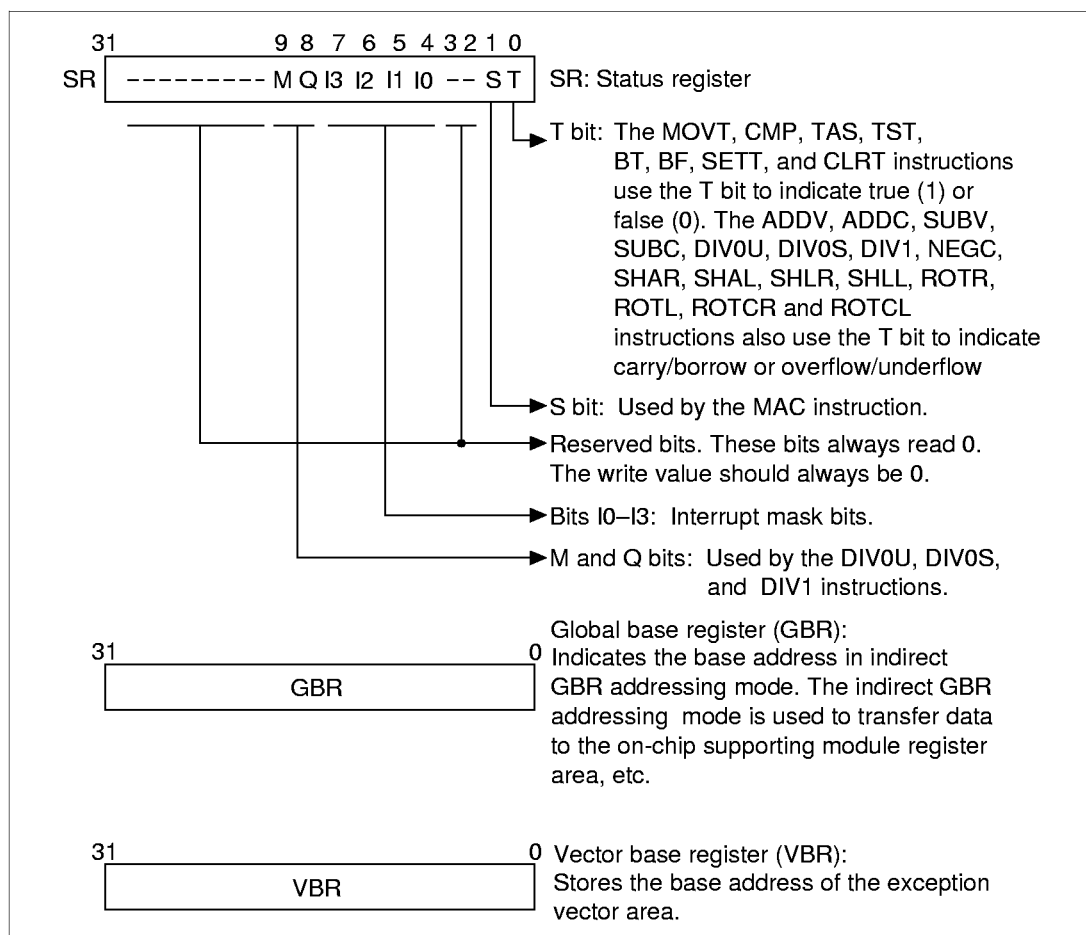
Figure 2.2 Control Registers
