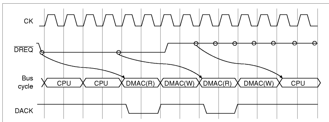
Figure 9.24 DREQ Pin Sampling Timing in Burst Mode (Dual Address DREQ Level Detection, DACK Active-Low, DACK Output in Read Cycle, 1 Bus Cycle = 2 States)
