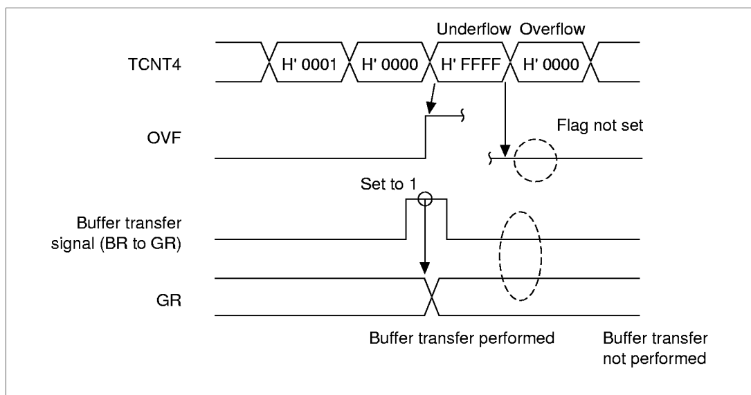
Figure 10.37 Undershoot Timing
