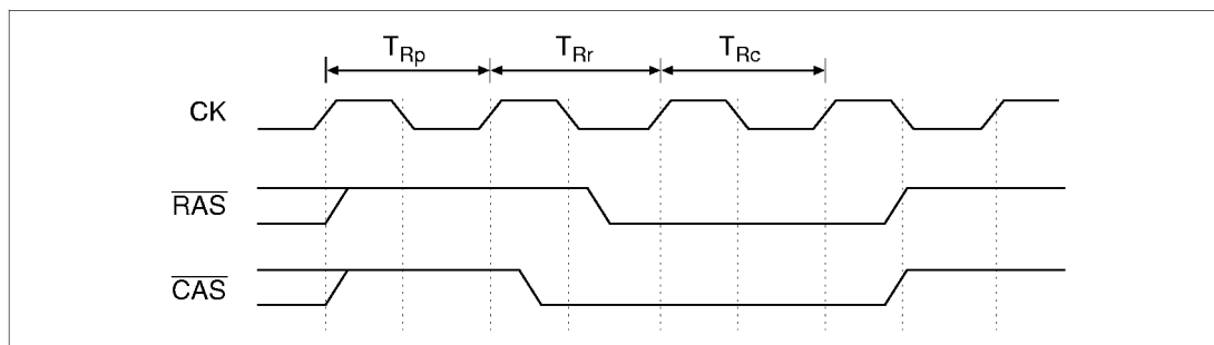
Figure 8.30 Output Timing for CAS-Before-RAS Refresh Signal
