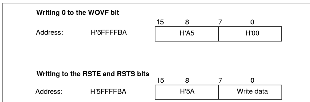
Figure 12.3 Writing to RSTCSR
