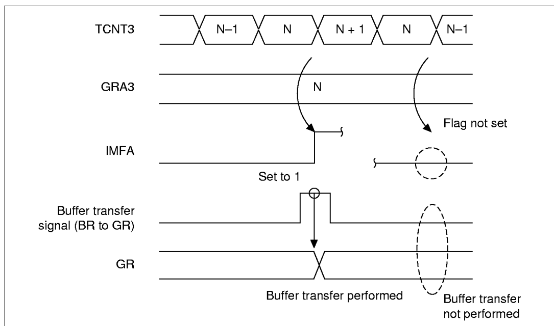
Figure 10.36 Overshoot Timing
