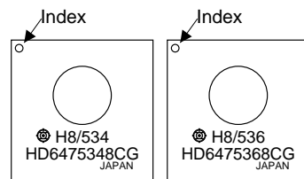
Figure 1-3 Pin Arrangement (CG-84, Top View)
