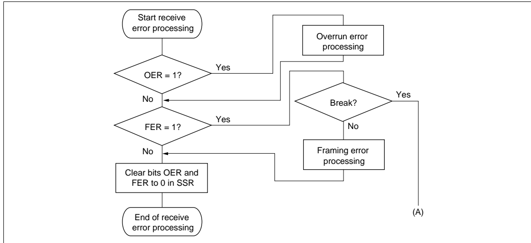
Figure 10-24 Example of Multiprocessor Data Reception Flowchart (cont)
