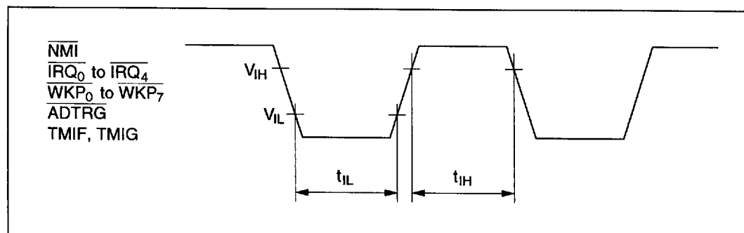
Figure 14-5 Input Timing
