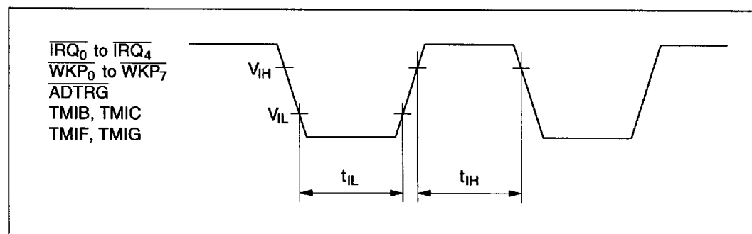
Figure 14-3 Input Timing
