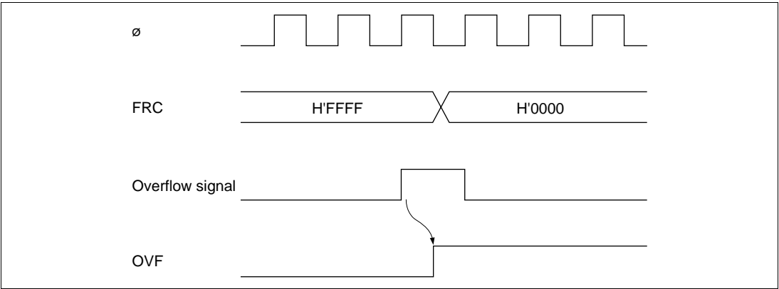
www.DataSheet4u.com Figure 9.30 OVF Set Timing
