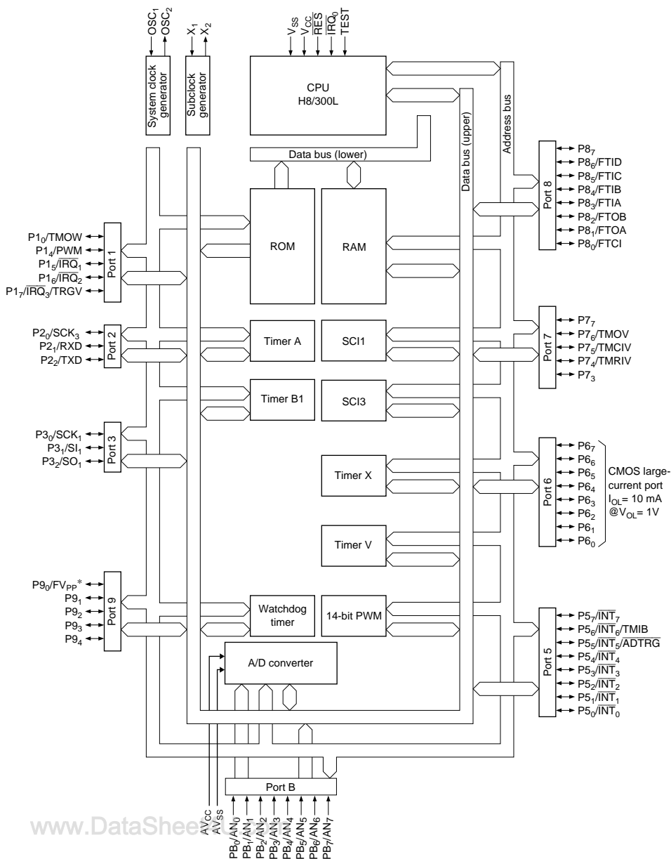
Figure 1.1 Block Diagram
