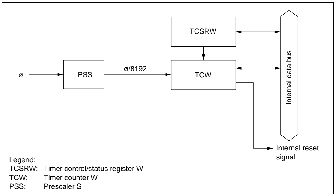
Figure 9.35 Block Diagram of Watchdog Timer
