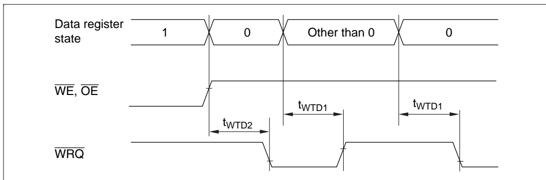
Figure 19.21 \overline{WRQ} Output Timing
