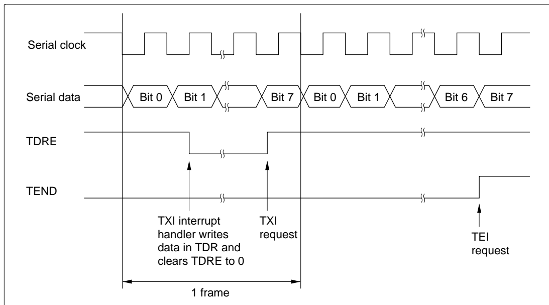
Figure 14.14 Example of SCI Transmit Operation
