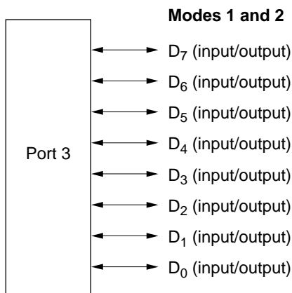
Figure 8.10 Pin Functions in Modes 1 and 2 (Port 3)
