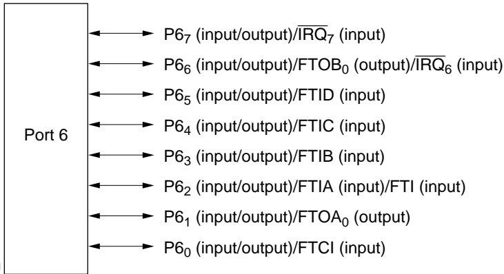
Figure 8.16 Pin Functions in Mode 3 (Port 6)
