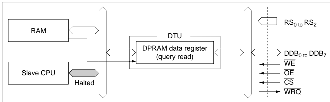
Figure 5.2 Concept of Buffer Queries
