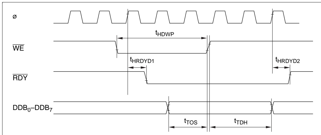
Figure 19.23 Receive Timing in Handshake Mode
