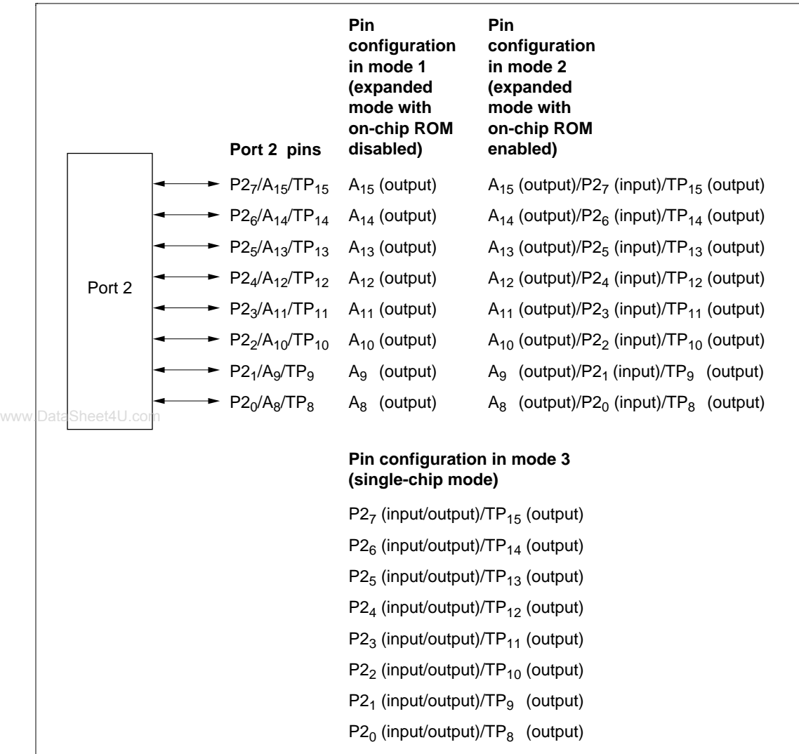
Figure 8.5 Port 2 Pin Configuration
