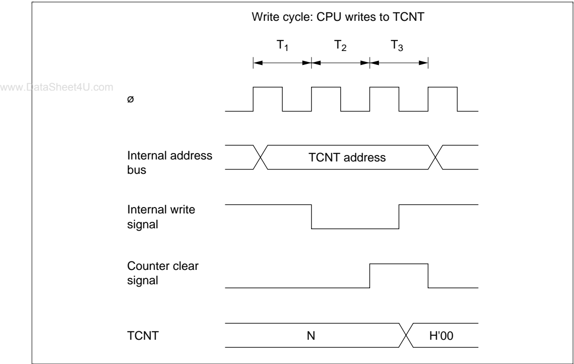
Figure 11.10 TCNT Write-Clear Contention
