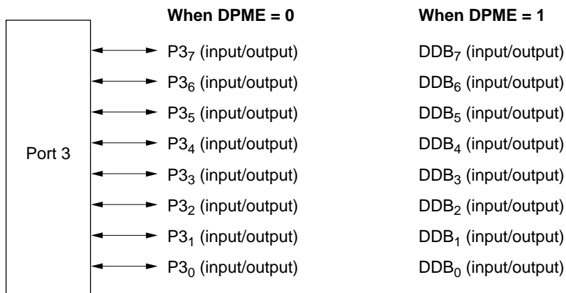
Figure 8.11 Pin Functions in Mode 3 (Port 3)
