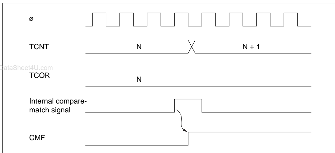
Figure 11.4 Setting of Compare-Match Flags
