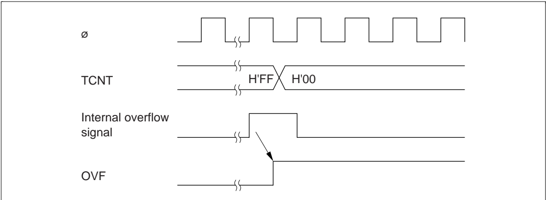
Figure 13.5 Setting the OVF Bit
