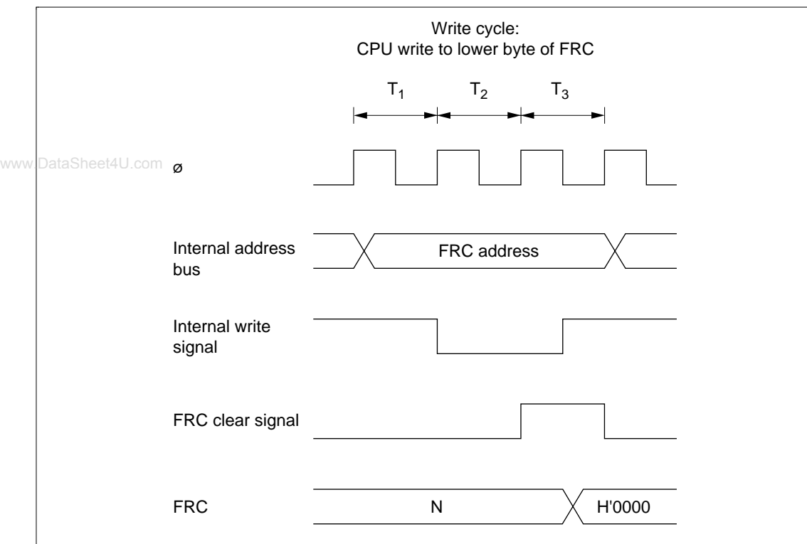
Figure 9.16 FRC Write-Clear Contention
