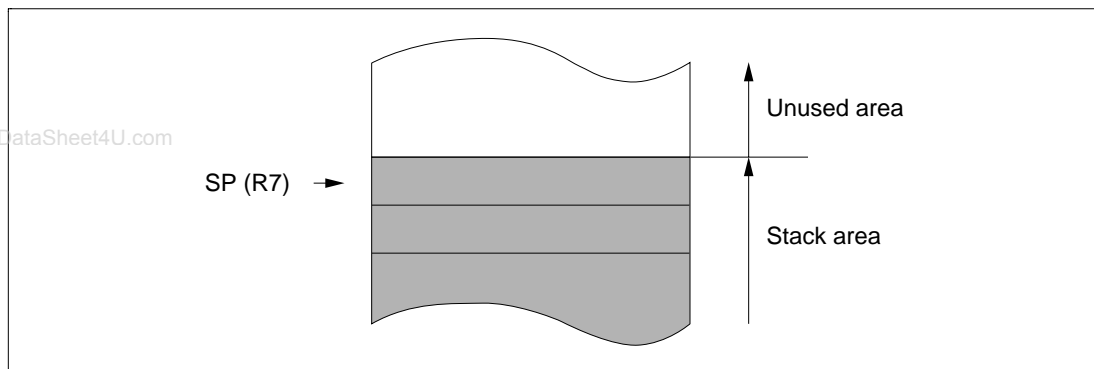
Figure 2.2 Stack Pointer
