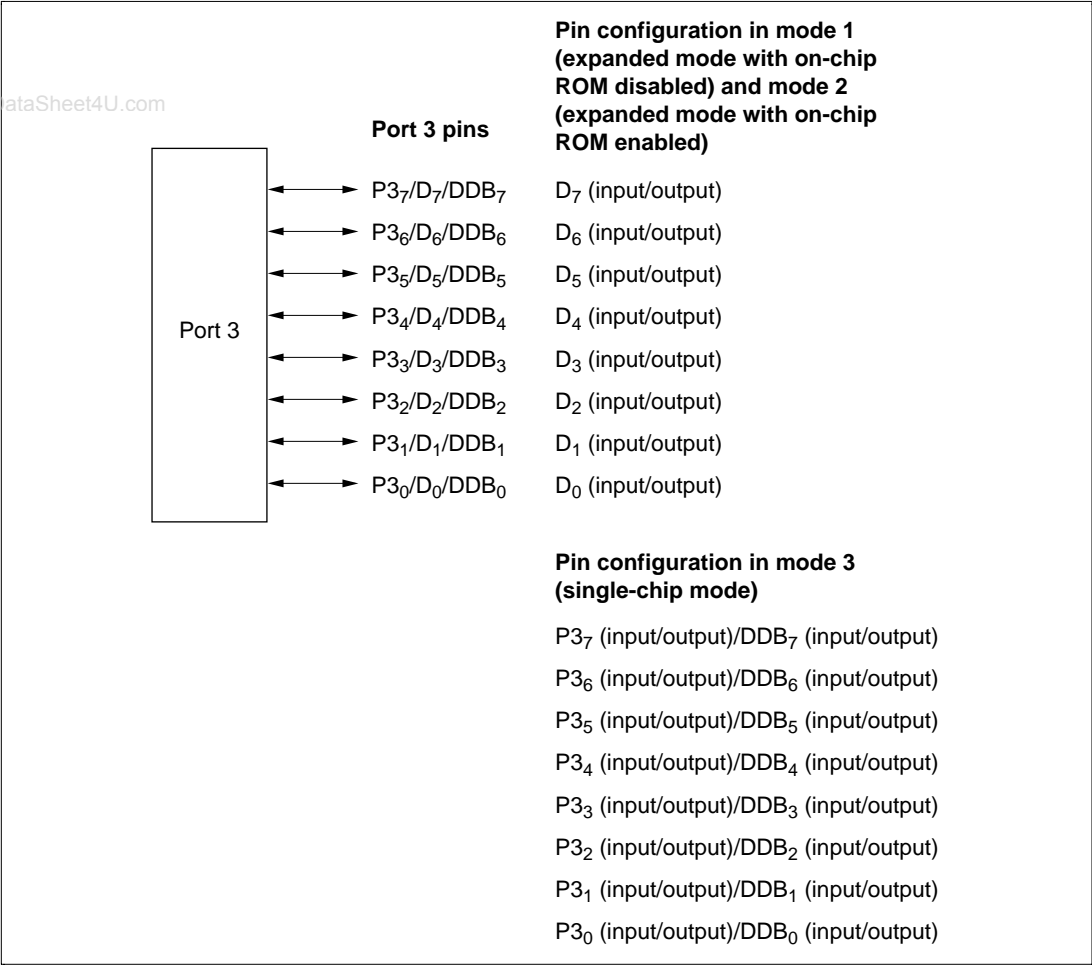
Figure 8.9 Port 3 Pin Configuration www.DataSheet4U.com
