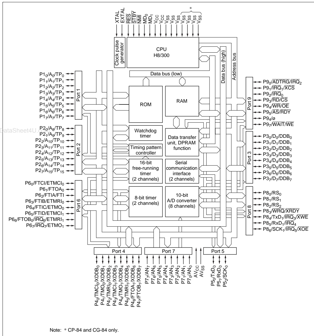
Figure 1.1 Block Diagram
