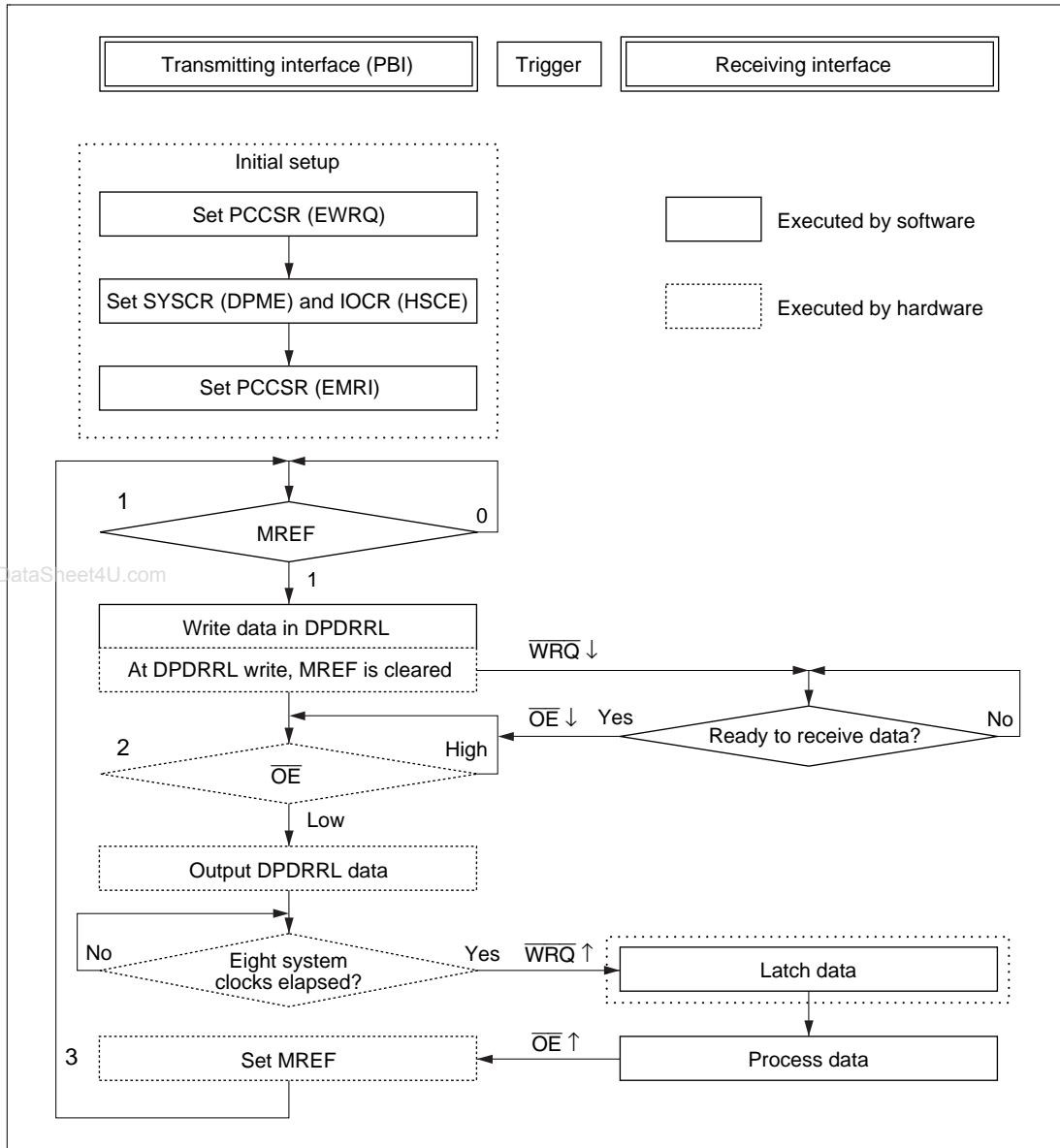
Figure 5.25 Flowchart of Transmit Operations in Handshake Mode
