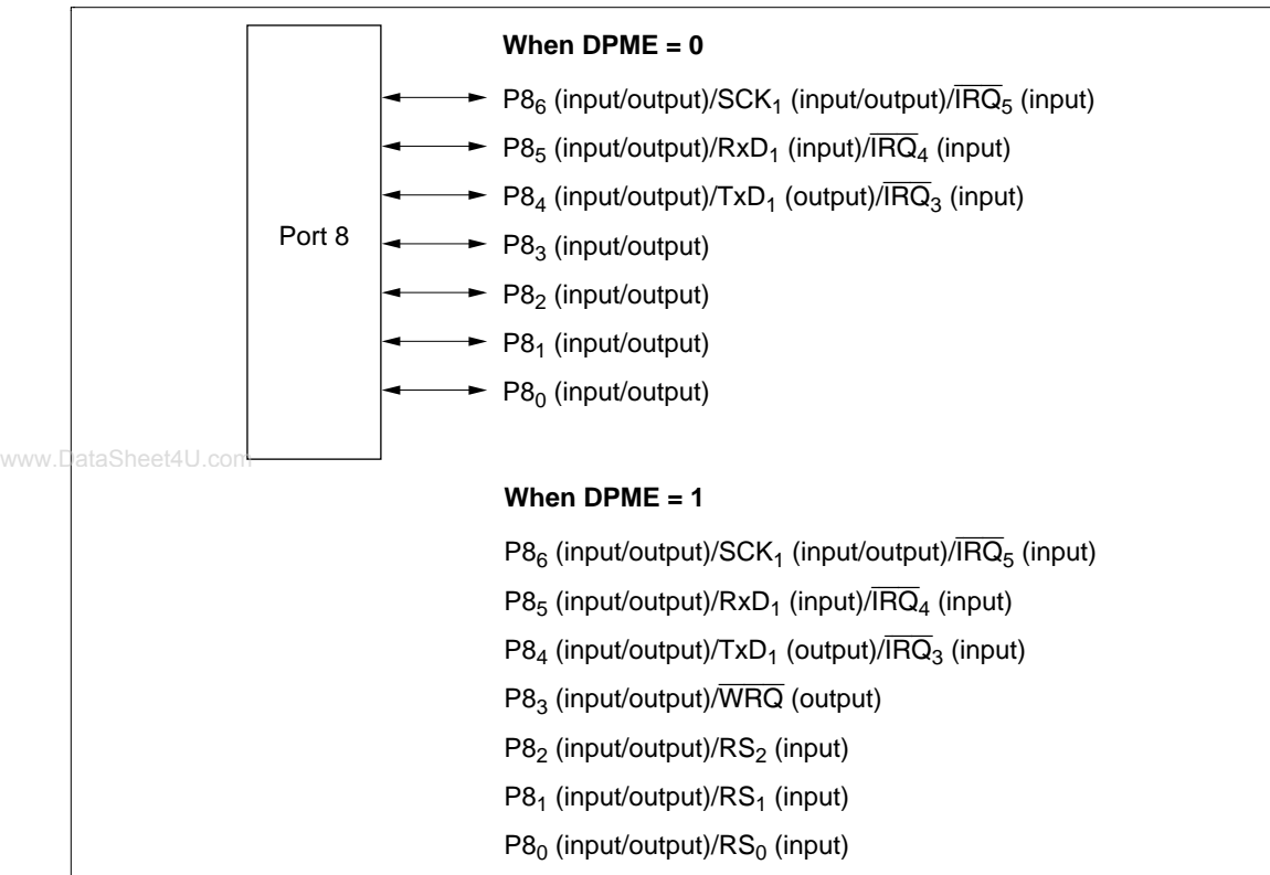
Figure 8.20 Pin Functions in Mode 3 (Port 8)
