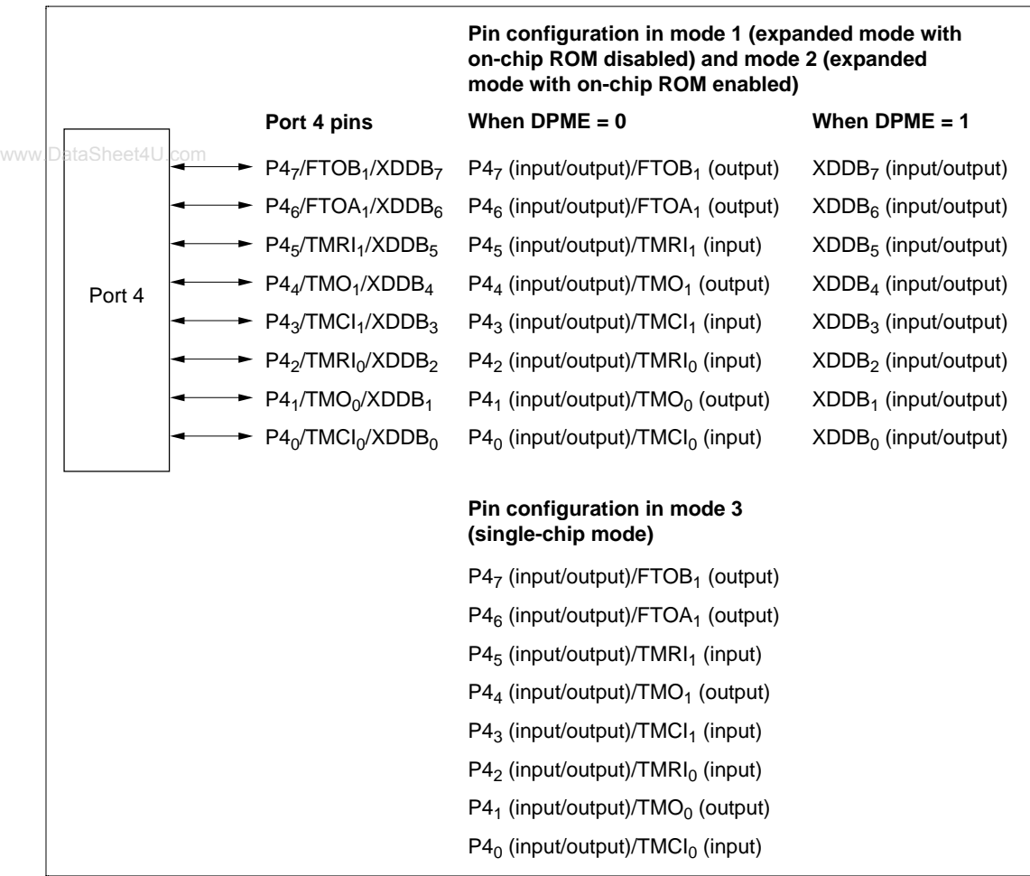
Figure 8.12 Port 4 Pin Configuration
