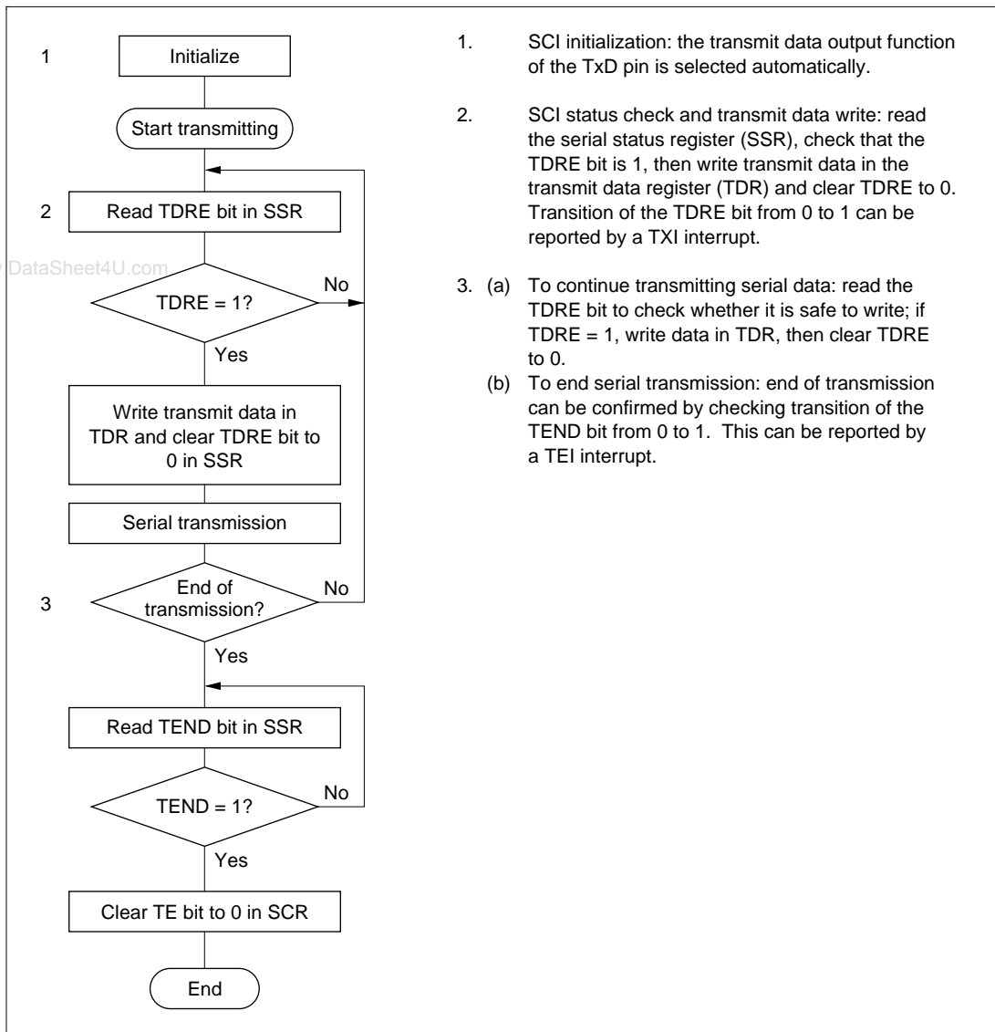
Figure 14.13 Sample Flowchart for Serial Transmitting
