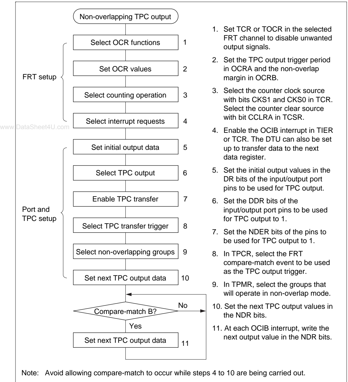
Figure 12.6 Setup Procedure for Non-Overlapping TPC Output (Example)
