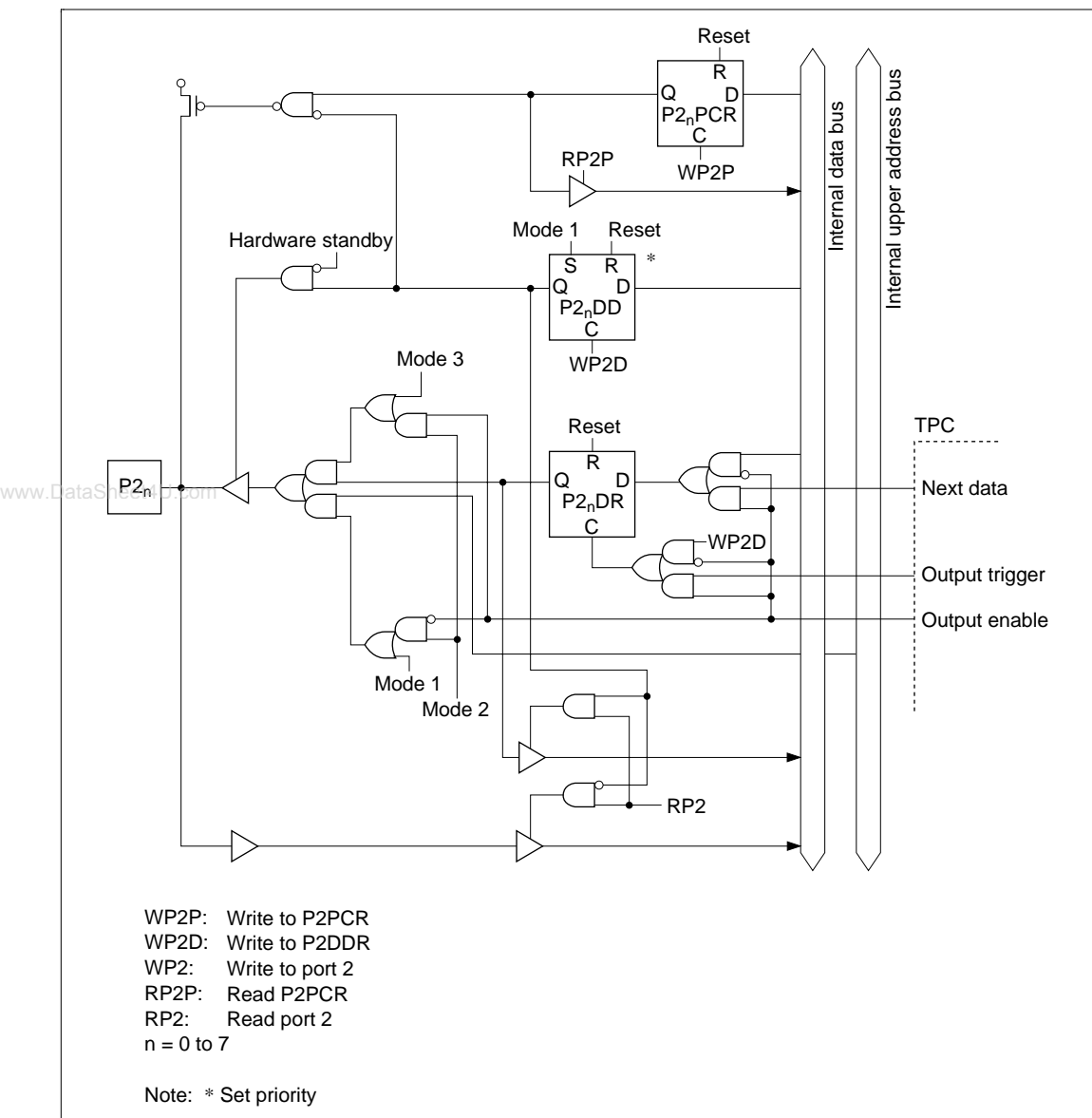
Figure C.2 Port 2 Block Diagram
