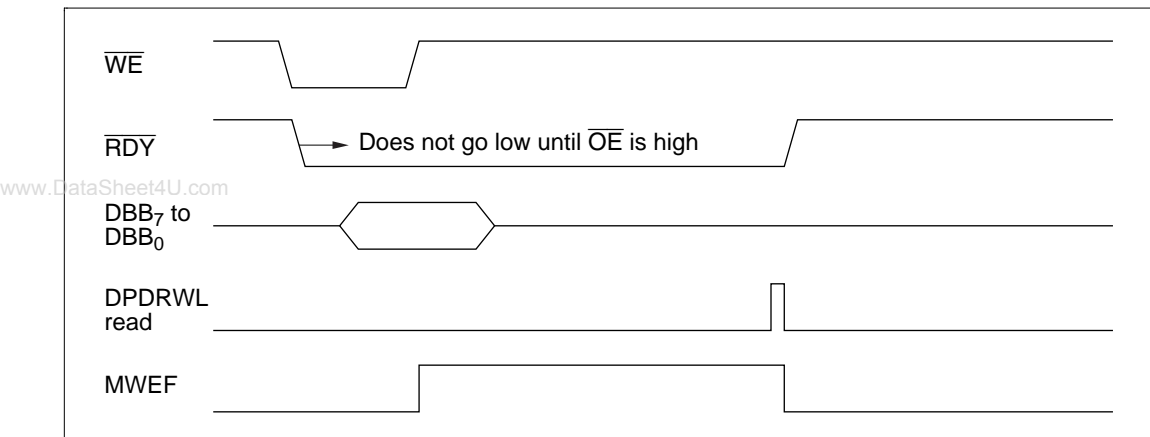
Figure 5.30 Receive Timing in Handshake Mode
