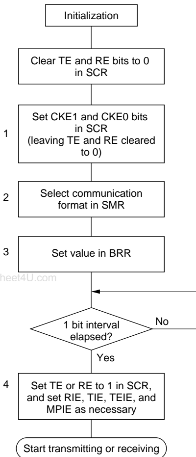
Figure 14.4 Sample Flowchart for SCI Initialization
