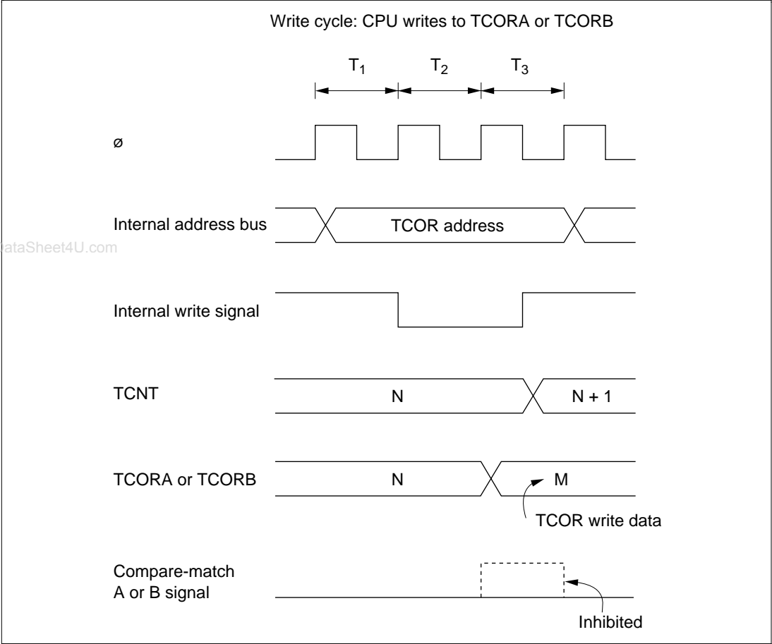
Figure 11.12 Contention between TCOR Write and Compare-Match
