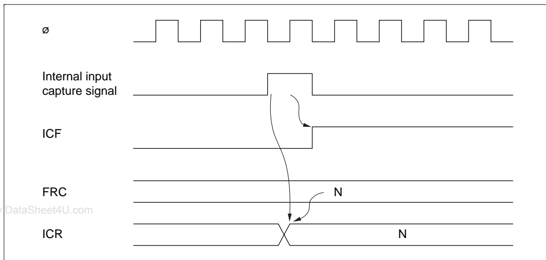
Figure 9.12 Setting of Input Capture Flag
