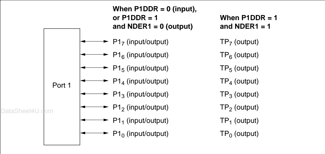
Figure 8.4 Pin Functions in Mode 3 (Port 1)
