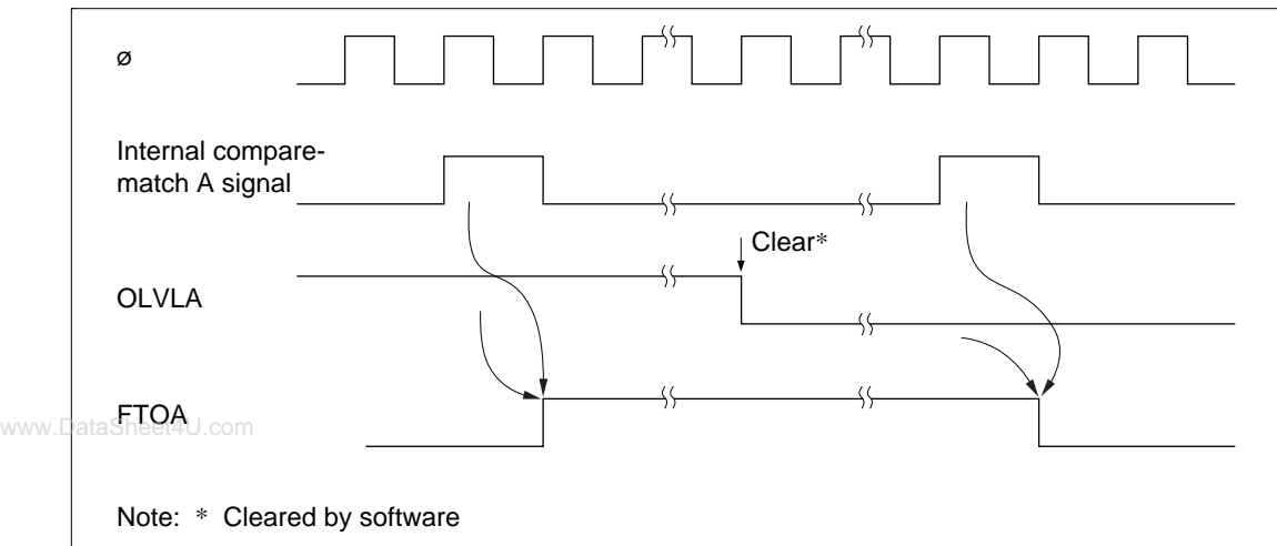
Figure 10.5 Timing of Output Compare A
