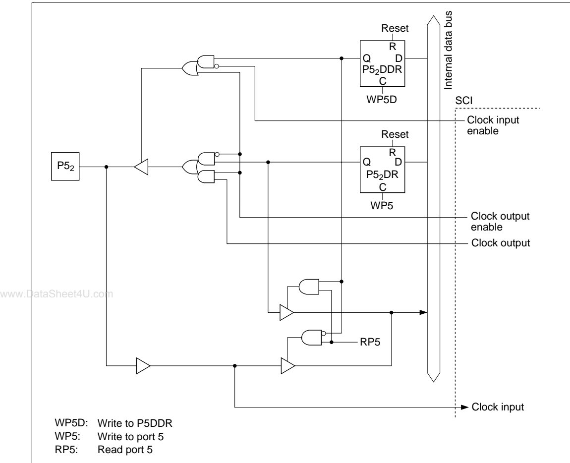
Figure C.5 (c) Port 5 Block Diagram (Pin P5 2 )
