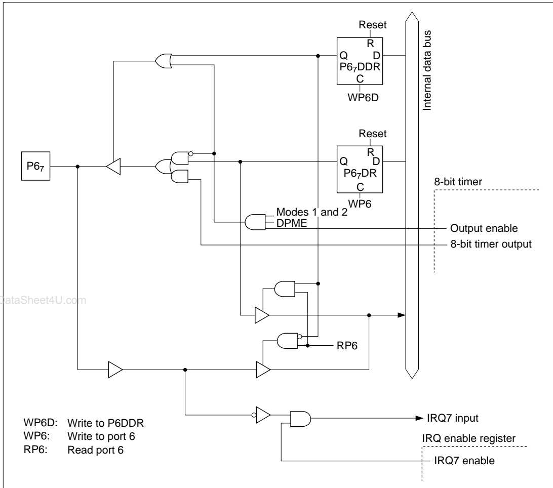
Figure C.6 (f) Port 6 Block Diagram (Pin P6 7 )
