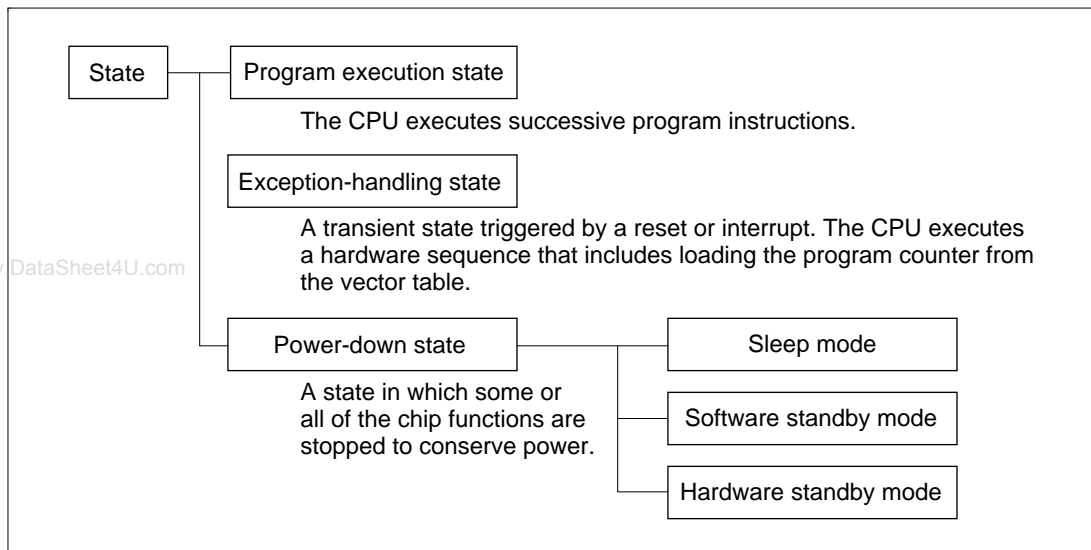
Figure 2.11 Operating States
