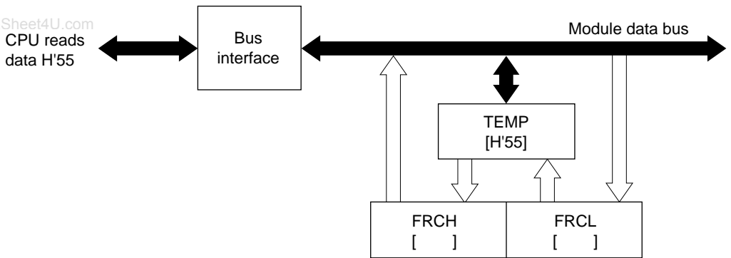
Figure 9.3b Read Access to FRC (when FRC Contains H'AA55)
