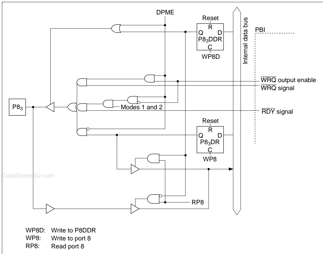
Figure C.8 (b) Port 8 Block Diagram (Pin P8 3 )
