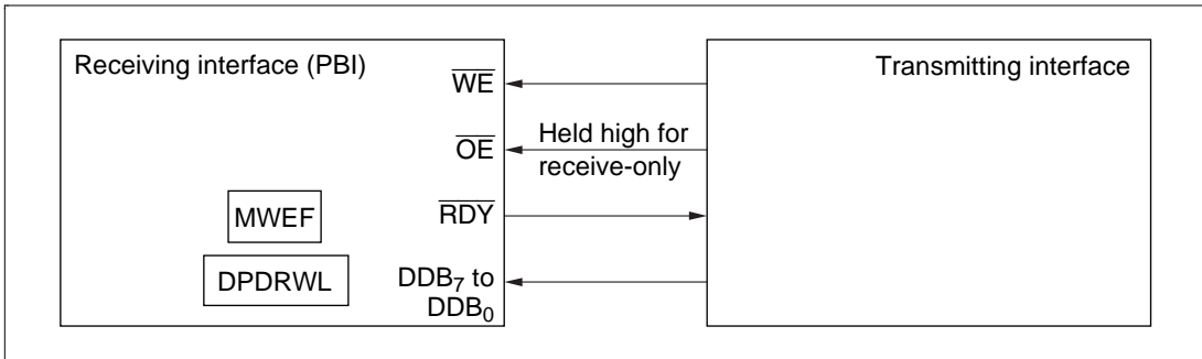
Figure 5.29 Receiving in Handshake Mode
