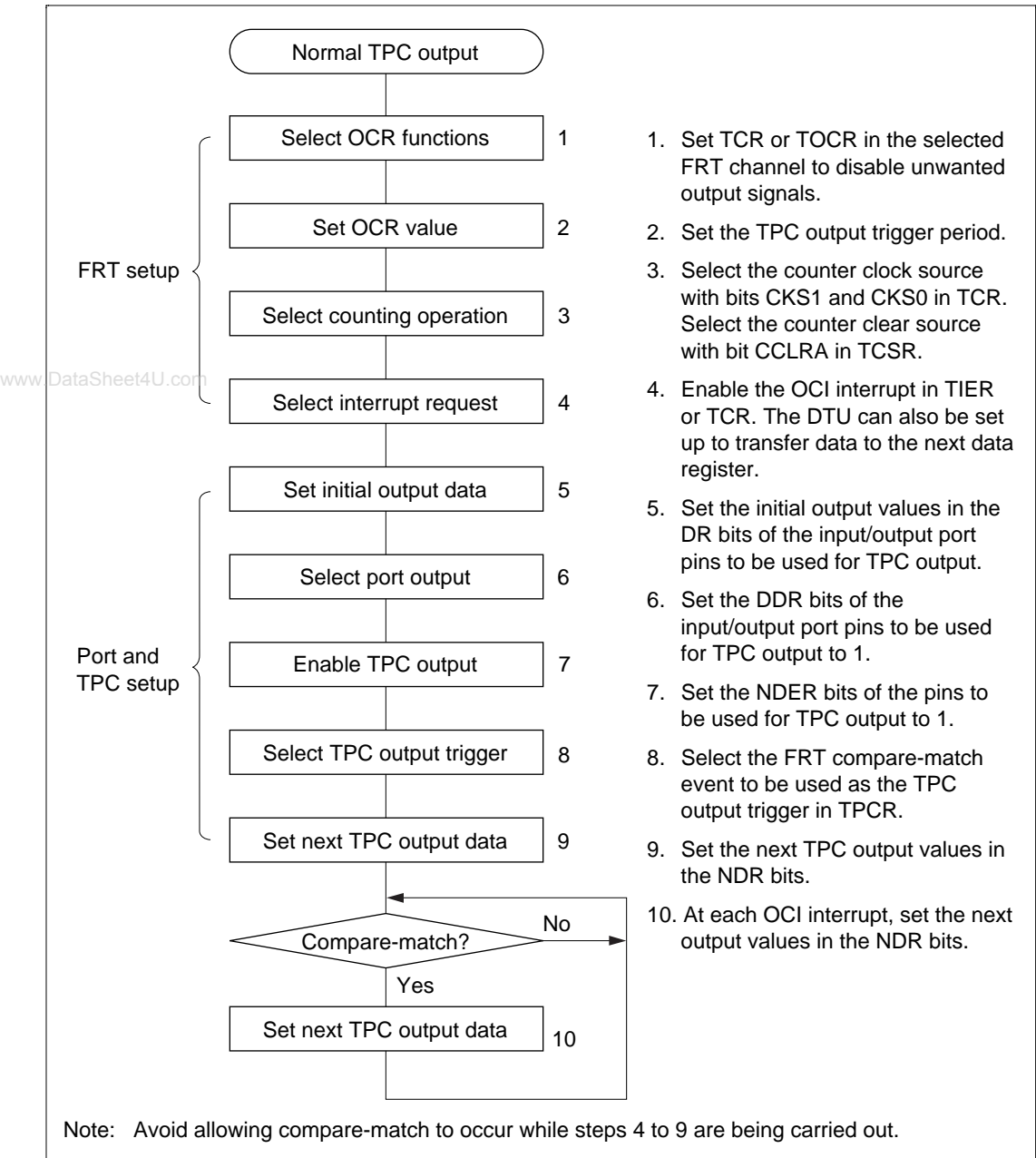
Figure 12.4 Setup Procedure for Normal TPC Output (Example)
