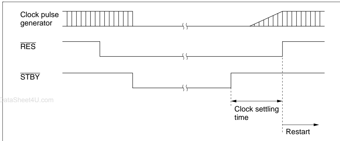
Figure 18.2 Hardware Standby Mode Timing
