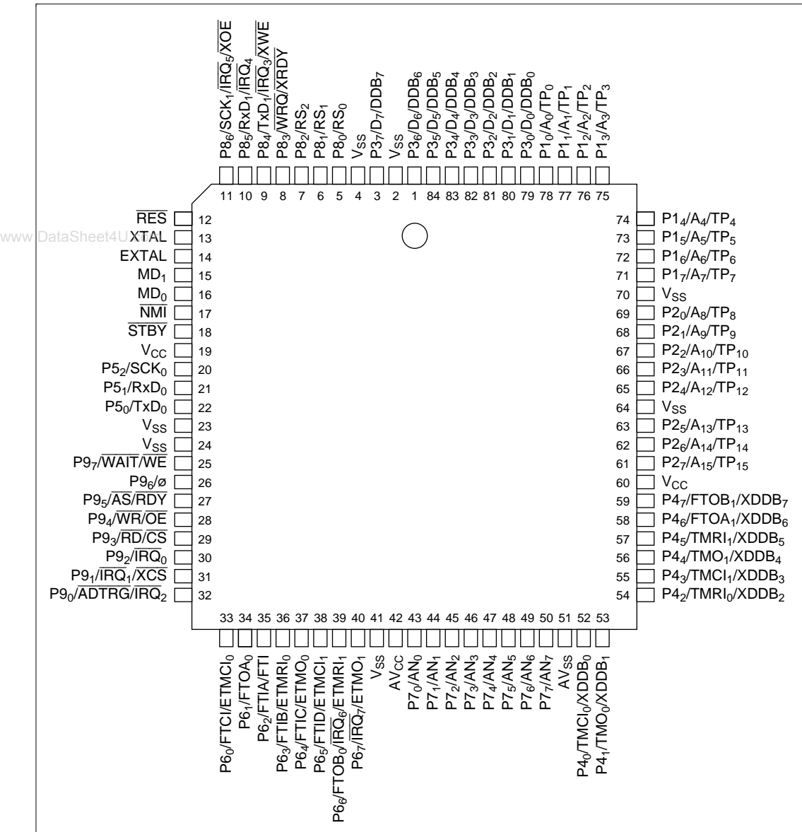
Figure 1.2 Pin Arrangement (CP-84 and CG-84, Top View)
