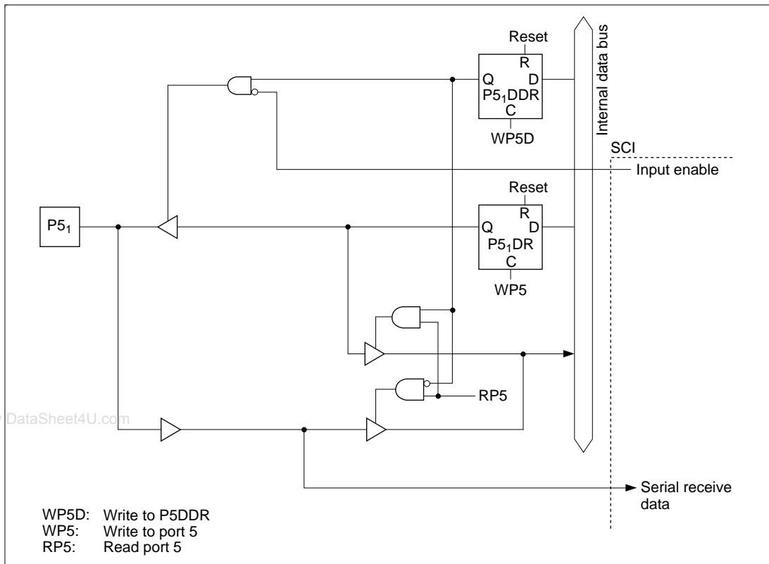
Figure C.5 (b) Port 5 Block Diagram (Pin P5 1 )
