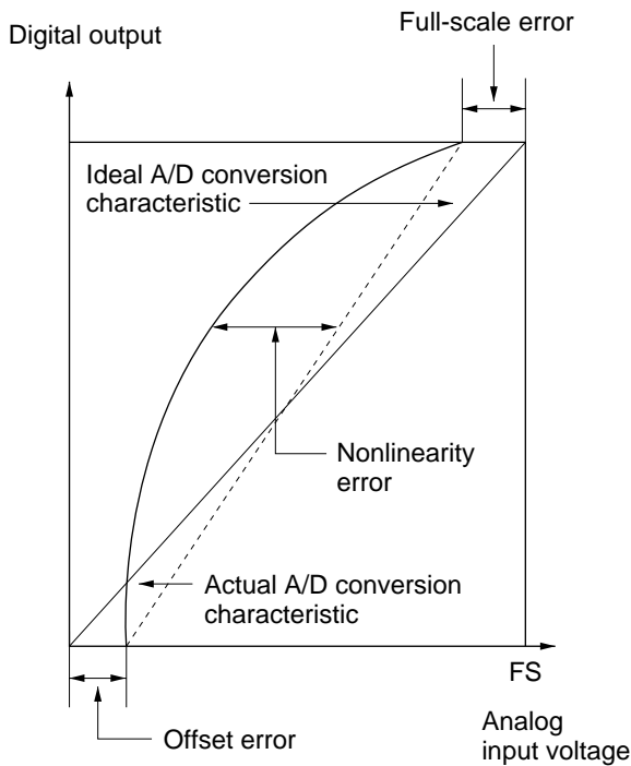
Figure 15.9 A/D Conversion Precision Definitions (2)
