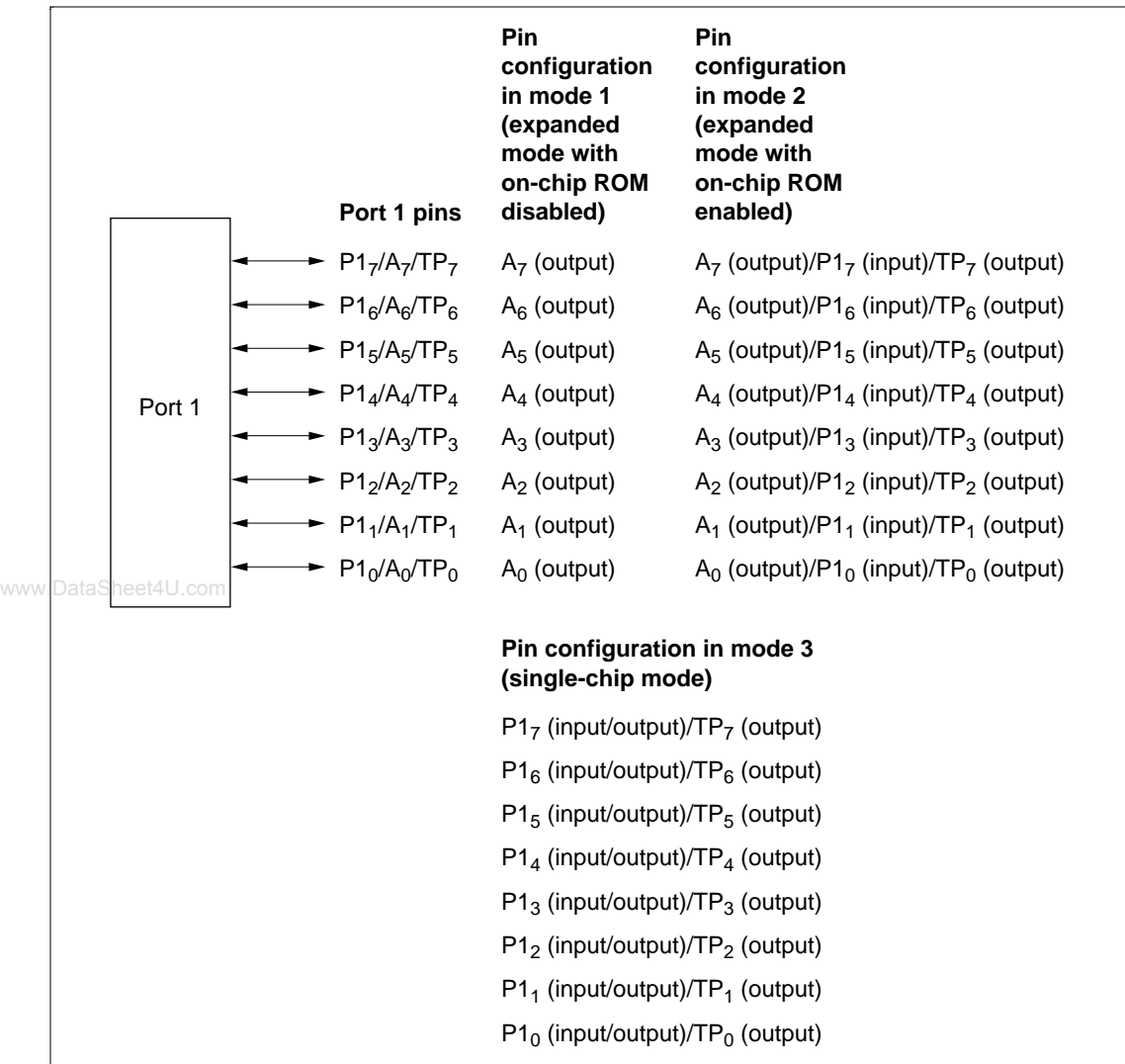
Figure 8.1 Port 1 Pin Configuration
