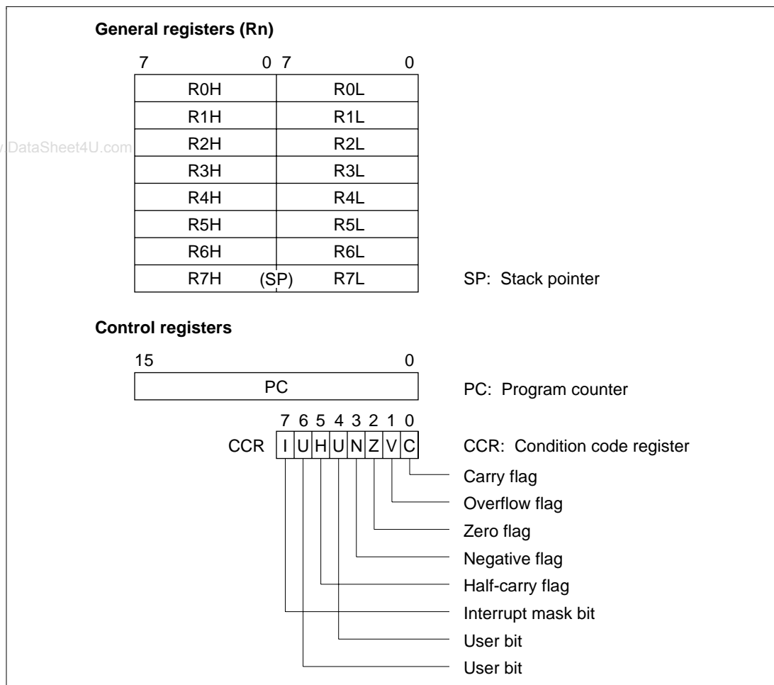
Figure 2.1 CPU Registers
