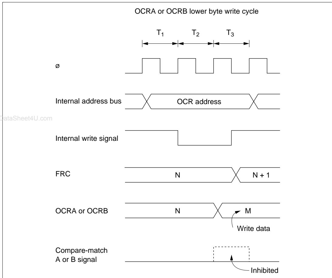
Figure 10.14 Contention between OCR Write and Compare-Match
