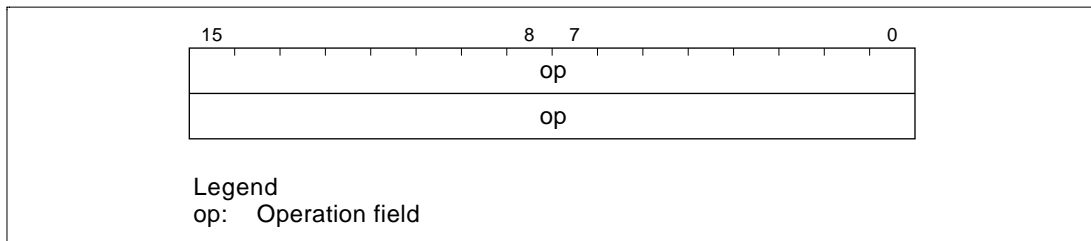
Instruction Size Function EEPMOV — if R4L \neq 0 then repeat @R5+ \rightarrow @R6+ R4L - 1 \rightarrow R4L until R4L = 0 else next; Moves a data block according to parameters set in general registers R4L, R5, and R6. R4L: size of block (bytes) R5: starting source address R6: starting destination address Execution of the next instruction starts as soon as the block transfer is completed.
