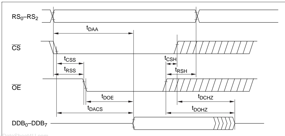
Figure 19.20 DPRAM Read Timing
