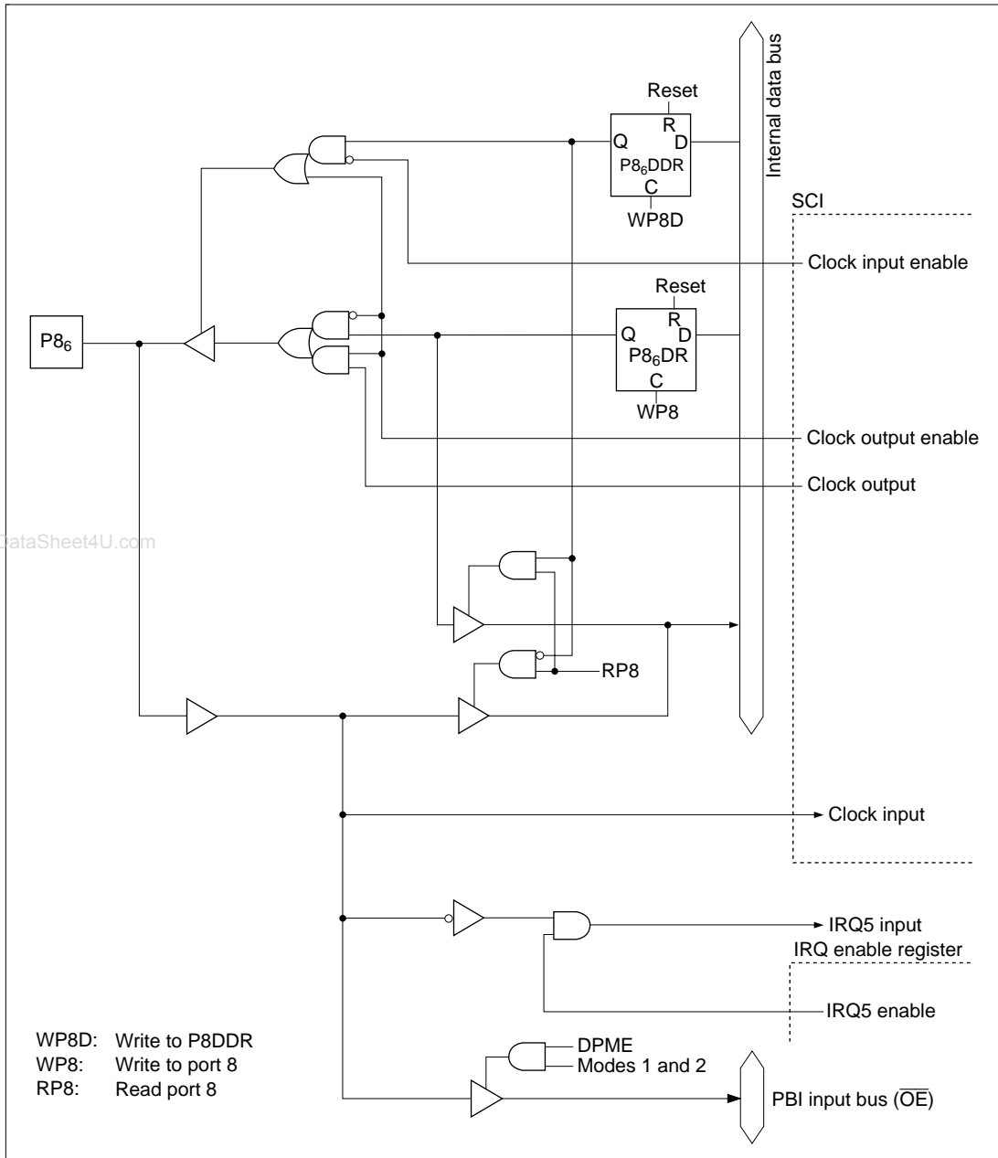
Figure C.8 (e) Port 8 Block Diagram (Pin P8 6 )
