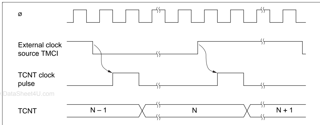
Figure 11.3 Count Timing for External Clock Input
