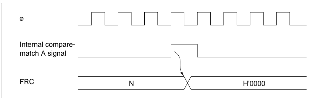
Figure 10.6 Clearing of FRC by Compare-Match A
