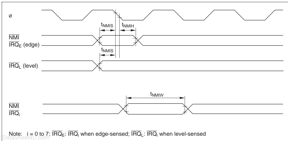
Figure 19.7 Interrupt Input Timing
