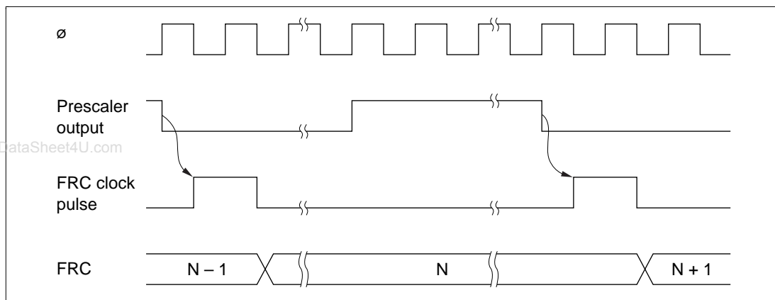
Figure 10.3 Increment Timing for Internal Clock Source
