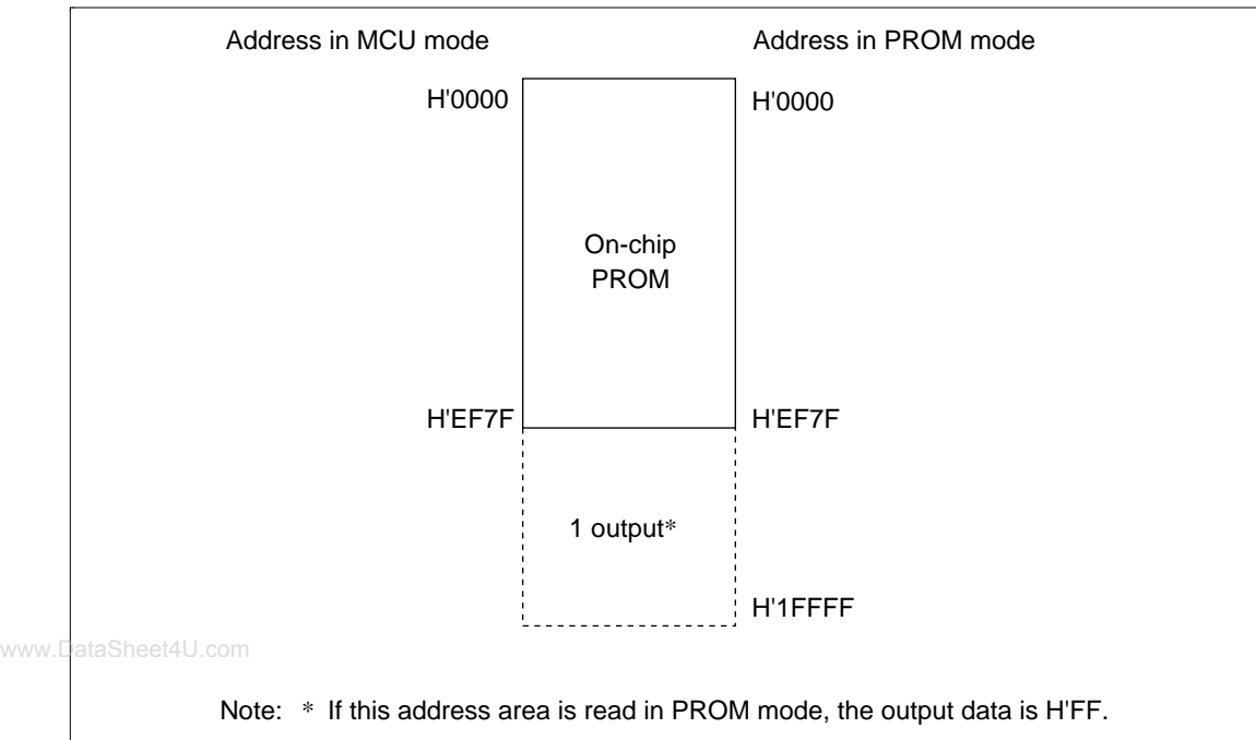
Figure 17.3 H8/3318 Memory Map in PROM Mode
