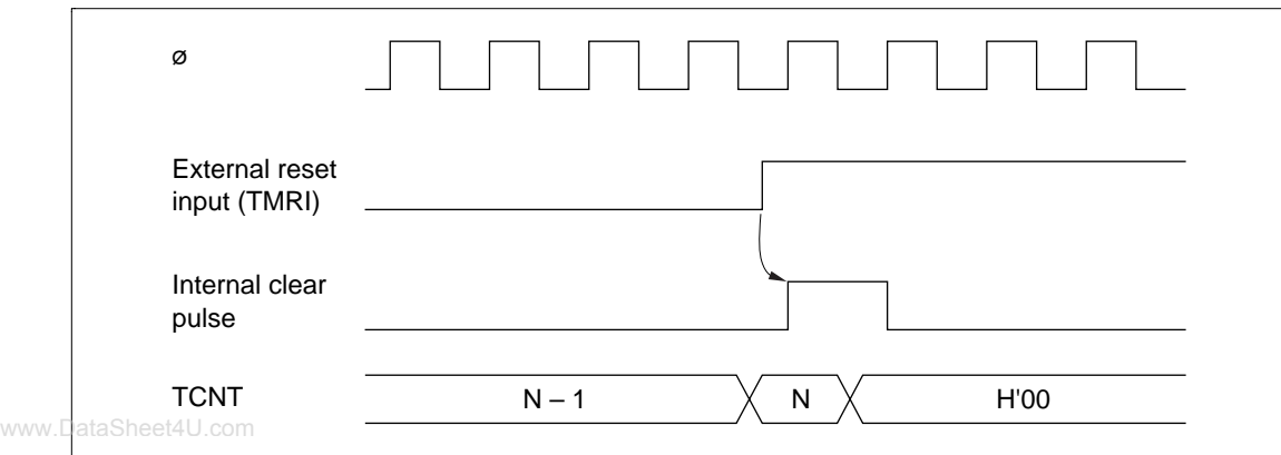
Figure 11.7 Timing of External Reset
