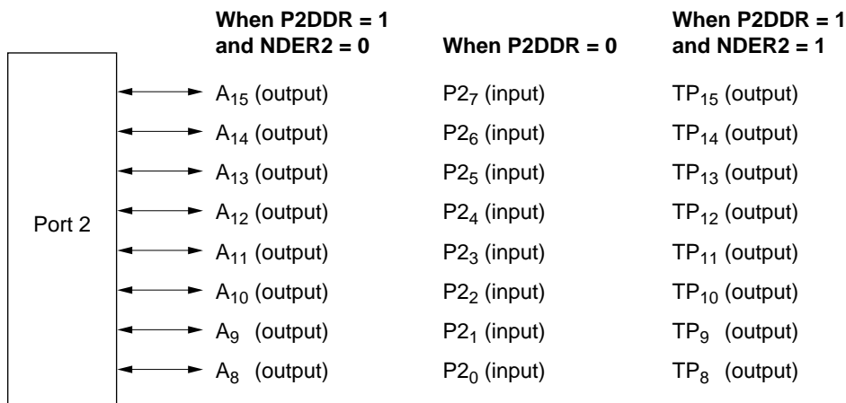
Figure 8.7 Pin Functions in Mode 2 (Port 2)
