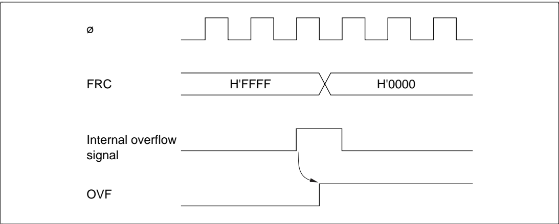
Figure 10.10 Setting of Overflow Flag (OVF)
