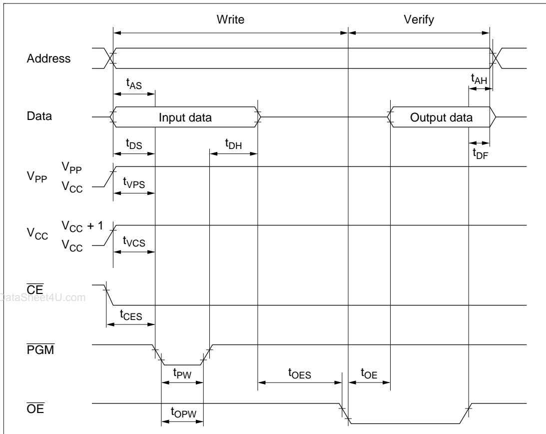
Figure 17.5 PROM Program/Verify Timing
