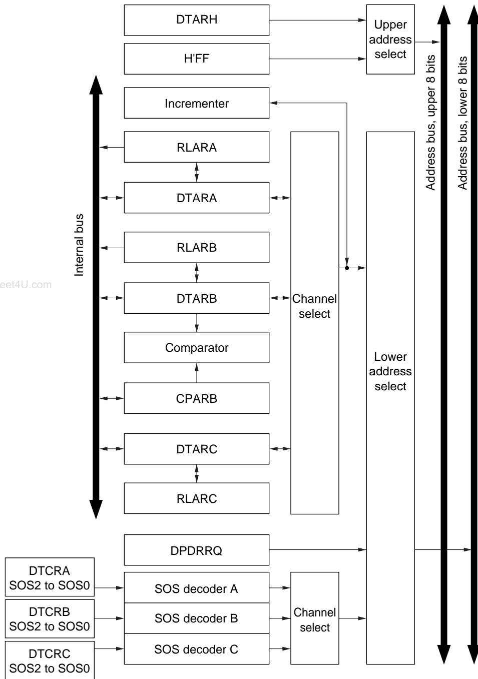
Figure 5.8 Concept of Address Bus Circuits
