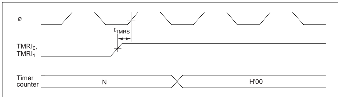
Figure 19.14 8-Bit Timer Reset Input Timing
