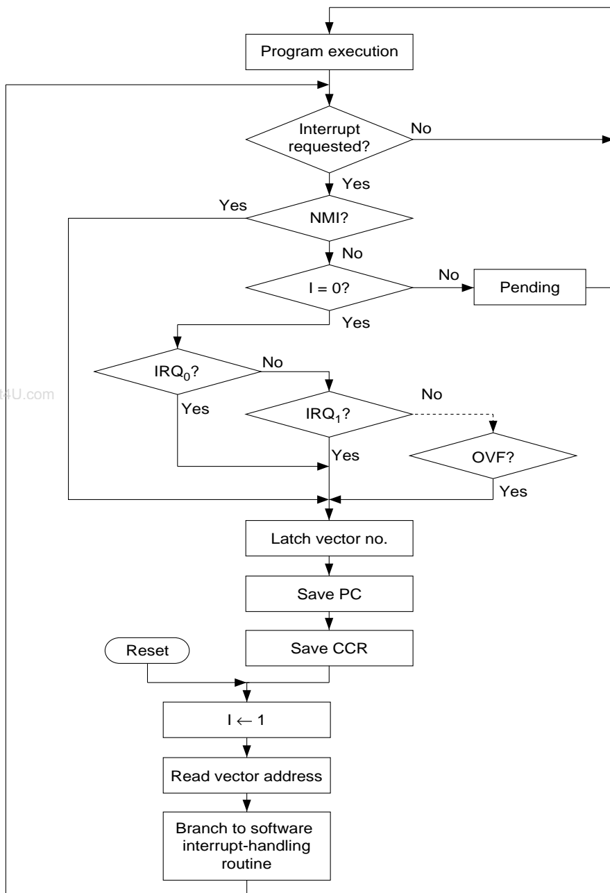
Figure 4.4 Hardware Interrupt-Handling Sequence
