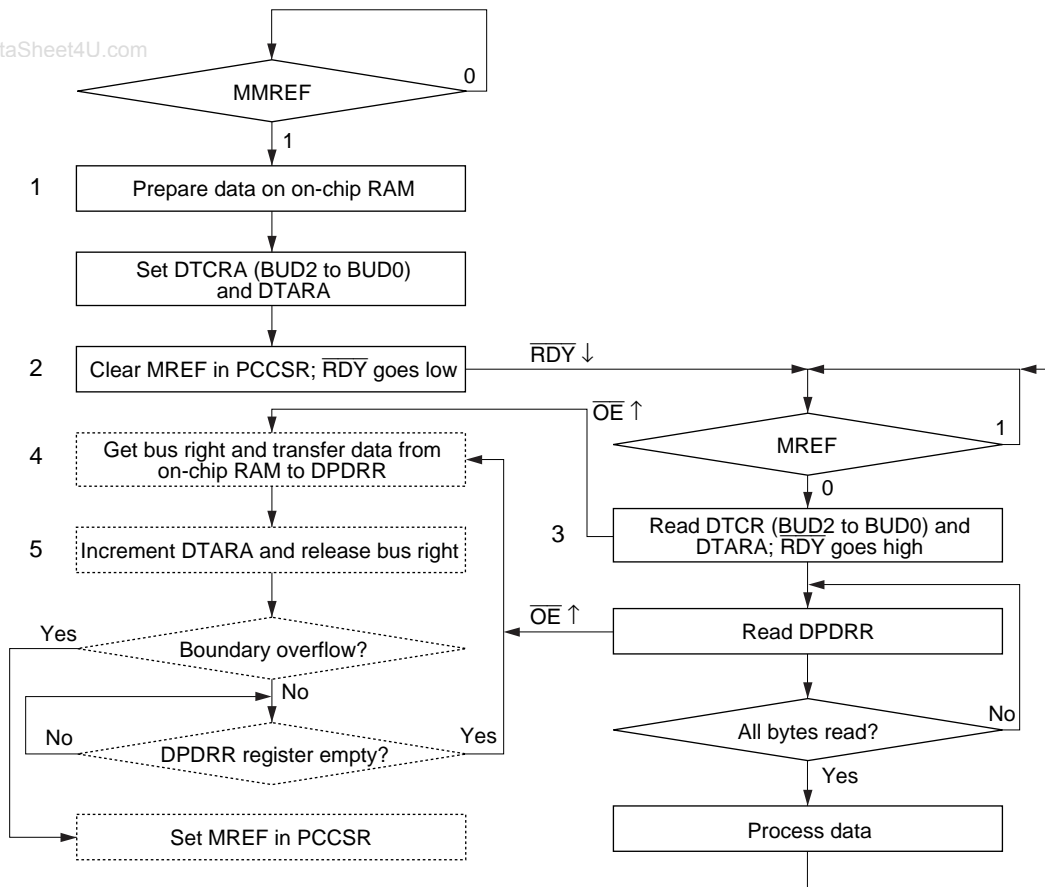
Figure 5.17 Flowchart of Read Operations in DPRAM Boundary Mode
