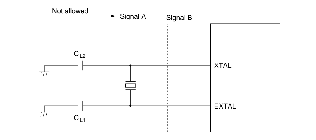
Figure 7.4 Notes on Board Design around External Crystal
