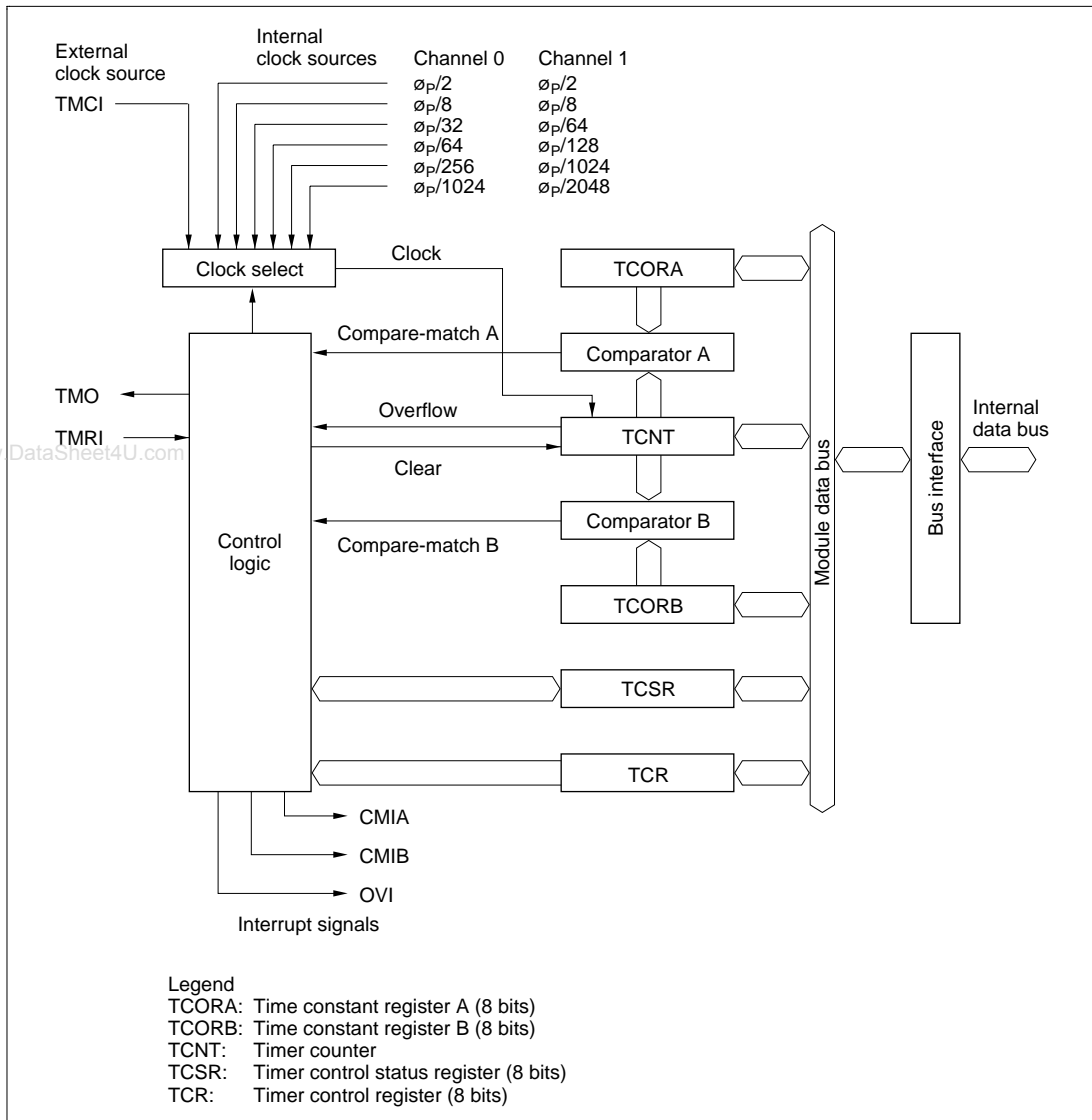
Figure 11.1 Block Diagram of 8-Bit Timer (1 Channel)
