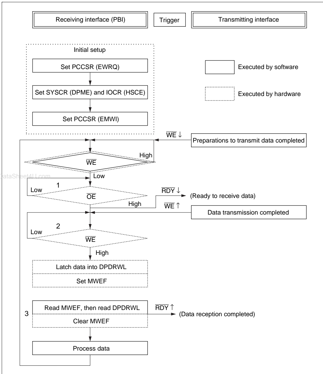
Figure 5.26 Flowchart of Receive Operations in Handshake Mode
