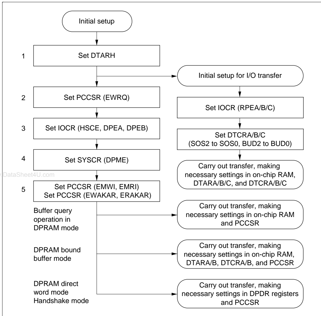
Figure 5.12 DTU and PBI Initialization Flowchart
