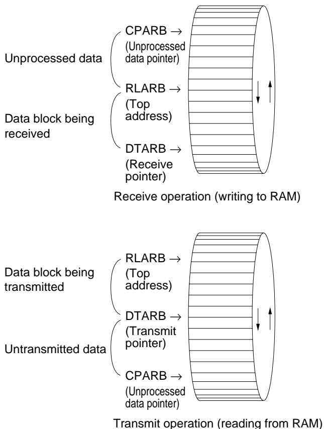
Figure 5.11 Pointer Operation in Ring Buffer
