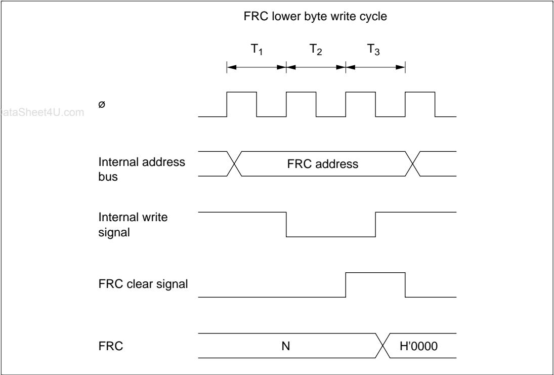
Figure 10.12 FRC Write-Clear Contention
