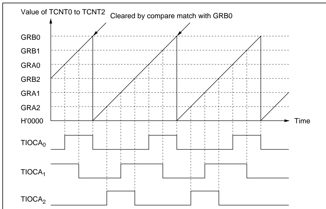
Figure 8.27 Synchronization (Example)
