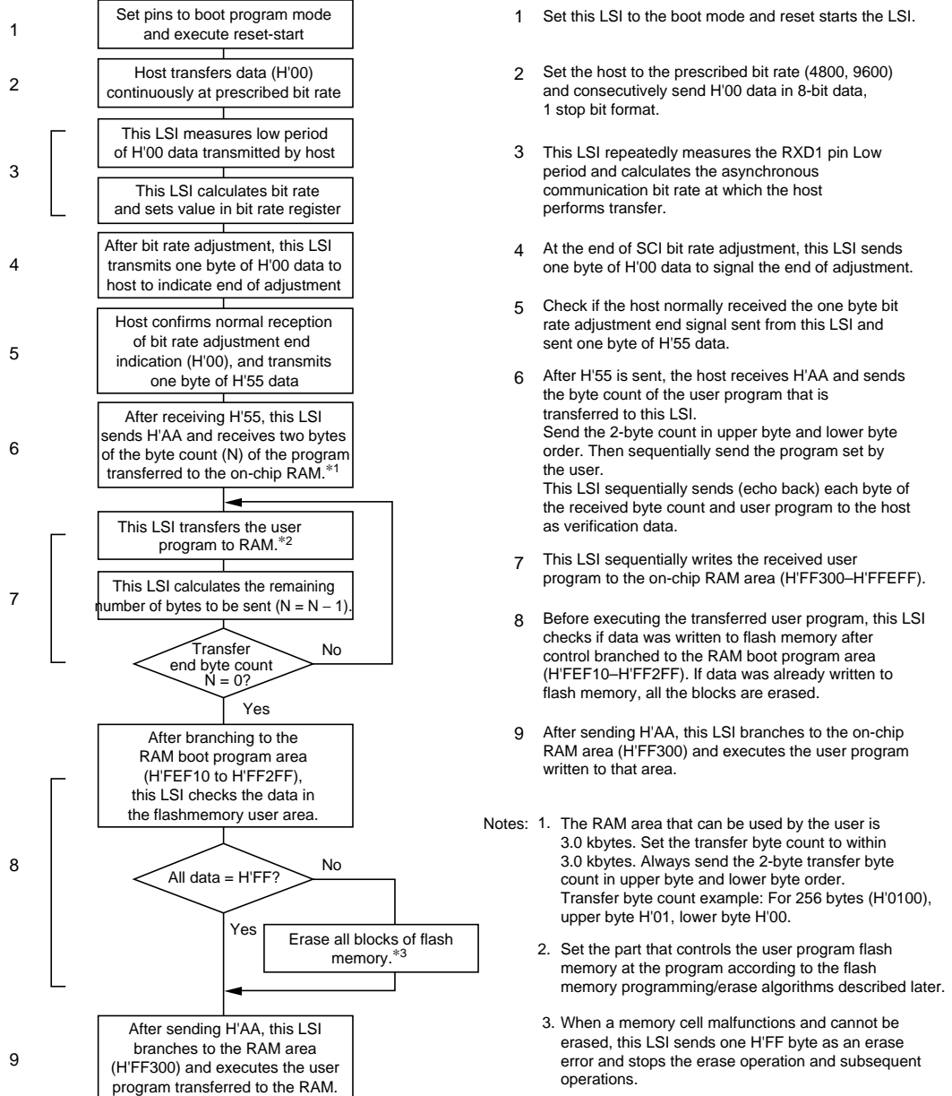
Figure 15.6 Boot Mode Execution Procedure
