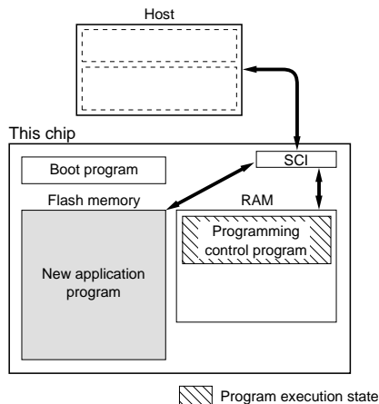
Figure 15.3 Boot Mode
