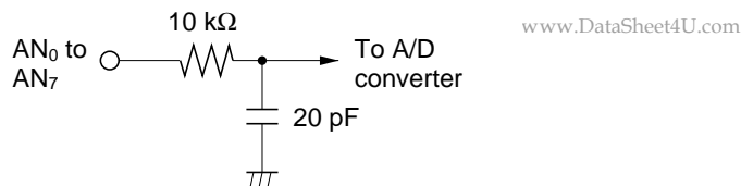
Figure 13.8 Analog Input Pin Equivalent Circuit
