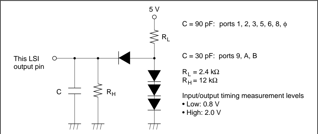
Figure 18.3 Output Load Circuit
