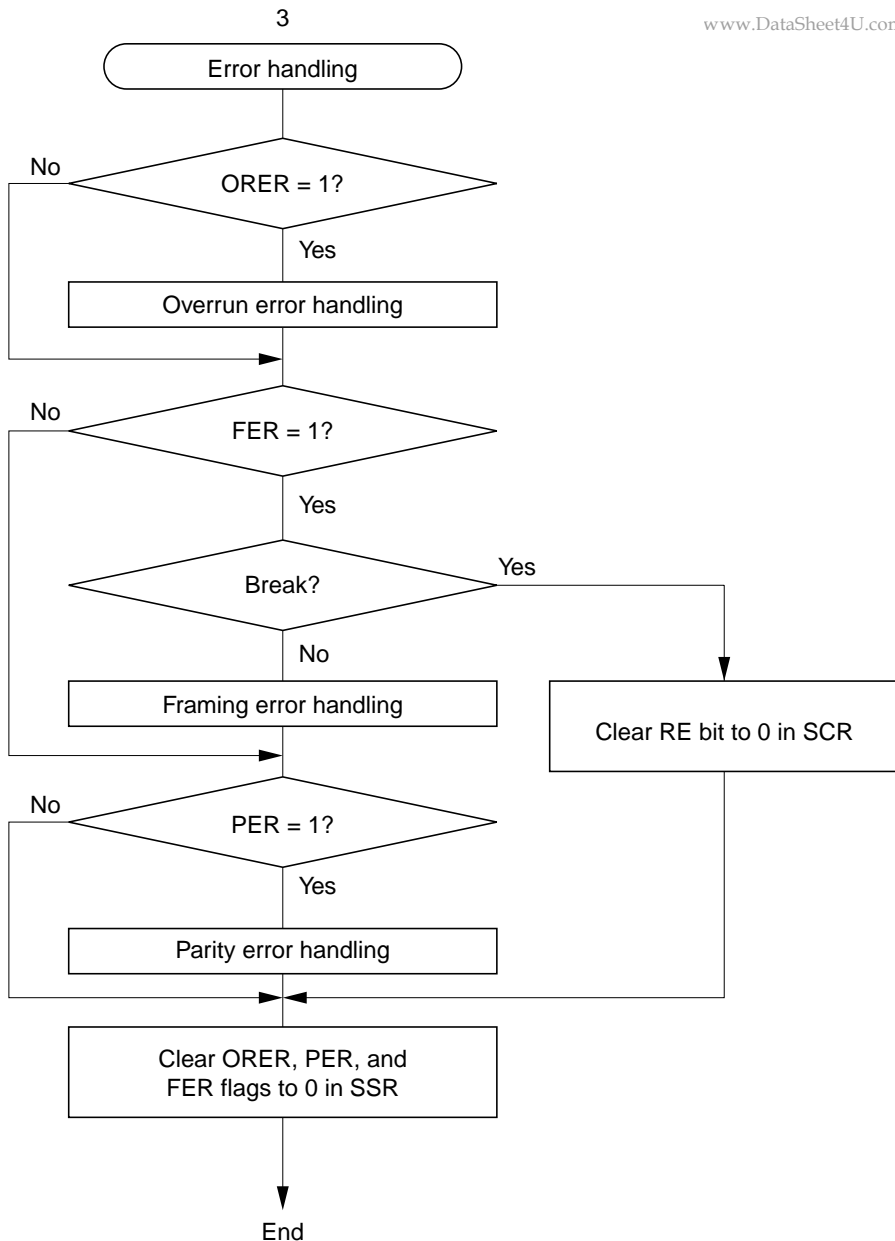
Figure 11.7 Sample Flowchart for Receiving Serial Data (2)
