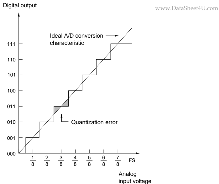
Figure 13.9 A/D Conversion Precision Definitions (1)
