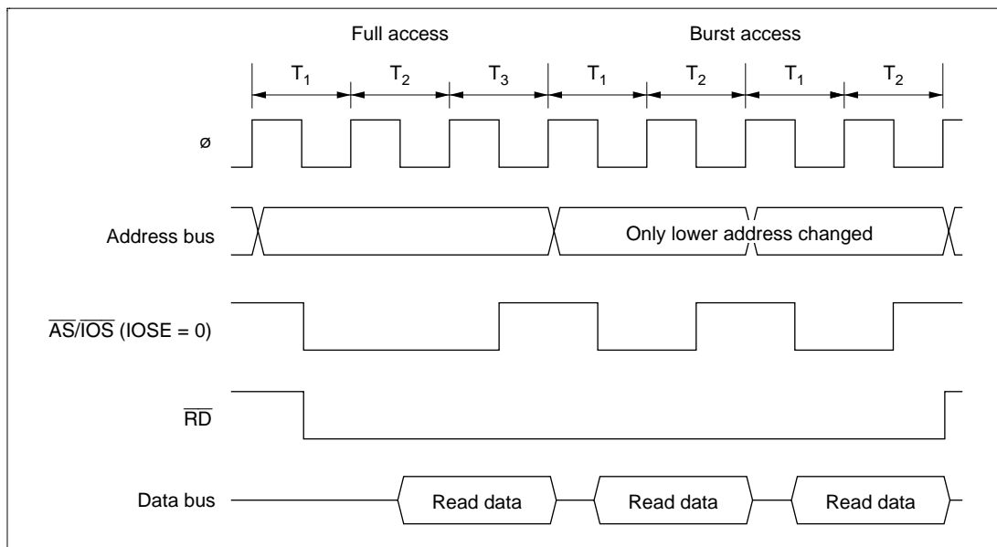
Figure 6.8 (a) Example of Burst ROM Access Timing (When AST and BRSTS1 are both set to 1)
