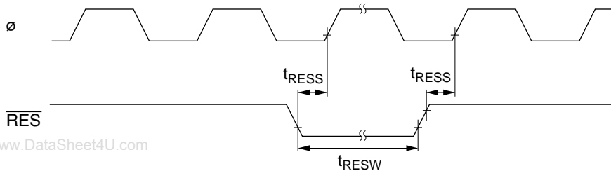
Figure 22.7 Reset Input Timing
