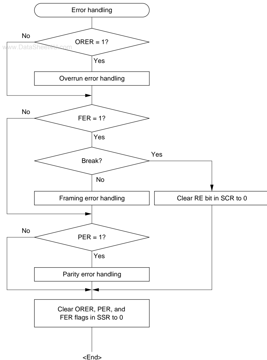
Figure 15.7 Sample Serial Reception Data Flowchart (cont)
