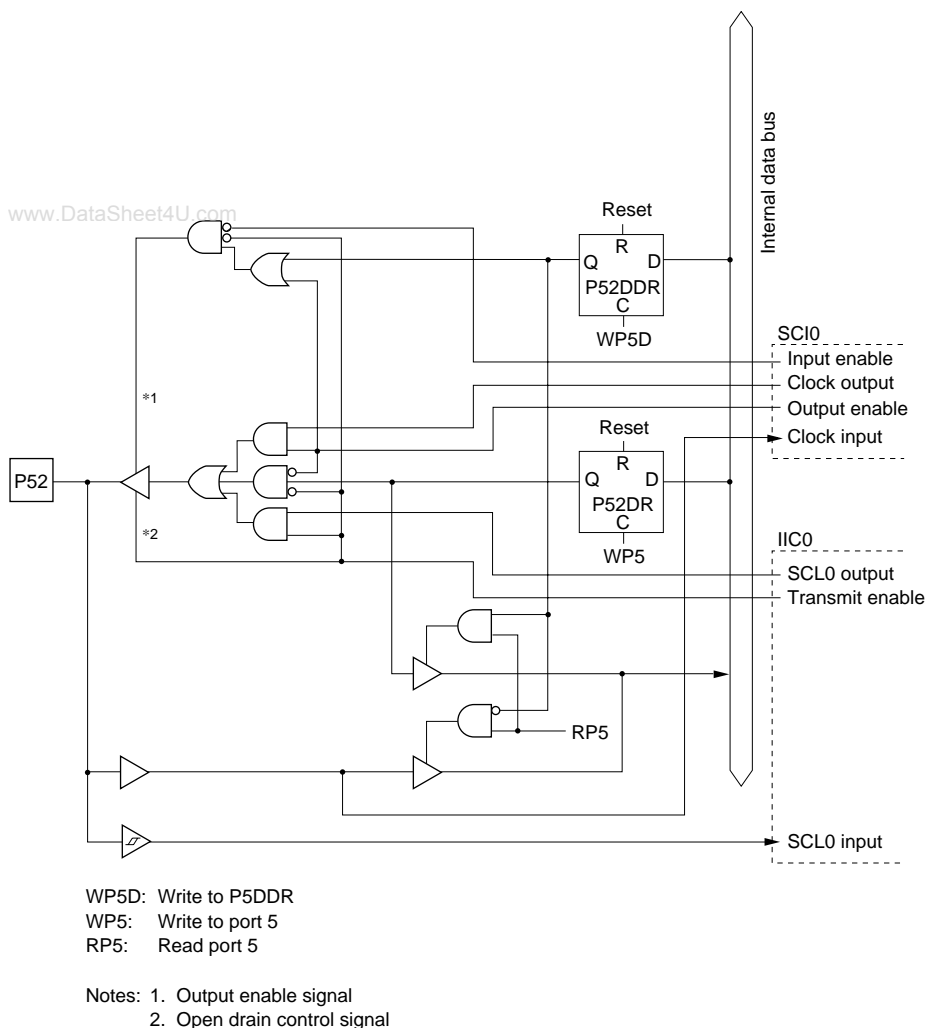
Figure C.17 Port 5 Block Diagram (Pin P52)
