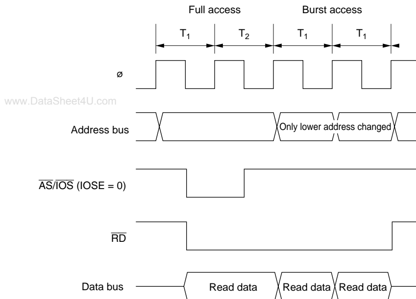
Figure 6.8 (b) Example of Burst ROM Access Timing (When AST = BRSTS1 = 0)
