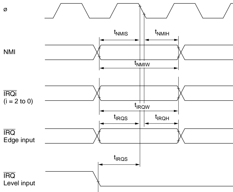
Figure 22.8 Interrupt Input Timing
