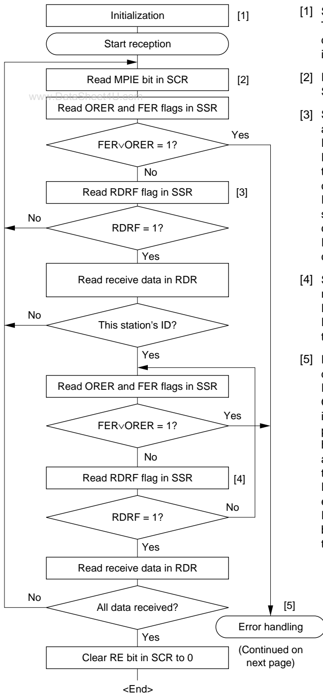
Figure 15.12 Sample Multiprocessor Serial Reception Flowchart www.DataSheet4U.com
