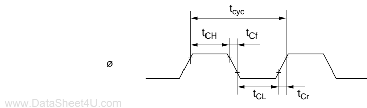
Figure 22.4 System Clock Timing
