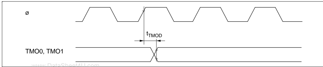
Figure 23.17 8-Bit Timer Output Timing
