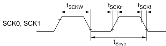
www.DataSheet4U.com Figure 22.21 SCK Clock Input Timing
