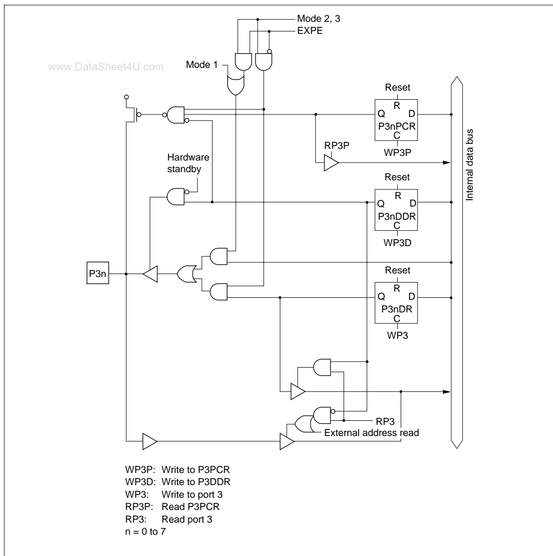
Figure C.9 Port 3 Block Diagram
