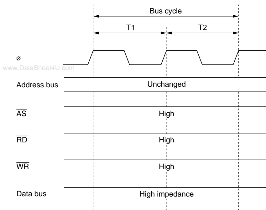
Figure 2.20 Pin States during On-Chip Supporting Module Access
