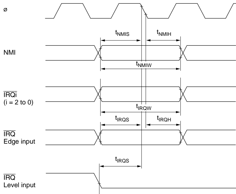
Figure 23.8 Interrupt Input Timing
