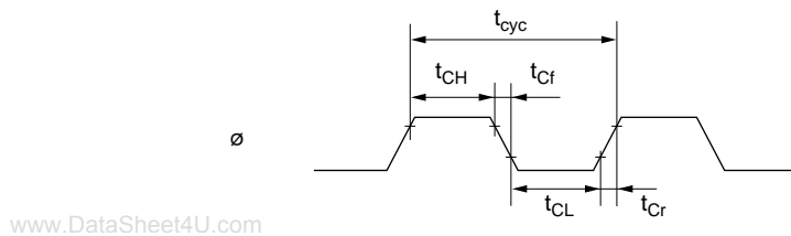
Figure 23.4 System Clock Timing
