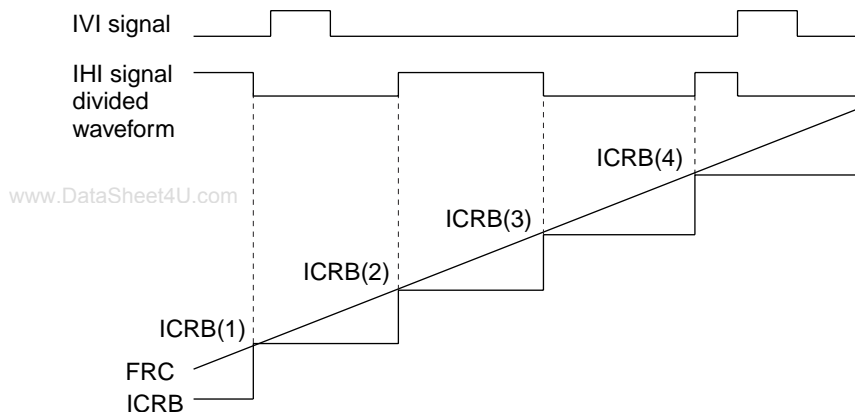
Figure 13.5 Timing Chart for Measurement of IVI Signal and IHI Signal Divided Waveform Periods
