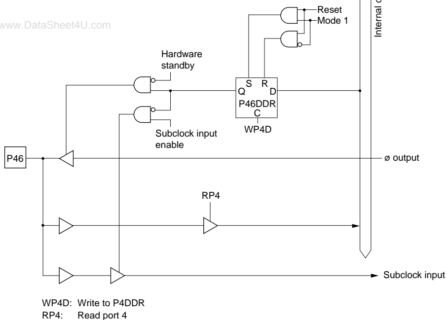
Figure C.13 Port 4 Block Diagram (Pin P46)
