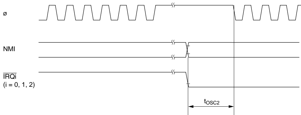
Figure 23.6 Oscillation Settling Timing (Exiting Software Standby Mode)
