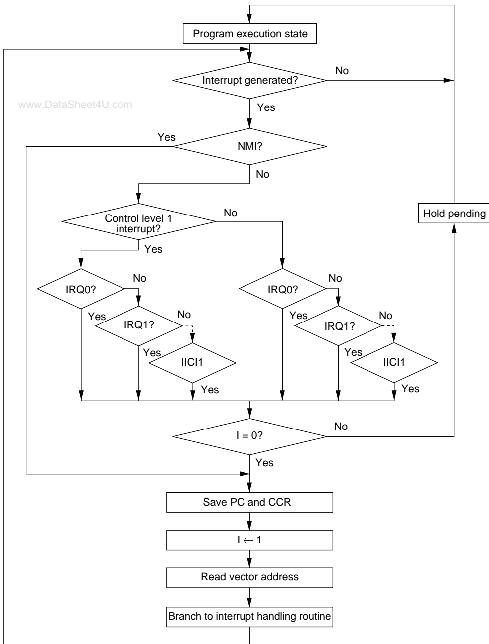
Figure 5.7 Flowchart of Procedure Up to Interrupt Acceptance in Interrupt Control Mode 0
