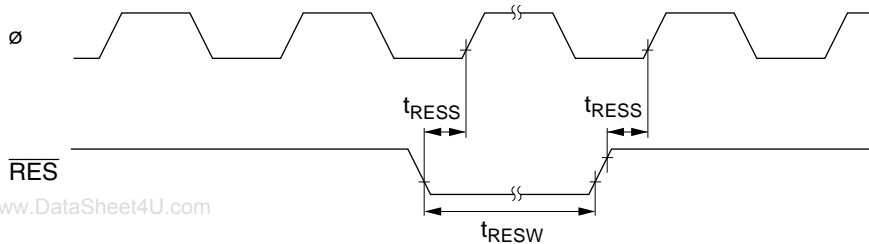
Figure 23.7 Reset Input Timing
