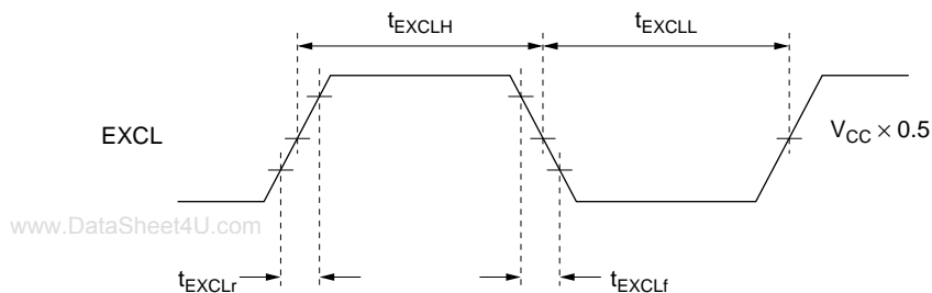
Figure 20.8 Subclock Input Timing
