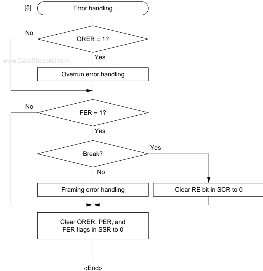
Figure 15.12 Sample Multiprocessor Serial Reception Flowchart (cont)
