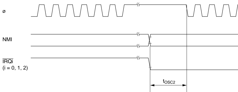
Figure 22.6 Oscillation Settling Timing (Exiting Software Standby Mode)
