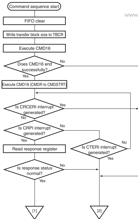
Figure 31.12 Operational Flowchart for Commands with Read Data (Open-ended Multiblock Transfer) (1)
