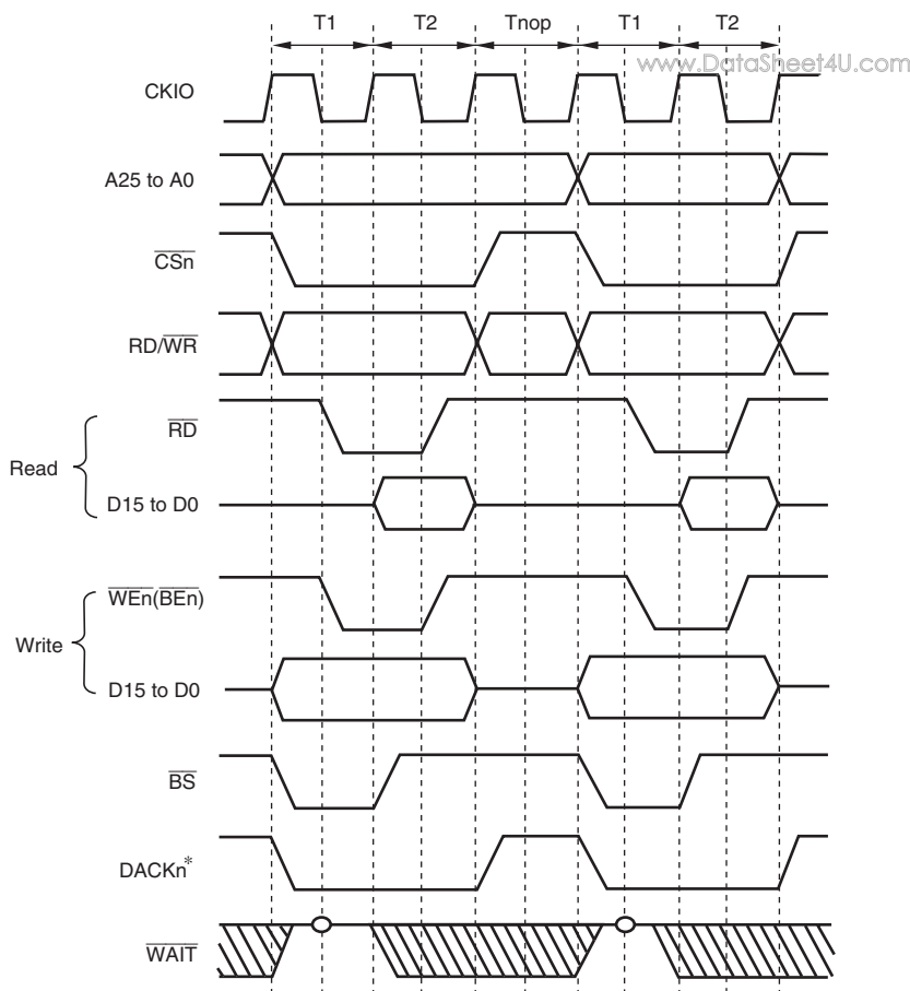
Figure 9.4 Continuous Access for Normal Space 1, Bus Width = 16 bits, Longword Access, CSnWCR.WM Bit = 0 (Access Wait = 0, Cycle Wait = 0)
