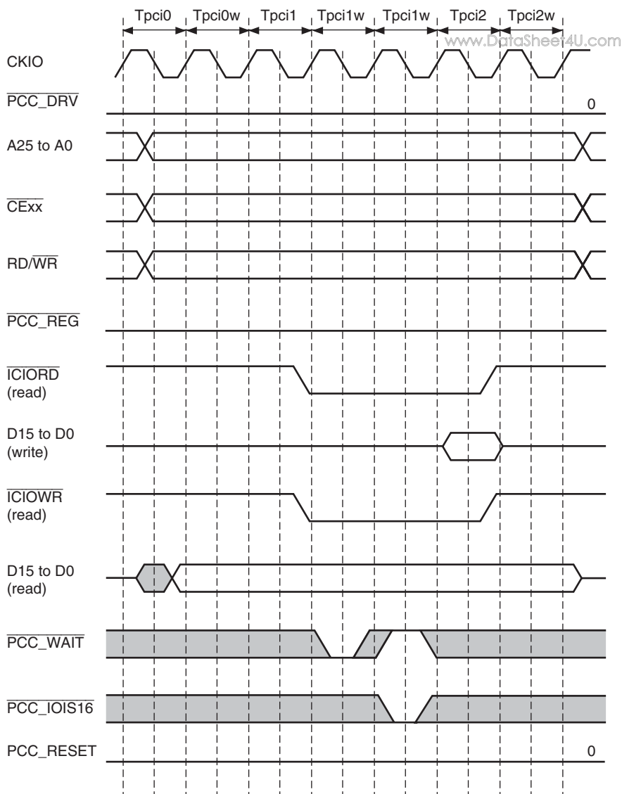
Figure 29.8 PCMCIA I/O Card Interface Wait Timing
