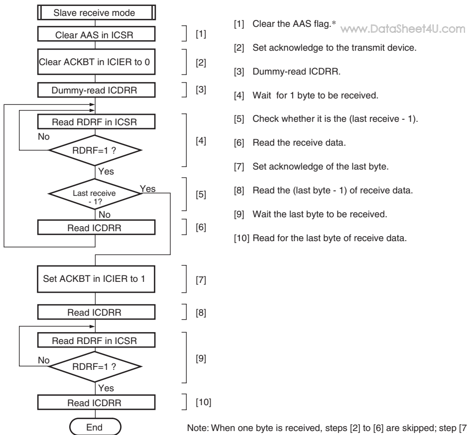
Figure 20.17 Sample Flowchart for Slave Receive Mode
