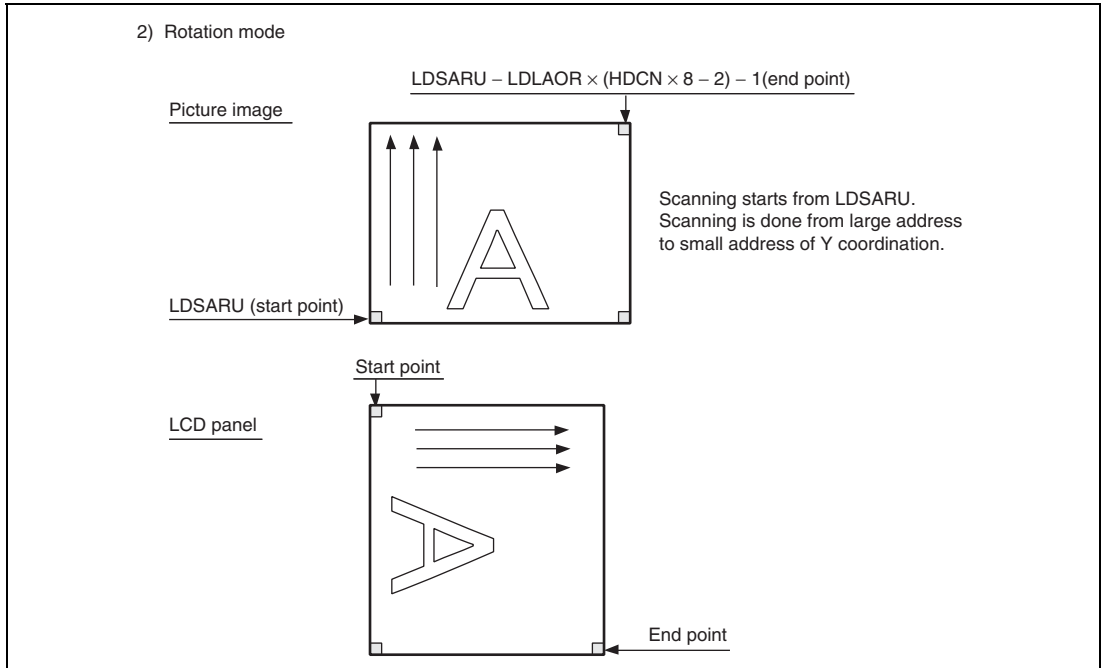
Figure 26.9 Operation for Hardware Rotation (Rotation Mode)
