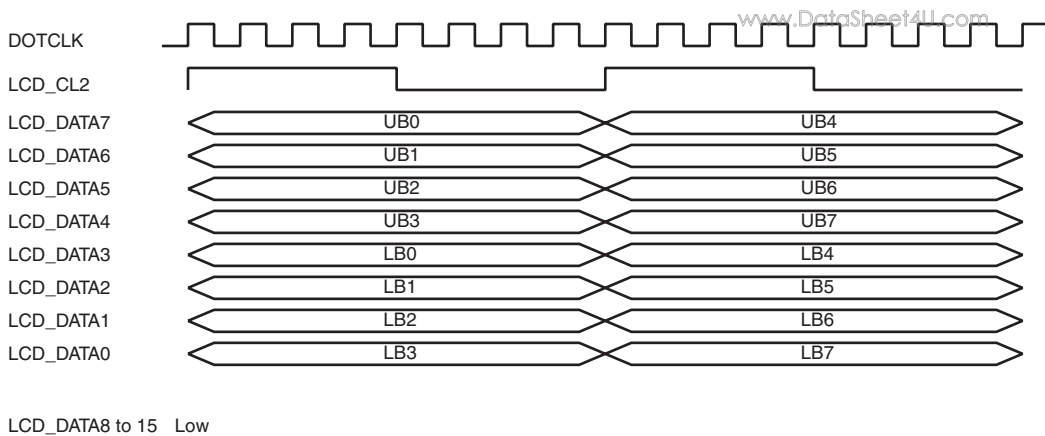
Figure 26.16 Clock and LCD Data Signal Example (DSTN Monochrome 8-Bit Data Bus Module)
