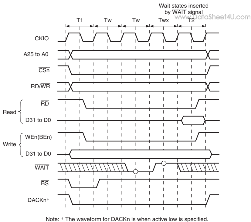
Figure 9.10 Wait State Timing for Normal Space Access (Wait State Insertion using \overline{WAIT} Signal)
