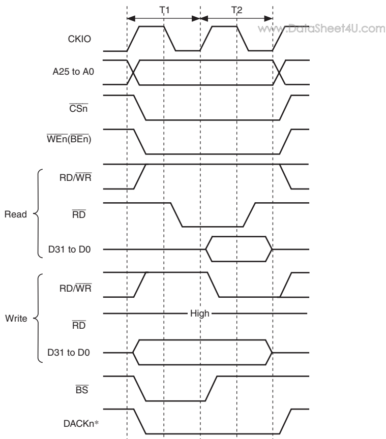
Figure 9.33 Basic Access Timing for Byte-Selection SRAM (BAS = 1)
