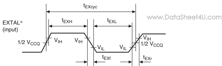
Figure 38.1 EXTAL Clock Input Timing
