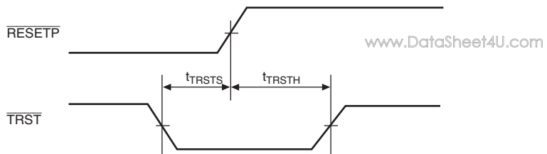
Figure 38.66 \overline{\text{TRST}} Input Timing (Reset Hold)
