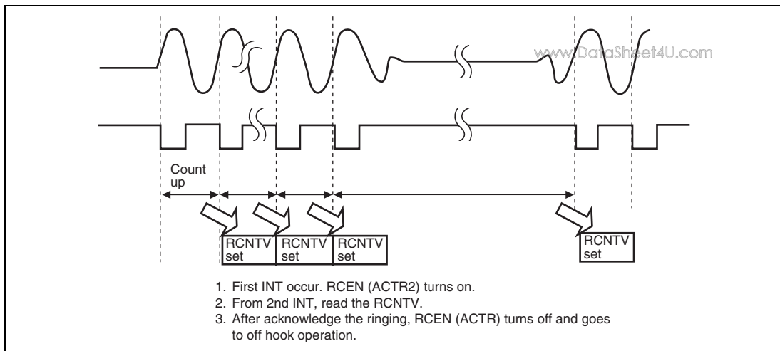
Figure 22.8 Ringing Detect Sequence
