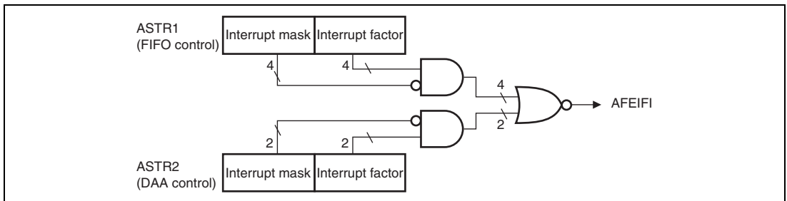
Figure 22.4 Interrupt Generator
