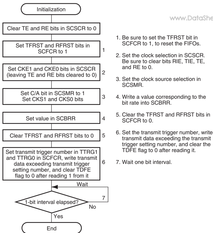
Figure 18.13 Sample SCIF Initialization Flowchart (3) (Simultaneous Transmission and Reception)
