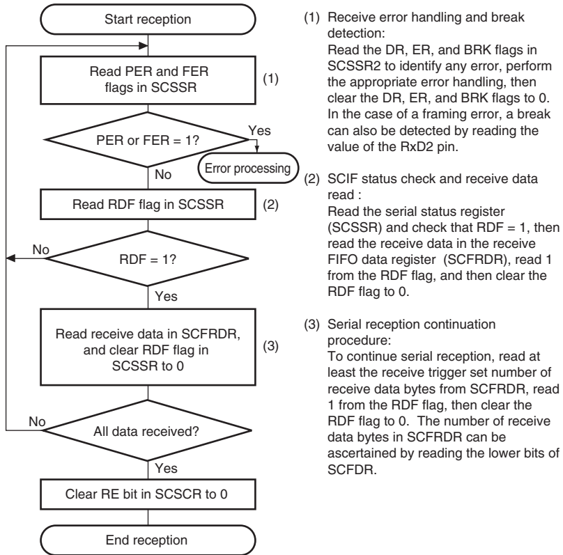
Figure 18.7 Sample Serial Reception Flowchart (1)
