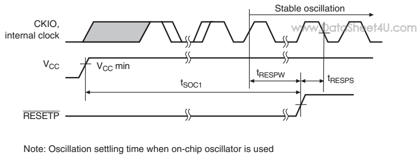
Figure 38.4 Power-On Oscillation Settling Time
