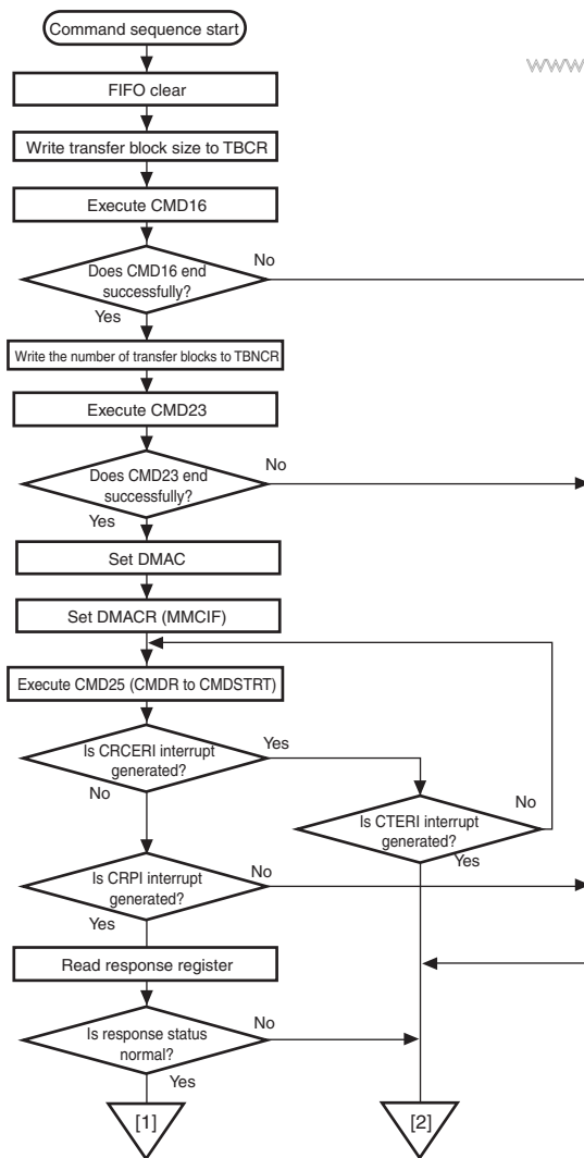
Figure 31.32 Operational Flowchart for Pre-defined Multiblock Write Transfer in Auto Mode (1)
