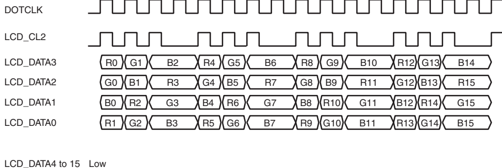
Figure 26.12 Clock and LCD Data Signal Example (STN Color 4-Bit Data Bus Module)
