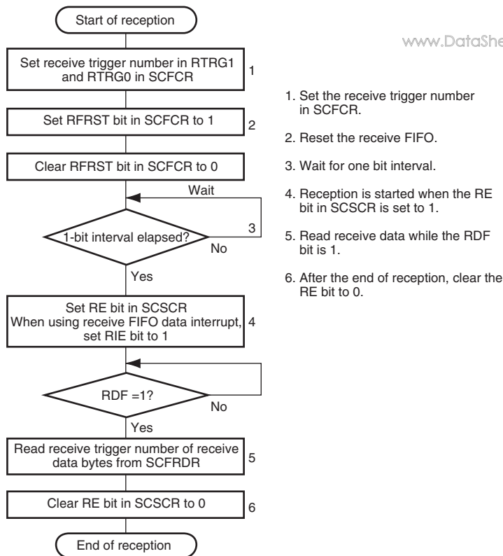
Figure 18.15 Sample Serial Reception Flowchart (2) (Second and Subsequent Reception)
