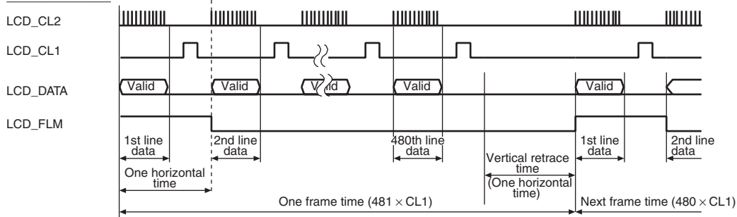
Figure 26.22 Clock and LCD Data Signal Example (8-Bit Interface Color 640 × 480)
