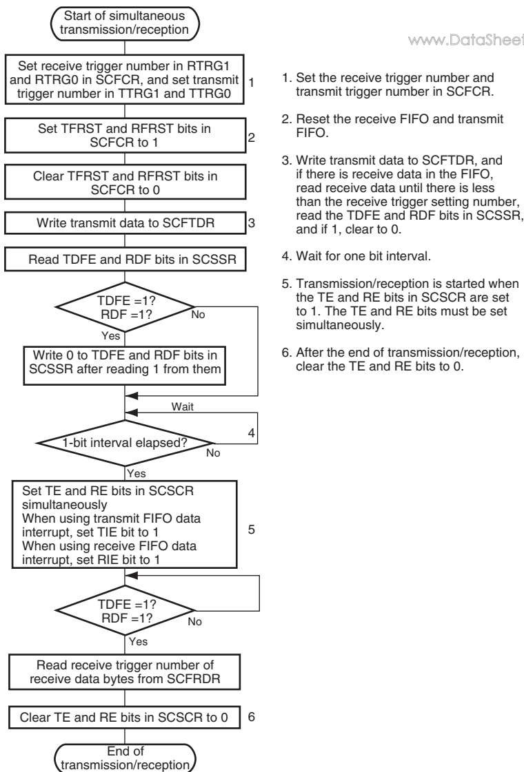
Figure 18.16 Sample Simultaneous Serial Transmission and Reception Flowchart (2) (Second and Subsequent Transfer)
