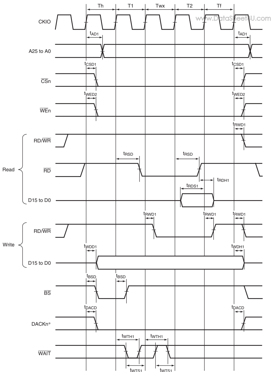
Figure 38.18 Bus Cycle of SRAM with Byte Selection (SW = 1 Cycle, HW = 1 Cycle, External Wait 1 Input, BAS = 1 (WE in Write Cycle Controlled))
