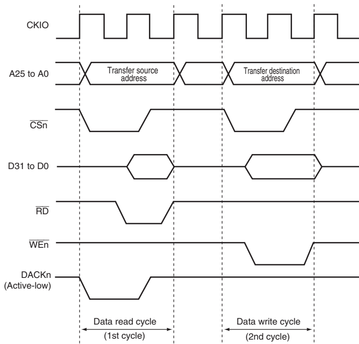
Figure 10.6 Example of DMA Transfer Timing in Dual Mode (Source: Ordinary Memory, Destination: Ordinary Memory)
