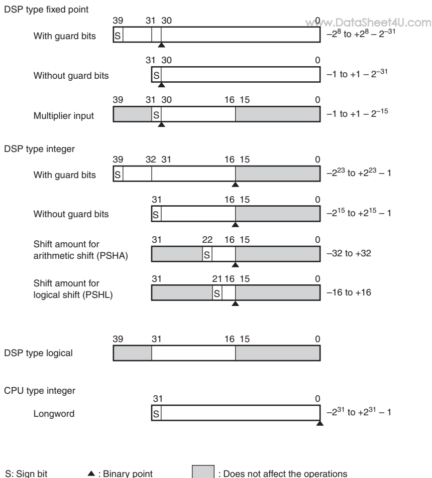
Figure 3.8 Data Formats
