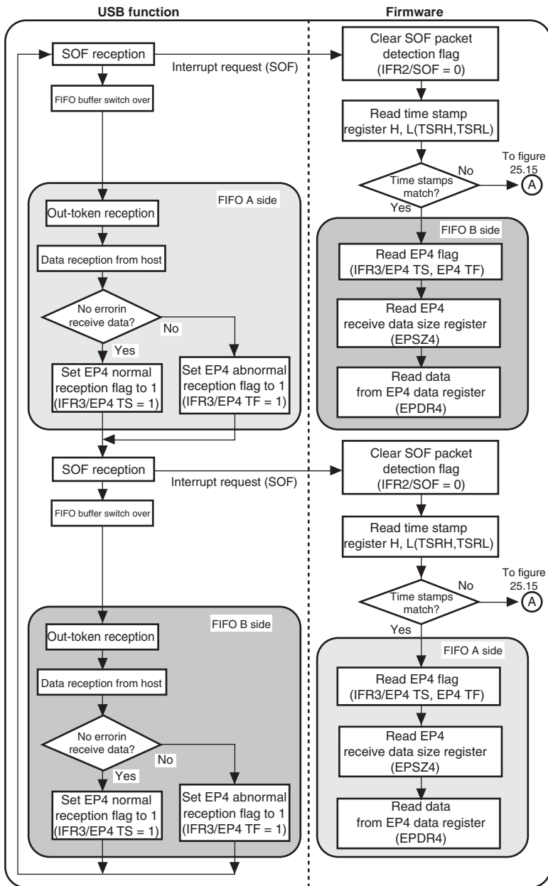
Figure 25.14 EP4 Isochronous-Out Transfer Operation (SOF is Normal)
