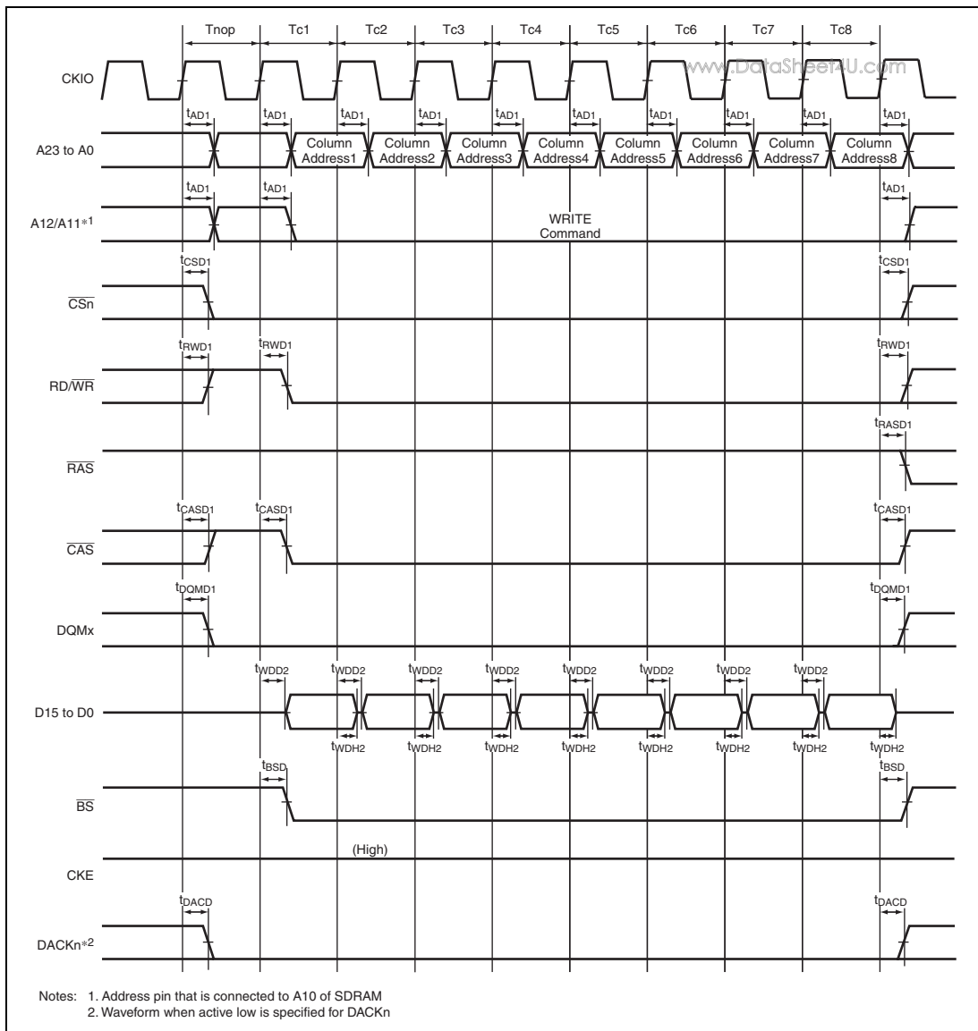
Figure 38.32 Burst Write Bus Cycle of SDRAM (Single Write \times 8 ) (Bank Active Mode: ACTV + WRIT Command, TRCD = 1 Cycle)
