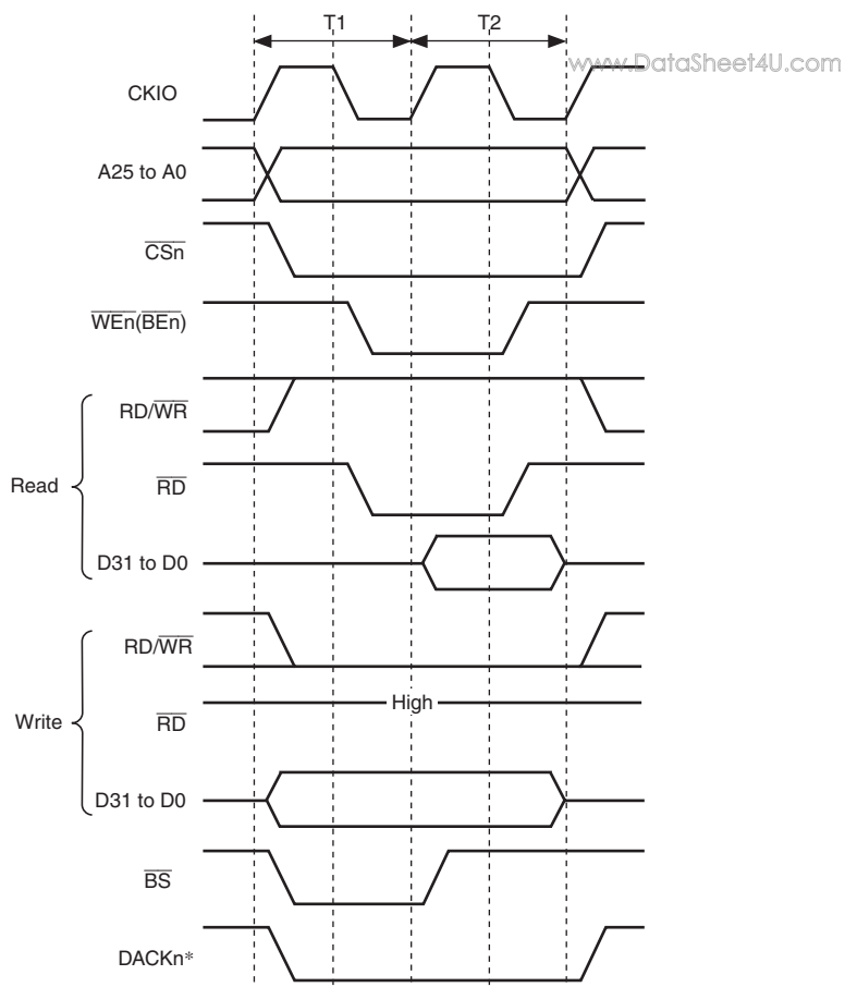
Figure 9.32 Basic Access Timing for Byte-Selection SRAM (BAS = 0)
