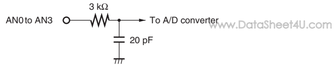
Figure 27.10 Analog Input Pin Equivalent Circuit
