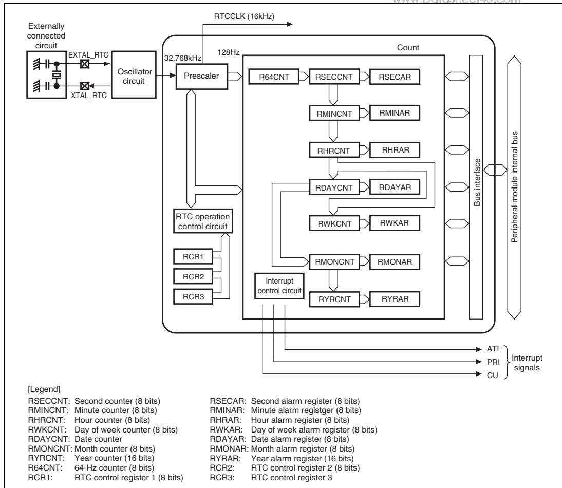
Figure 17.1 RTC Block Diagram
