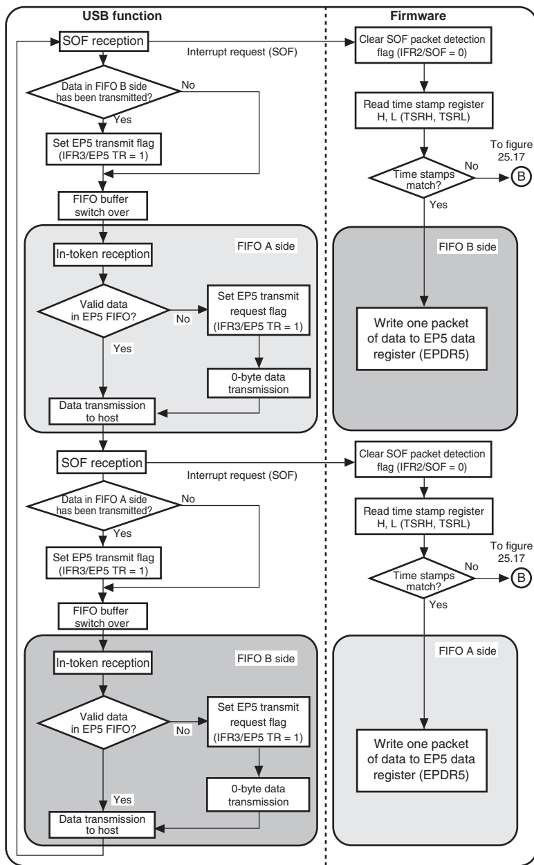
Figure 25.16 EP5 Isochronous-In Transfer Operation (SOF is Normal)
