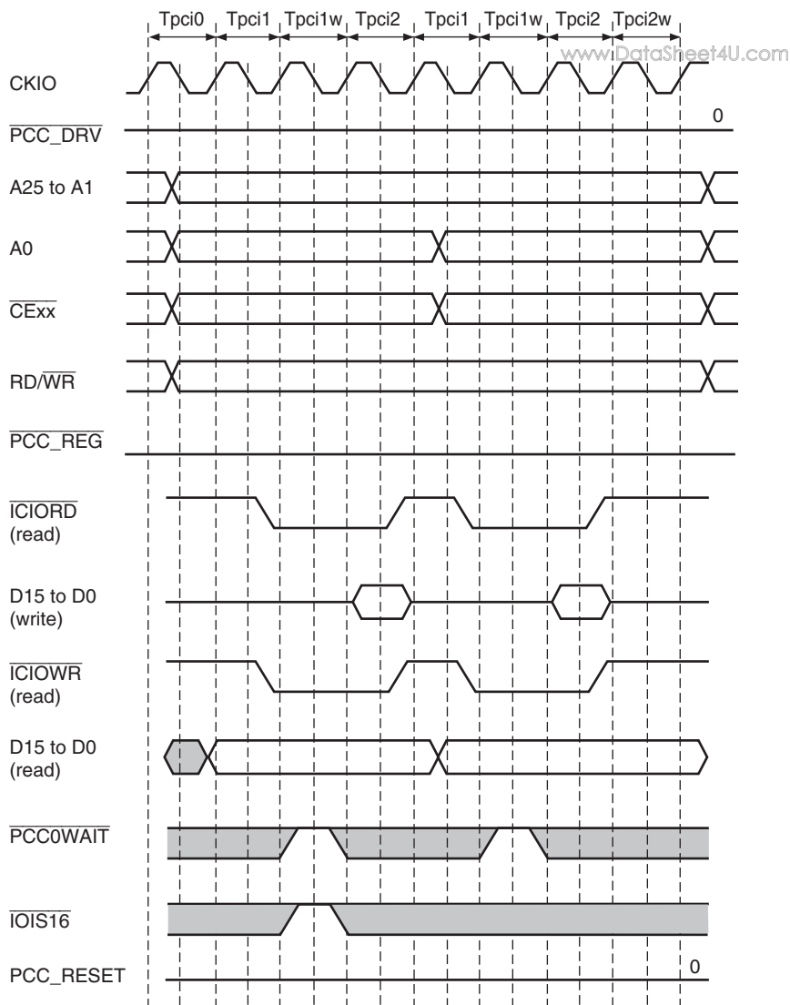
Figure 29.9 Dynamic Bus Sizing Timing for PCMCIA I/O Card Interface
