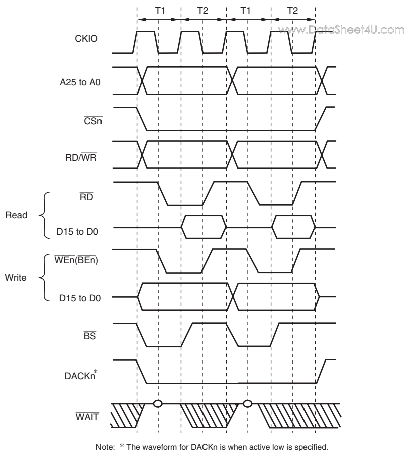
Figure 9.5 Continuous Access for Normal Space 2, Bus Width = 16 bits, Longword Access, CSnWCR.WM Bit = 1 (Access Wait = 0, Cycle Wait = 0)
