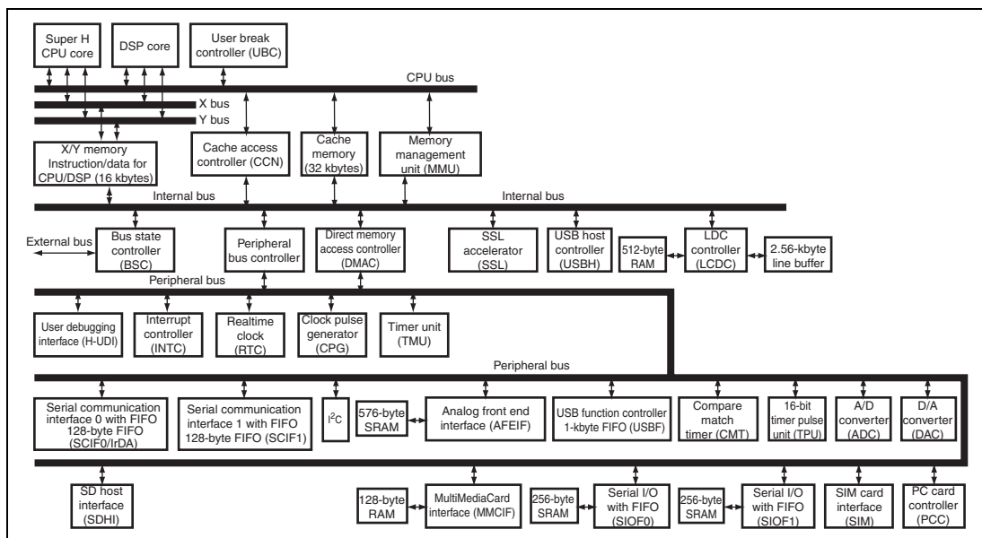
Figure 1.1 Block Diagram
