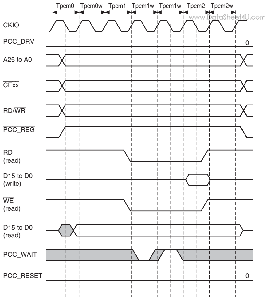
Figure 29.6 PCMCIA Memory Card Interface Wait Timing
