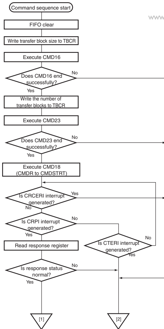
Figure 31.13 Operational Flowchart for Commands with Read Data (Pre-defined Multiblock Transfer) (1)
