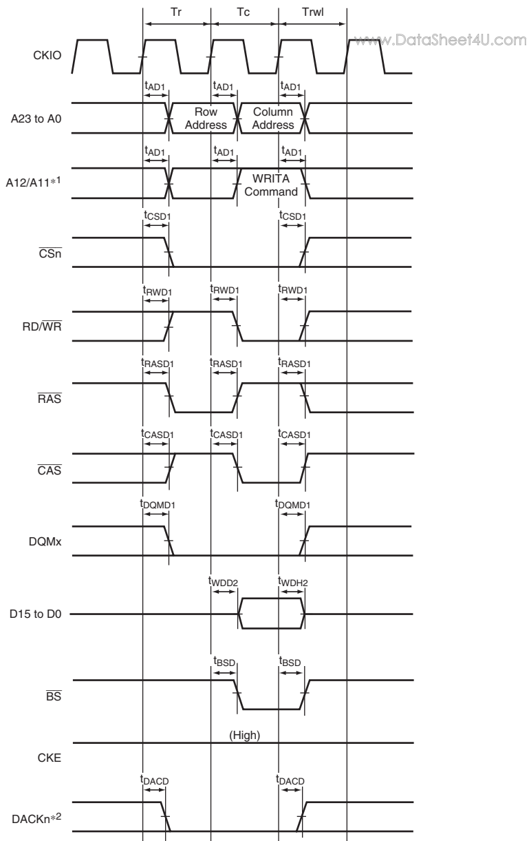
Figure 38.24 Single Write Bus Cycle of SDRAM (Auto Precharge Mode, TRWL = 1 Cycle)
