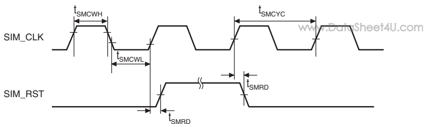
Figure 38.62 SIM Module Signal Timing
