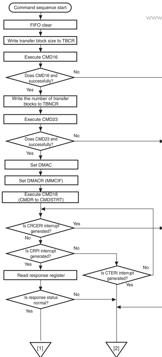
Figure 31.27 Operational Flowchart for Pre-defined Multiblock Read Transfer in Auto Mode (1)
