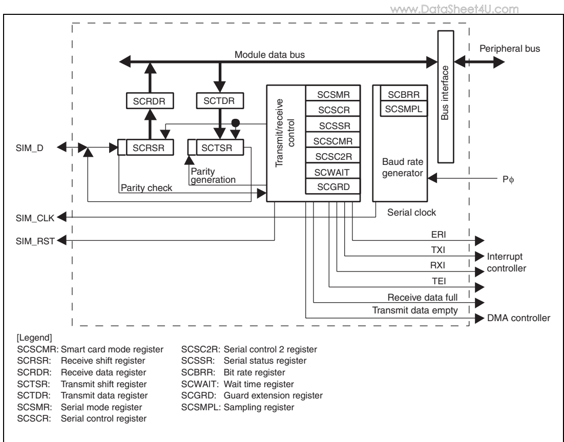
Figure 30.1 Smart Card Interface
