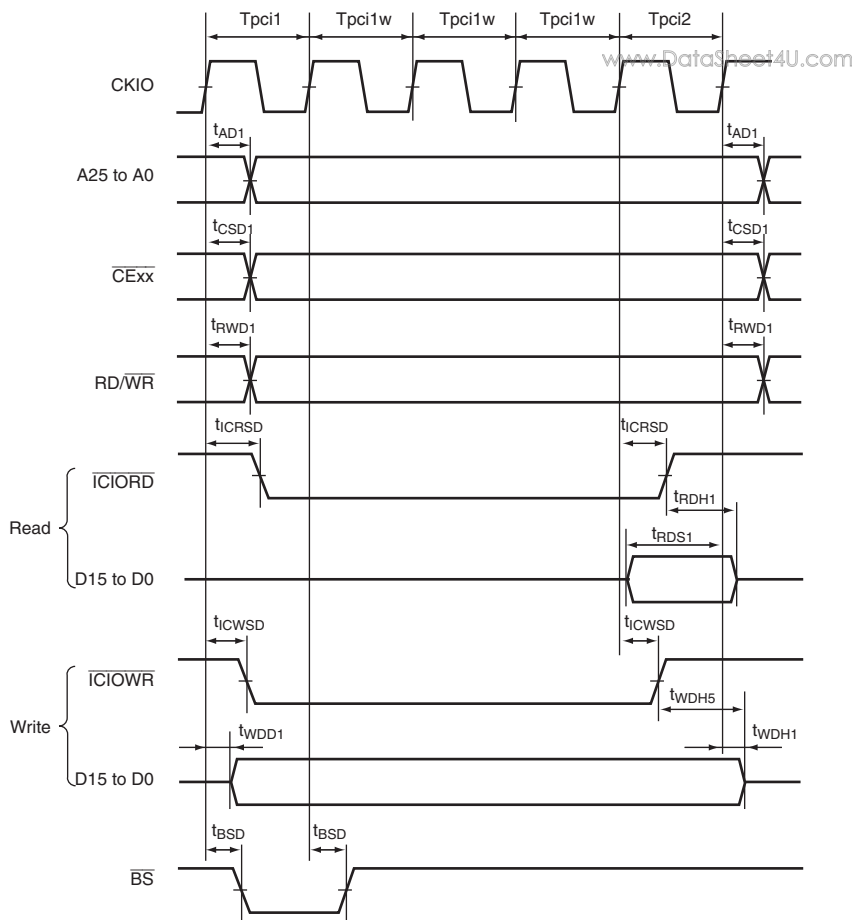
Figure 38.41 PCMCIA I/O Card Interface Bus Timing
