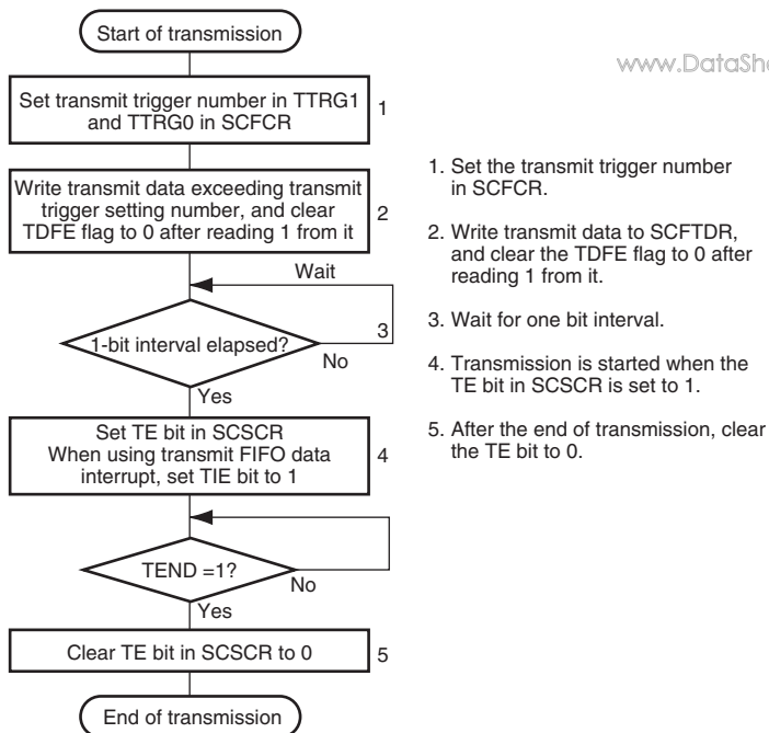
Figure 18.14 Sample Serial Transmission Flowchart (2) (Second and Subsequent Transmission)
