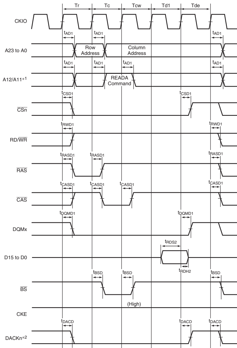
Figure 38.20 Single Read Bus Cycle of SDRAM
