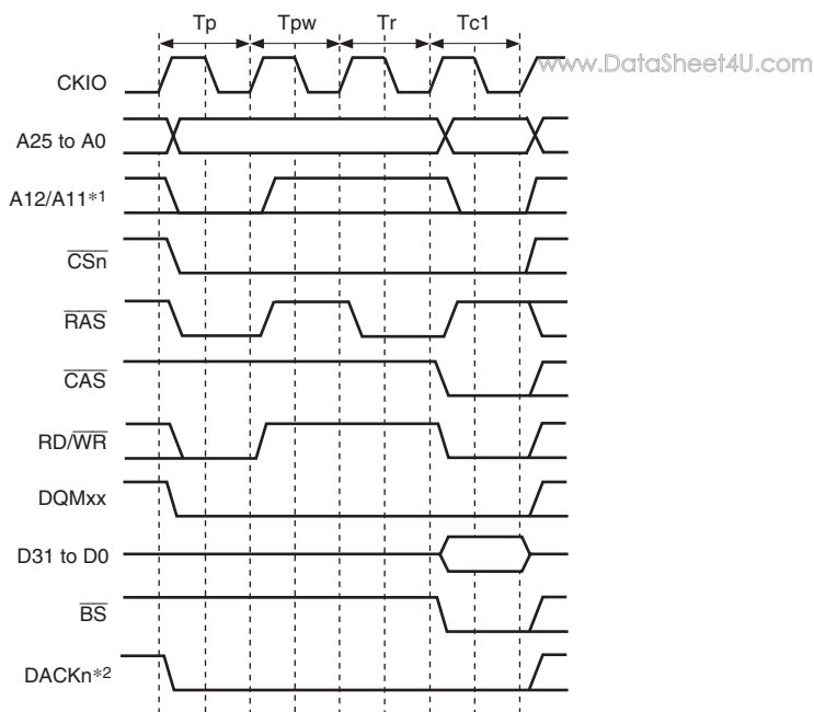
Figure 9.24 Single Write Timing (Bank Active, Different Row Addresses)
