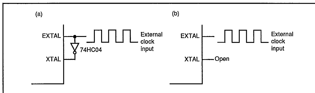
Figure 14-5. External Clock Input (Example)
