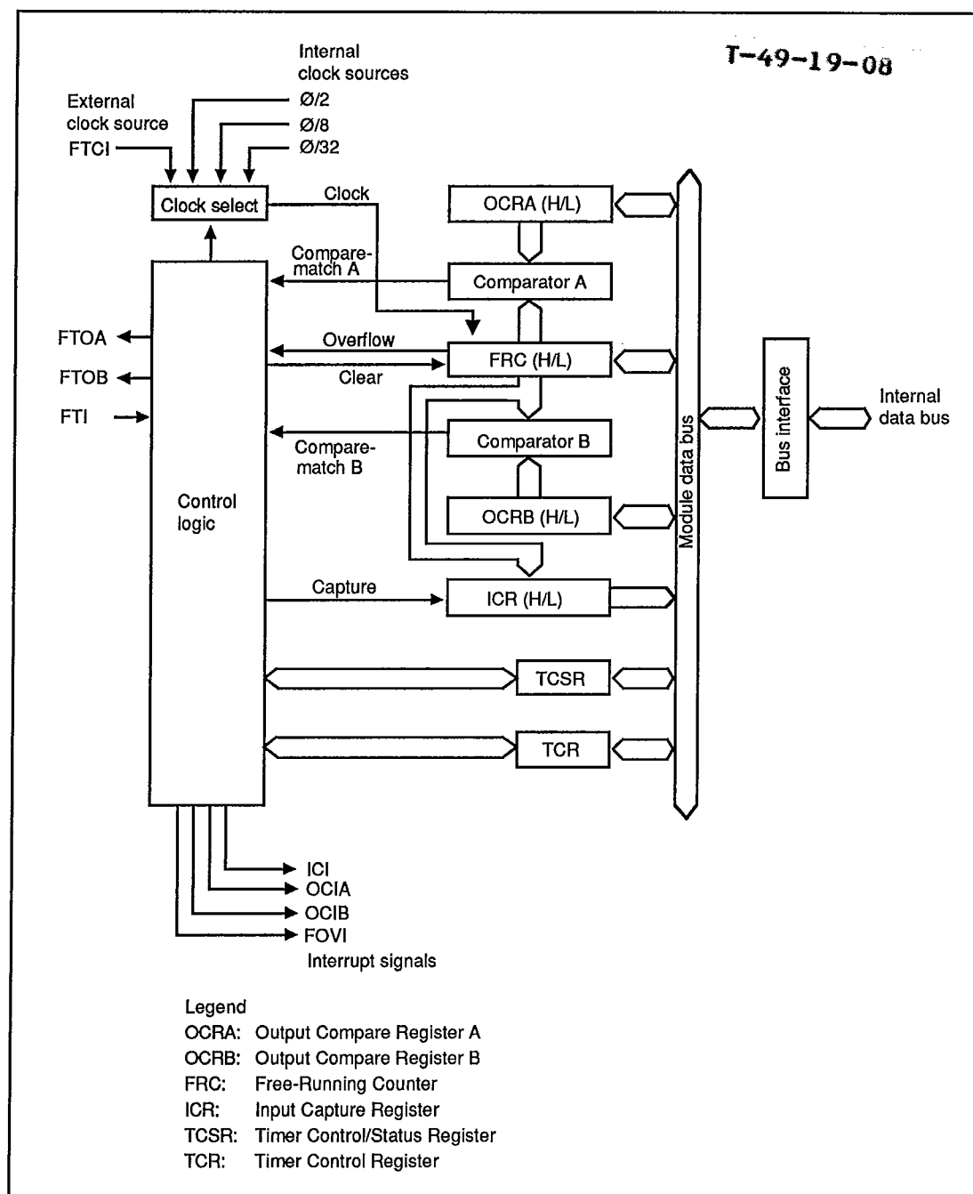
Figure 7-1. Block Diagram of 16-Bit Free-Running Timer
