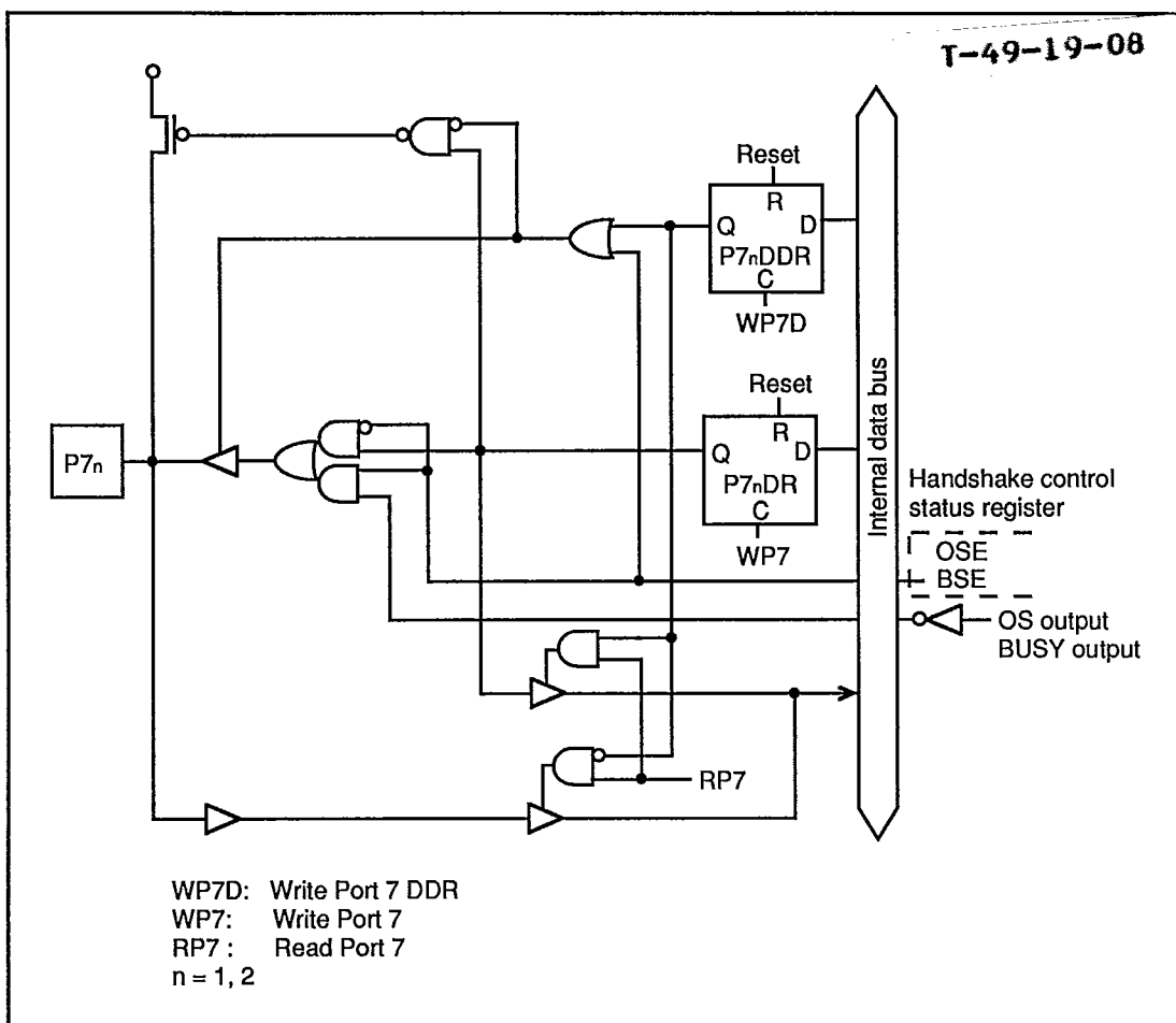
Figure 5-15. Port 7 Schematic Diagram (Pins P71 and P72)
