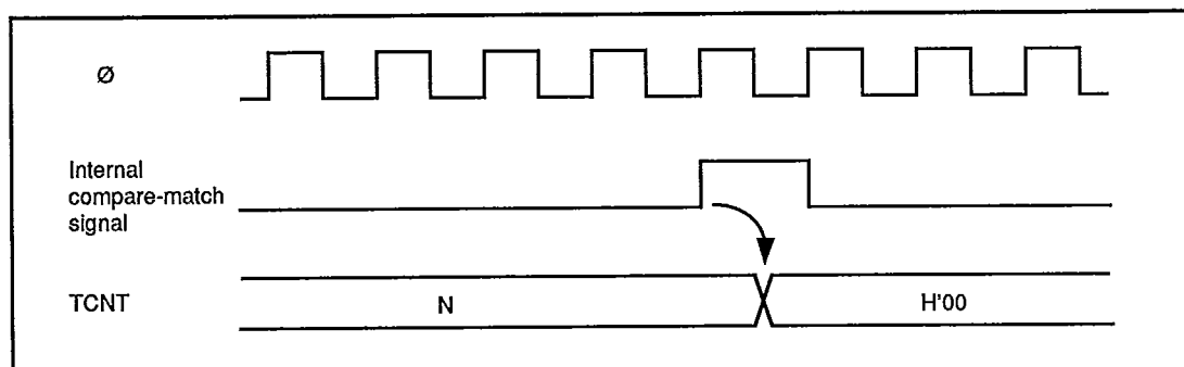
Figure 8-8. Timing of Compare-Match Clear
