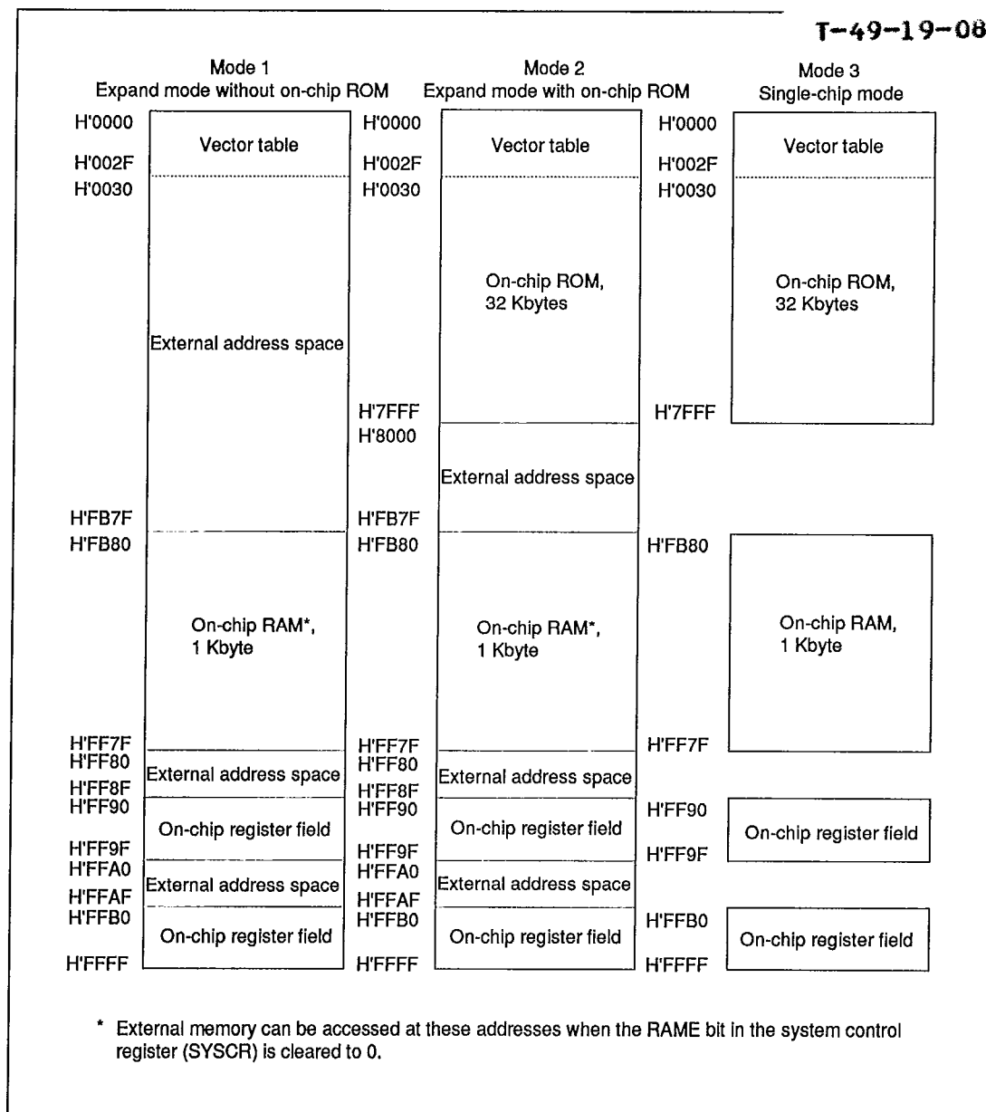
Figure 2-1. H8/325 Address Space Map
