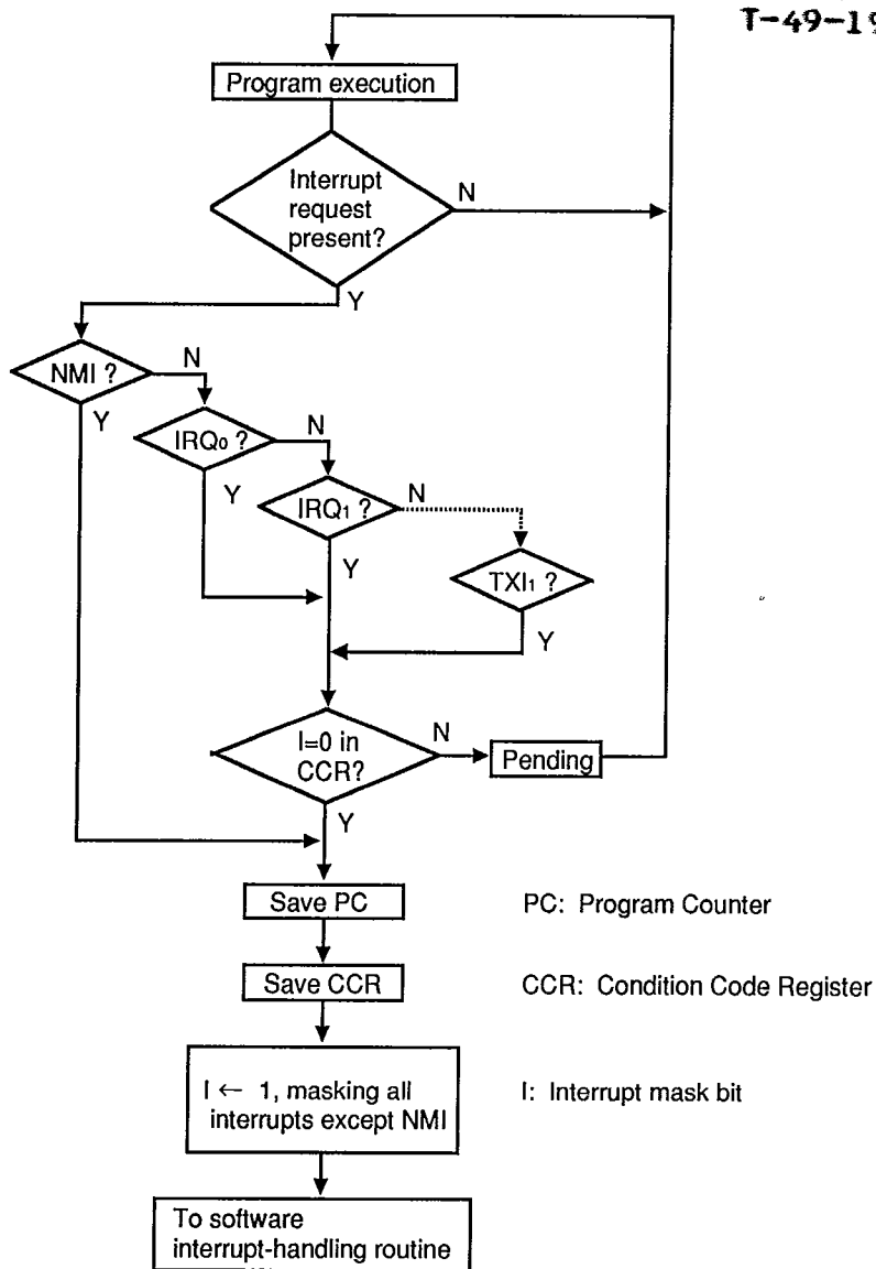
Figure 4-4. Hardware Interrupt-Handling Sequence
