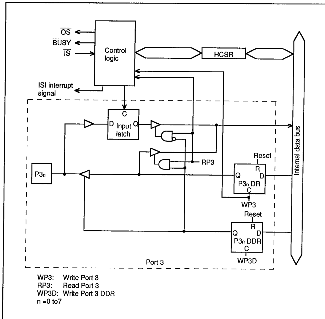
Figure 6-1. Block Diagram of Parallel Handshaking Interface
