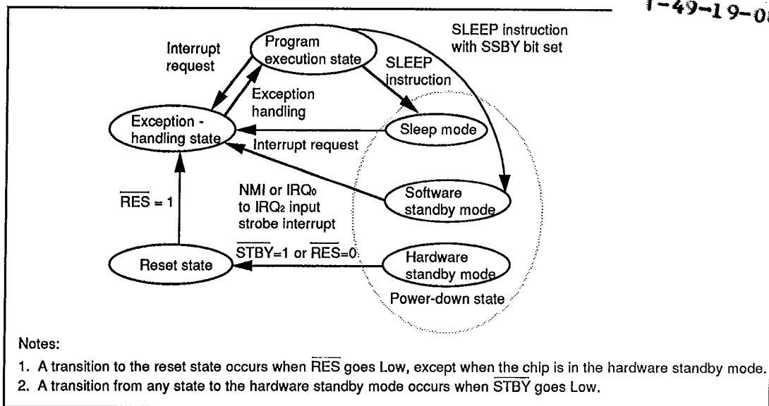
Figure 3-12. State Transitions
