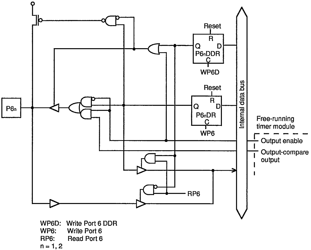
Figure 5-12. Port 6 Schematic Diagram (Pins P61 and P62)
