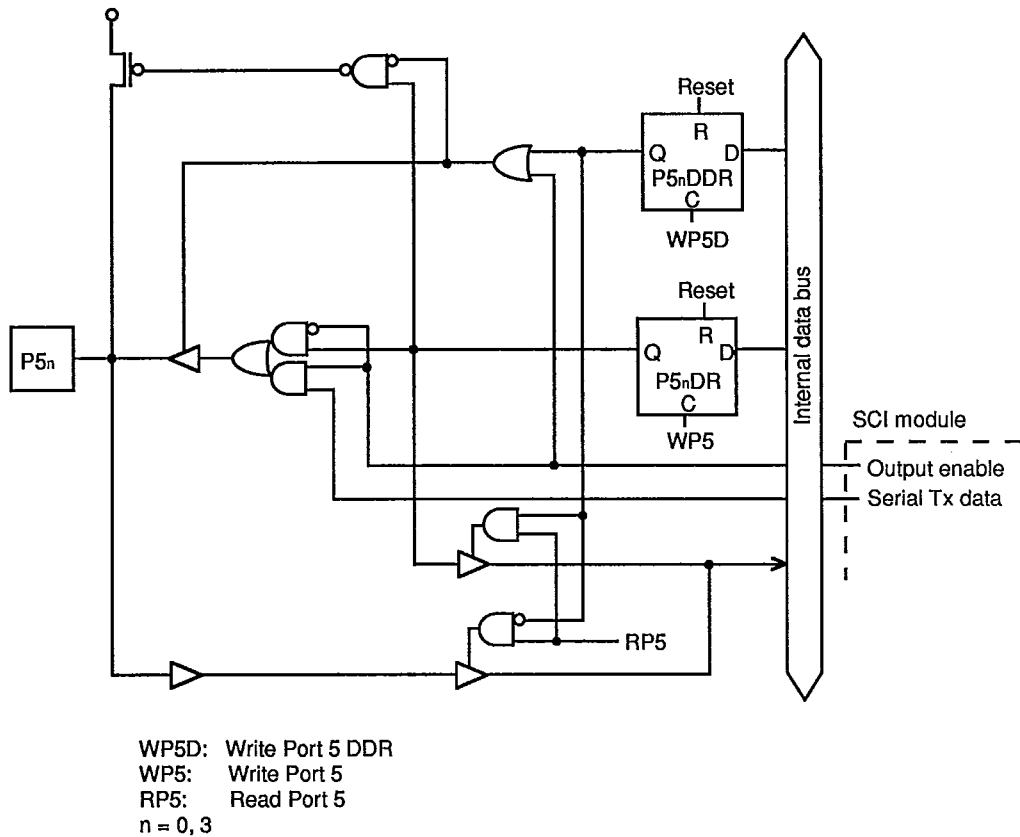
Figure 5-8. Port 5 Schematic Diagram (Pins P50 and P53)
