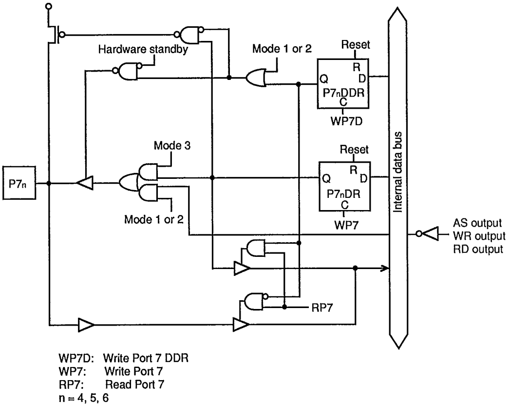
Figure 5-17. Port 7 Schematic Diagram (Pins P74, P75, and P76)
