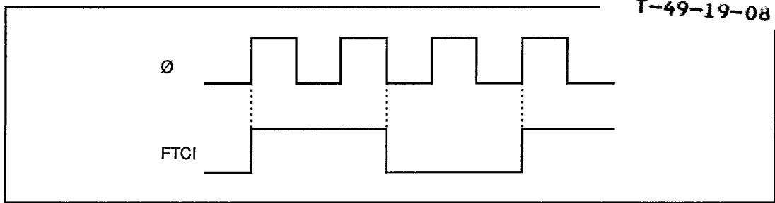
Figure 7-6. Minimum External Clock Pulse Width
