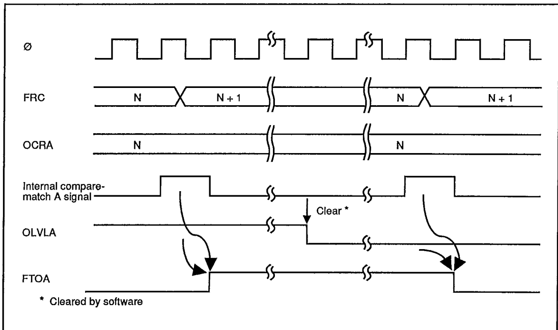
Figure 7-7. Timing of Output Compare A
