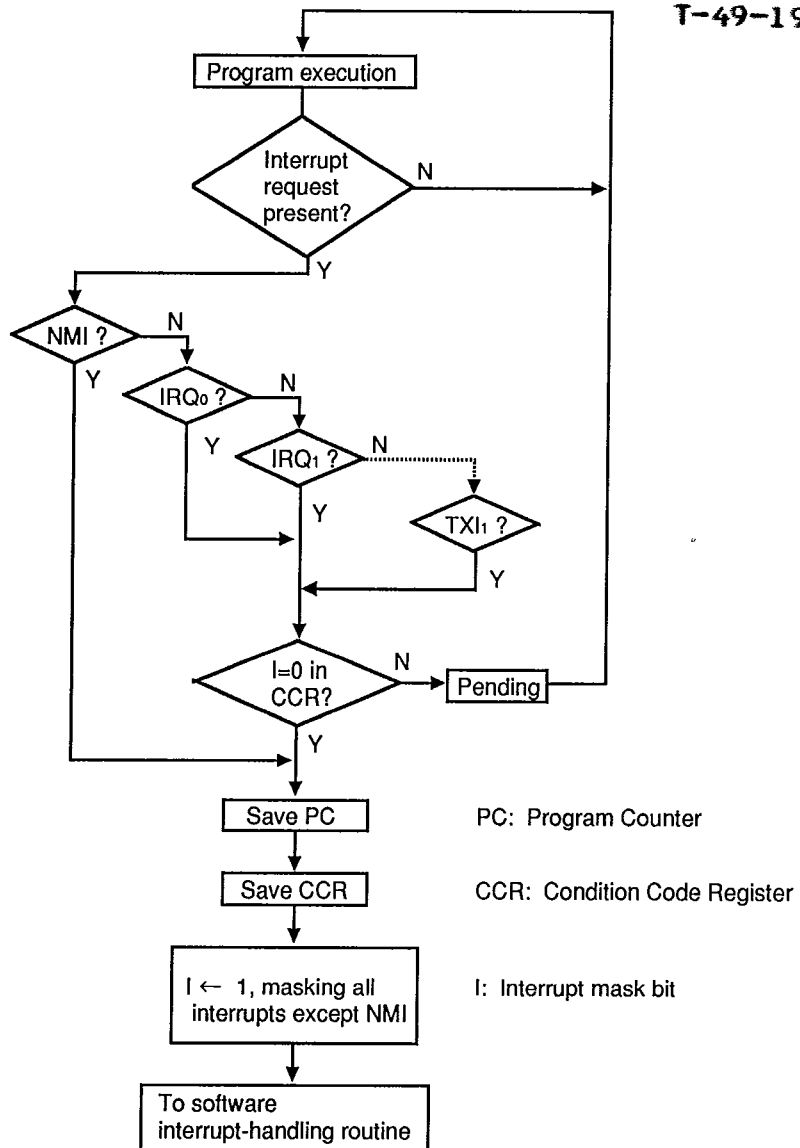
Figure 4-4. Hardware Interrupt-Handling Sequence
