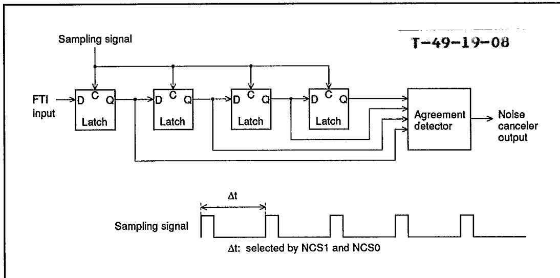
Figure 7-14. Noise Canceler Block Diagram
