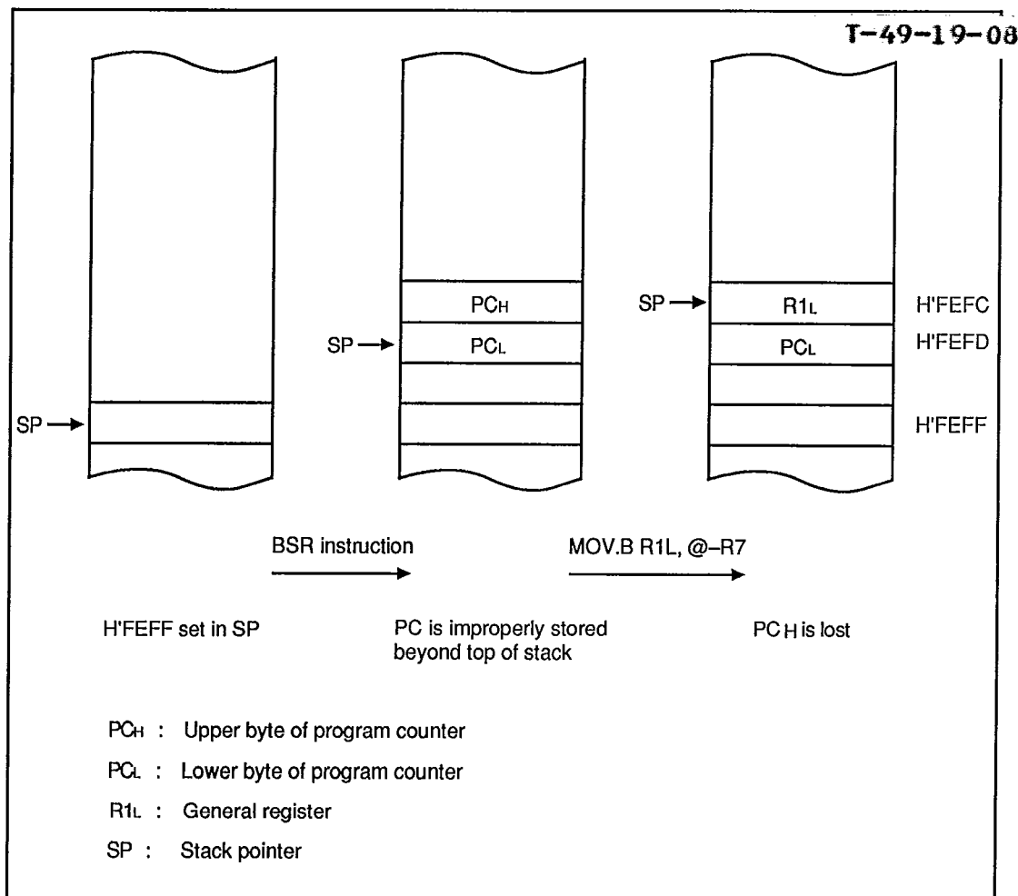
Figure 4-7. Example of Damage Caused by Setting an Odd Address in R7
