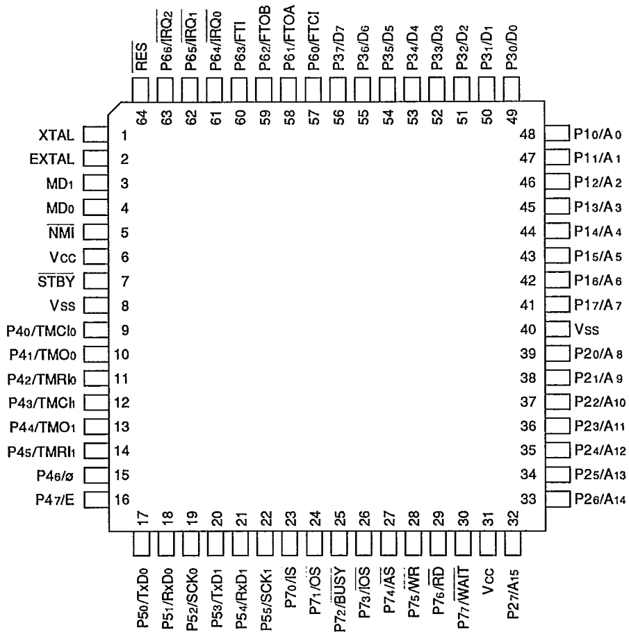
Figure 1-3. Pin Arrangement (FP-64A, Top View)
