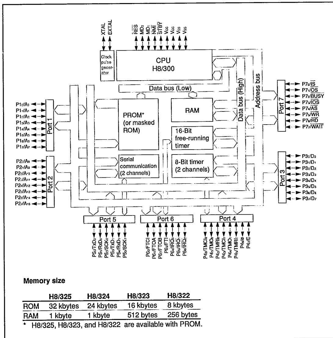
Figure 1-1. Block Diagram
