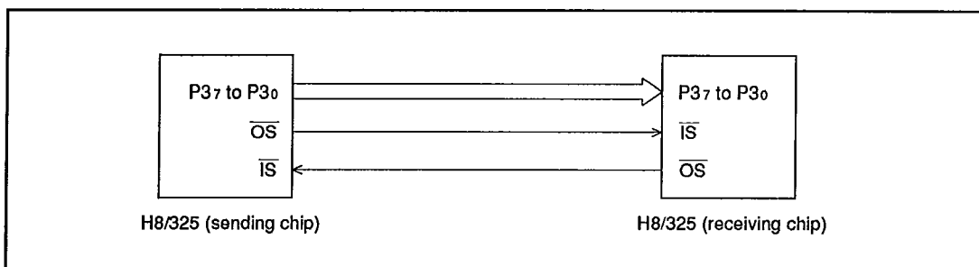
Figure 6-6. Sample Usage of Parallel Handshaking Interface
