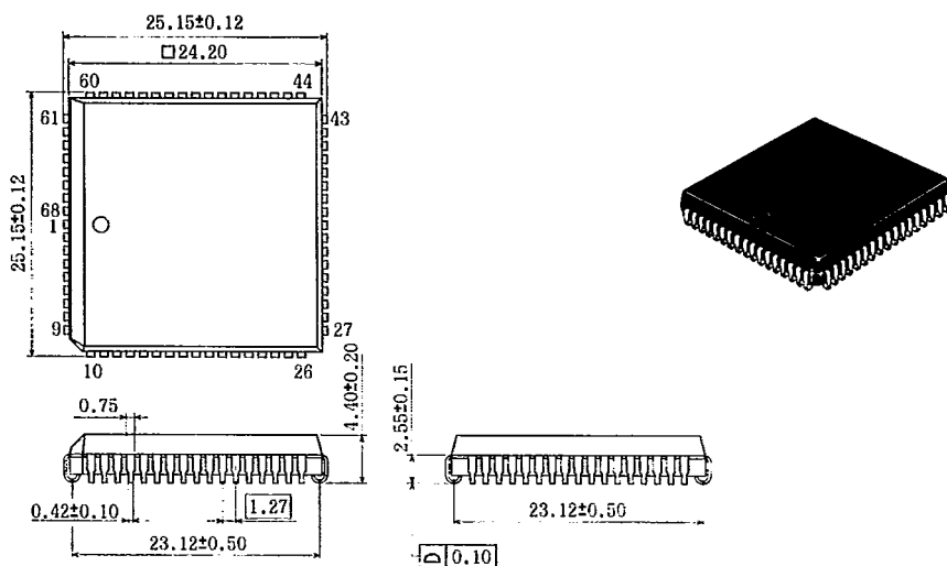
Figure E-4. Package Dimensions (CP-68)
