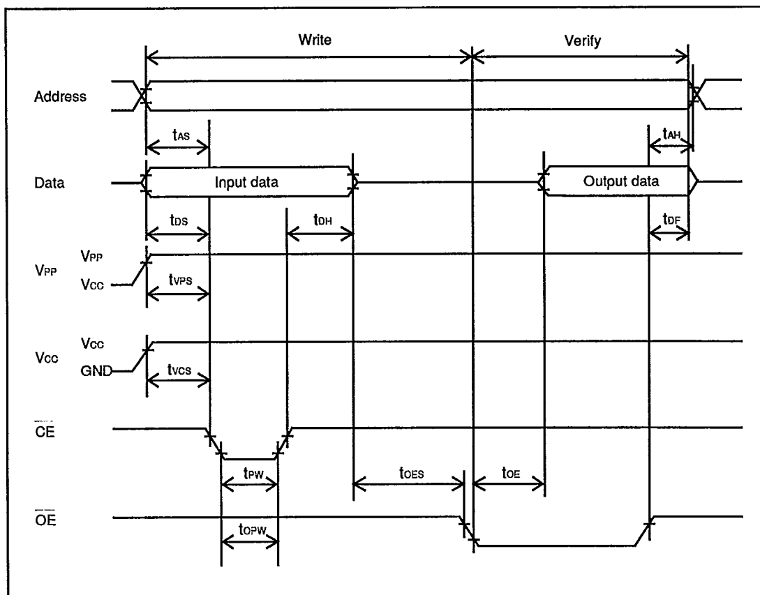
Figure 11-7. PROM Write/Verify Timing
