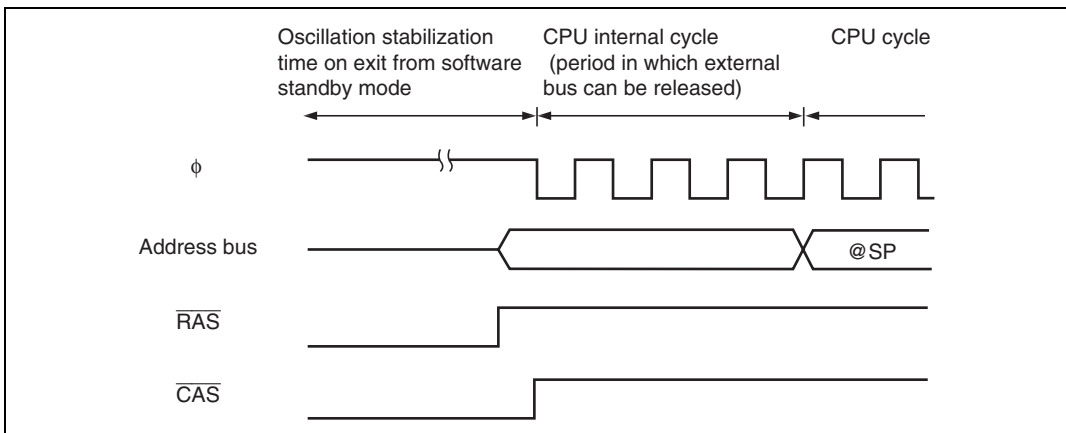
Figure 6.35 Self-Refresh Clearing
