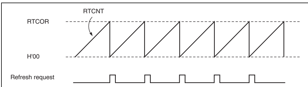
Figure 6.24 RTCNT Operation
