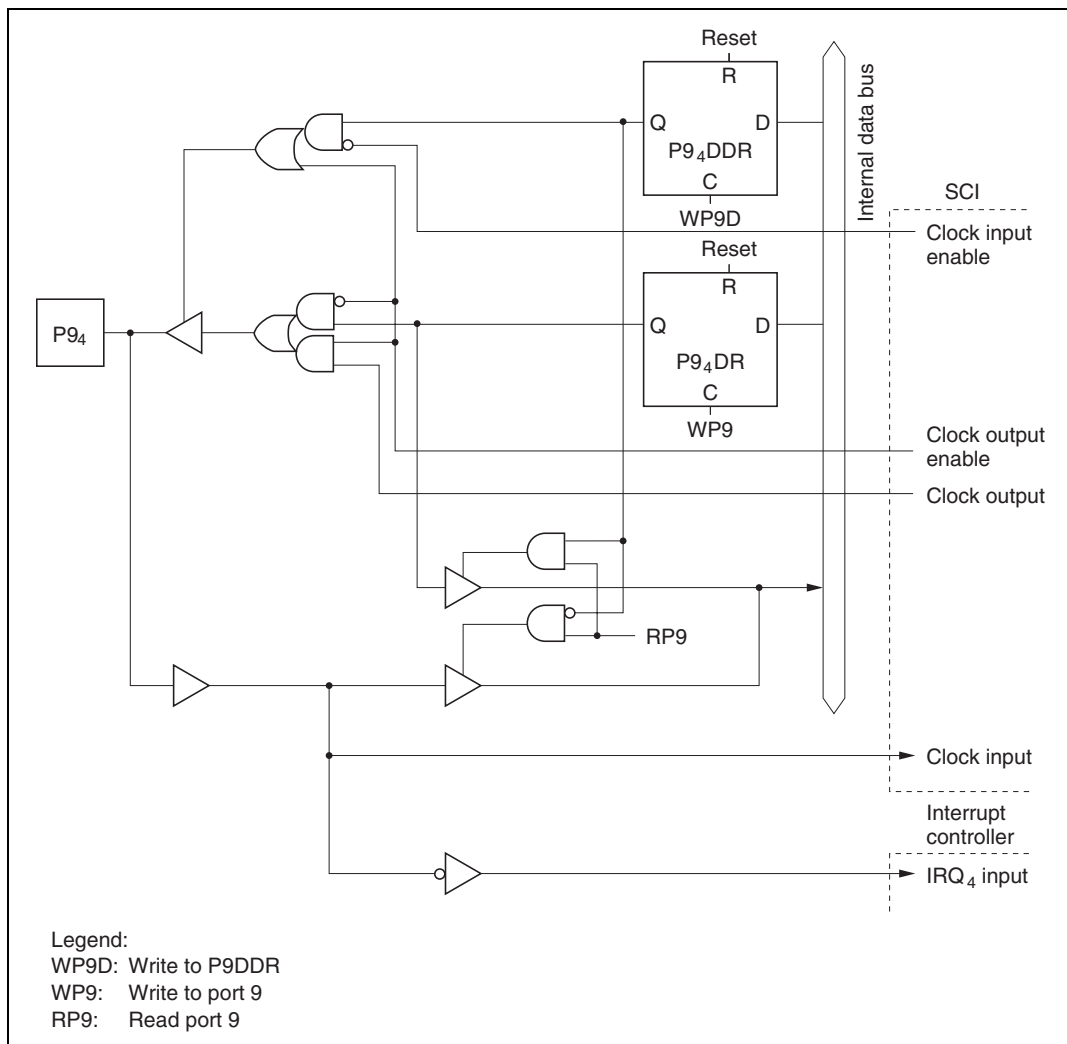
Figure C.5 (e) Port 9 Block Diagram (Pin P9 A )
