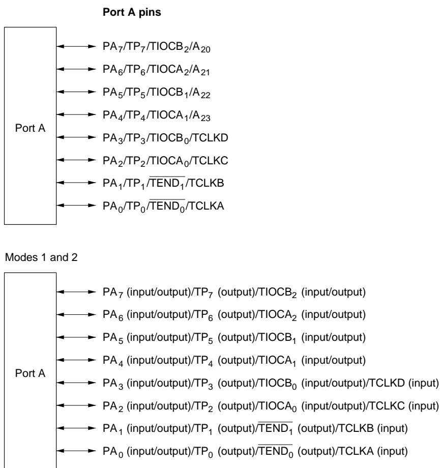
Figure 9-8 Port A Pin Configuration (1)
