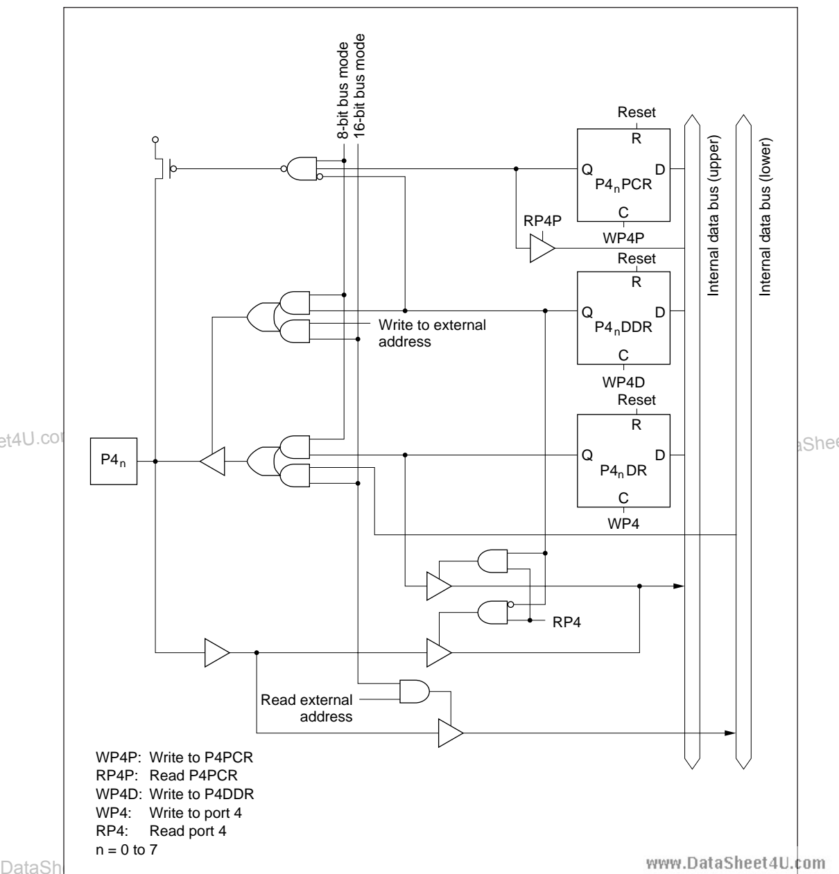
Figure C-1 Port 4 Block Diagram
