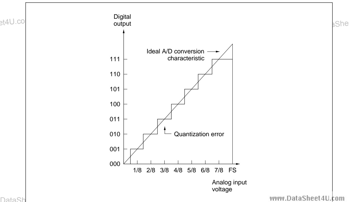
Figure 14-9 A/D Converter Accuracy Definitions (1)
