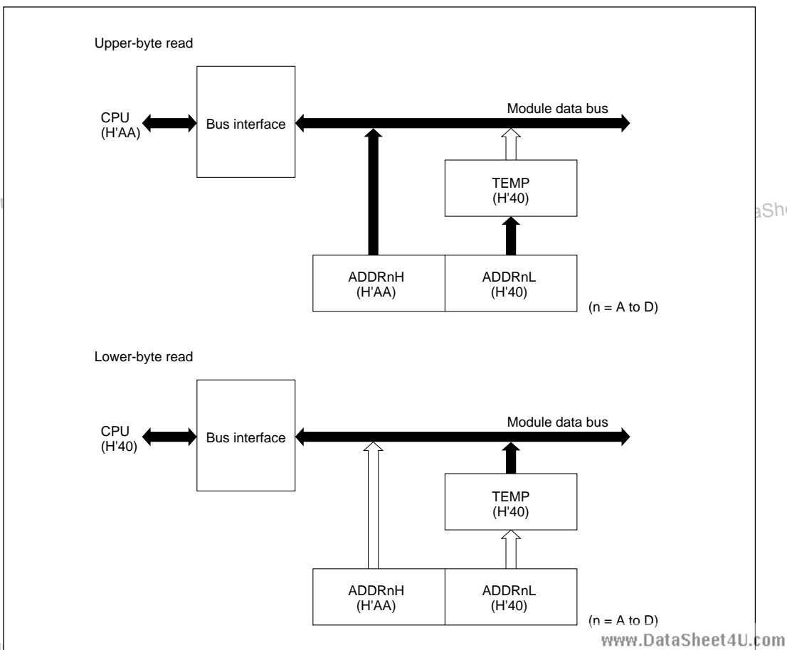
Figure 14-2 A/D Data Register Access Operation (Reading H'AA40)
