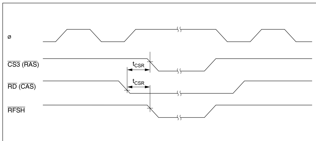
Figure 18-9 DRAM Bus Timing (Self-Refresh Mode) www.DataSheet4U.com — \overline{2WE} Mode —
