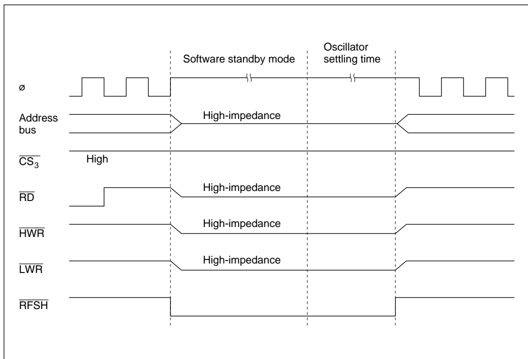
Figure 7-16 Signal Output Timing in Self-Refresh Mode (PSRAME = 1, DROME = 0)
