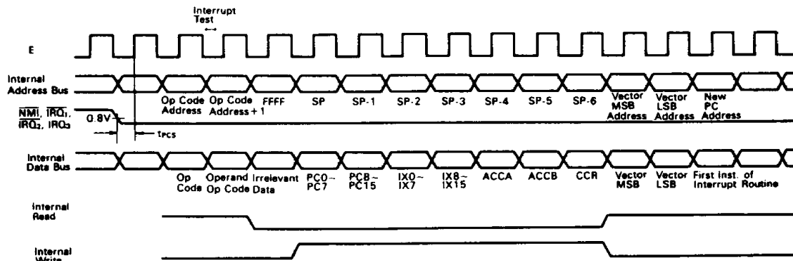
Figure 10 Interrupt Sequence
