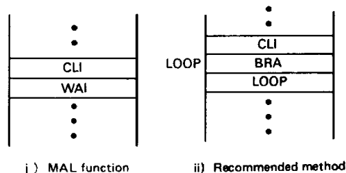
Figure 31 Program to wait for interrupt
