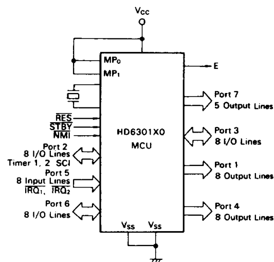
Figure 17 Mode 3
