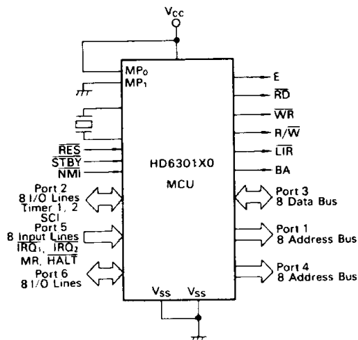
Figure 15 Mode 1
