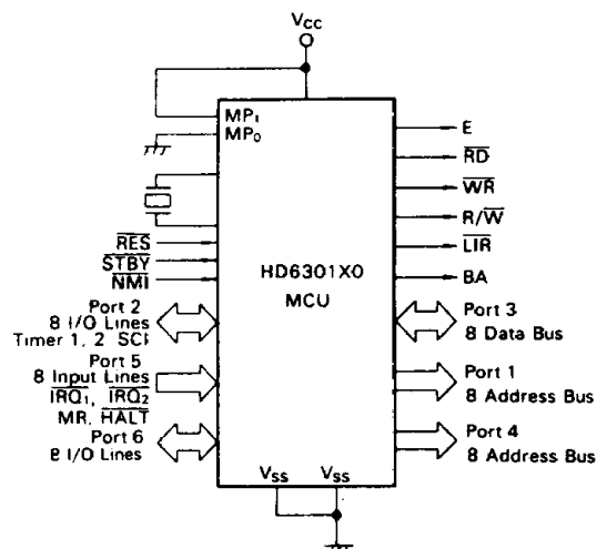
Figure 16 Mode 2
