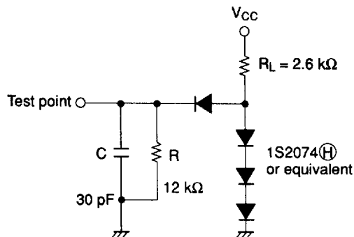
Figure 37 Timing Load Circuit
