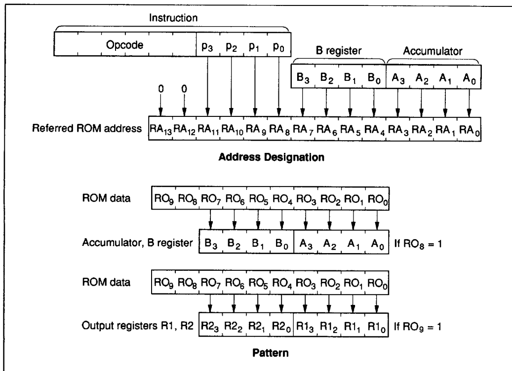
Figure 24 P Instruction
