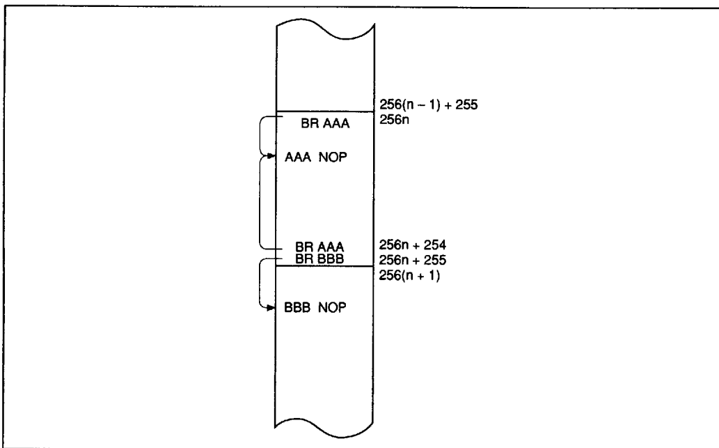
Figure 23 BR Instruction Branch Destination on a Page Boundary
