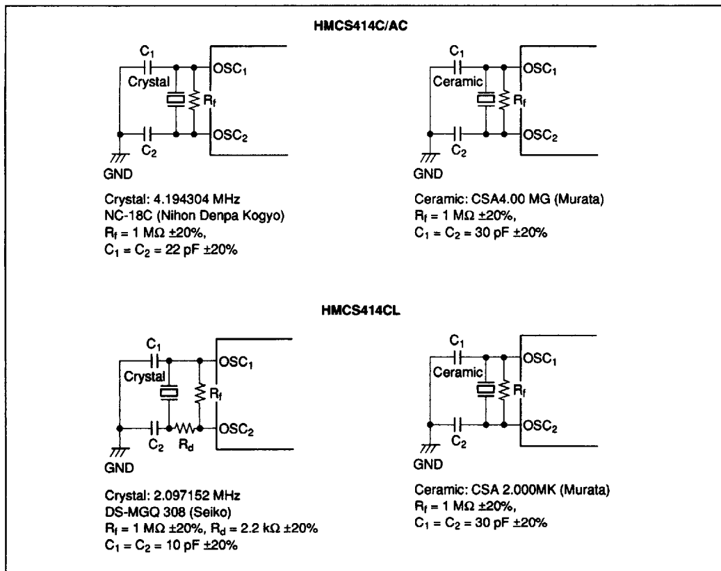
Figure 29 Oscillation Circuits
