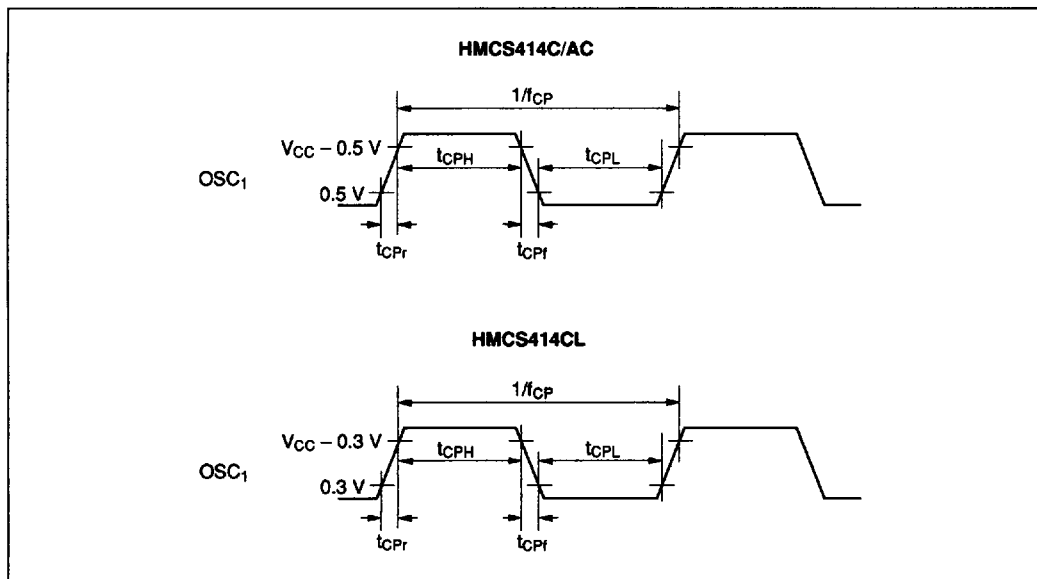
Figure 30 Oscillator Timing
