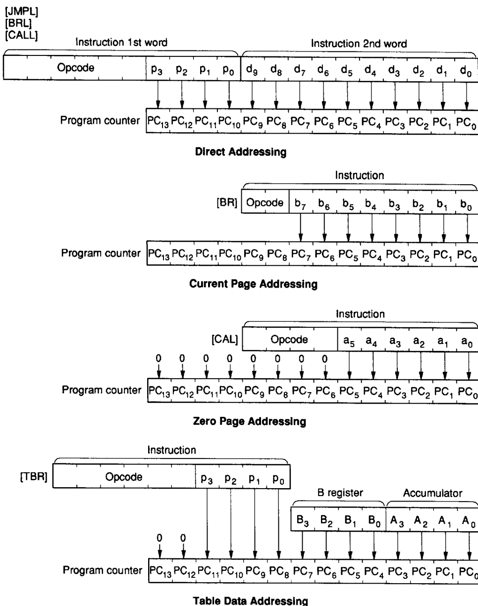
Figure 22 ROM Addressing Modes
