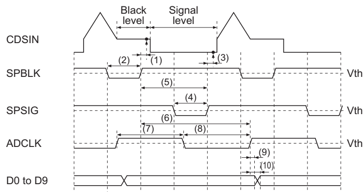
Figure 3 Detailed Timing Chart when CDSIN Input Mode is Used
