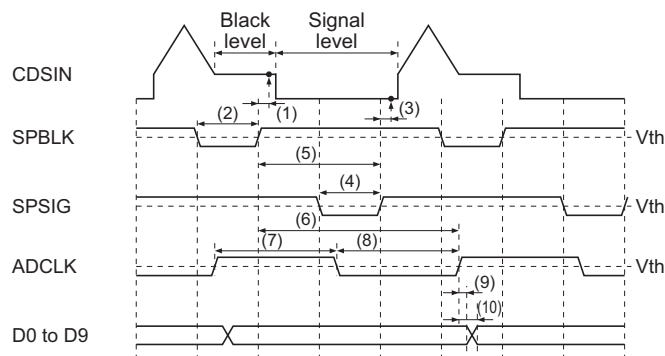
Figure 3 Detailed Timing Chart when CDSIN Input Mode is Used
