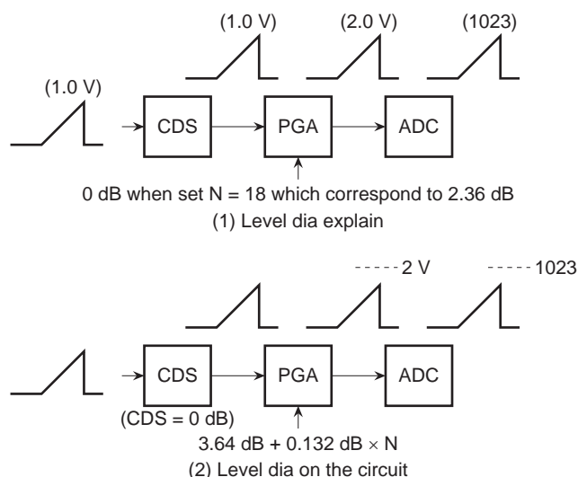
Figure 9 Level Dia of PGA
