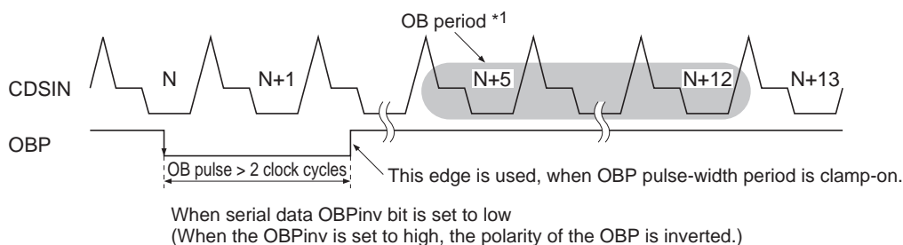
Figure 4 OBP Detailed Timing Specifications
