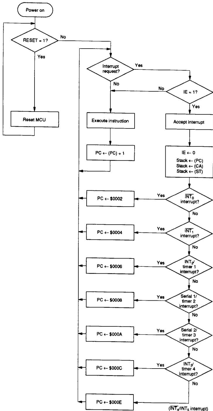
Figure 8 Interrupt Processing Flowchart
