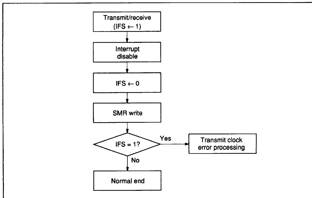
Figure 27 Transmit Clock Error Detection
