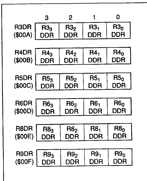
Figure 17 R3 to R9 Port Data Direction Registers
