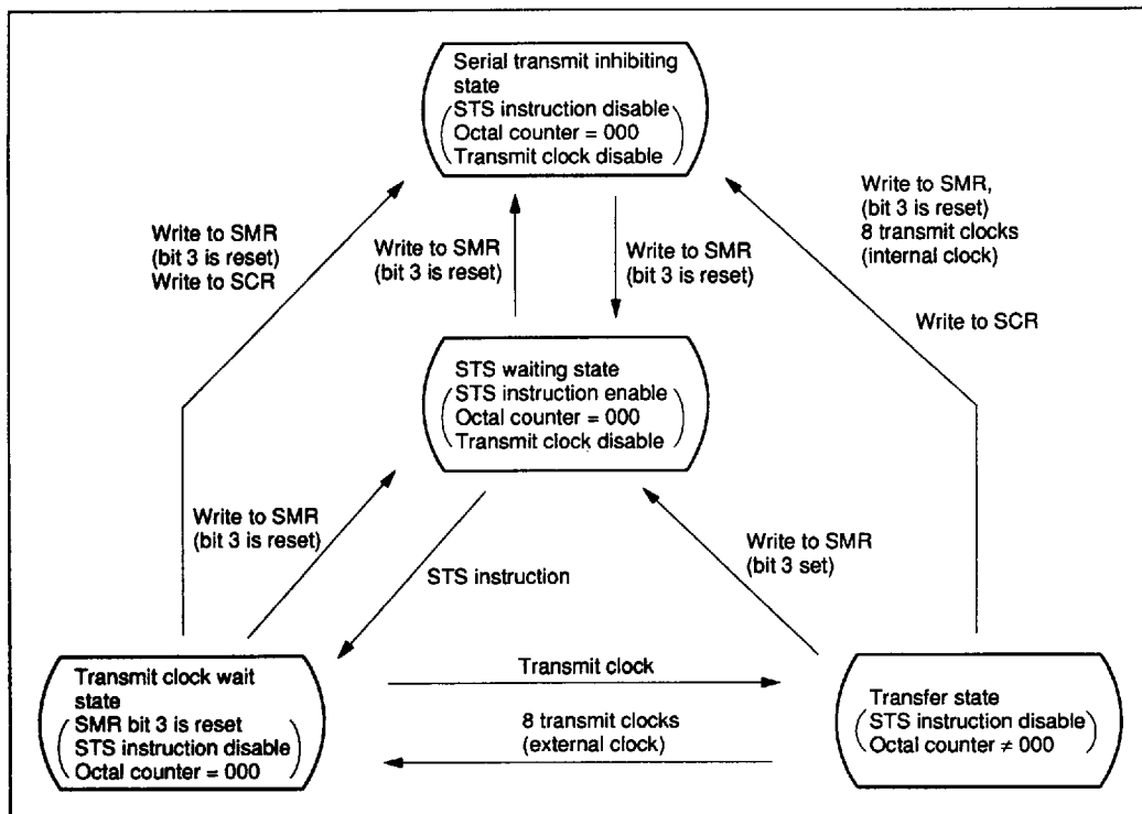
Figure 26 Serial Interface Operation State
