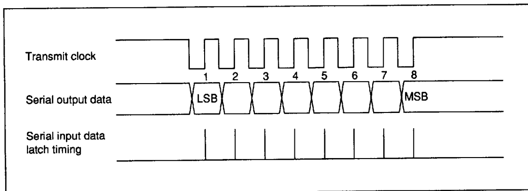
Figure 25 Serial Interface I/O Timing
