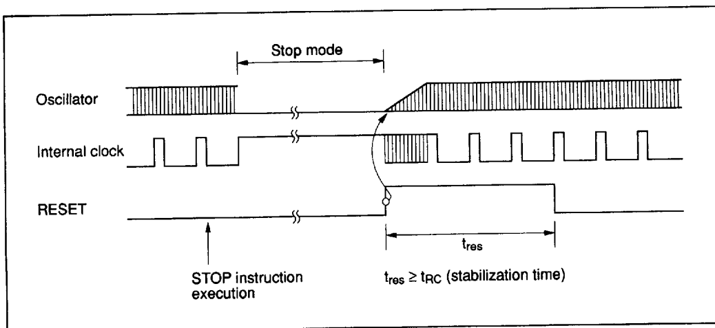
Figure 11 Timing of Stop Mode Cancellation
