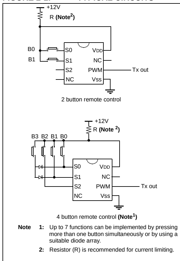
FIGURE 2-1: TYPICAL CIRCUITS
