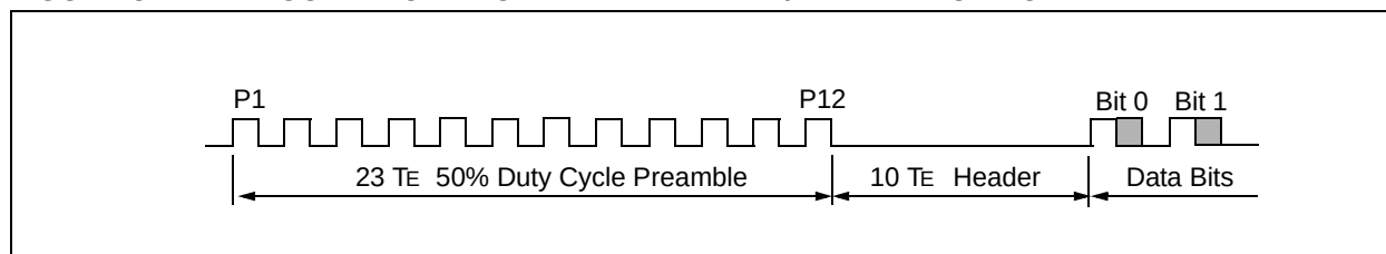
FIGURE 8-4: CODE WORD FORMAT: PREAMBLE/HEADER PORTION
