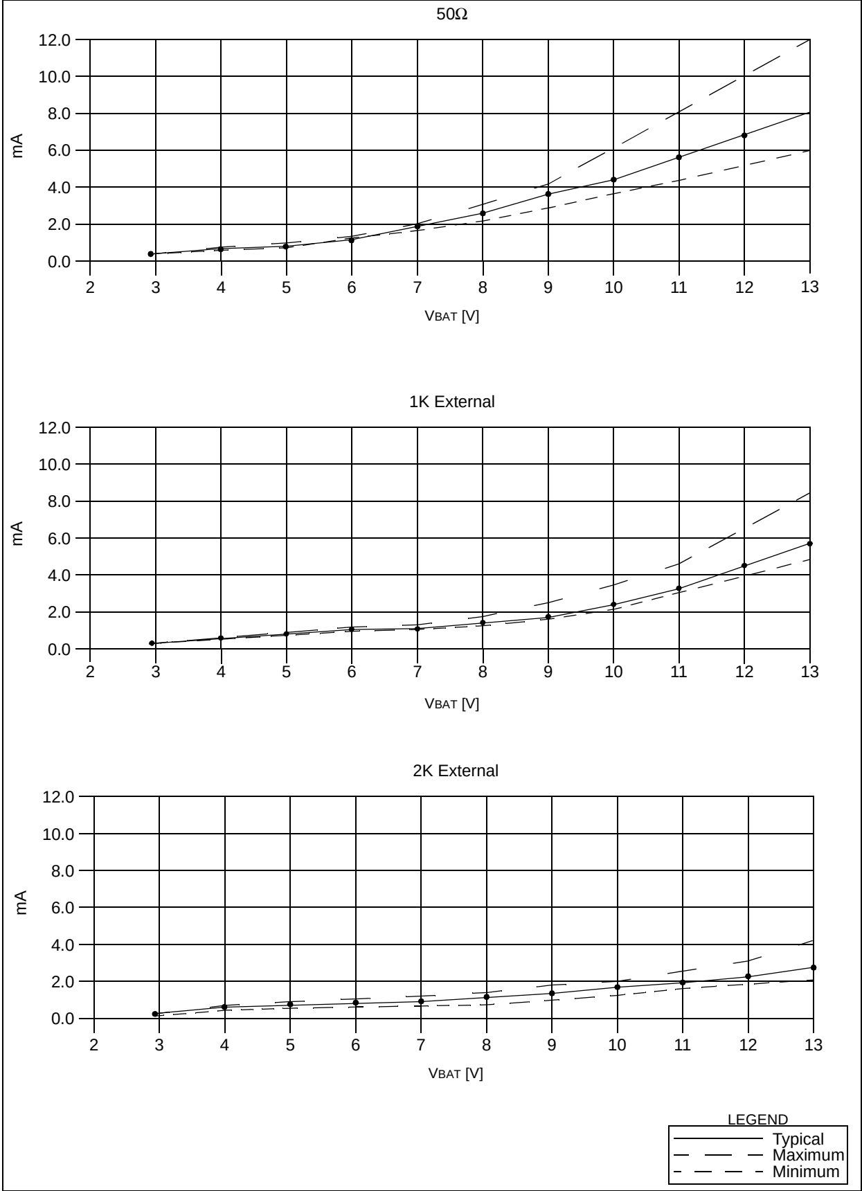
FIGURE 8-1: TYPICAL ICC CURVE OF HCS200 WITH EXTERNAL RESISTORS
