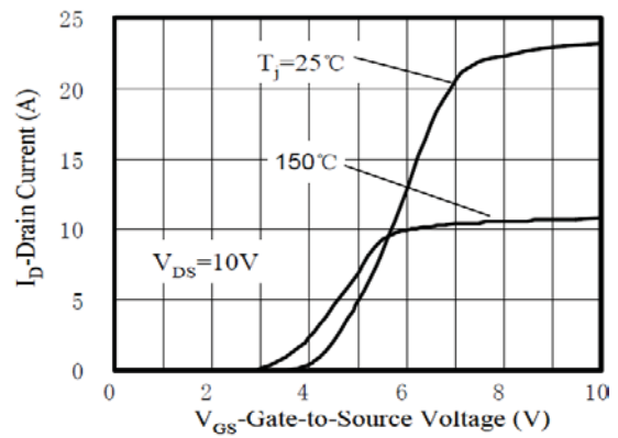
Figure 2. Transfer Characteristics
