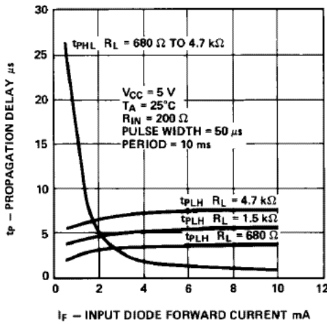
Figure 7 Propagation Delay vs. Input Diode Forward Current
