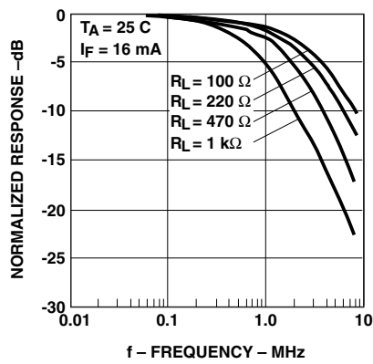
Figure 8. Frequency response.
