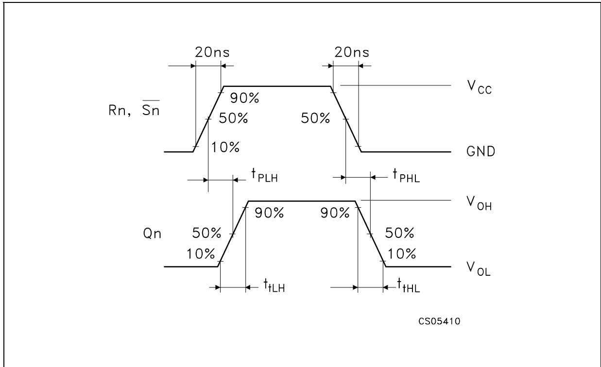
WAVEFORM 1: PROPAGATION DELAY TIMES ( f=1\text{MHz} ; 50% duty cycle)
