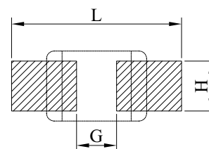
PCB PATTERN
