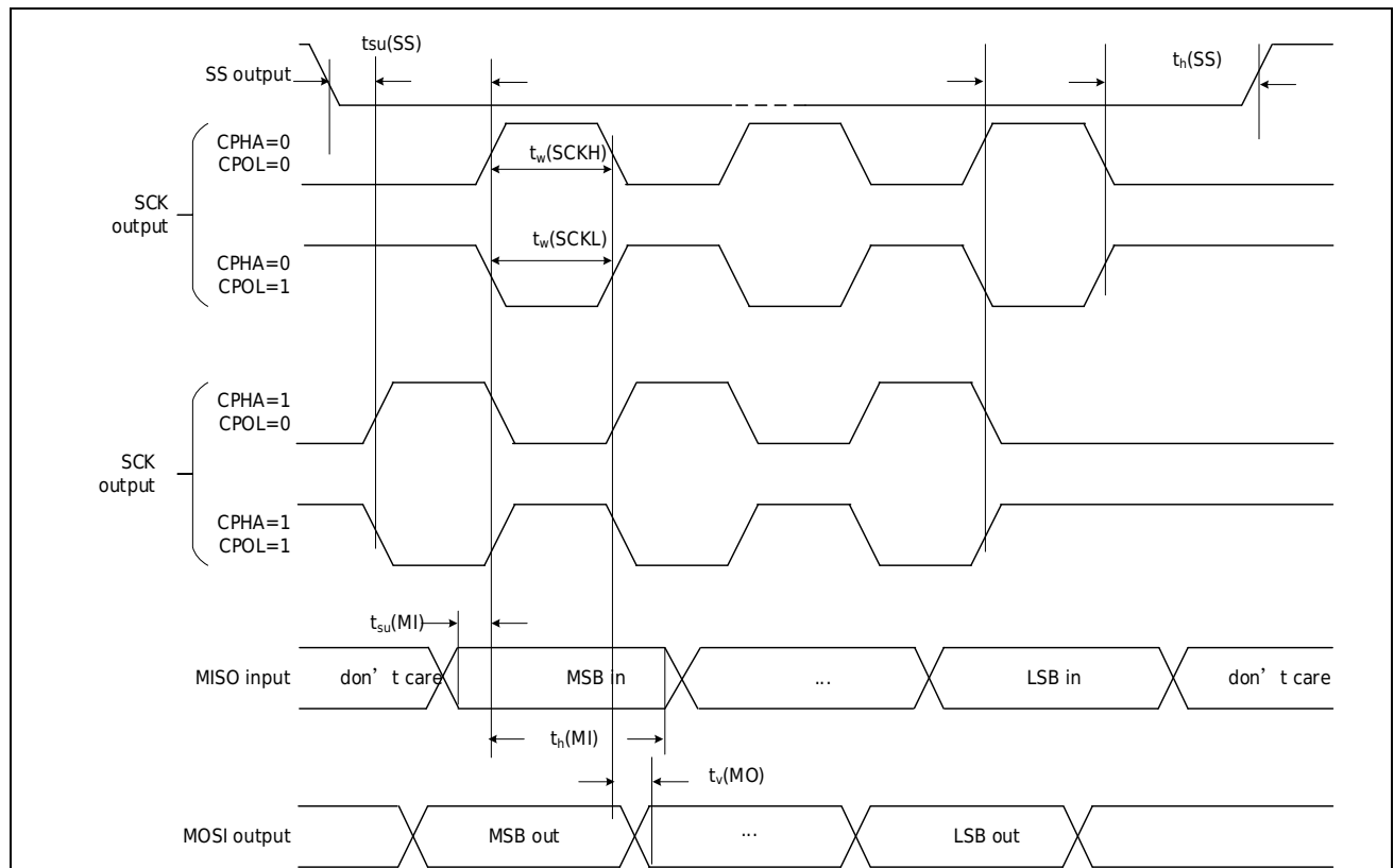
Figure 3-12 SPI timing diagram -host mode
