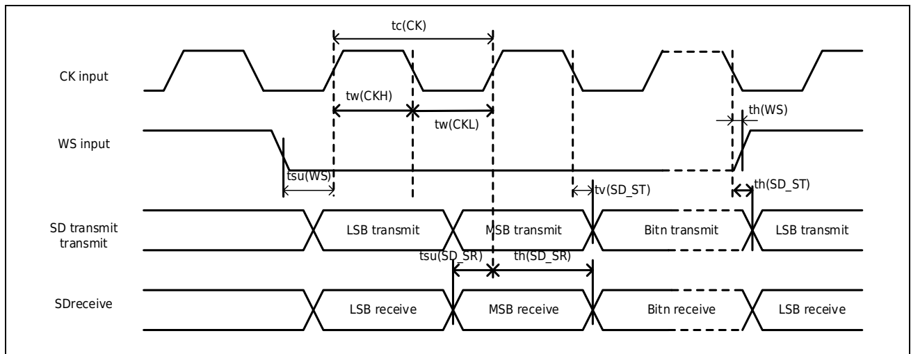
Figure 3-15 I2S slave mode timing (Philips protocol)
