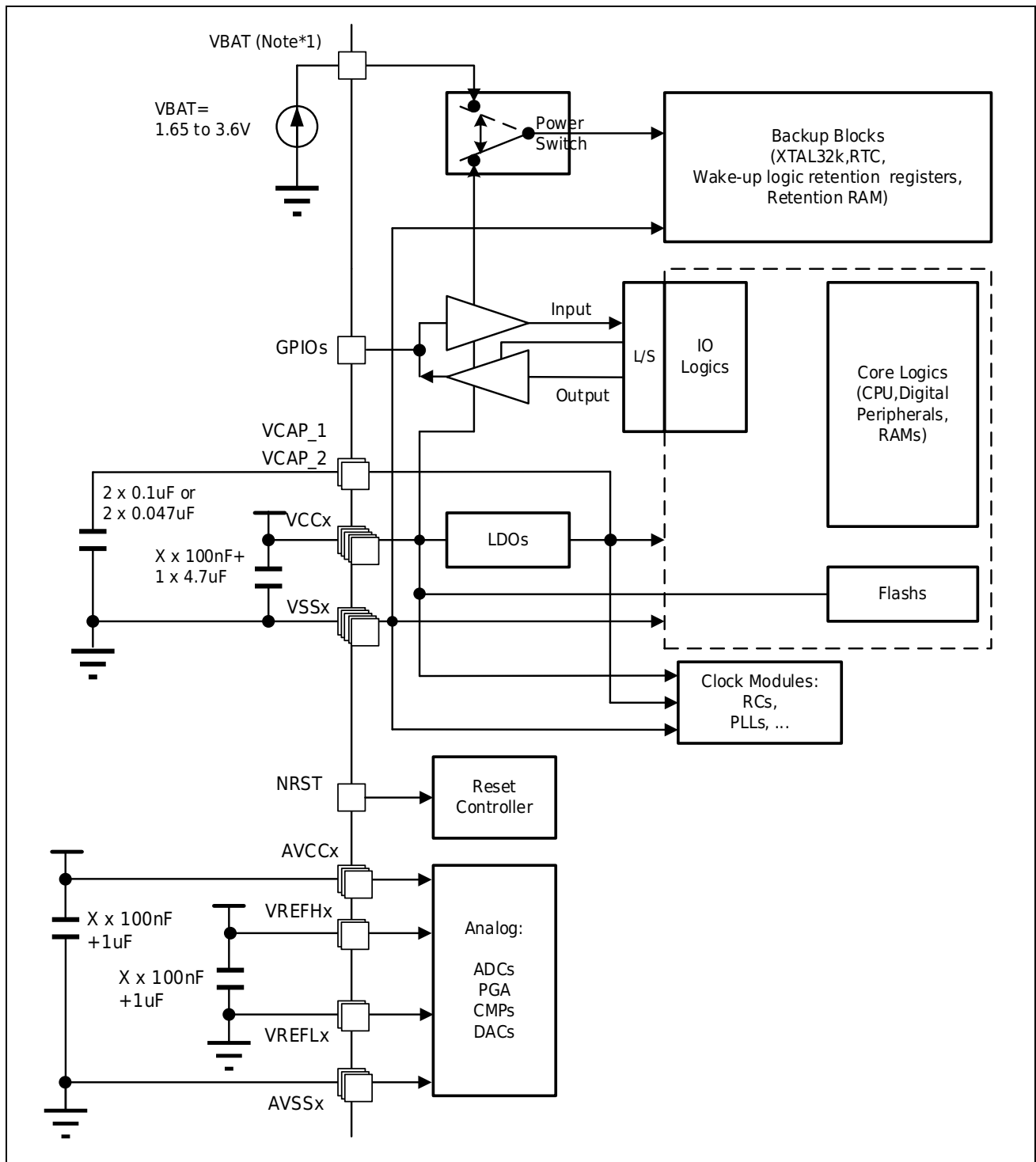
Figure 3-2 Power scheme
