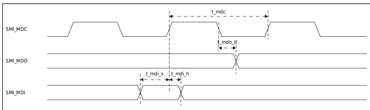
Figure 3-19 ETHMAC-SMI interface timing diagram
