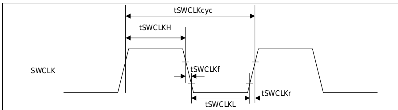
Figure 3-27 SWD SWCLK clock
