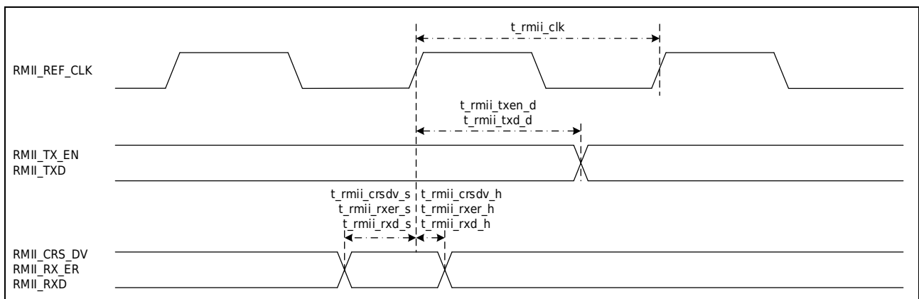
Figure 3-22 ETHMAC-RMII interface timing diagram
