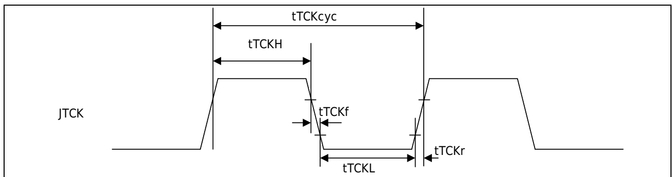
Figure 3-25 JTAG TCK clock
