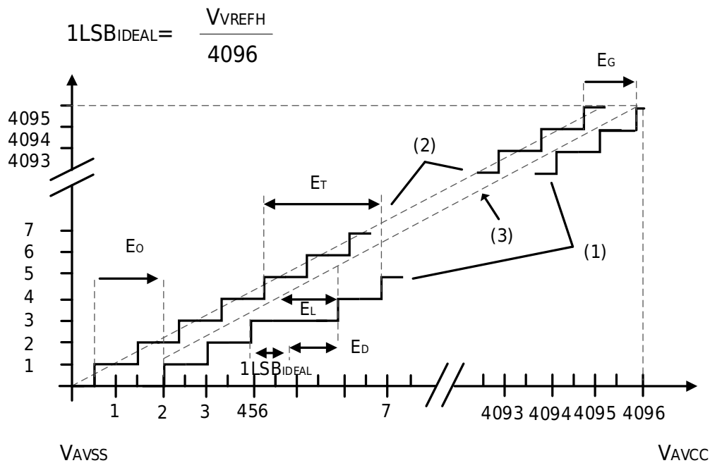
Figure 3-31 ADC Accuracy Characteristics
