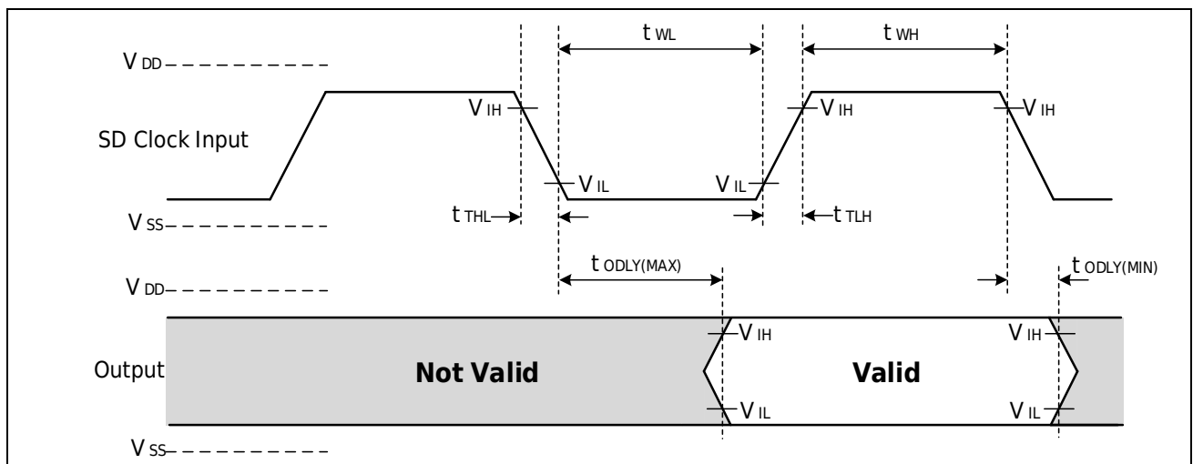
Figure 3-38 Default Speed Mode Output Timing Diagram
