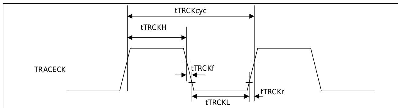
Figure 3-29 TRACE clock
