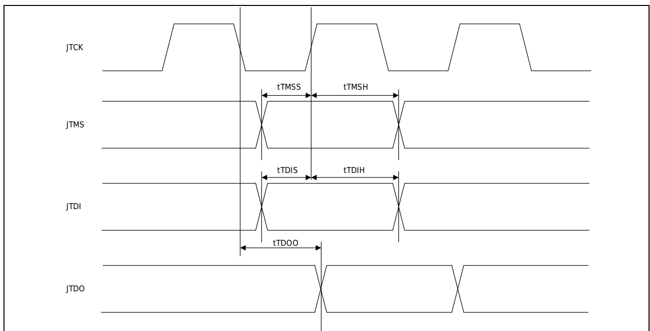
Figure 3-26 JTAG input and output
