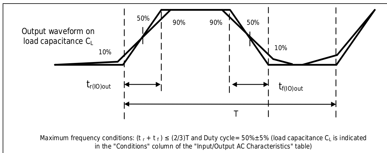
Figure 3-8 I/O AC Characteristics Definition
