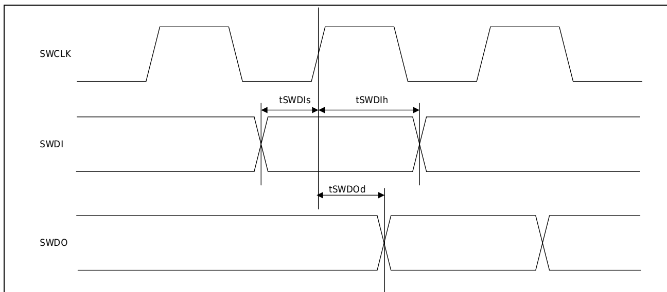
Figure 3-28 SWDIO input and output
