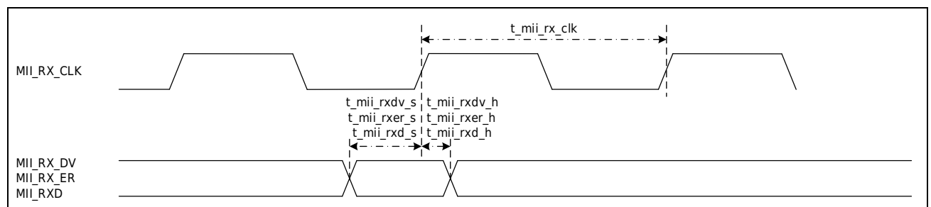
Figure 3-21 ETHMAC-MII interface input signal timing diagram
