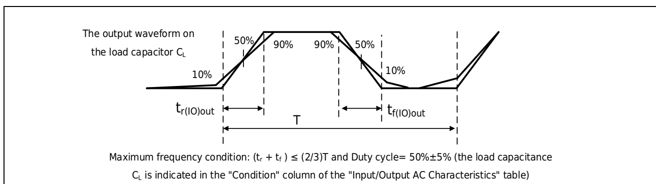
Figure 3-6 Definition of I/O AC Characteristics
