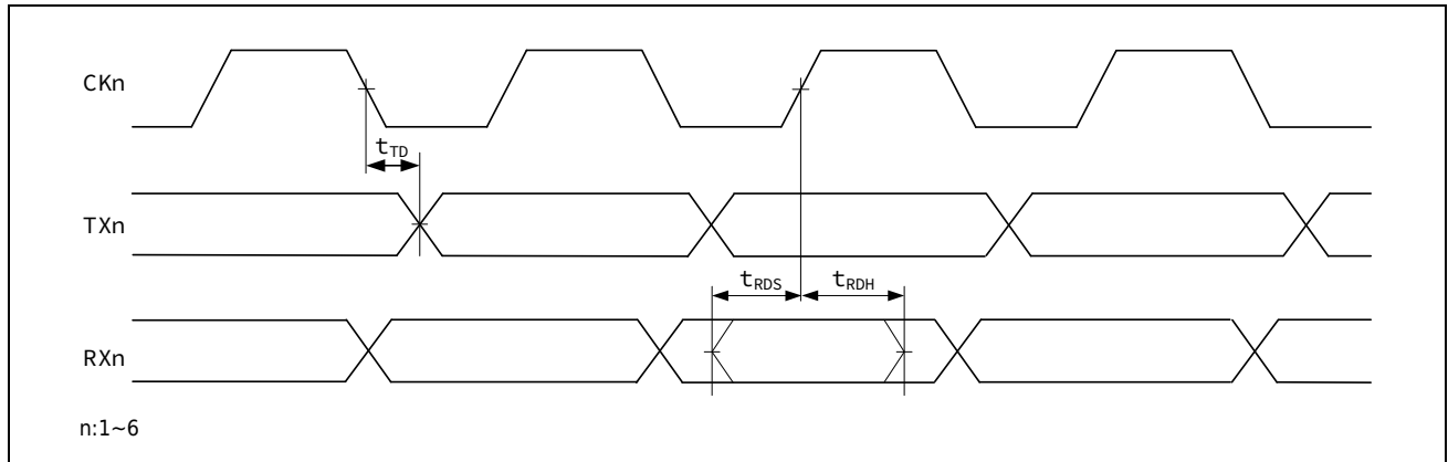
Figure 3-14 USART (CSI) Input and Output Timing
