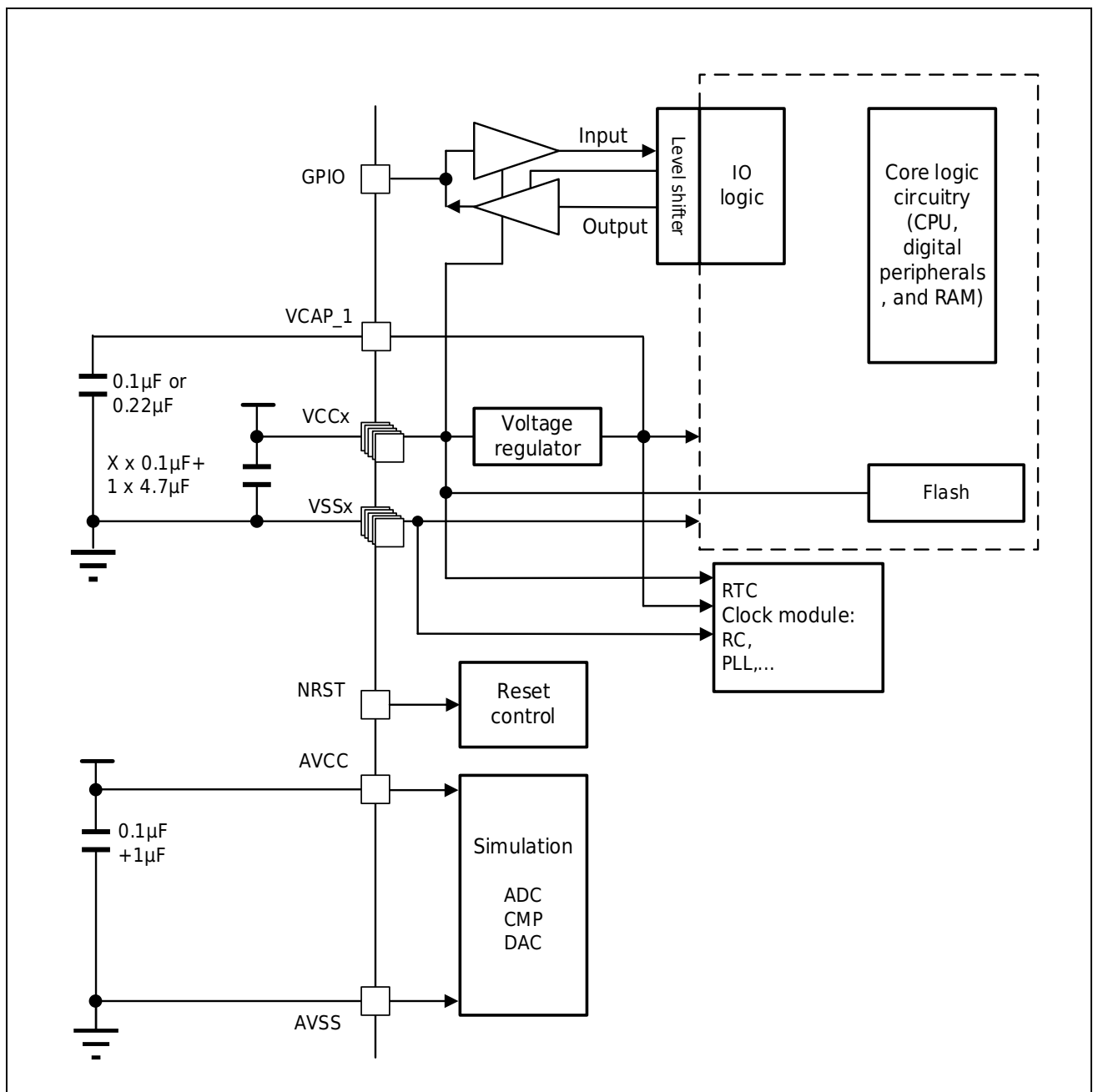
Figure 3-2 Power Scheme
