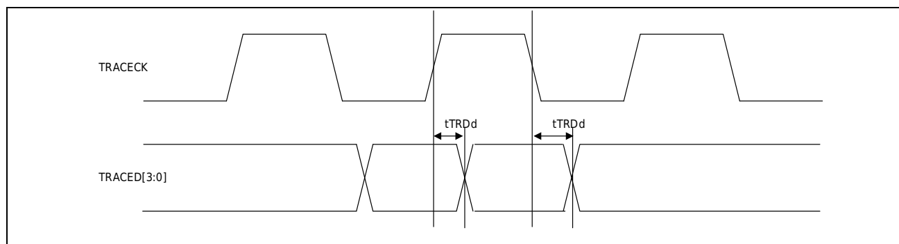
Figure 3-20 TRACE Data Output
