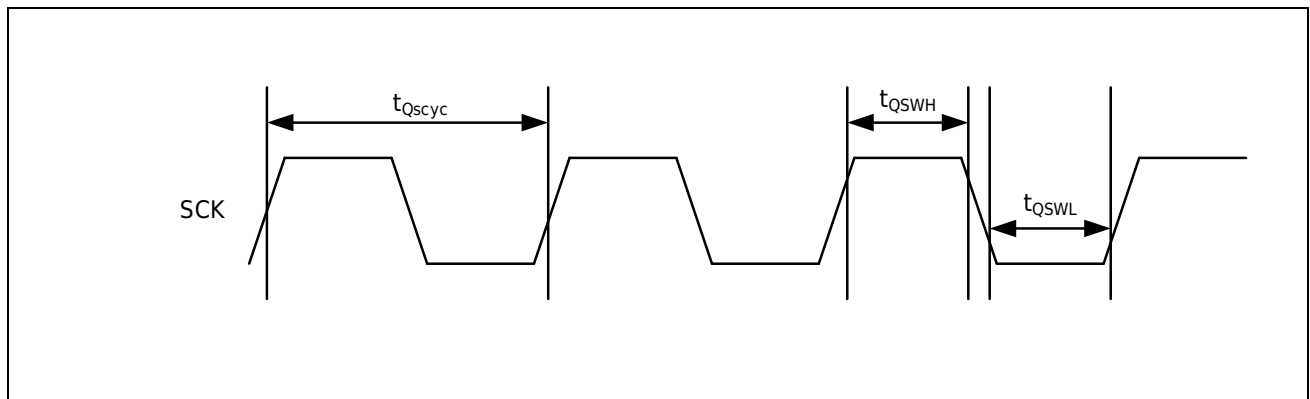
Figure 3-11 QSPI Clock Timing
