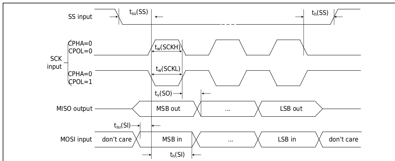
Figure 3-8 SPI timing definition (slave mode, CPHA=0)
