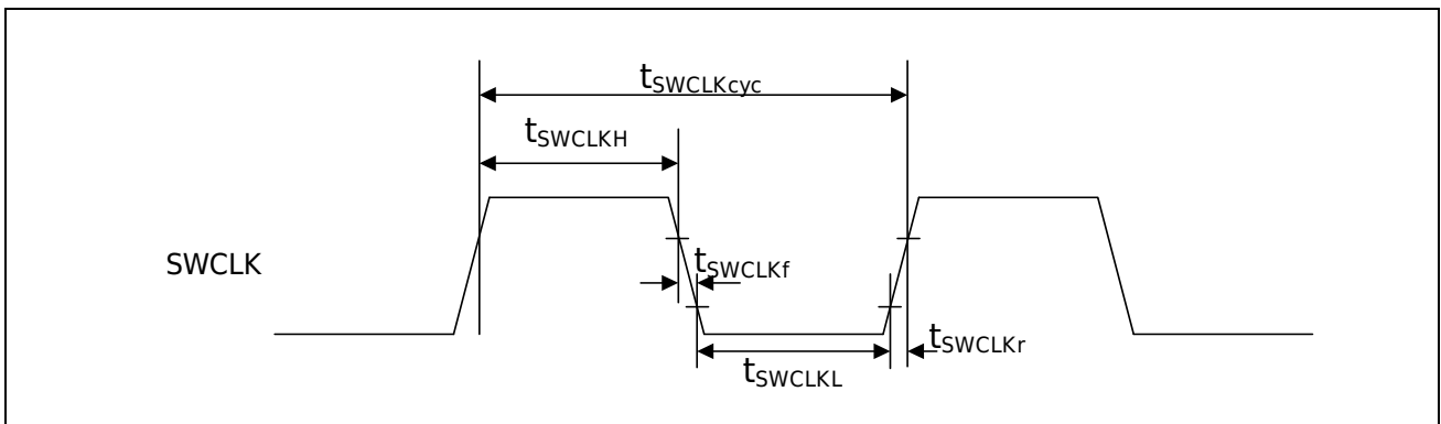
Figure 3-17 SWD SWCLK Clock
