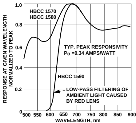
Figure 5. Relative Spectral Response of Sensors.
