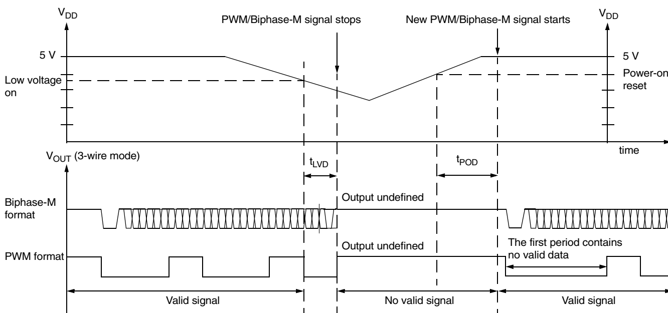
Fig. 4-8: Power-drop operation
