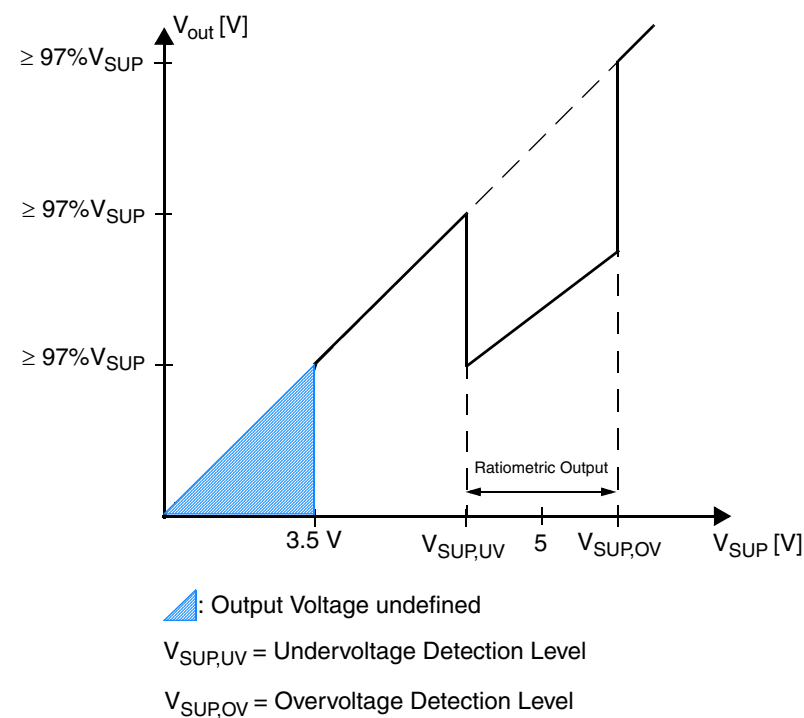
Fig. 4–5: Analog output behavior for different supply voltages
