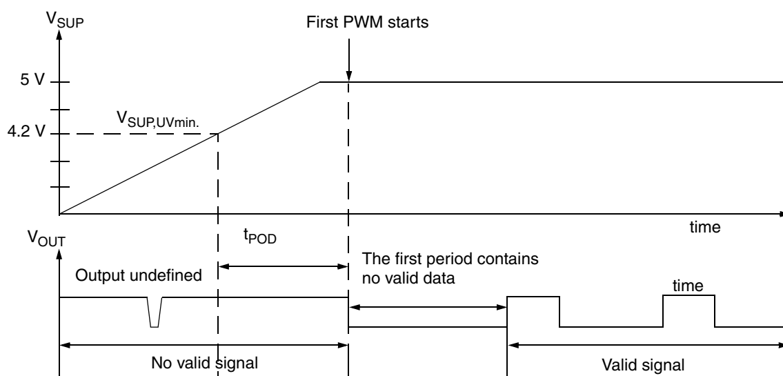
Fig. 4–6: Power-up behavior of HAL835 with PWM output activated
