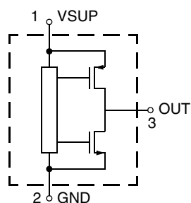
Fig. 4-3: Pin configuration
