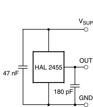
Fig. 5-1: Recommended application circuit
