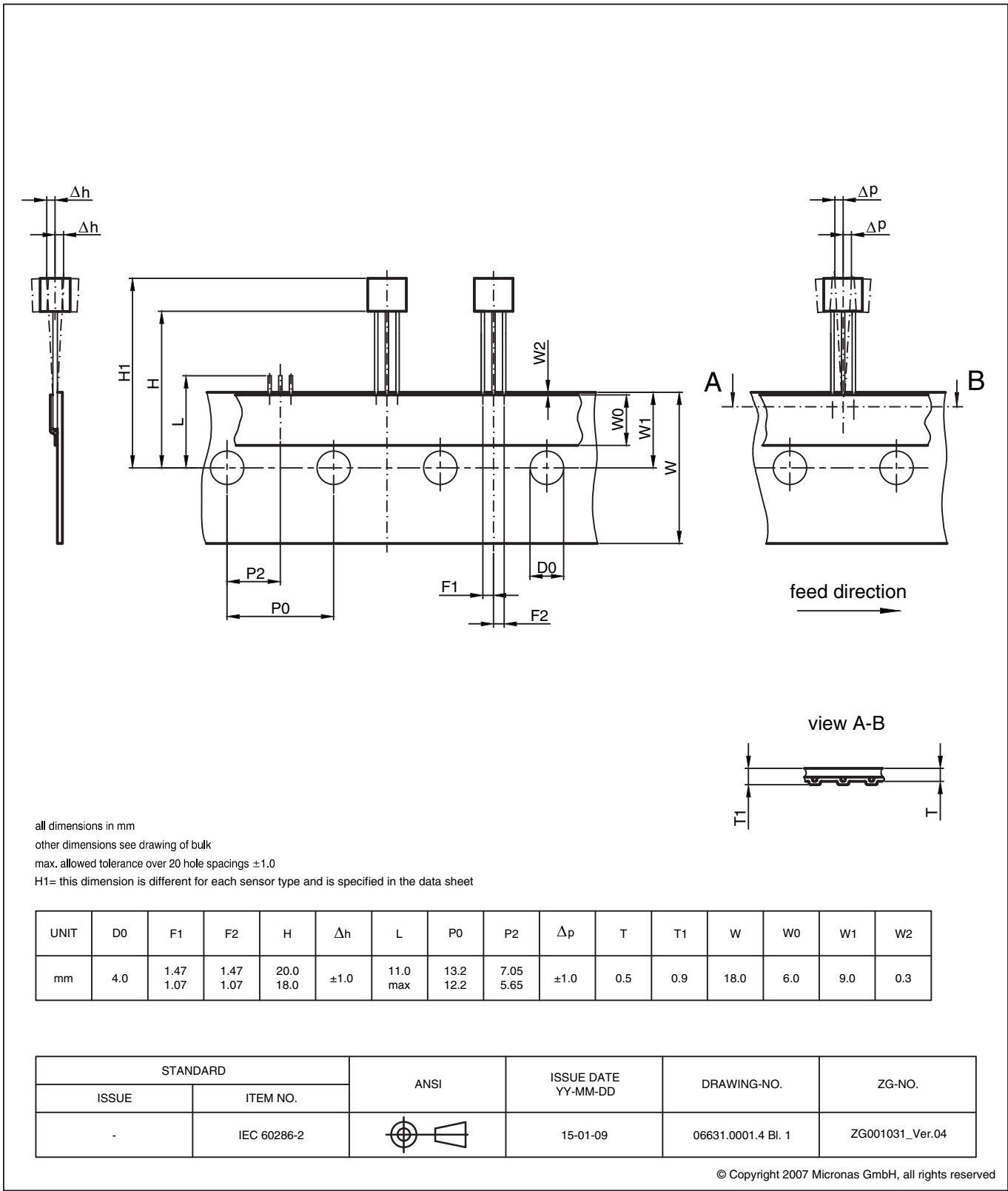
Fig. 4-5: TO92UA/UT: Dimensions ammpack inline, not spread
