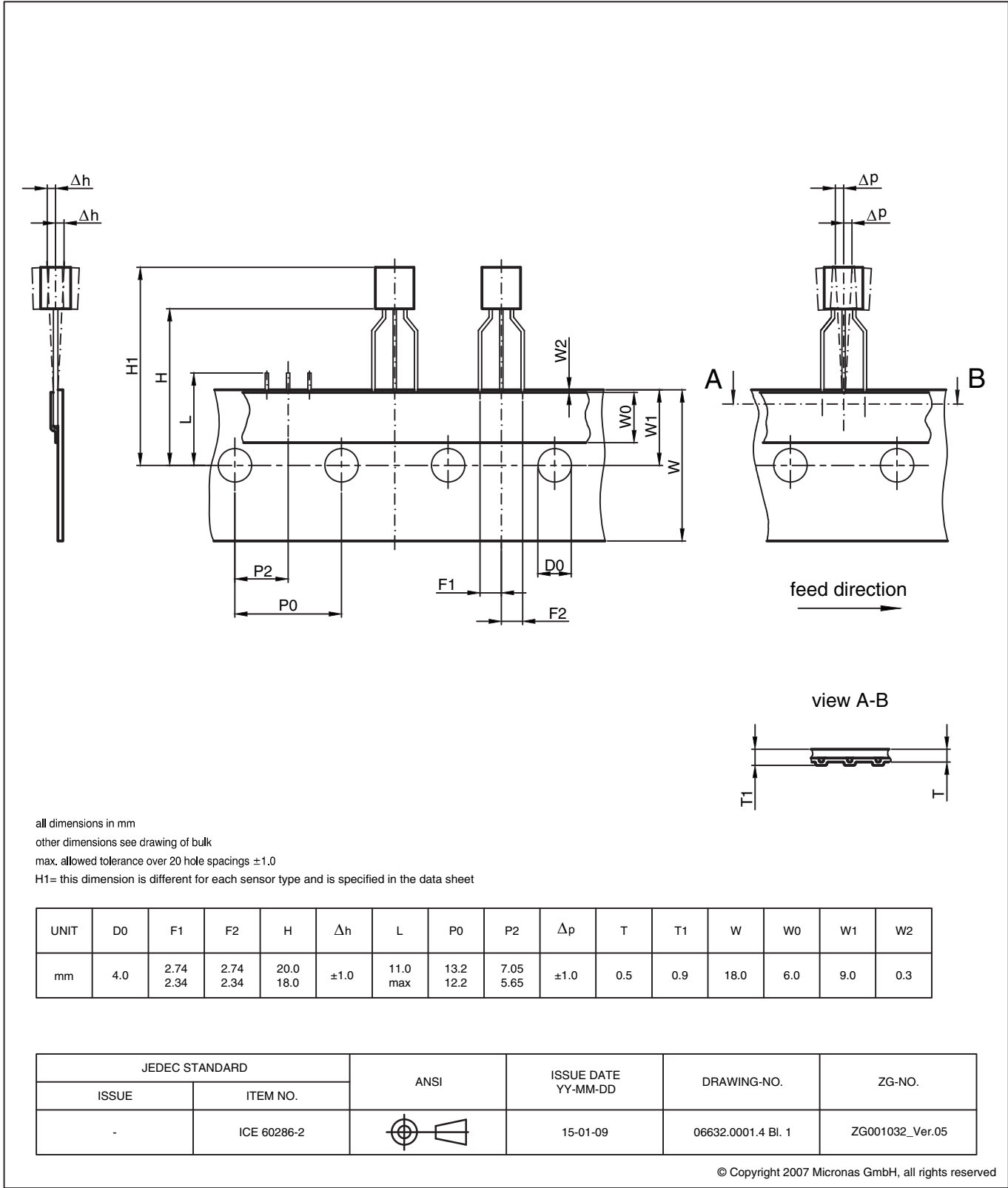
Fig. 4-6: TO92UA/UT: Dimensions ammopack inline, spread
