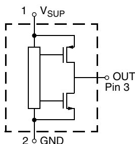
TO92UT package
