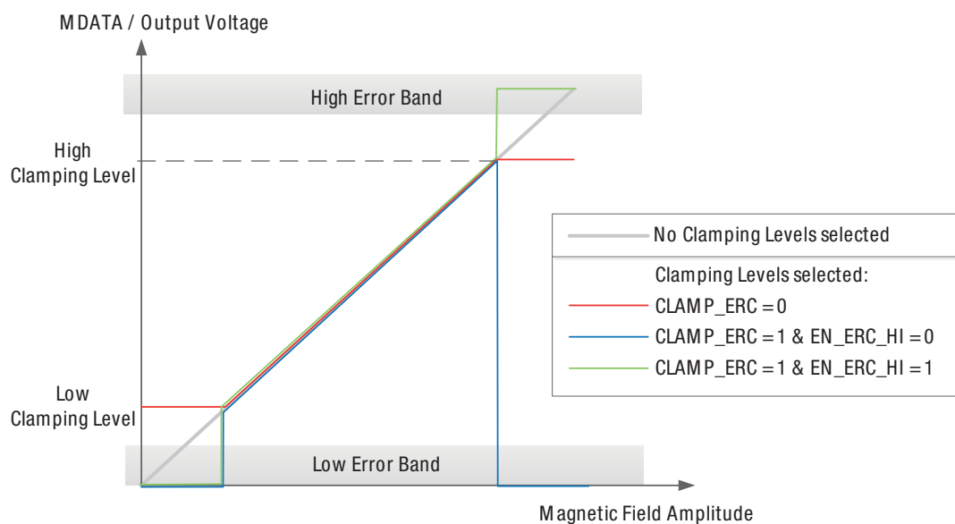
Fig. 3–3: Clamping levels HAL 1880
