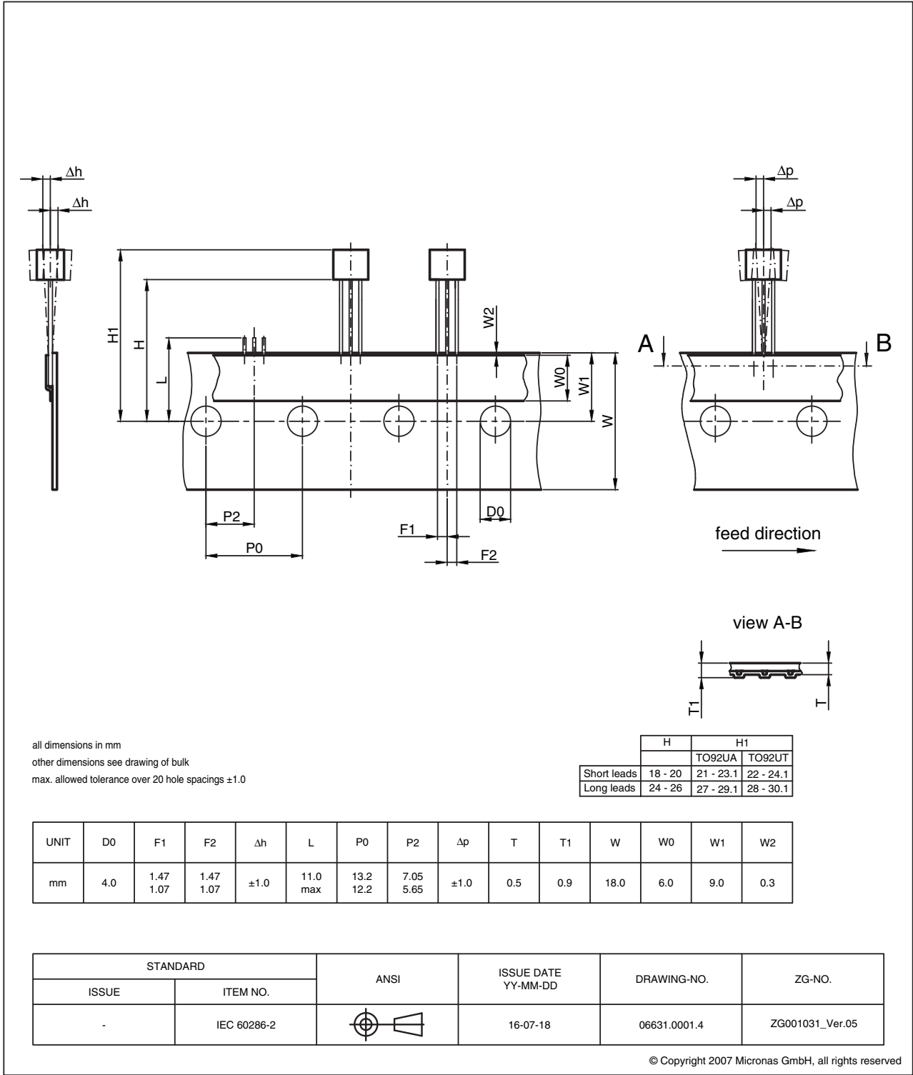
Fig. 4-2: TO92UA: Dimensions ammpack inline, not spread, standard lead length
