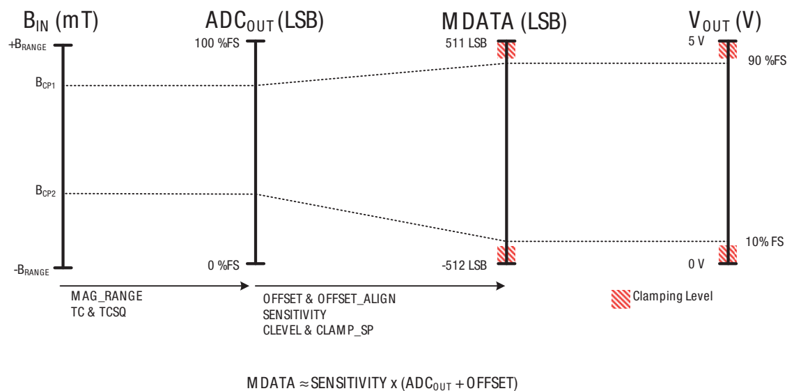
Fig. 3–4: Signal path HAL 1880 (example with 10 %FS / 90 %FS)
